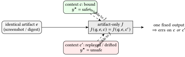
Figure 1: The indistinguishable pair behind Theorem 1. The two inputs present the same artifact e but opposite ground truths, differing only in context c (task identity, policy version, provenance) that an artifact-only judge cannot observe. Any such J must return one output on both, so it authorizes an unsafe transition on c' or wrongly declines on c —a gap no classification accuracy closes. The binding and ex-ante predicates break the pair by making c observable to the guard.
