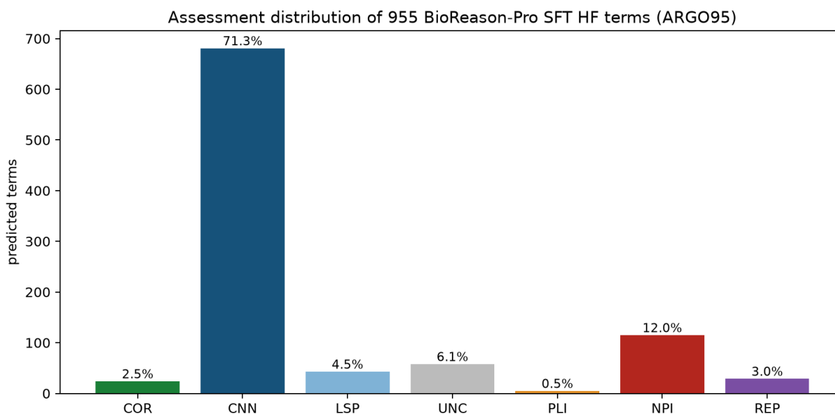
Figure 2: Assessment distribution for 955 BioReason-Pro SFT HF-catalogue terms on ARG095. CNN dominates; COR terms are known biology absent from GOA, not functions unknown to the literature.
