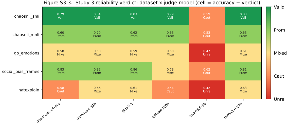
Figure 11: Study 3. Dataset×judge-model reliability verdict (cell = accuracy + verdict). The scale effect (qwen3.5-9b column) and the construct-subjectivity gradient (rows) are both visible.
