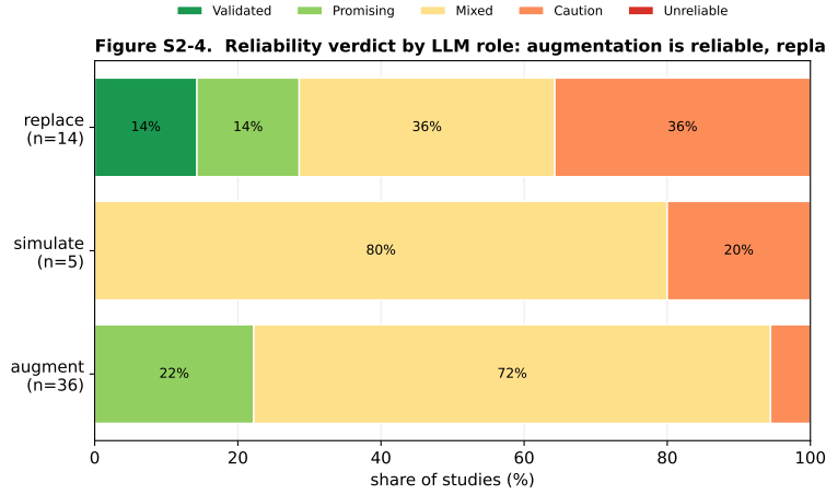
Figure 8: Study 2. Reliability verdict by LLM role. Augmentation is reliable; replacement is reliable only for objective annotation; participant/usability simulation is the least reliable.
