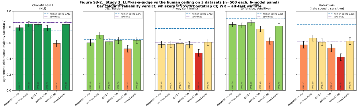
Figure 10: Study 3. Per-dataset accuracy vs the human ceiling (blue dashed) for the 6-model panel (n=500 each; whiskers = 95% bootstrap CI; bar colour = verdict; WR = alt-test winning rate). Datasets ordered by construct subjectivity. LLMs clear LOW ceilings (NLI) but fall short of HIGH ceilings on subjective social-computing tasks.
