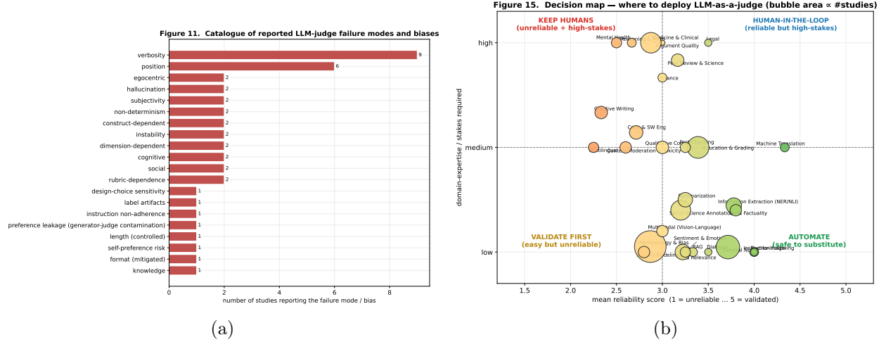
Figure 4: Study 1. (a) Catalogue of reported failure modes/biases. (b) Deployment decision map (reliability \times stakes; bubble area \propto studies).
