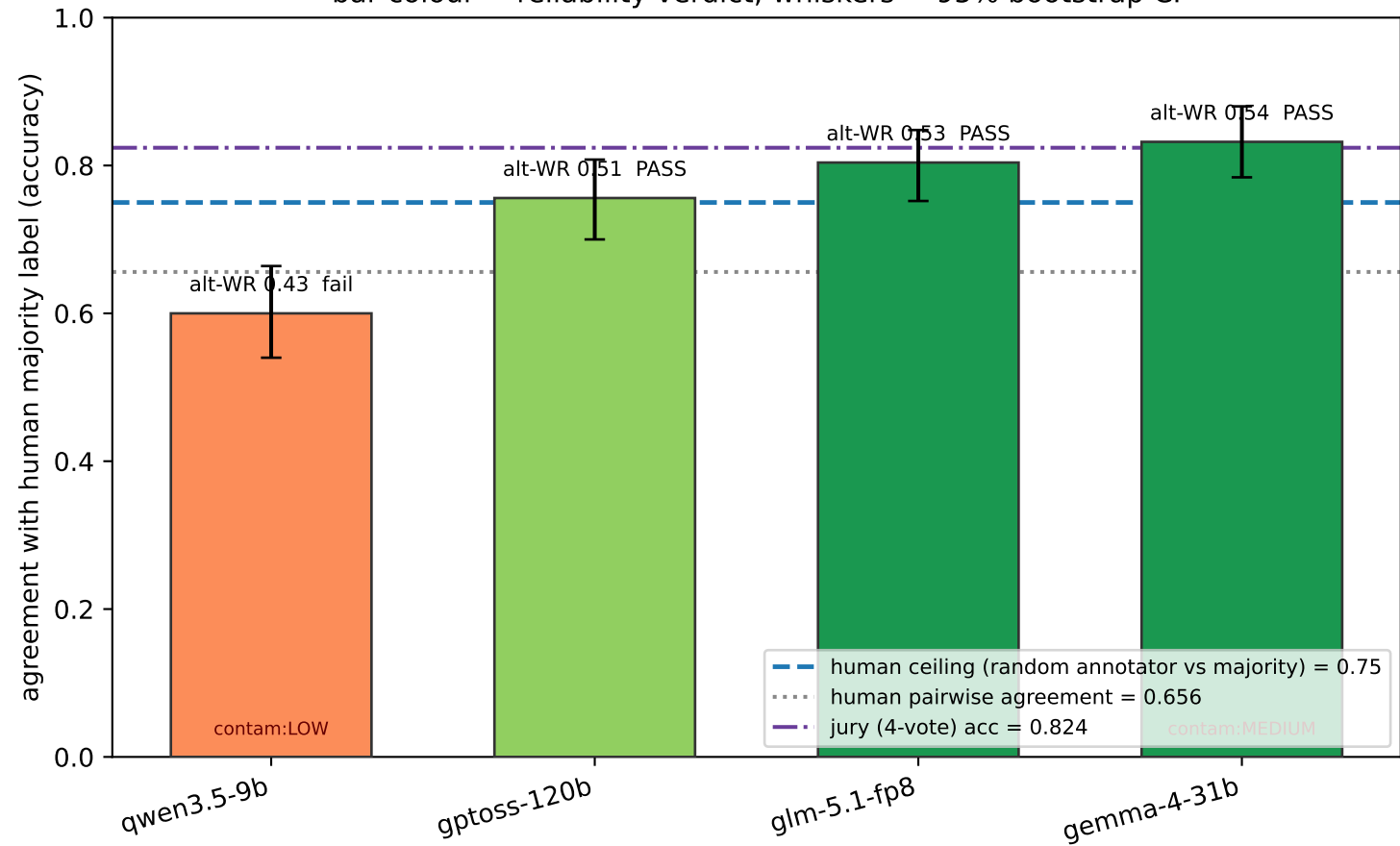
Figure S3-1 (pilot). LLM-as-a-judge vs the human ceiling on ChaosNLI (n=250) bar colour = reliability verdict; whiskers = 95% bootstrap CI
