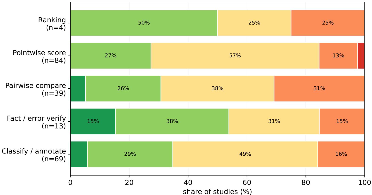
Figure 12. Reliability verdict by judging-task formulation
