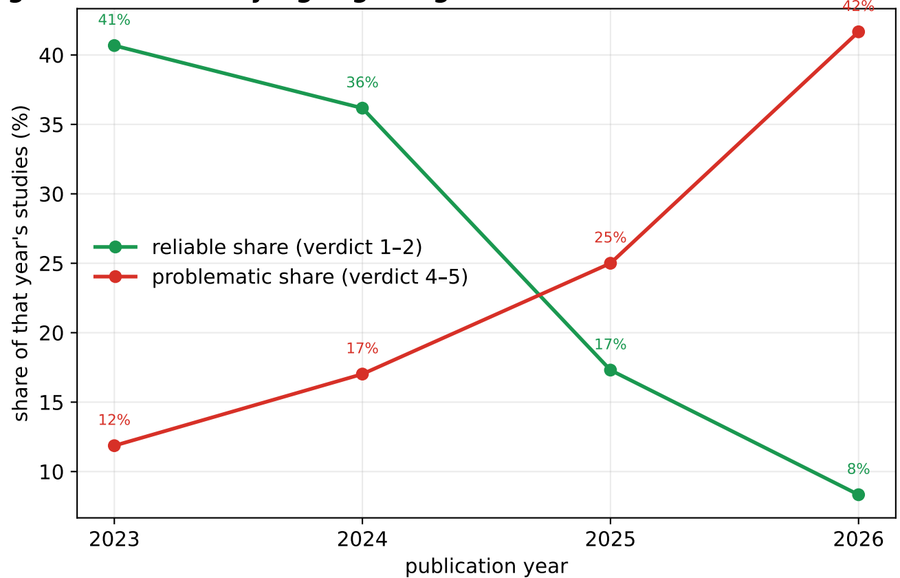
Figure 14. Are LLM judges getting more reliable? Verdict shares over time
