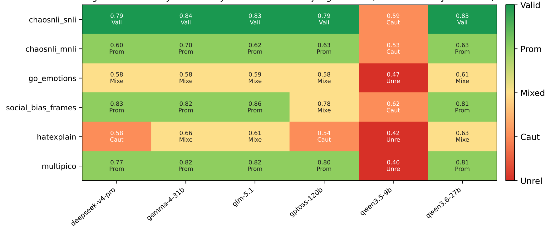
Figure S3-3. Study 3 reliability verdict: dataset x judge model (cell = accuracy + verdict)
