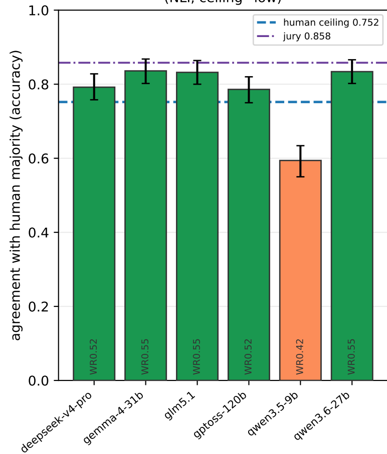
Figure S3-2. Study 3: LLM-as-a-judge vs the human ceiling on 3 datasets (n=500 each, 6-model panel)
