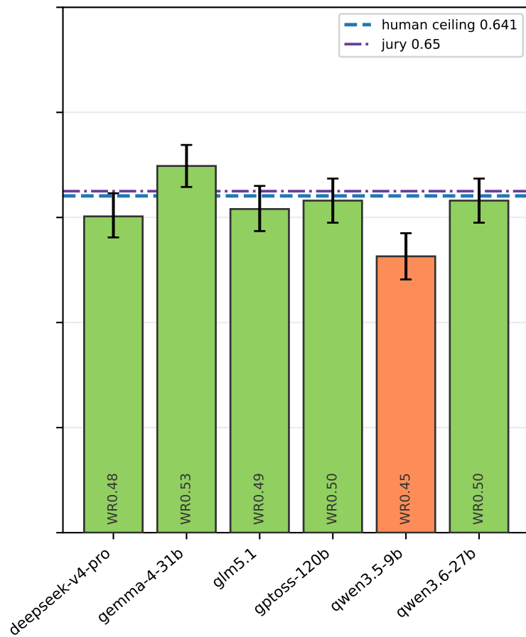
Figure S3-2. Study 3: LLM-as-a-judge vs the human ceiling on 3 datasets (n=500 each, 6-model panel)
