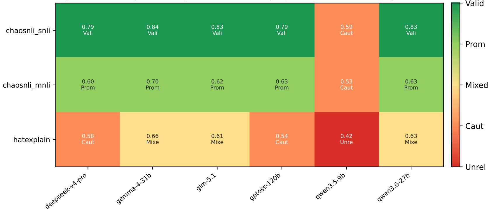
Figure S3-3. Study 3 reliability verdict: dataset x judge model (cell = accuracy + verdict)
