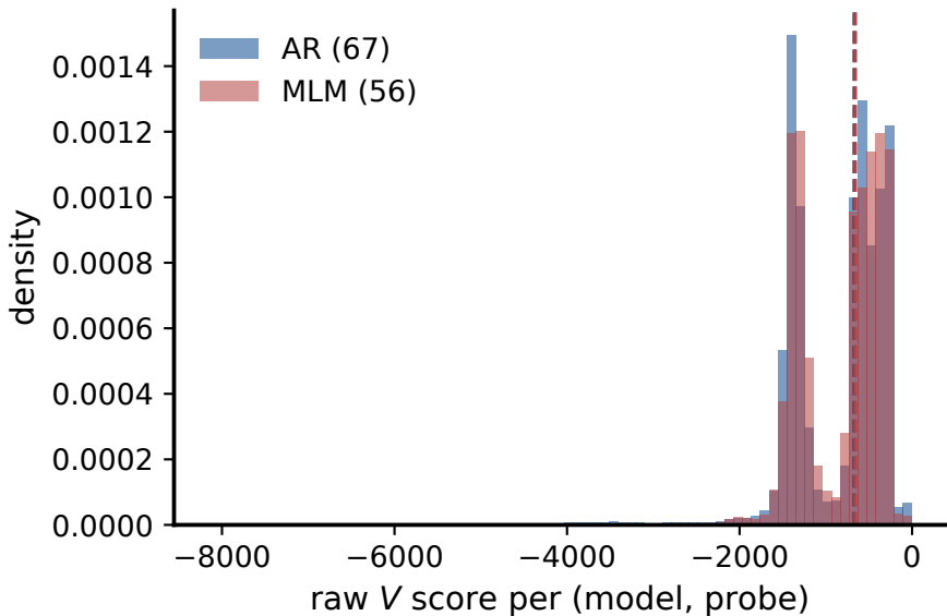
(a) Raw score scale before centering median ratio AR/MLM = 1.02
