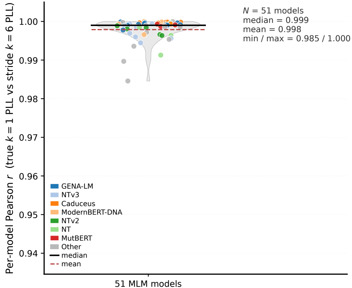
Per-model k = 1 vs k = 6 PLL correlation
