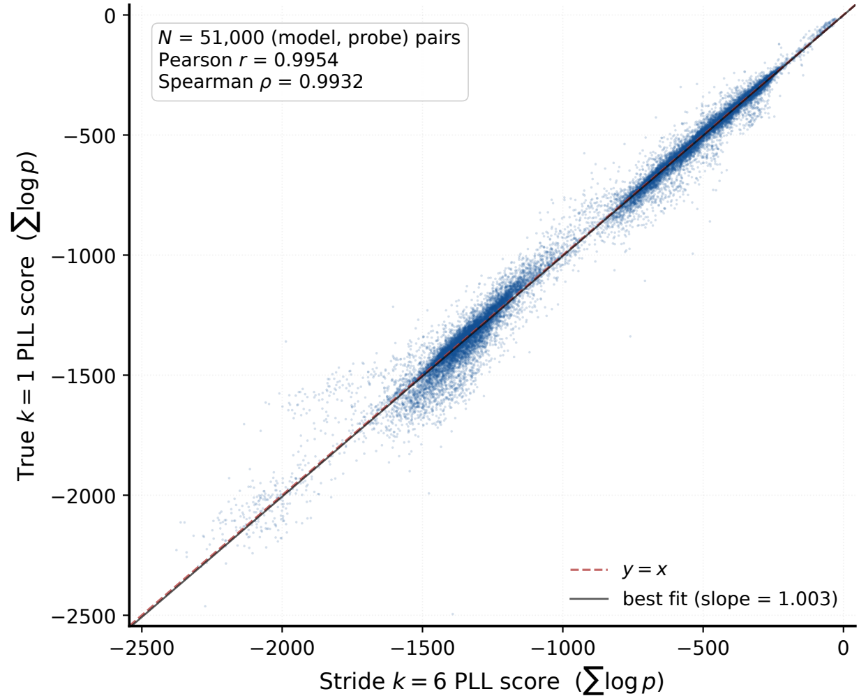
Pooled k = 1 vs k = 6 PLL scores
