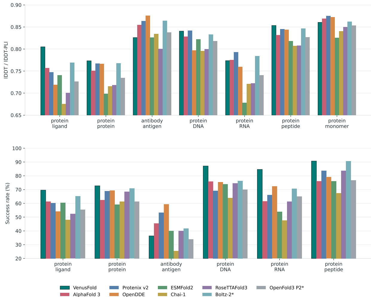
Figure 1 FoldBench evaluation across all nine models. Both panels use confidence-ranked predictions. DNA and RNA monomers are not included. Boltz-2 and OpenFold3 Preview 2 are post-cutoff references. ESMFold2 is sequence-only and was run without MSA input.
