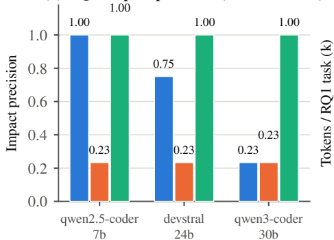
(b) RQ2: impact precision (recall = 1.00 \forall )
