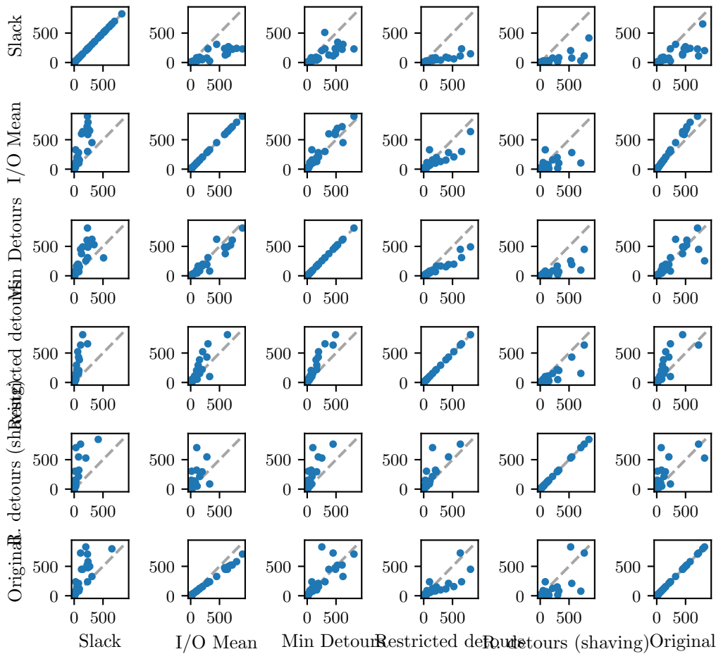
Runtime of one method against another (only on instances solved by both)
