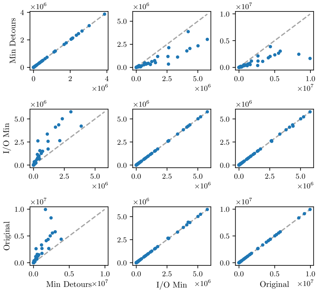
Number of nodes to prove optimality (only on instances solved by both)
