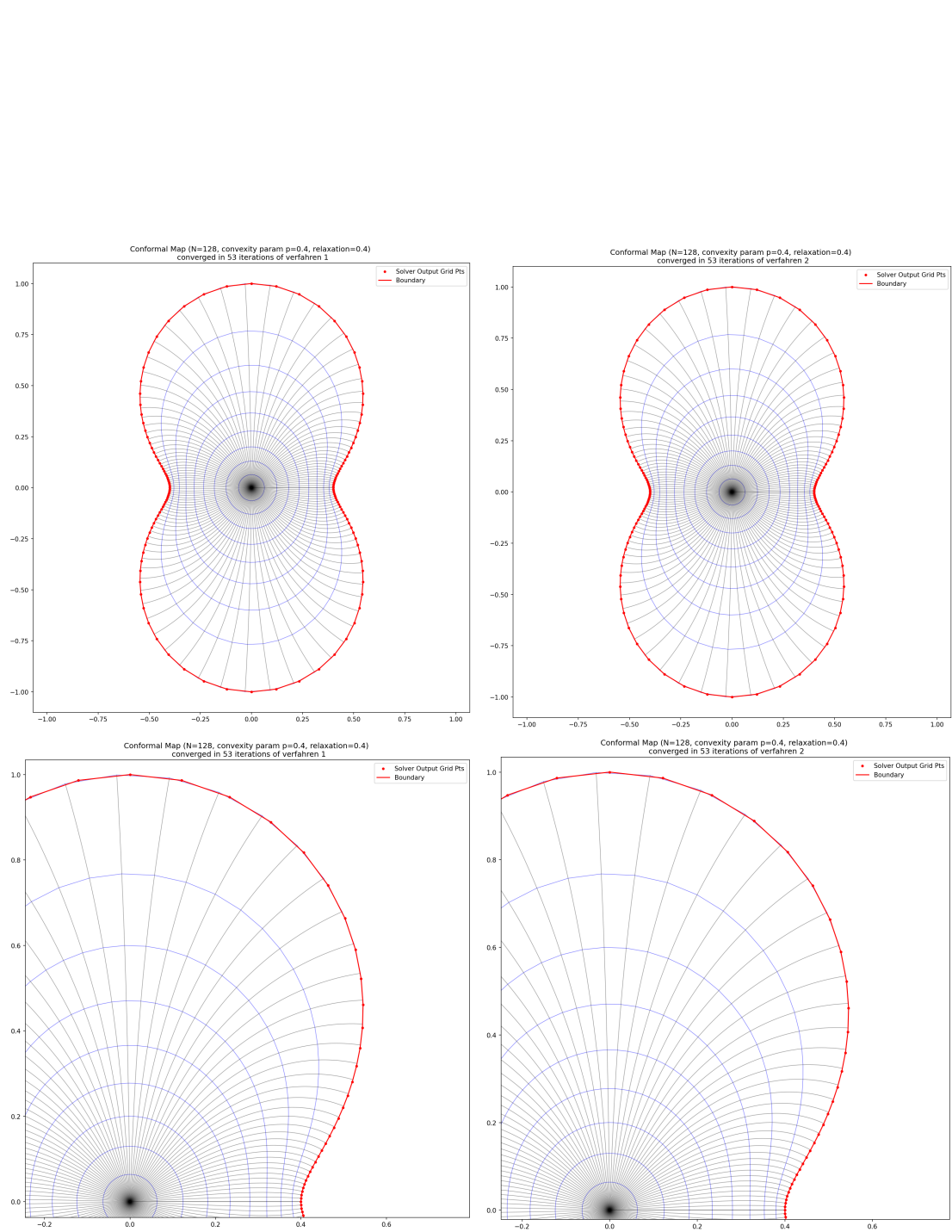
Figure 5: Gaier's inverted ellipse ut more convex. [Gai64, Anhang 5, p. 264]
