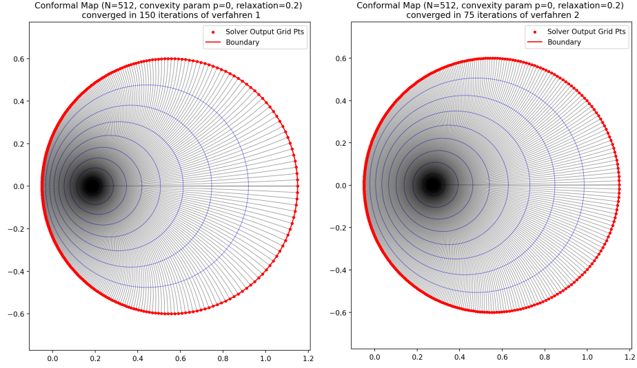
Figure 3: Gaier's eccentric circle [Gai64, Anhang 5, p. 264]
