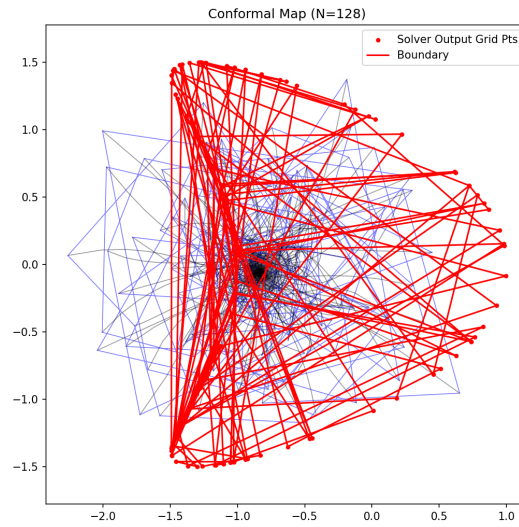
Figure 2: In this case, the initial guess was chosen to be a star, which shares some of the properties with the kite's tangent vector, but it is still too convex and therefore far away from the kite to guarantee convergence of the solver.
