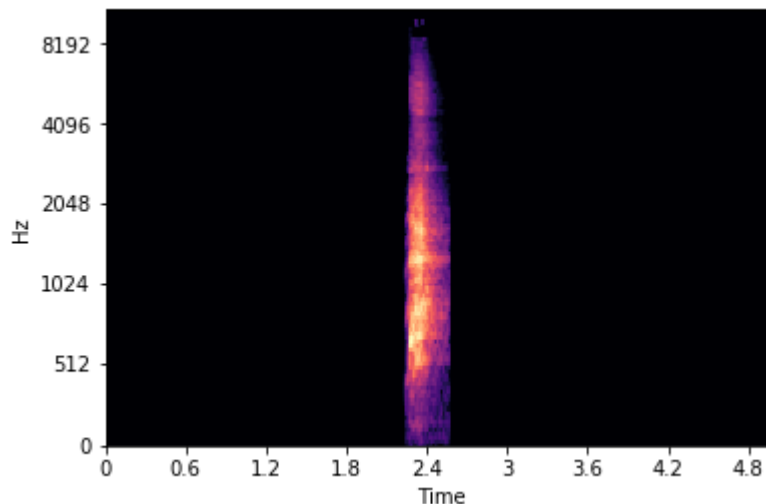
Figure 6-5. Log mel spectrogram
