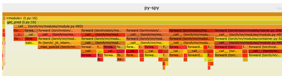
Figure 7-8. Flame graph on ResNet loading and inference
