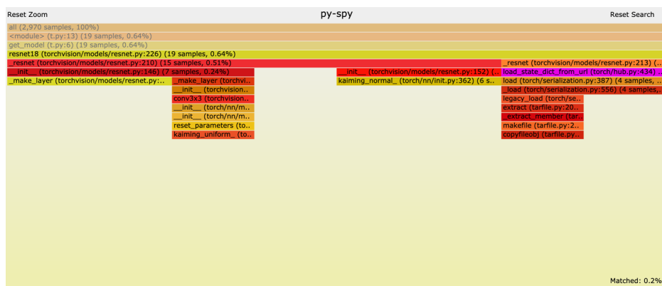
Figure 7-9. Zoomed flame graph
