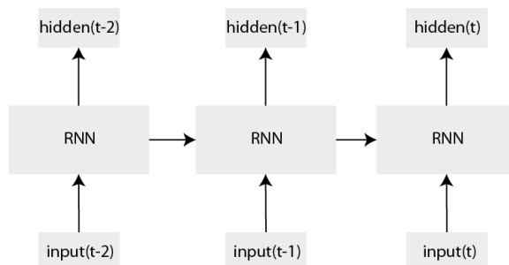
Figure 5-2. An unrolled RNN
