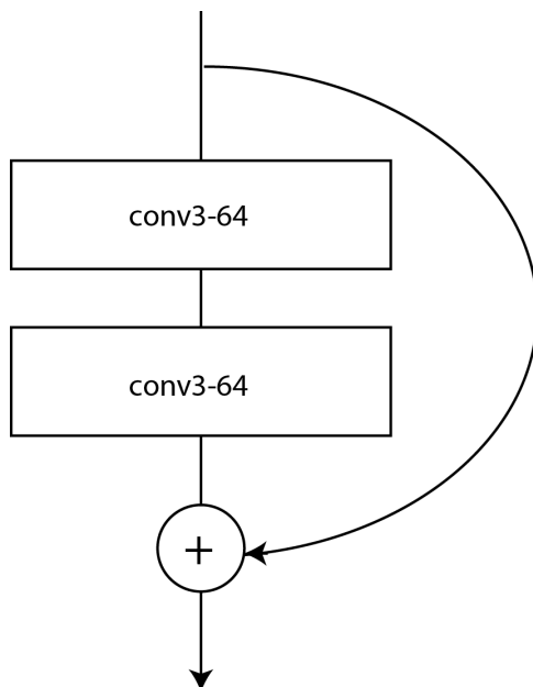
Figure 3-4. A ResNet block
