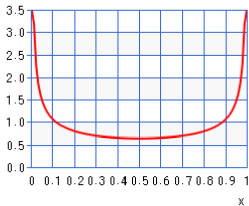
Figure 9-3. Beta distribution, where \alpha = \beta
