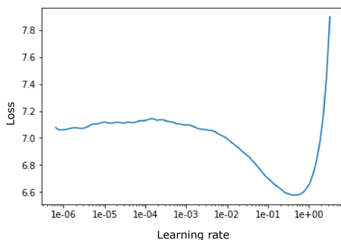
Figure 9-12. ULMFiT learning rate plot
