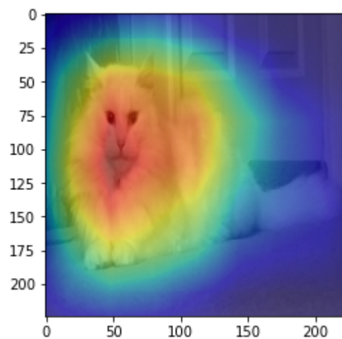
Figure 7-6. Class activation mapping with Casper
