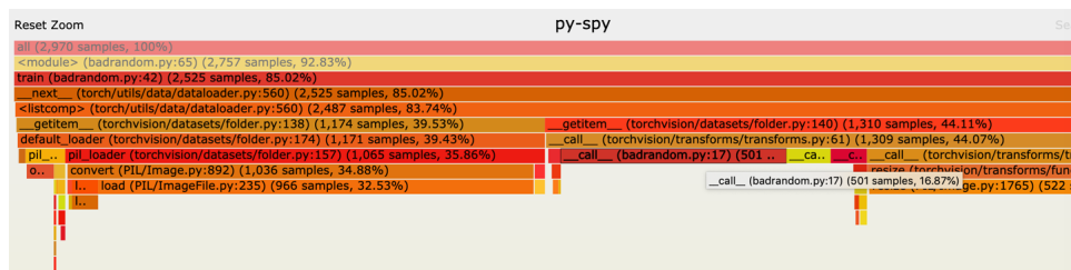
Figure 7-10. Flame graph with BadRandom
