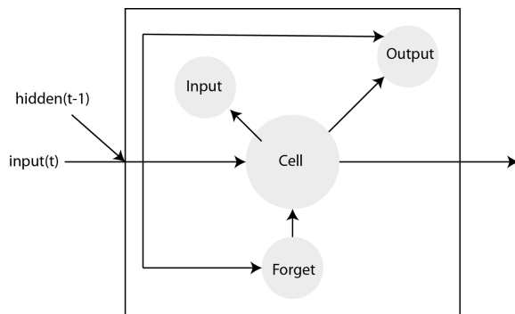
Figure 5-3. An LSTM
