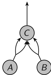
Or: C = A \vee B
