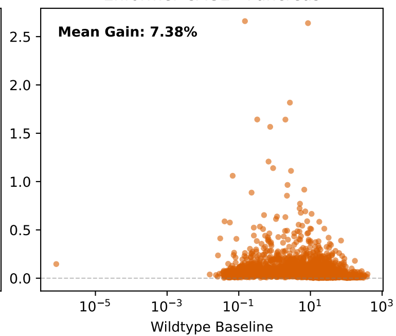
Enformer CAGE - Pancreas
