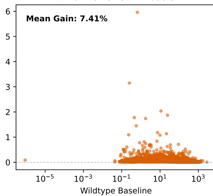
Enformer CAGE - Muscle
