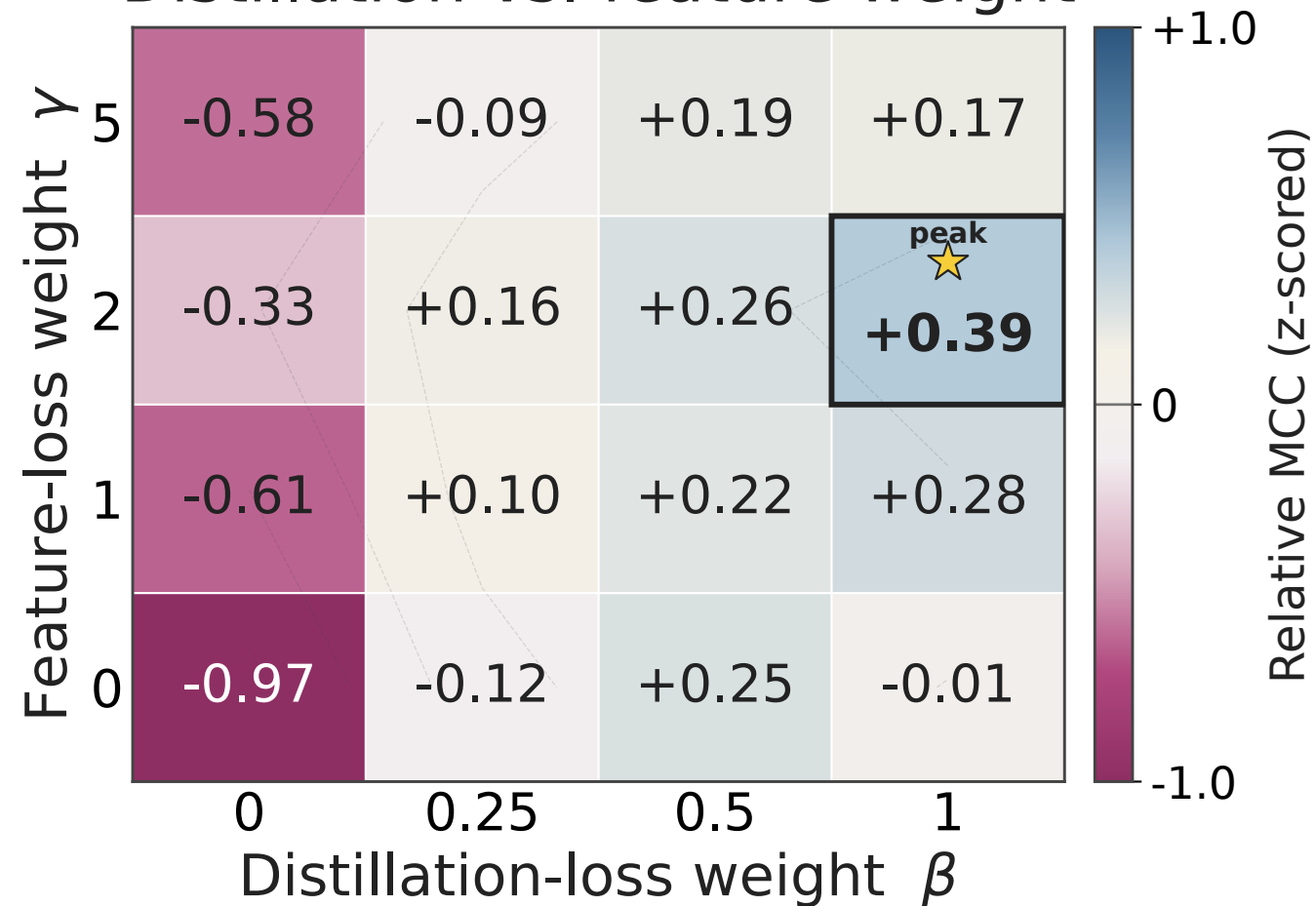
D Distillation vs. feature weight
