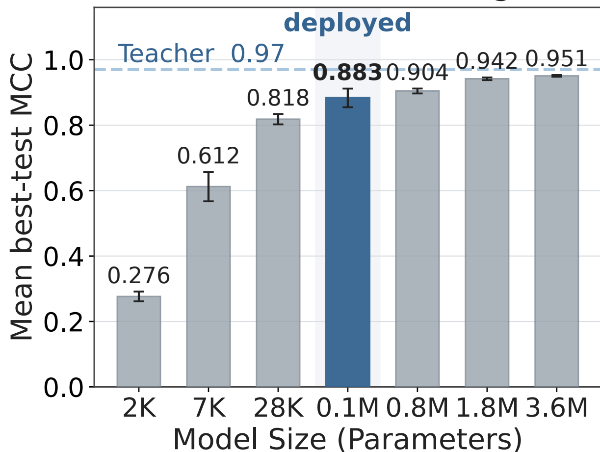
B Student-size scaling
