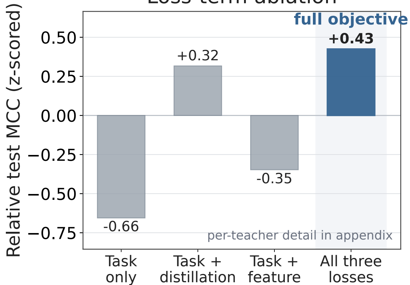
C Loss-term ablation
