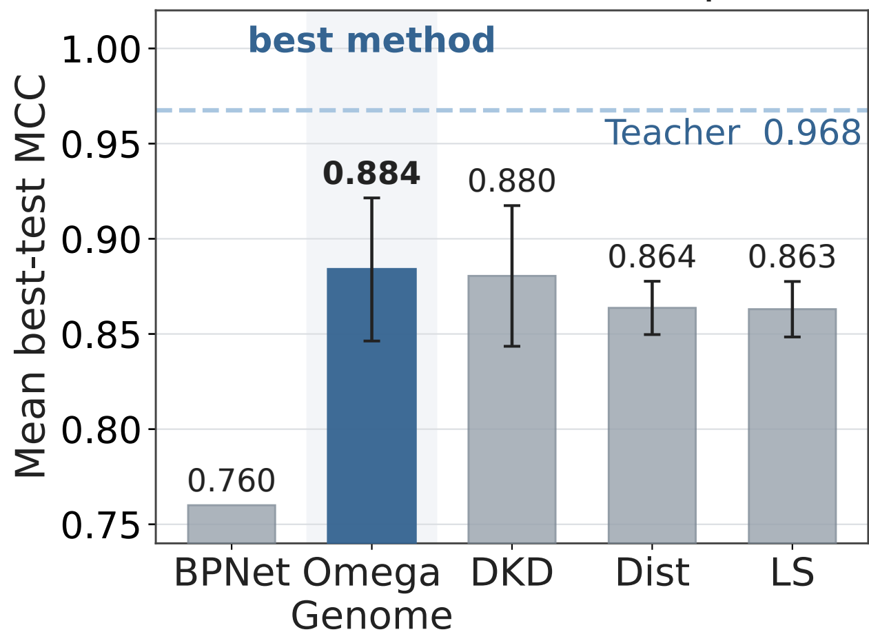
A Distillation-method comparison
