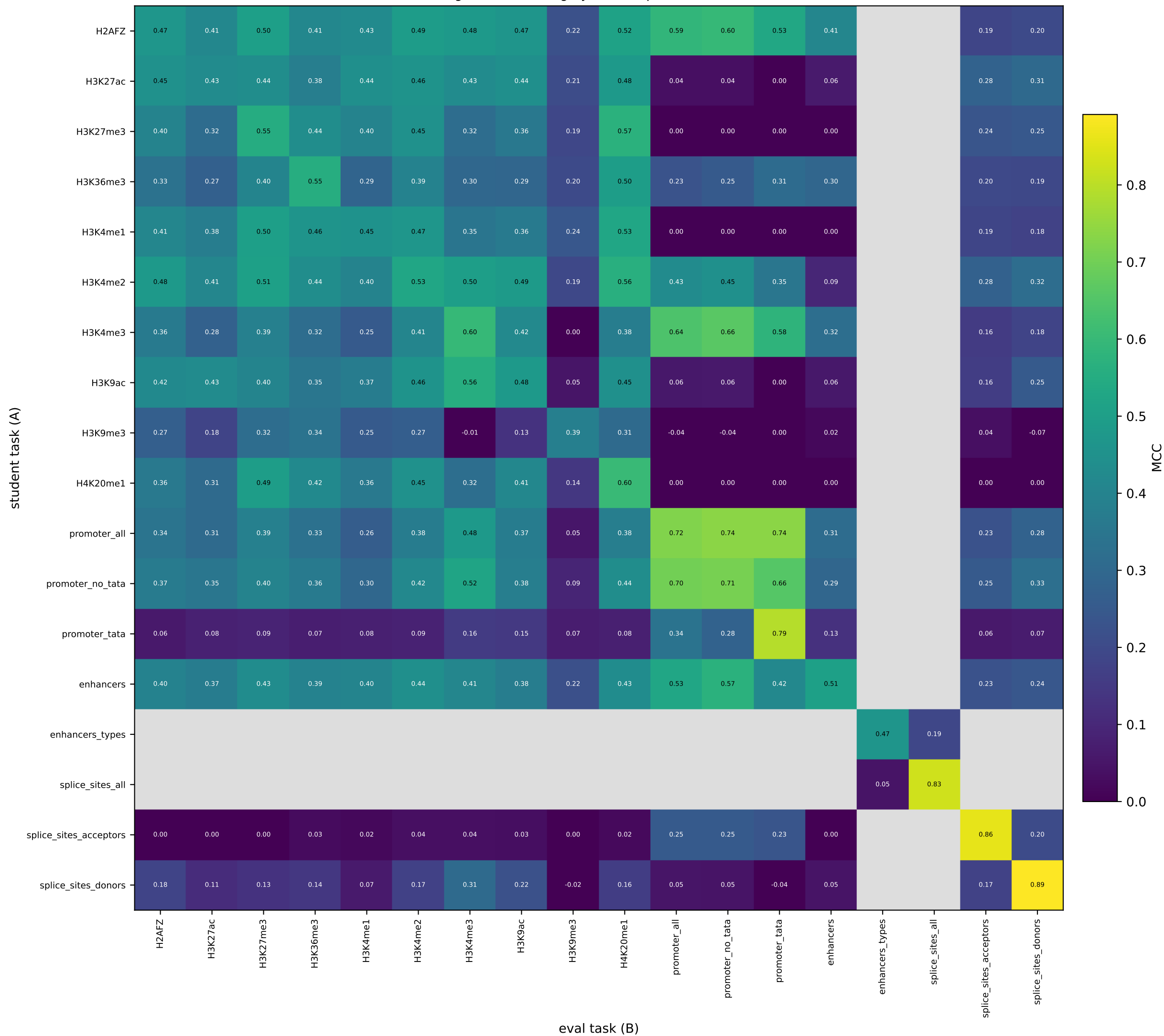
Cross-task transfer MCC -- baseline students (R2.3) diagonal = in-task; grey = incompatible head (N/A)
