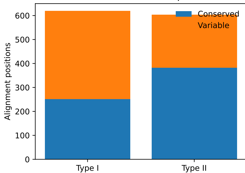
Conserved and variable positions
