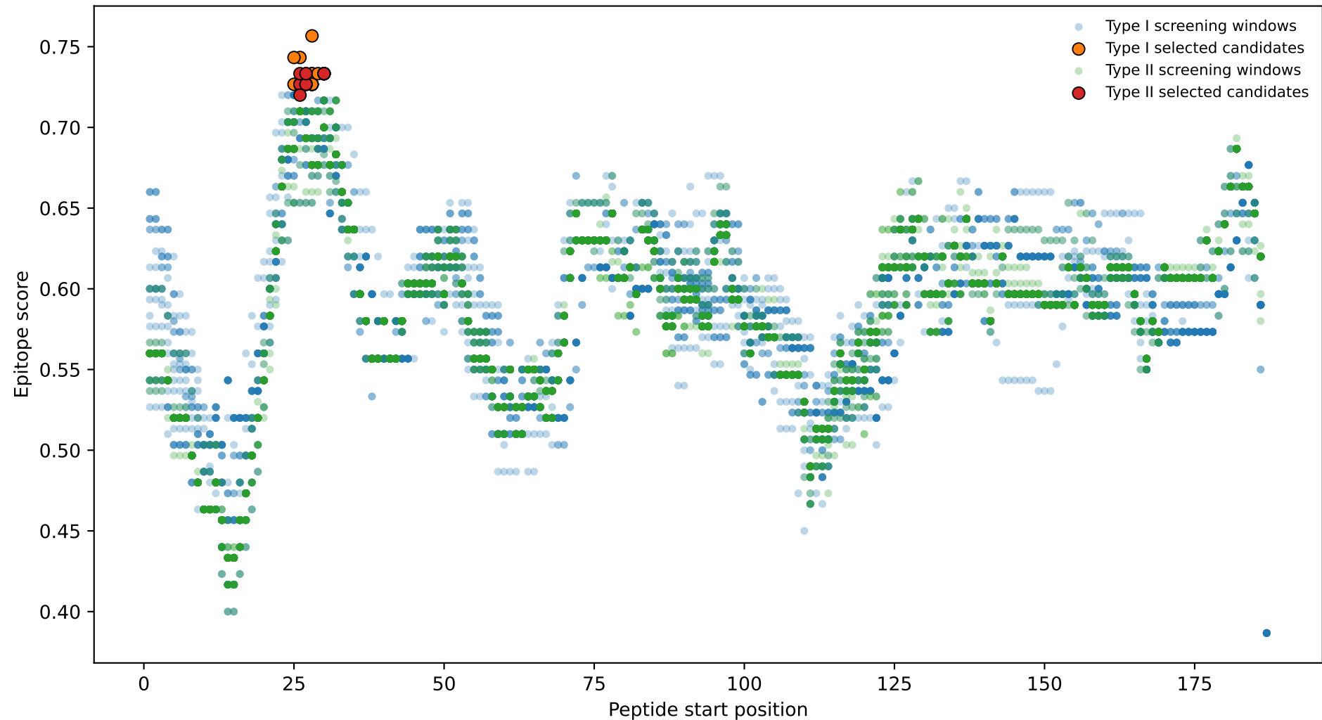
Sequence-derived peptide candidate landscape
