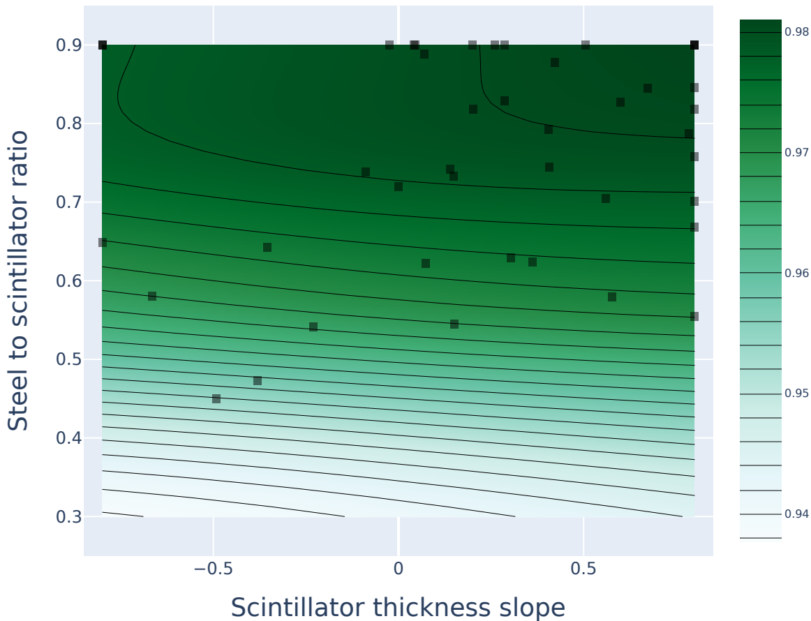
Low energy Muon/Pion separation ROC AUC
