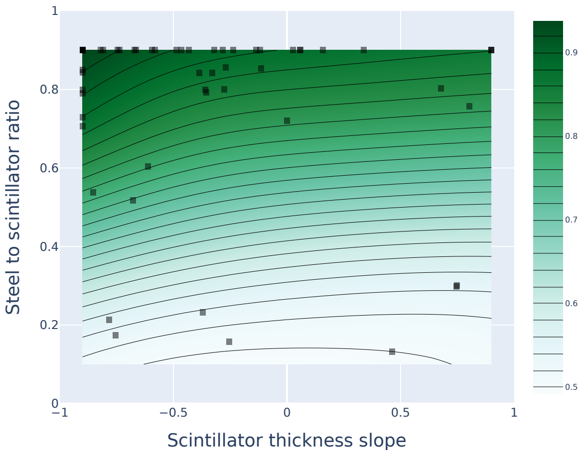
5GeV Muon/Pion separation ROC AUC
