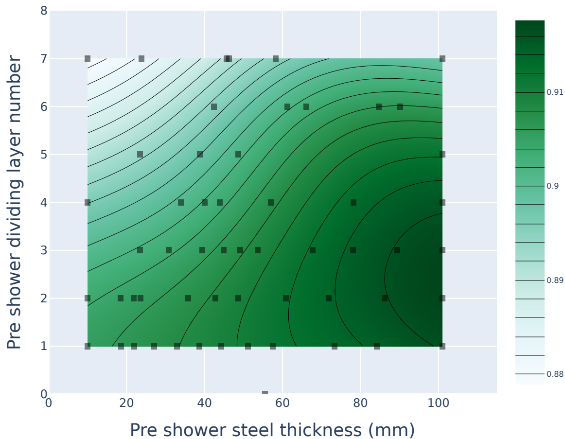
1GeV Muon/Pion separation ROC AUC
