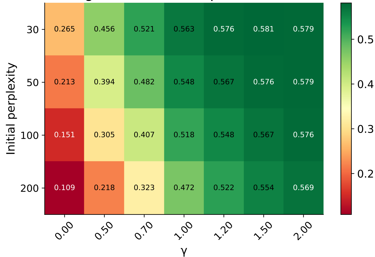
(a) Neighborhood Overlap AUC (k=1-10)
