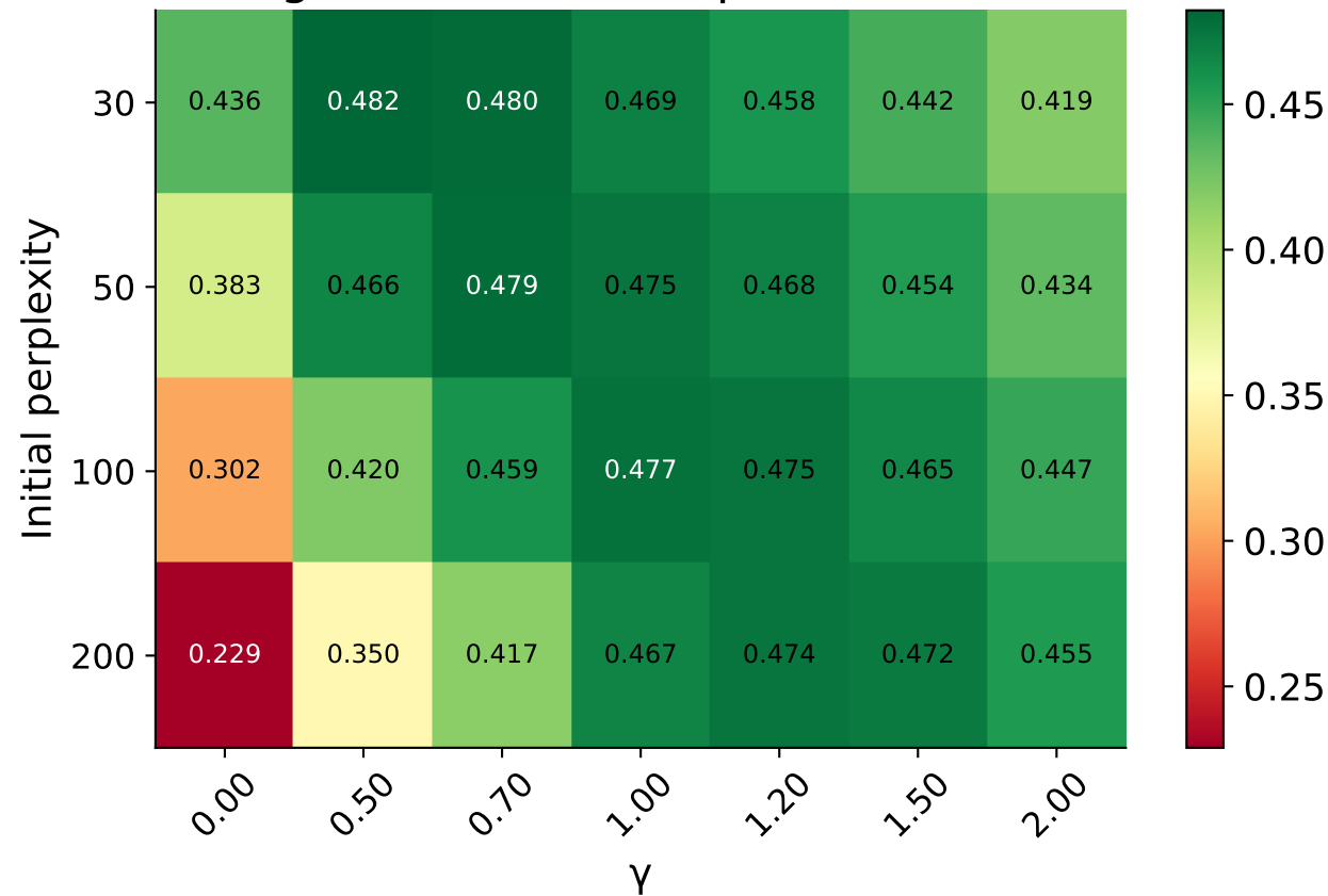
(b) Neighborhood Overlap AUC (k=11-90)
