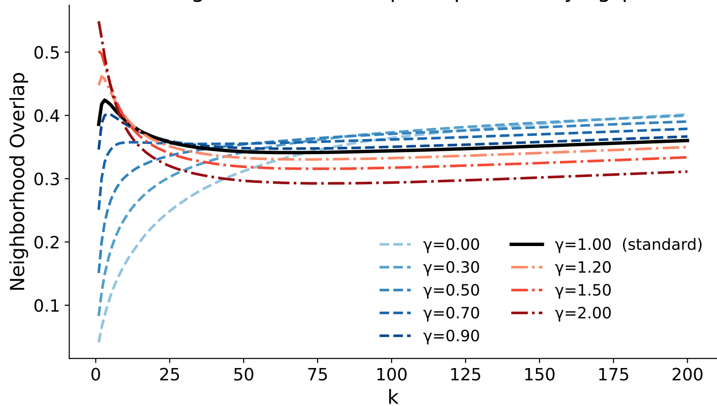
Neighborhood Overlap — \rho=30 , varying \gamma
