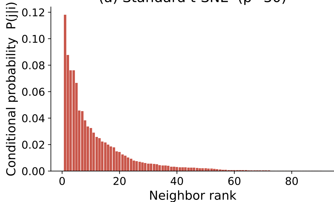
(a) Standard t-SNE ( \rho=30 )
