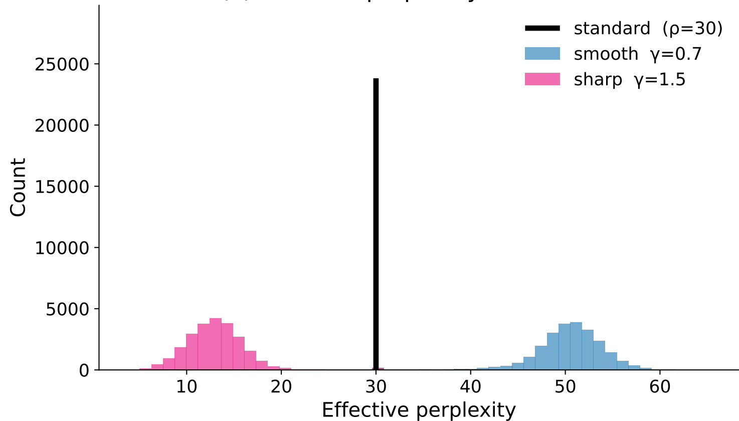
(a) Effective perplexity distribution
