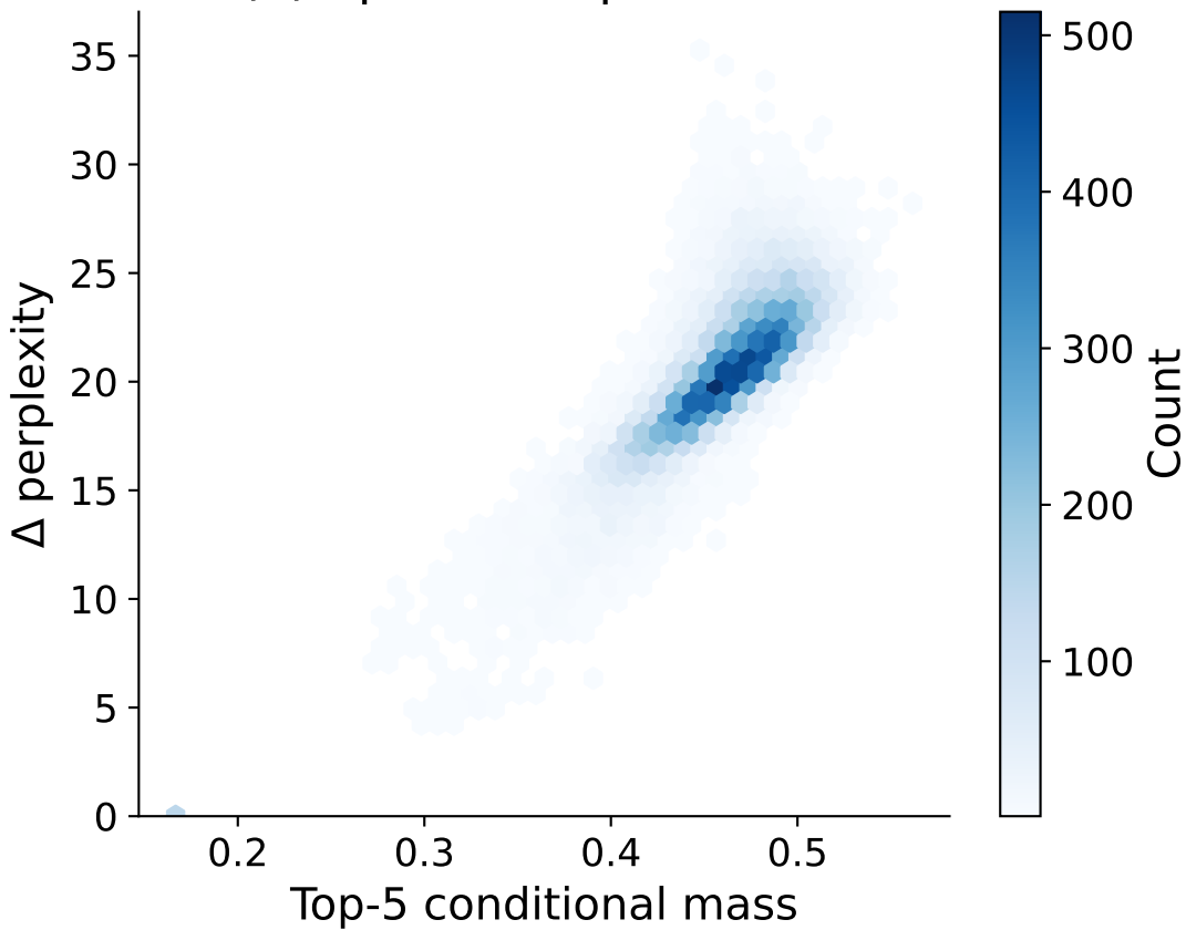
(a) Spearman \rho = 0.801
