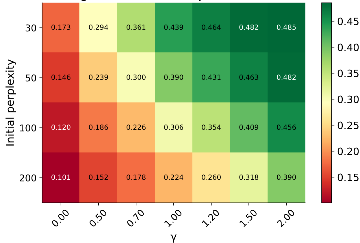
(a) Neighborhood Overlap AUC (k=1-10)
