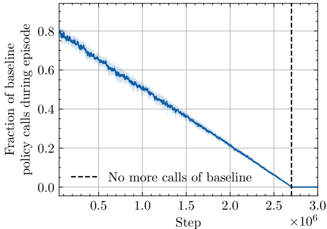
Baseline policy calls during training
