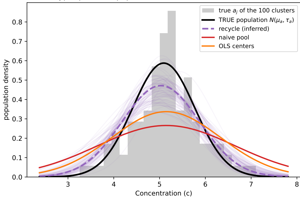
The hyper-posterior population distribution for the concentration
