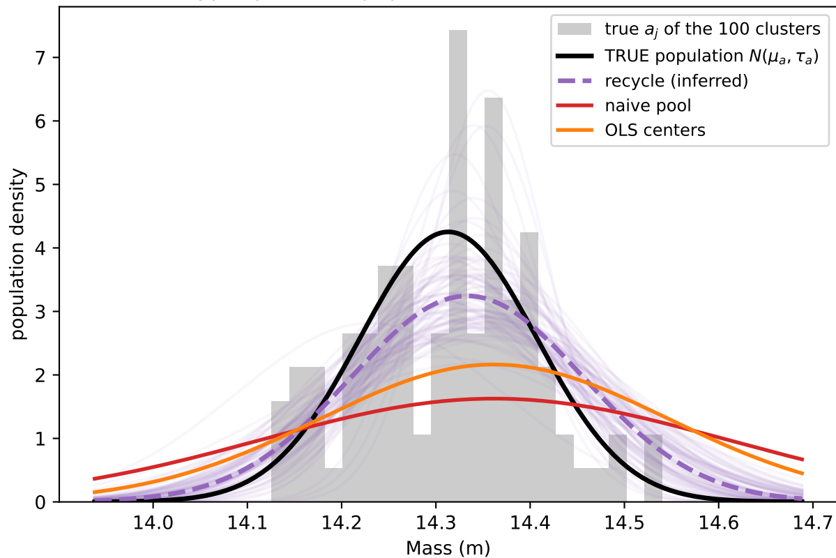
The hyper-posterior population distribution for the mass
