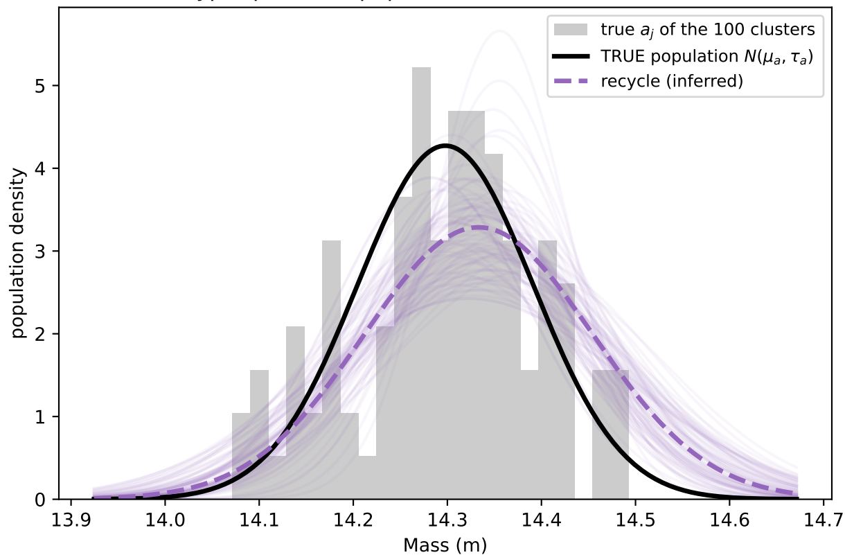
The hyper-posterior population distribution for the mass
