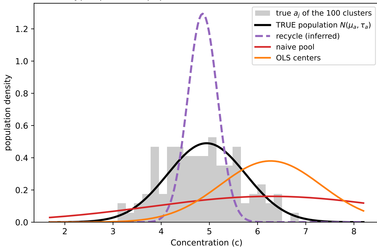
The hyper-posterior population distribution for the concentration
