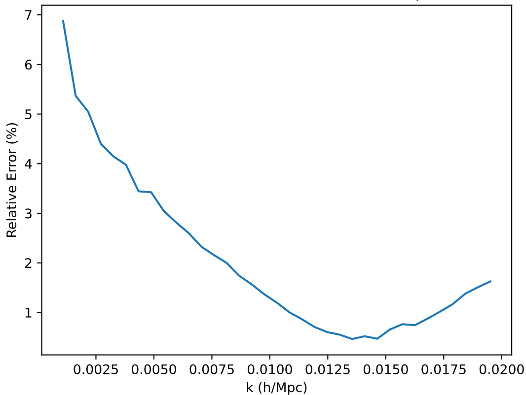
Relative Error as a Function of k for \text{dtau}_0 , A_p and n_s
