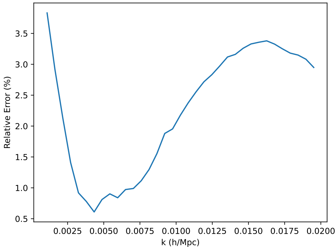
Relative Error as a Function of k for ns, hub, and hireionz
