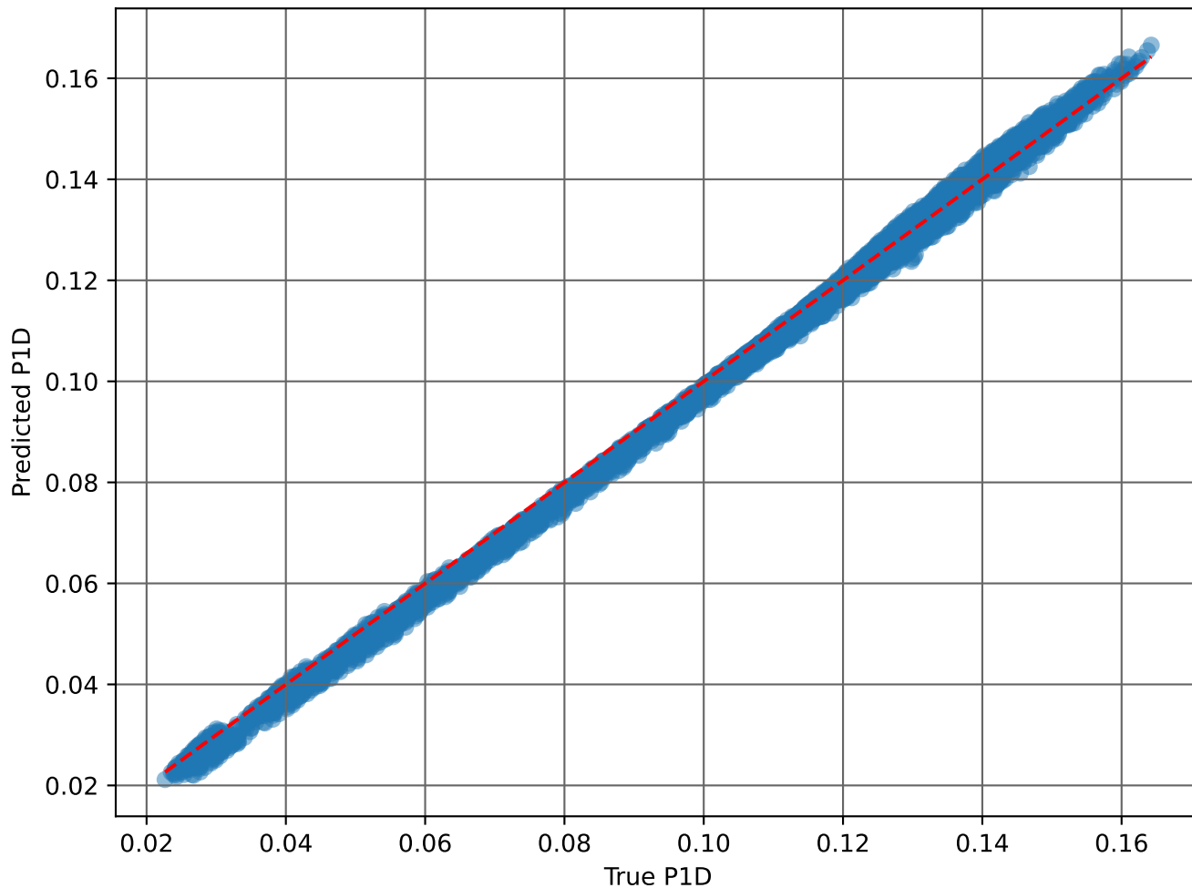
True vs Predicted P1D for dtau0, Ap and ns (denormalized)
