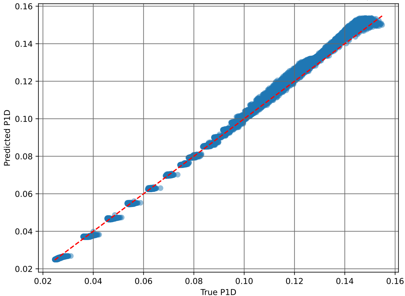
True vs Predicted P1D for ns, hub, and hireionz (denormalized)
