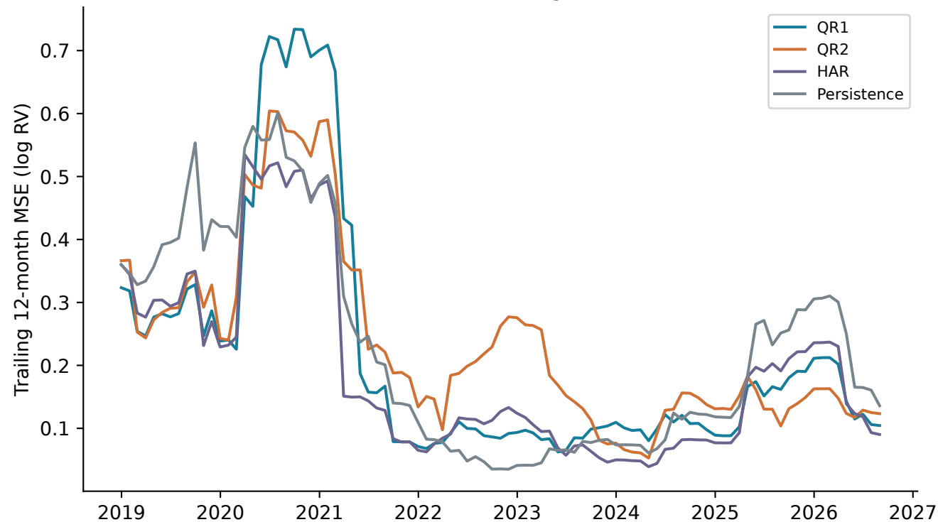
120-month training window
