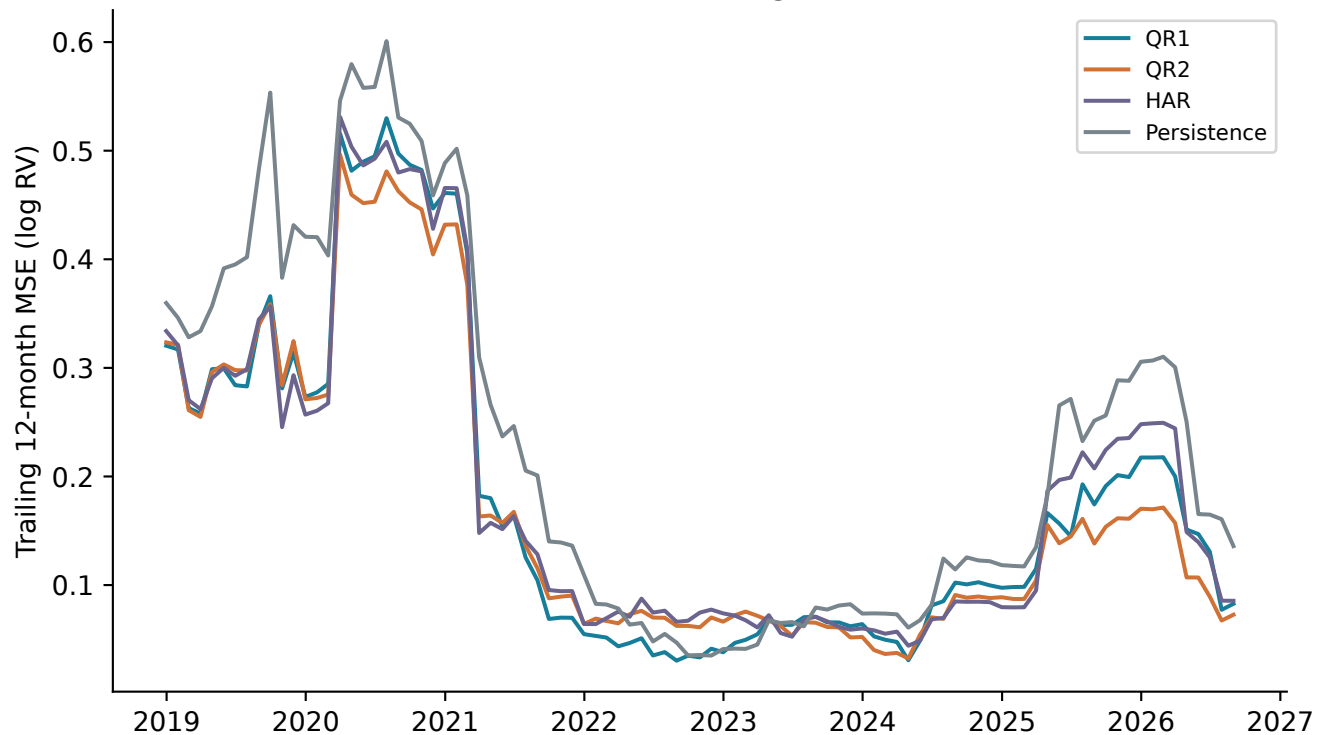
571-month training window
