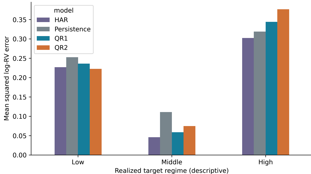
120-month window
