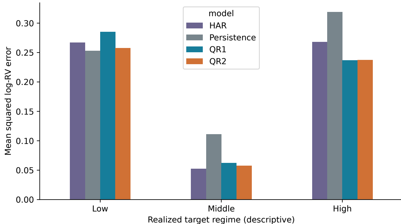
571-month window
