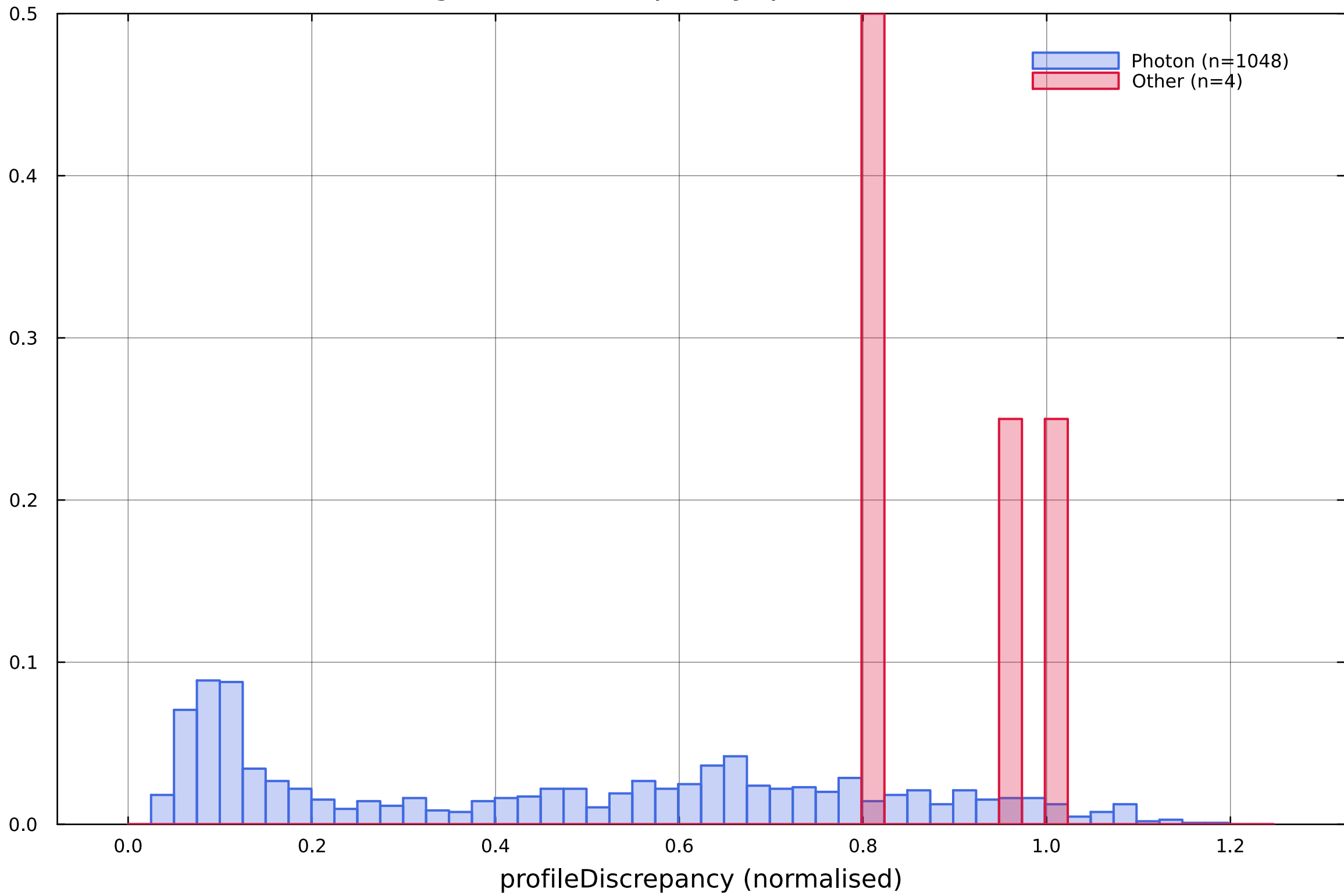
LongProfileDiscrepancy: photon vs other
