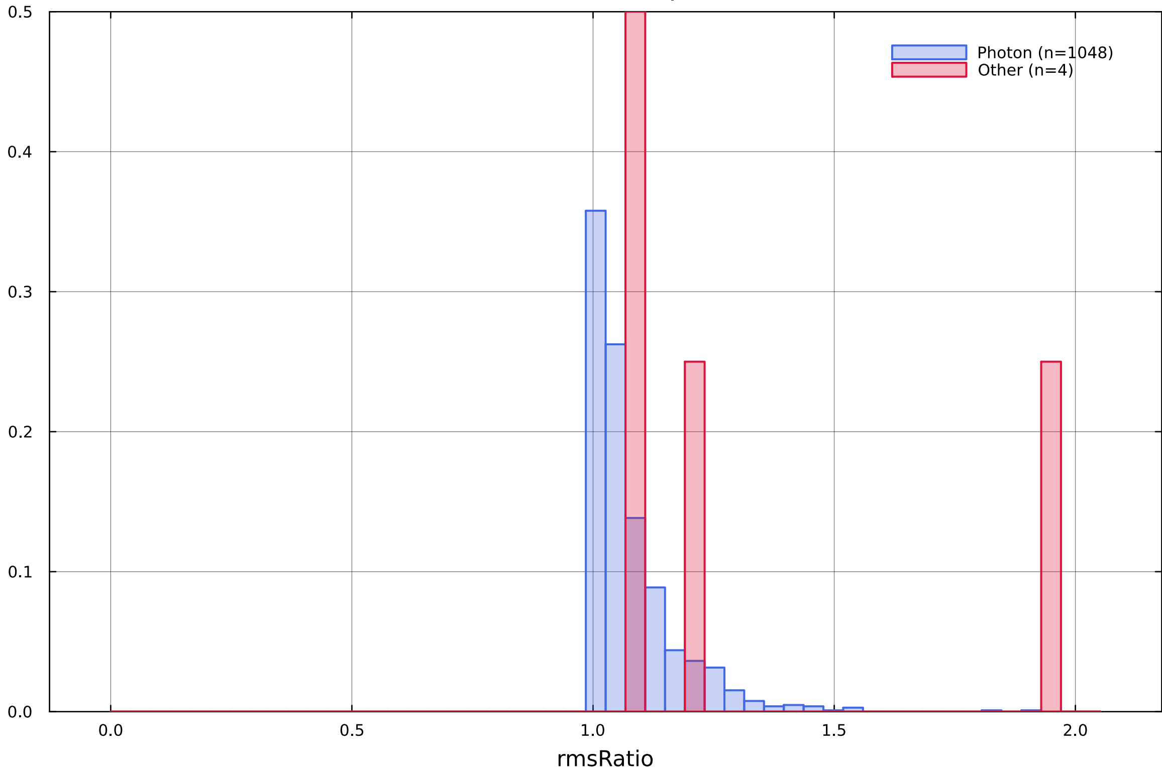
RmsRatio (RmsXYRatio): photon vs other
