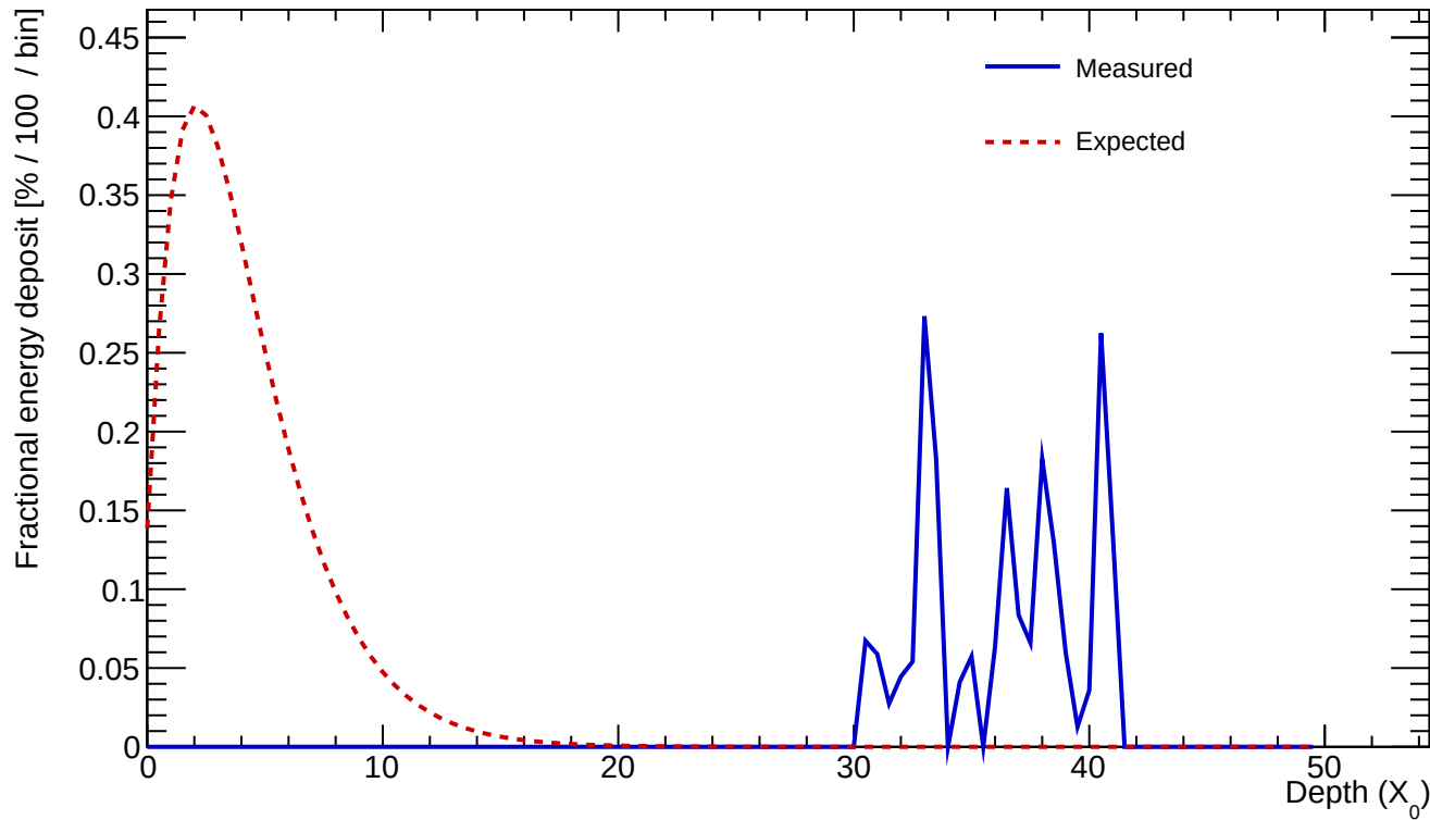
Cluster 314 E=0.641 GeV profileStart=40.00 X_0 \chi=0.8426
