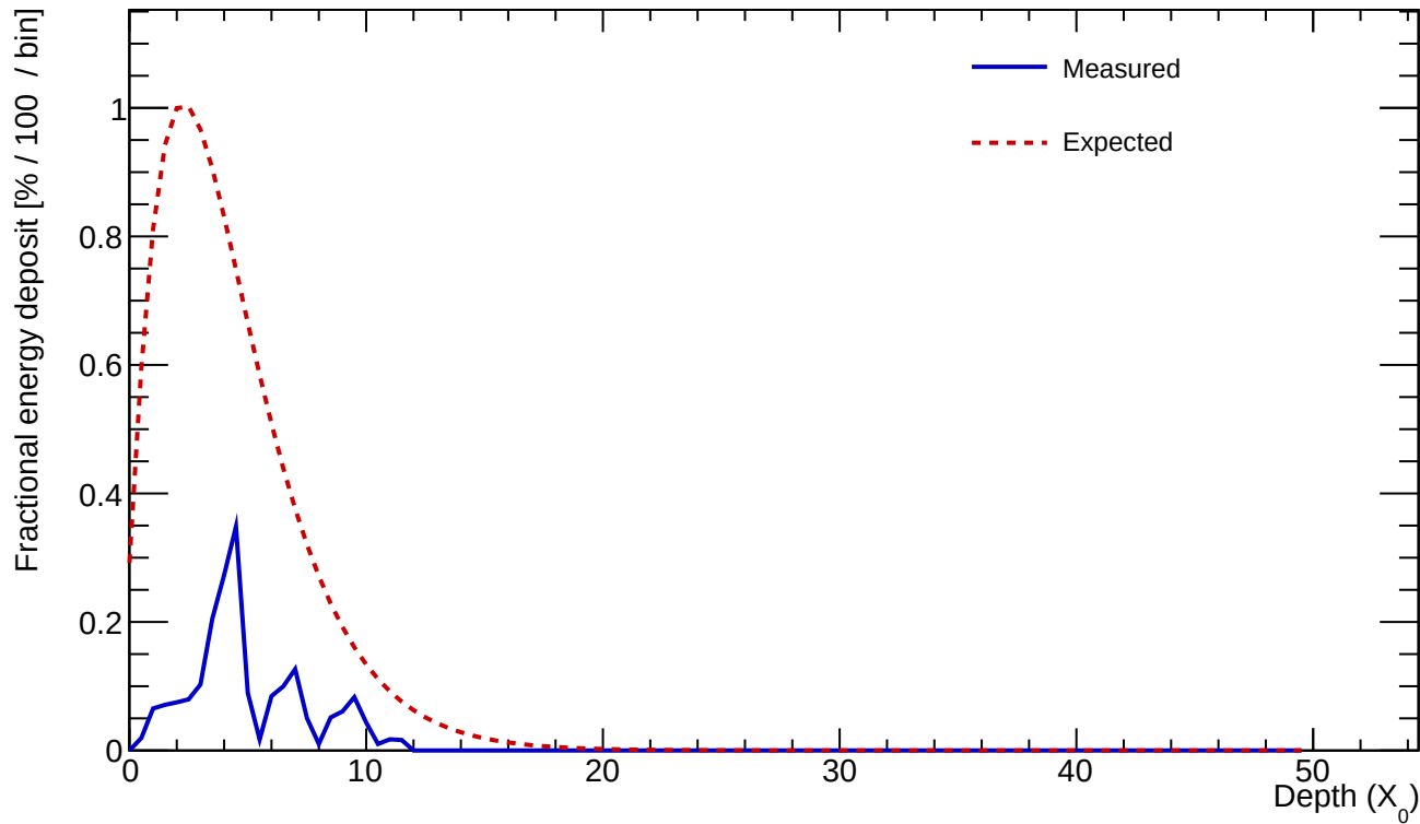
Cluster 52 E=0.776 GeV profileStart=1.00 X_0 \chi=0.4978
