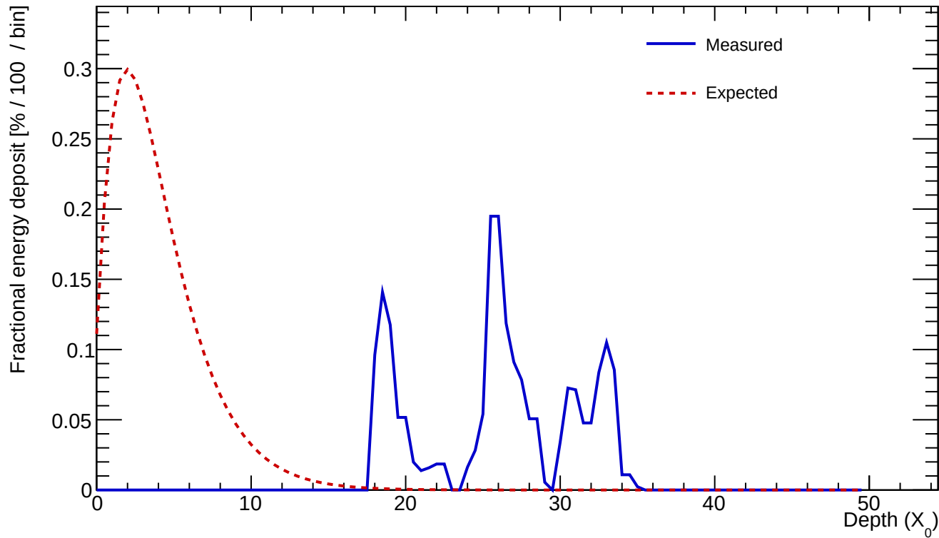
Cluster 191 E=0.576 GeV profileStart=24.50 X_0 \chi=0.7870
