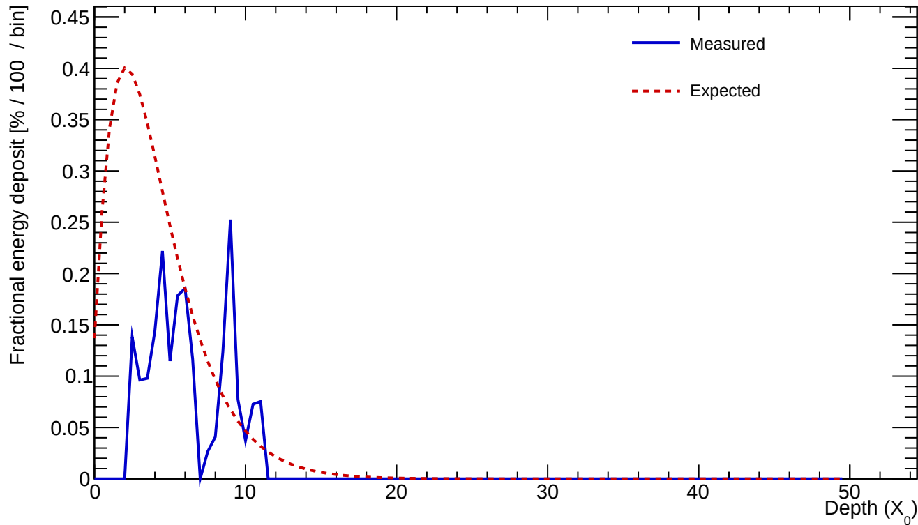
Cluster 338 E=0.637 GeV profileStart=2.50 X_0 \chi=0.4358
