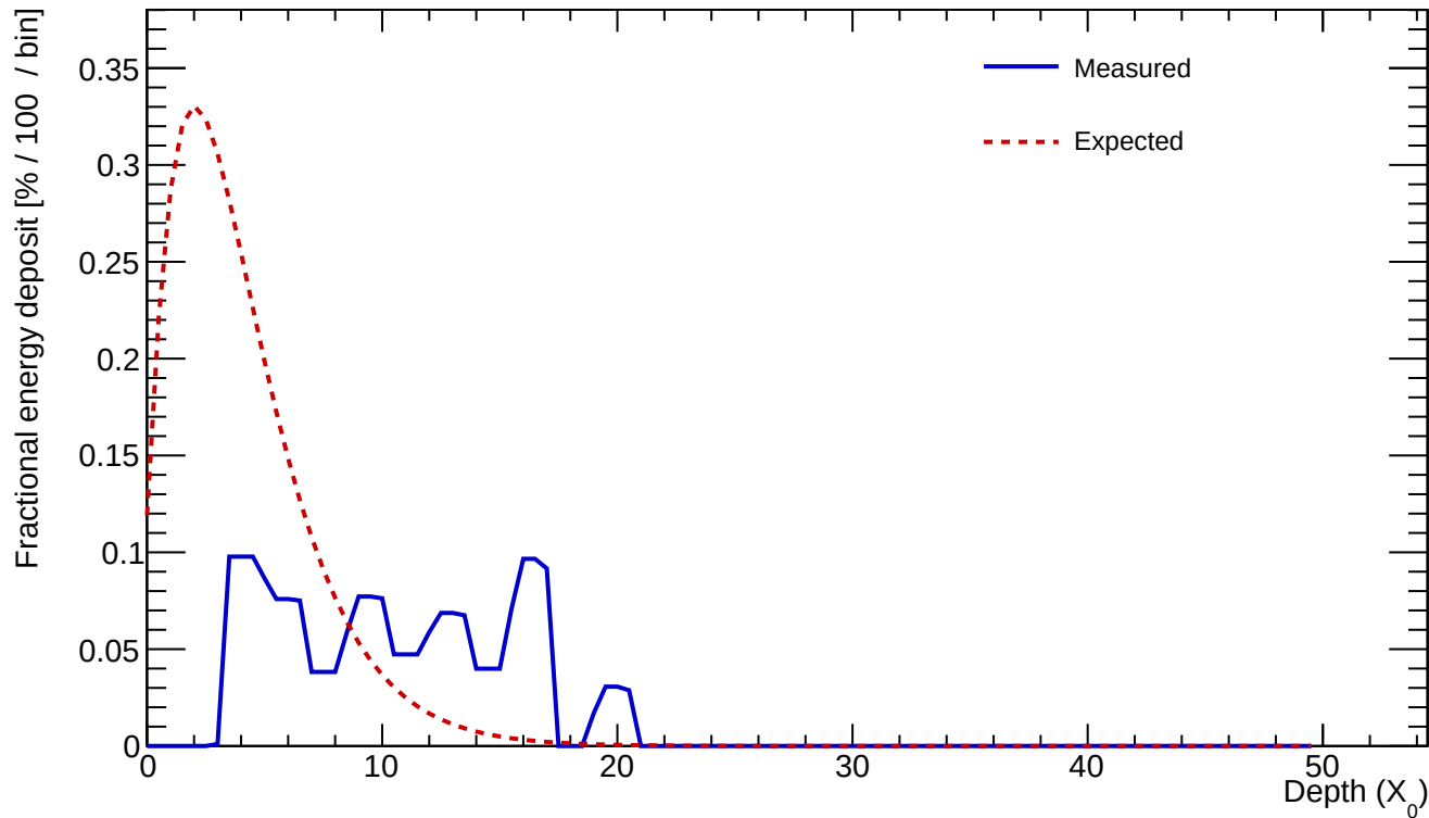
Cluster 336 E=0.598 GeV profileStart=3.50 X_0 \chi=0.7217
