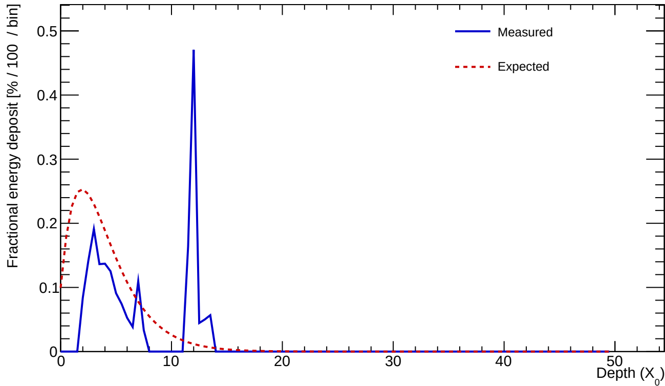
Cluster 308 E=0.537 GeV profileStart=1.50 X_0 \chi=0.7300
