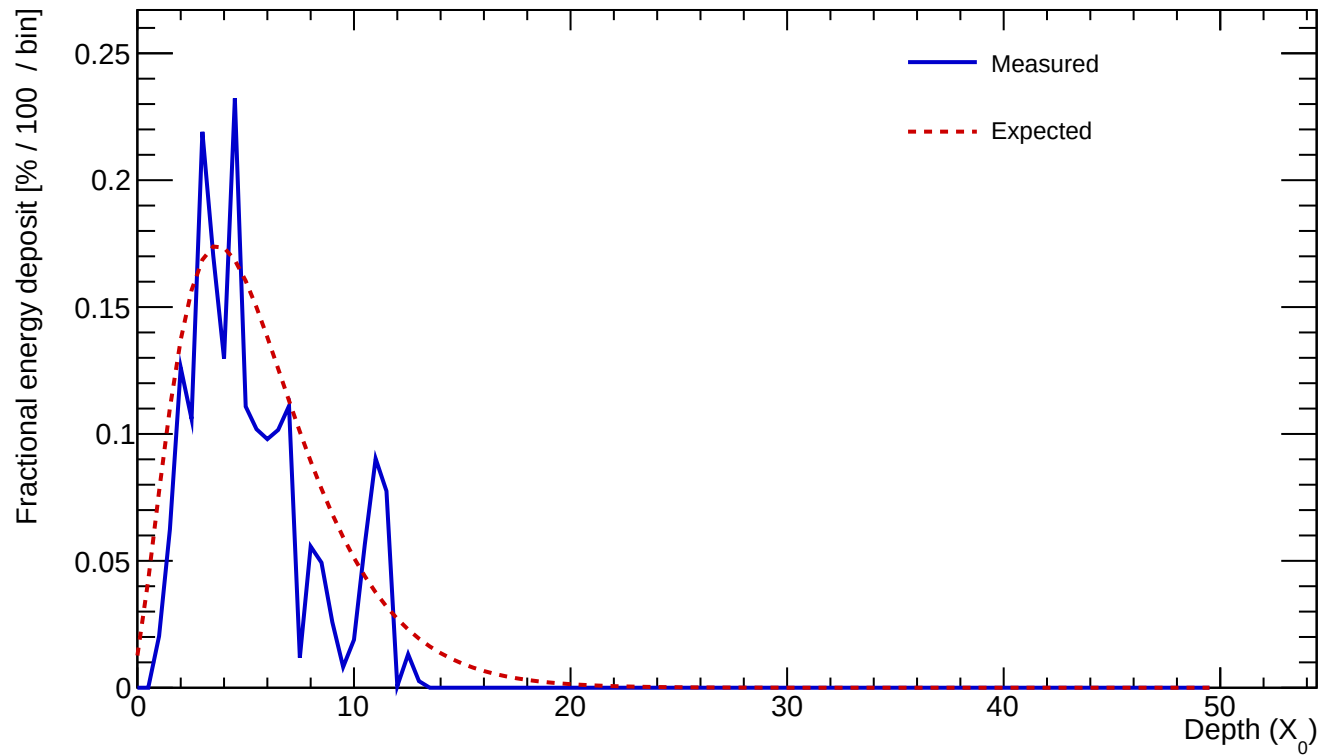
Cluster 321 E=3.238 GeV profileStart=0.50 X_0 \chi=0.3790
