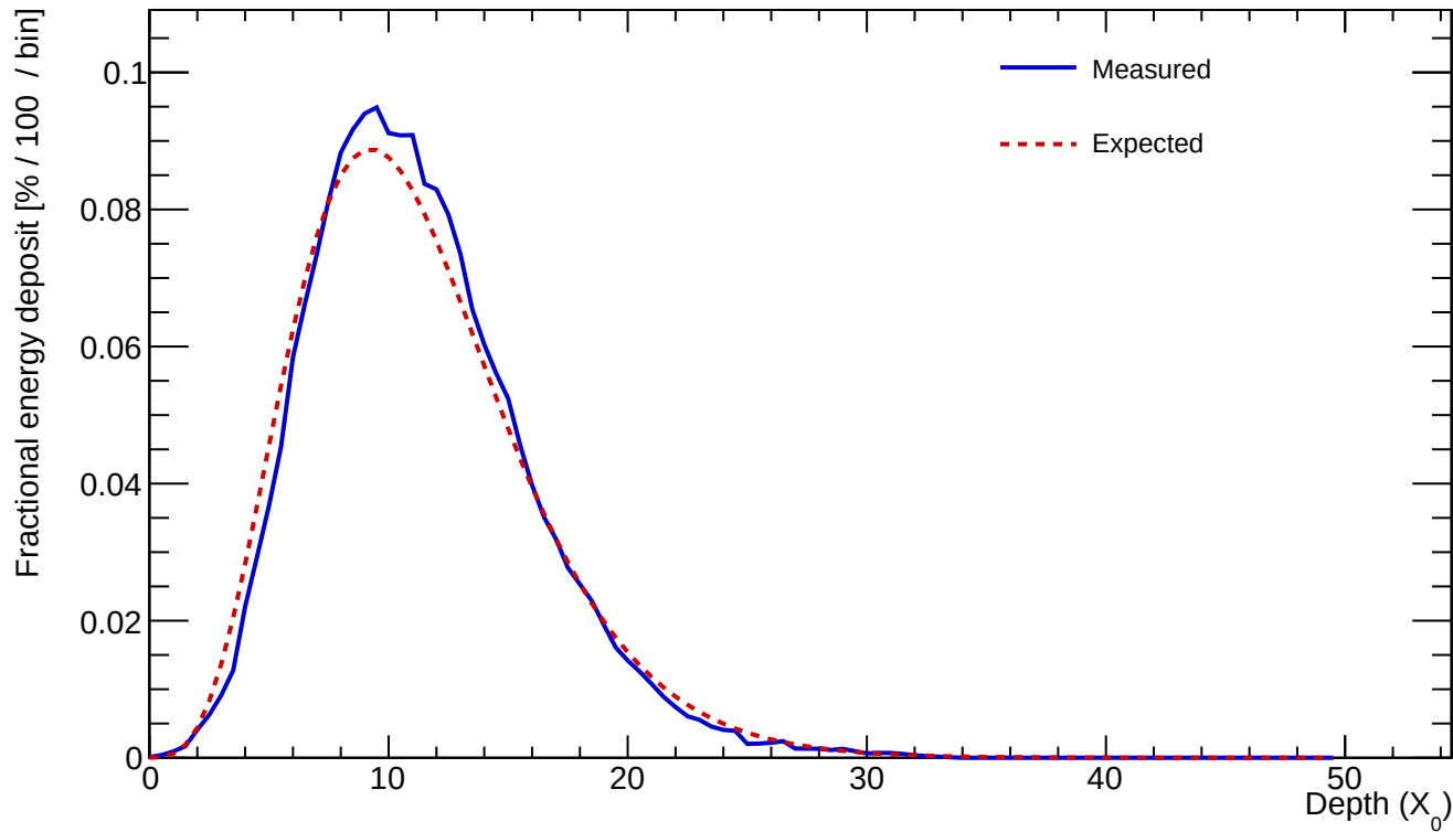
Cluster 21 E=833.134 GeV profileStart=0.50 X_0 \chi=0.0712
