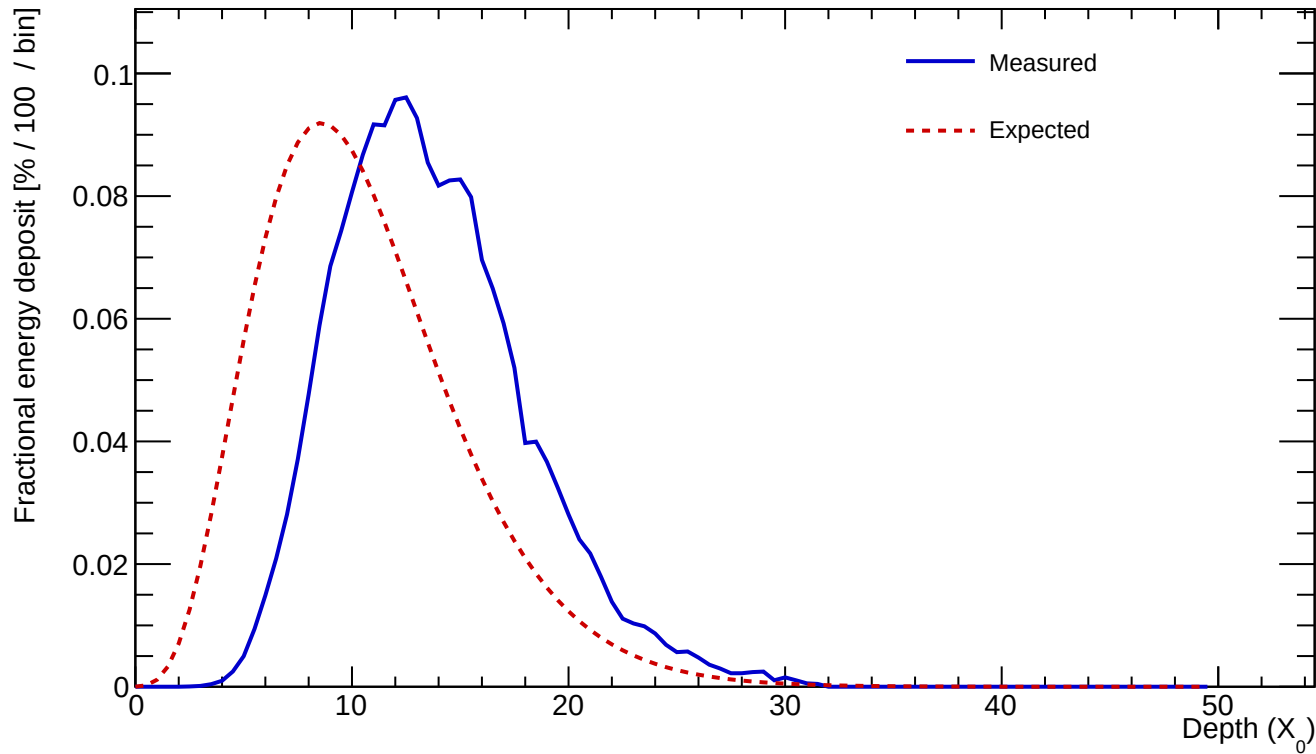
Cluster 26 E=427.585 GeV profileStart=3.50 X_0 \chi=0.0614
