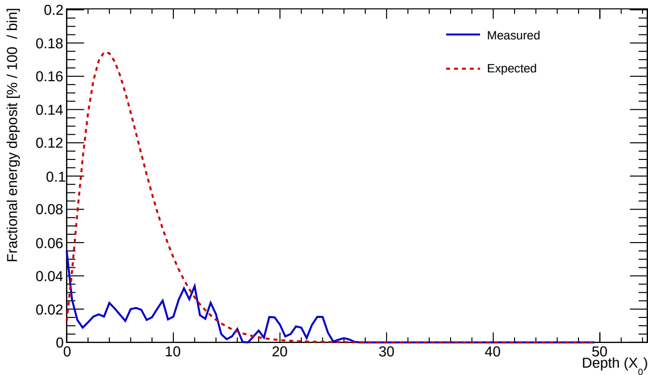
Cluster 383 E=3.219 GeV profileStart=3.00 X_0 \chi=0.8422
