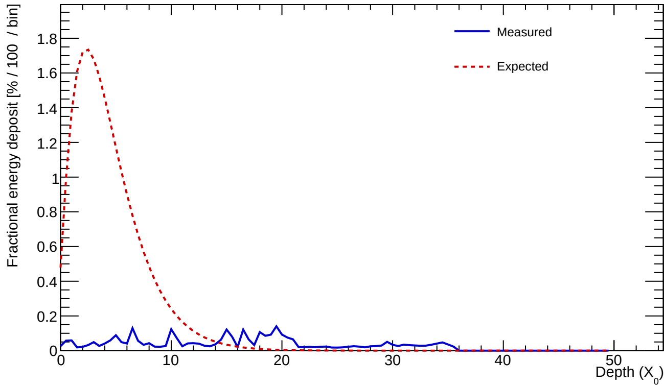
Cluster 107 E=0.823 GeV profileStart=13.50 X_0 \chi=1.1625
