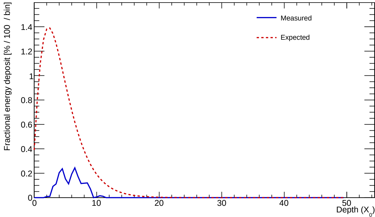
Cluster 355 E=0.807 GeV profileStart=2.50 X_0 \chi=0.3314
