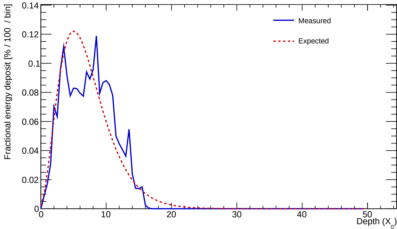
Cluster 29 E=12.246 GeV profileStart=0.50 X_0 \chi=0.2511
