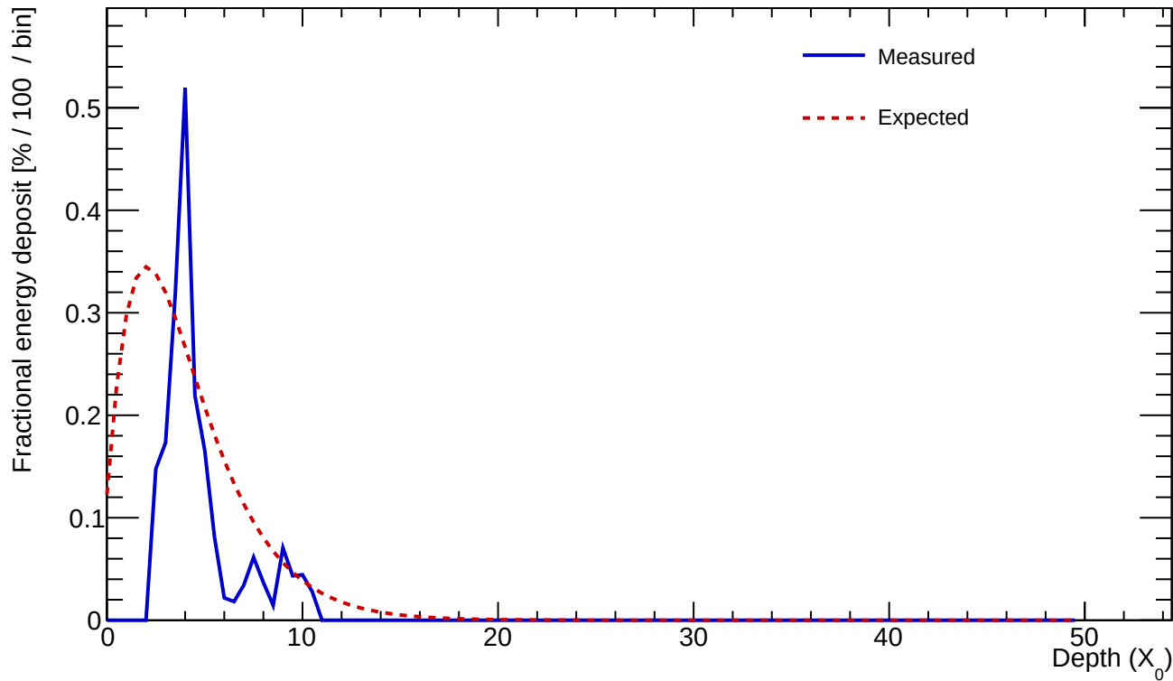
Cluster 337 E=0.607 GeV profileStart=2.00 X_0 \chi=0.5869
