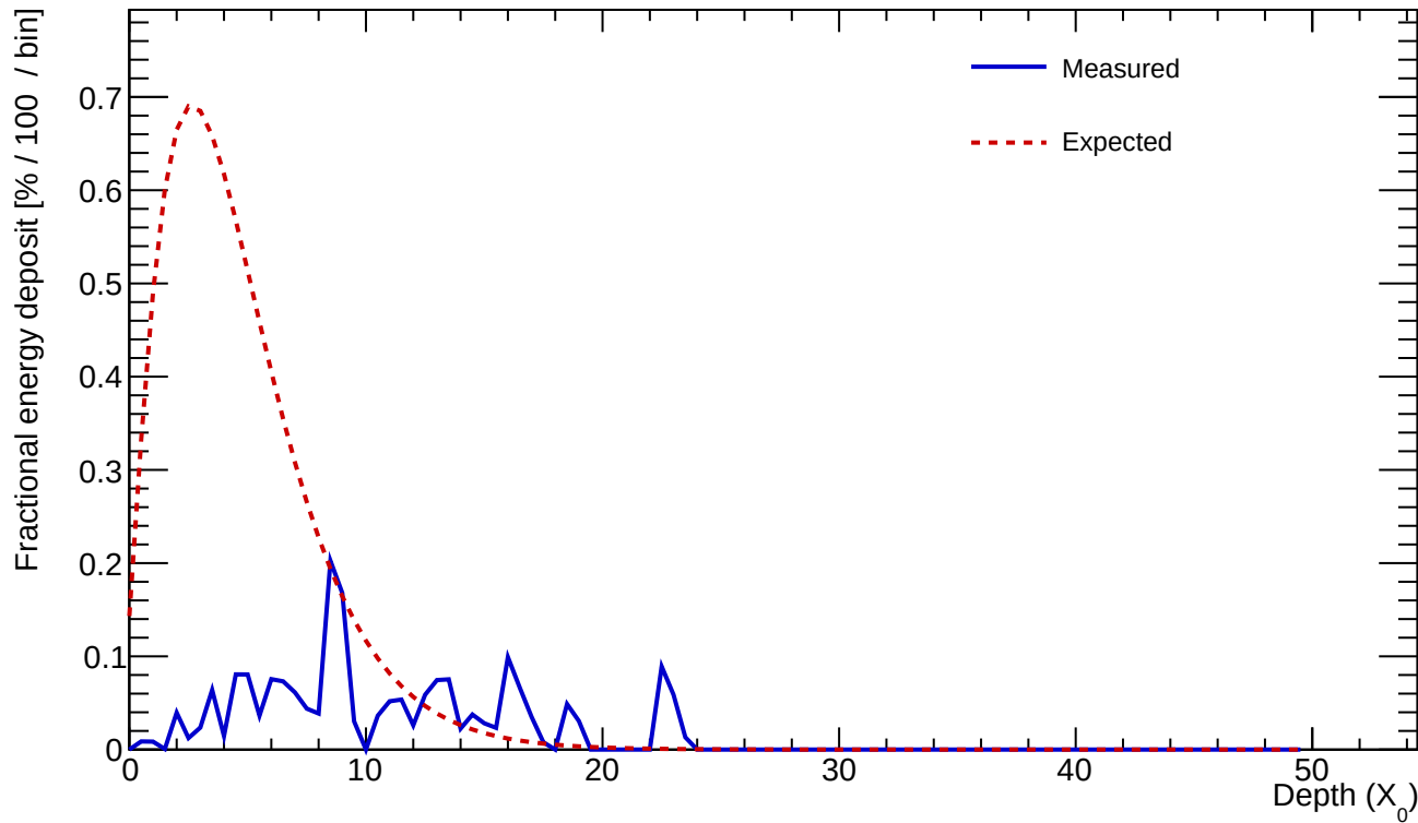
Cluster 232 E=1.133 GeV profileStart=5.50 X_0 \chi=0.8213
