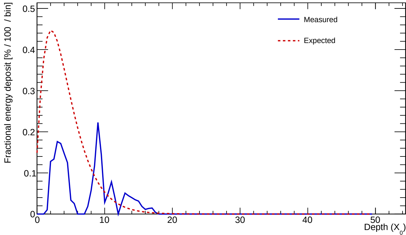
Cluster 193 E=0.659 GeV profileStart=1.50 X_0 \chi=0.7058
