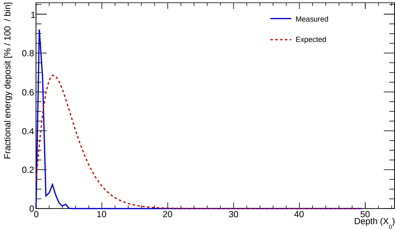
Cluster 384 E=1.134 GeV profileStart=4.50 X_0 \chi=0.9929
