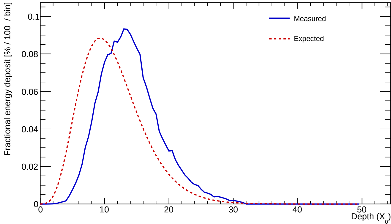
Cluster 59 E=899.600 GeV profileStart=3.00 X_0 \chi=0.0617
