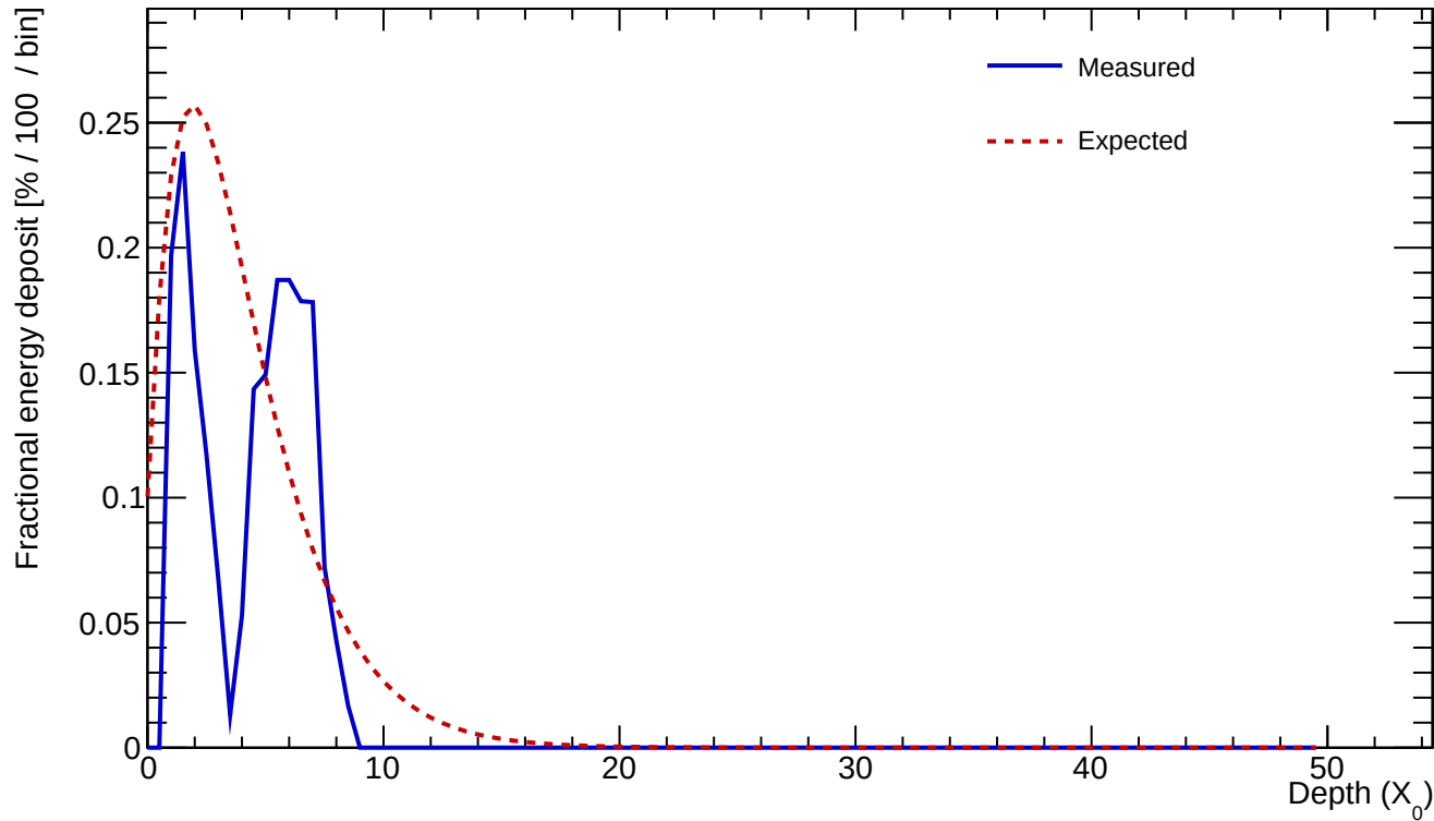
Cluster 386 E=0.540 GeV profileStart=4.00 X_0 \chi=0.5302
