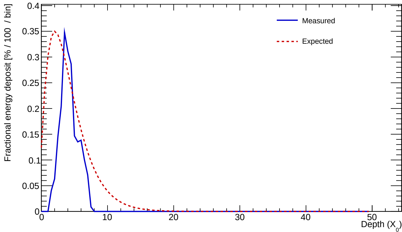
Cluster 219 E=0.610 GeV profileStart=1.50 X_0 \chi=0.3122
