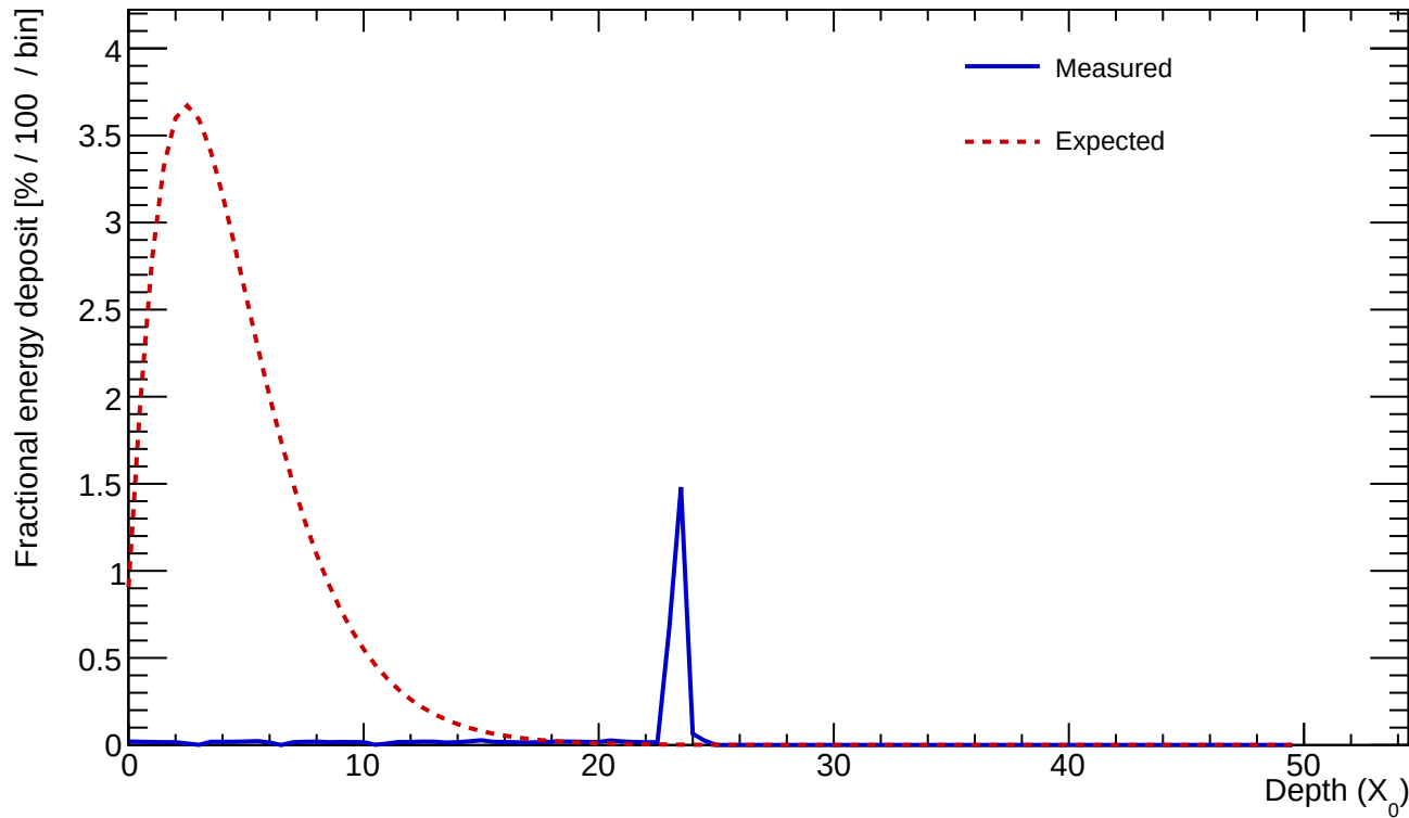
Cluster 27 E=0.934 GeV profileStart=22.50 X_0 \chi=0.9270
