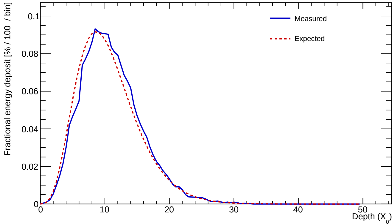
Cluster 65 E=454.072 GeV profileStart=0.50 X_0 \chi=0.0469
