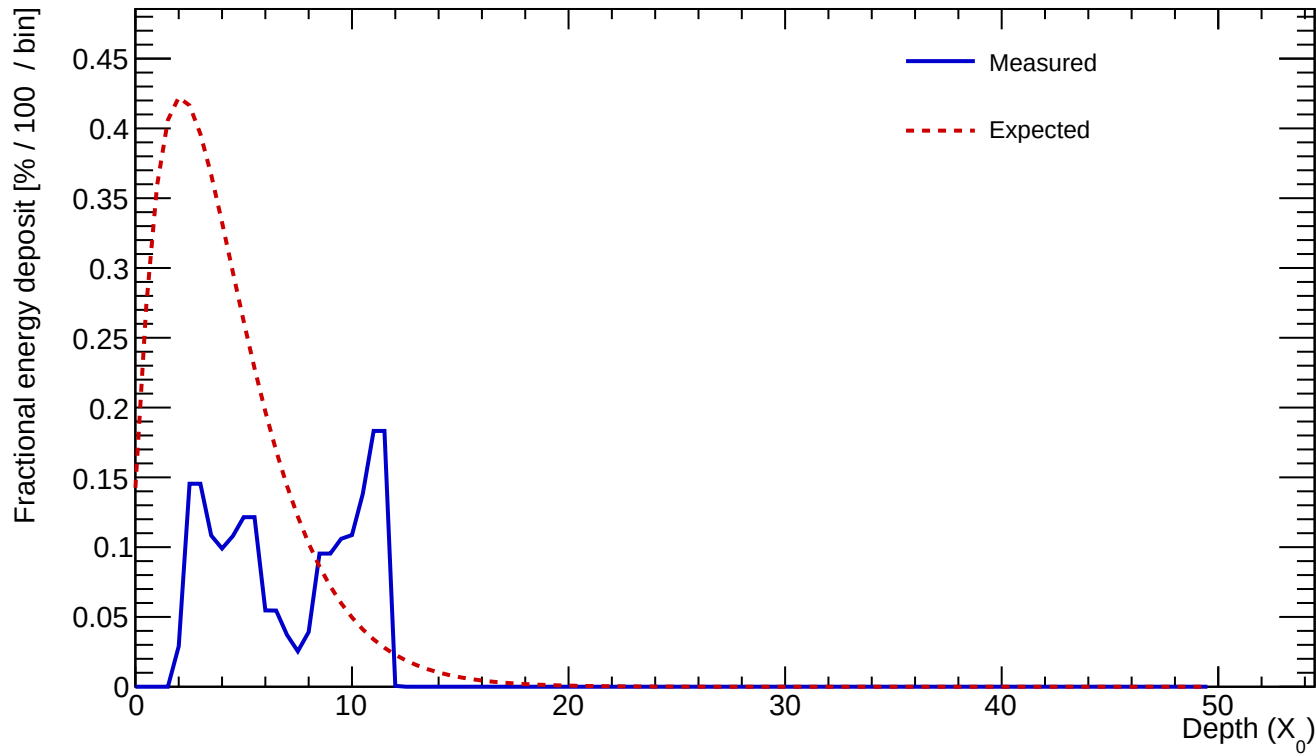
Cluster 90 E=0.648 GeV profileStart=2.00 X_0 \chi=0.6062
