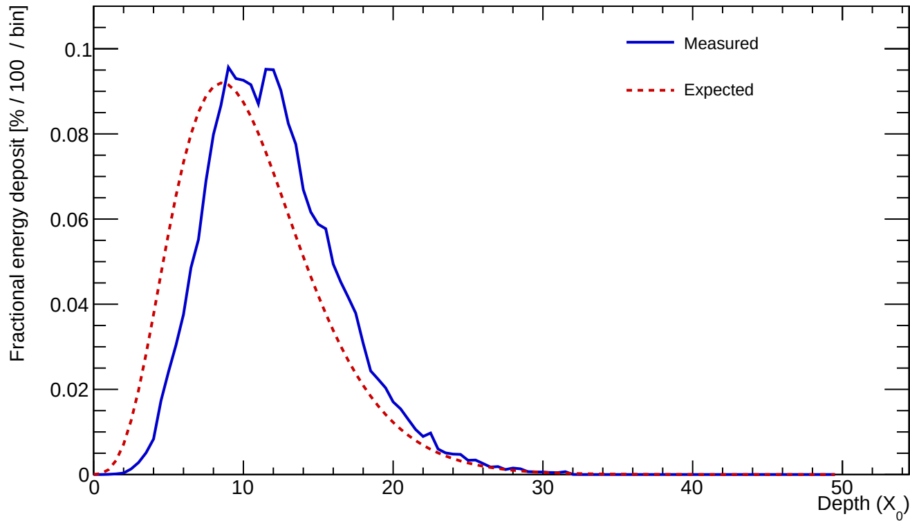
Cluster 34 E=423.436 GeV profileStart=2.00 X_0 \chi=0.0755
