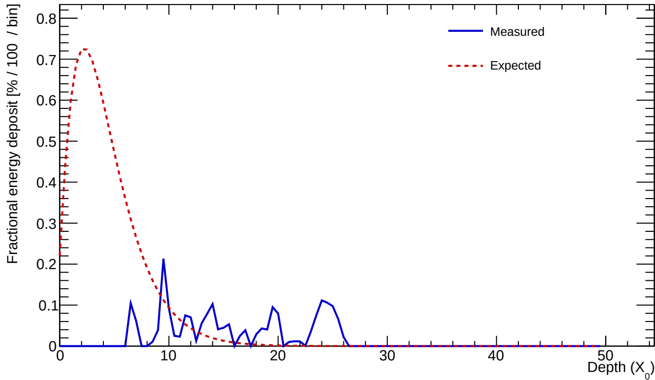
Cluster 366 E=0.737 GeV profileStart=8.50 X_0 \chi=0.9587
