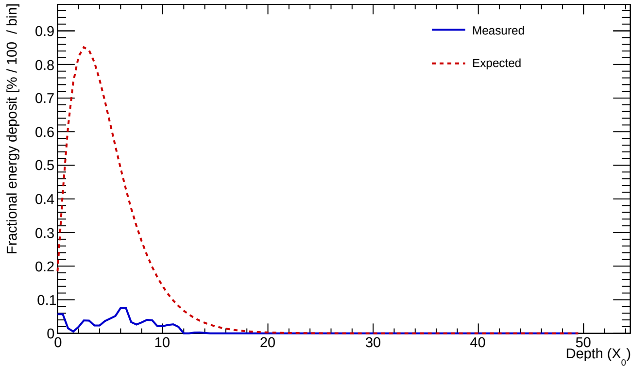
Cluster 71 E=1.081 GeV profileStart=2.00 X_0 \chi=0.5132
