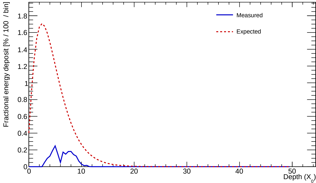
Cluster 187 E=0.981 GeV profileStart=3.00 X_0 \chi=0.3395
