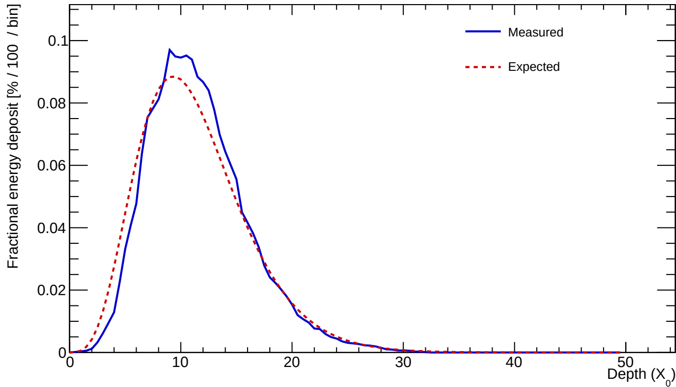
Cluster 47 E=888.224 GeV profileStart=0.50 X_0 \chi=0.0894
