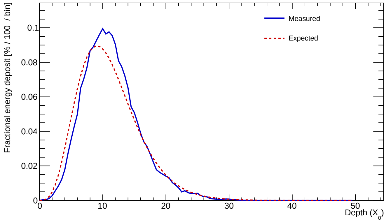
Cluster 375 E=714.284 GeV profileStart=0.50 X_0 \chi=0.0978
