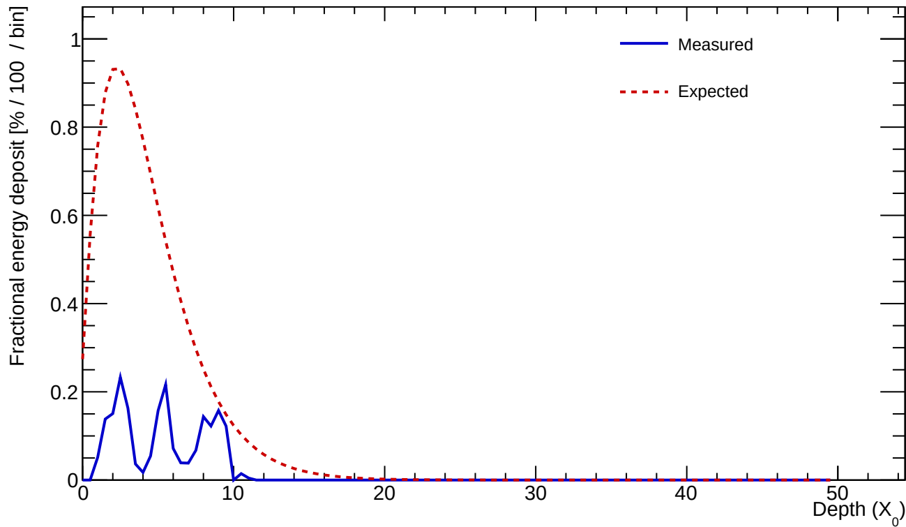
Cluster 3 E=0.768 GeV profileStart=1.00 X_0 \chi=0.5788
