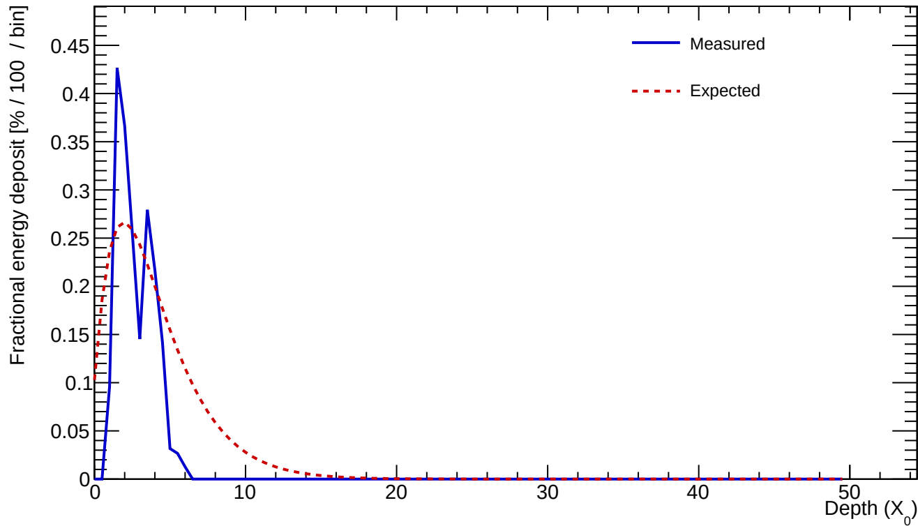
Cluster 267 E=0.549 GeV profileStart=1.00 X_0 \chi=0.5147
