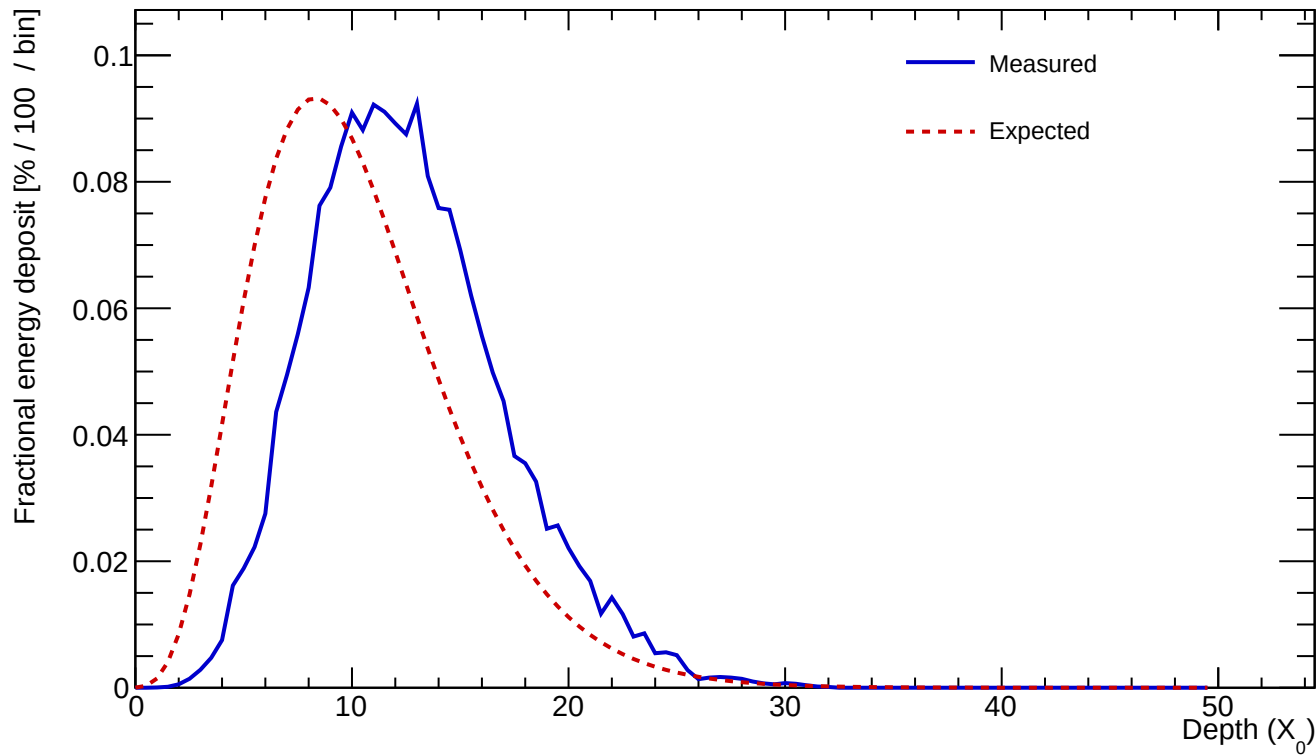
Cluster 145 E=327.017 GeV profileStart=2.50 X_0 \chi=0.0622
