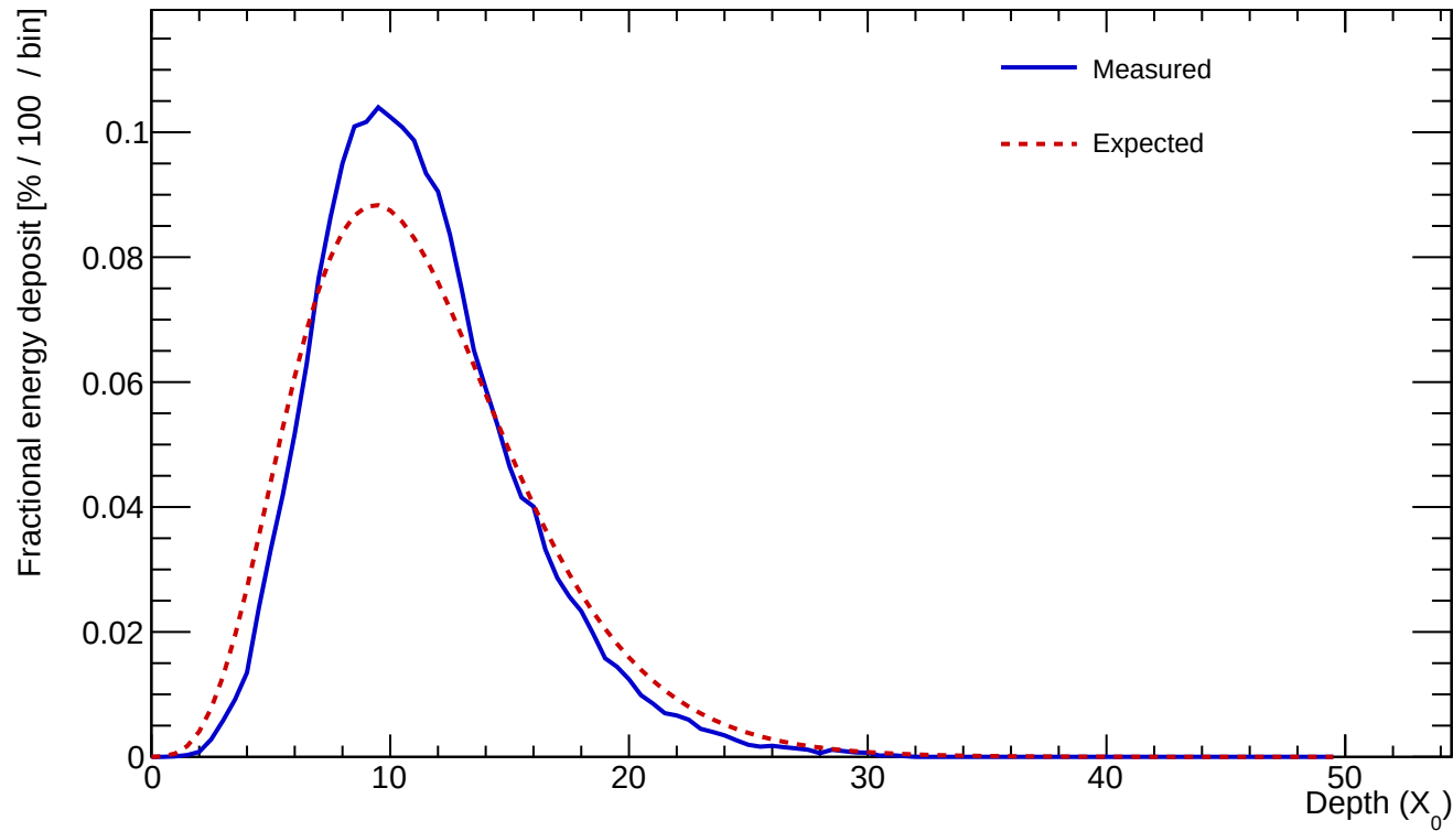
Cluster 214 E=922.184 GeV profileStart=0.50 X_0 \chi=0.1555
