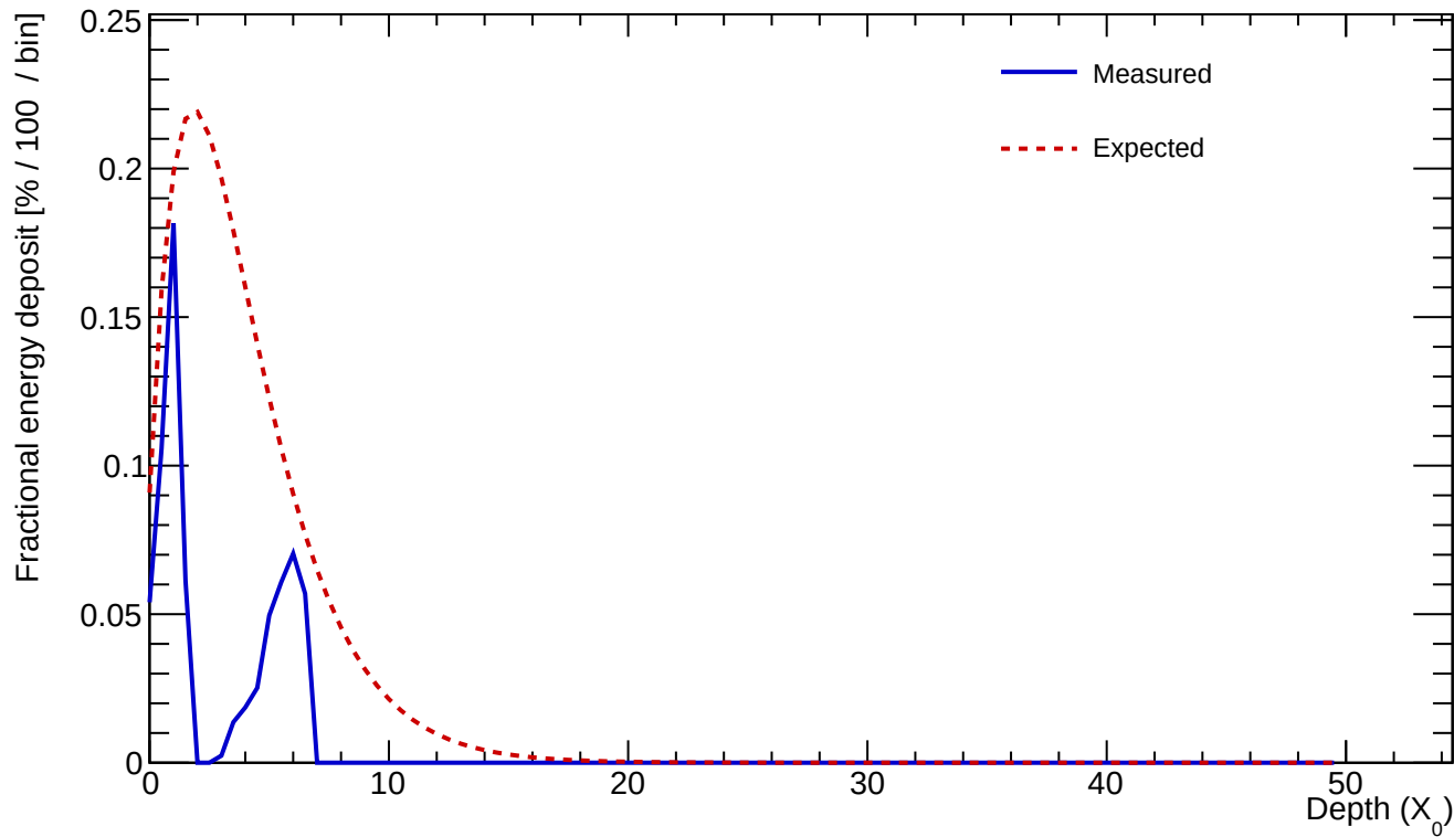
Cluster 349 E=0.501 GeV profileStart=4.00 X_0 \chi=0.6570
