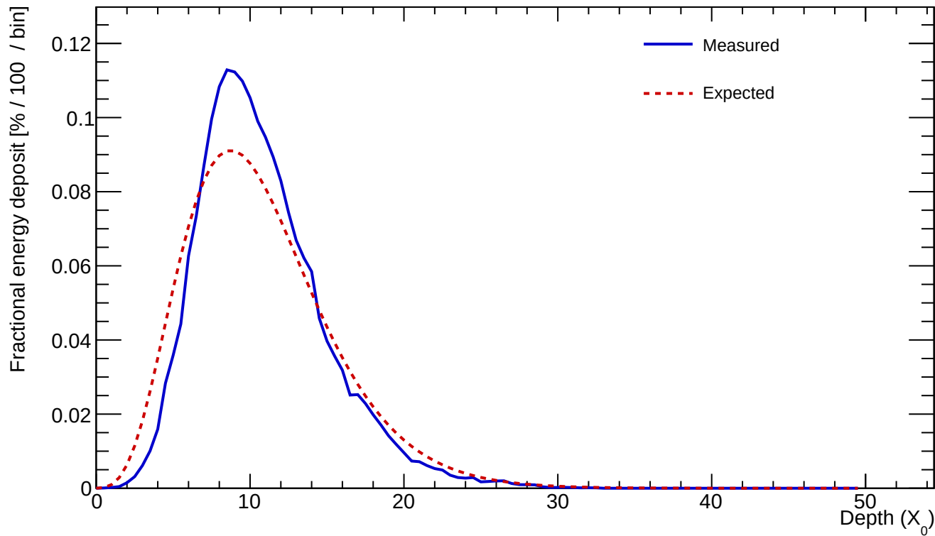
Cluster 25 E=500.274 GeV profileStart=0.50 X_0 \chi=0.1676
