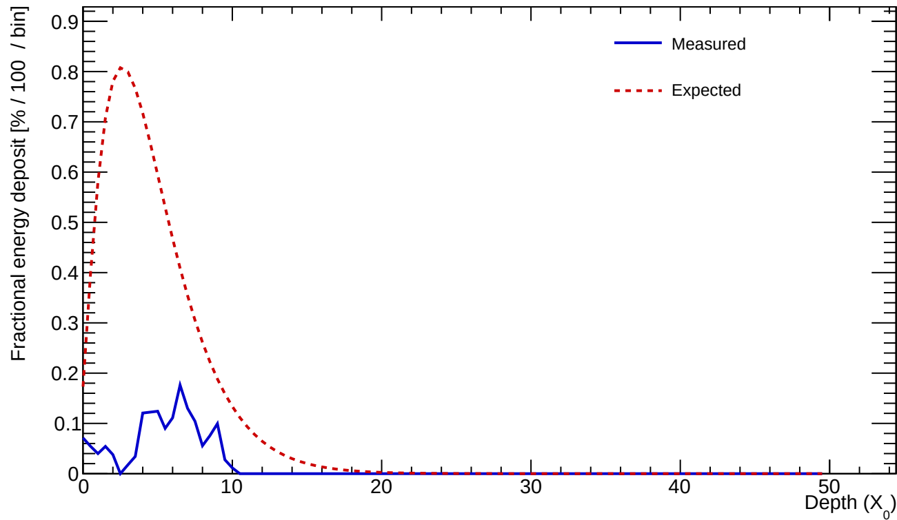
Cluster 4 E=1.092 GeV profileStart=3.00 X_0 \chi=0.3733
