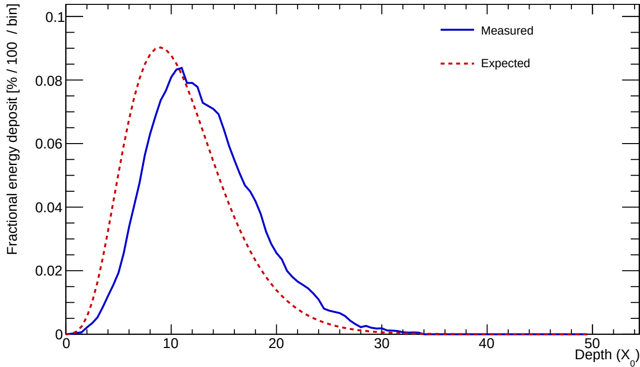
Cluster 318 E=603.898 GeV profileStart=2.00 X_0 \chi=0.0979
