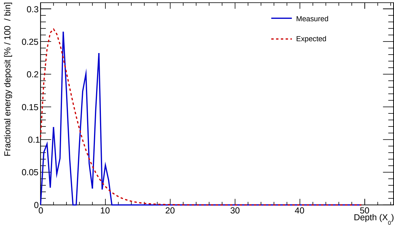
Cluster 51 E=0.551 GeV profileStart=1.50 X_0 \chi=0.7238
