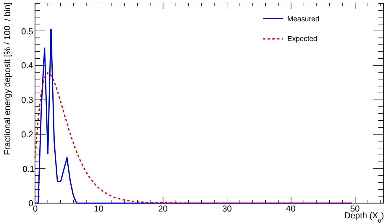
Cluster 70 E=0.626 GeV profileStart=0.50 X_0 \chi=0.5853
