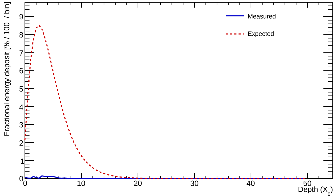
Cluster 231 E=0.912 GeV profileStart=0.50 X_0 \chi=0.5617
