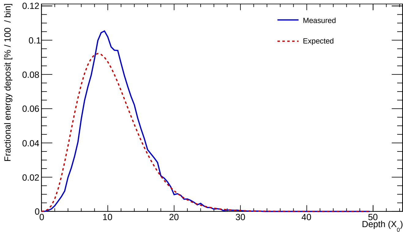
Cluster 44 E=404.431 GeV profileStart=1.00 X_0 \chi=0.0955
