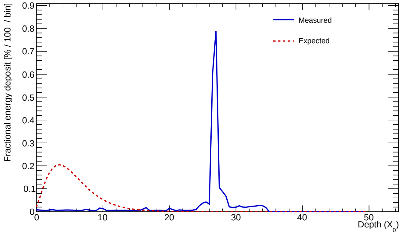
Cluster 45 E=2.449 GeV profileStart=24.00 X_0 \chi=1.0932
