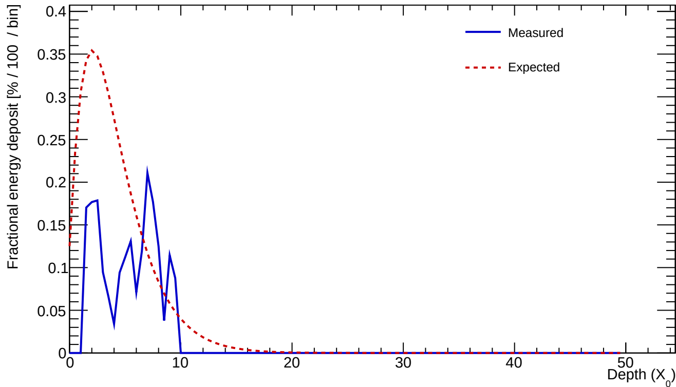
Cluster 68 E=0.612 GeV profileStart=1.00 X_0 \chi=0.5016
