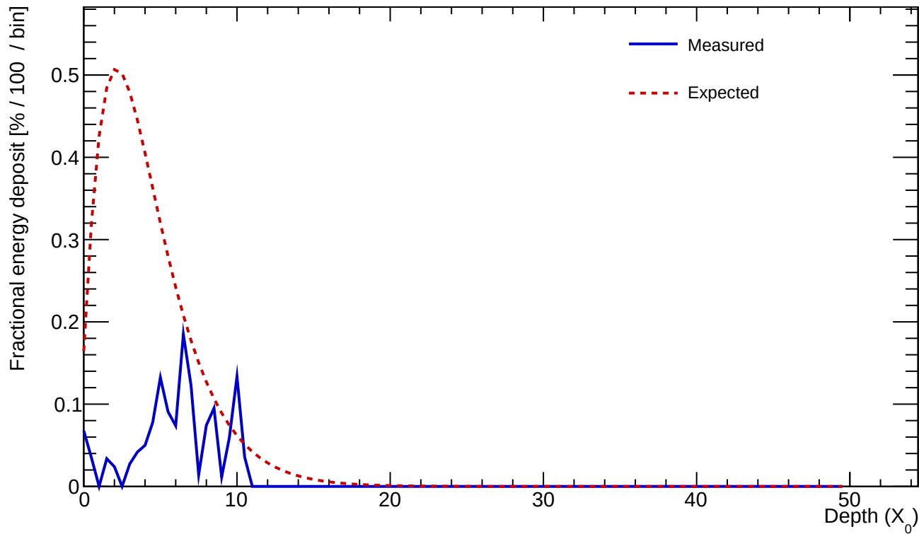
Cluster 53 E=0.681 GeV profileStart=3.50 X_0 \chi=0.4815
