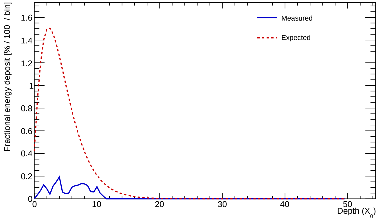
Cluster 396 E=0.813 GeV profileStart=2.00 X_0 \chi=0.4751
