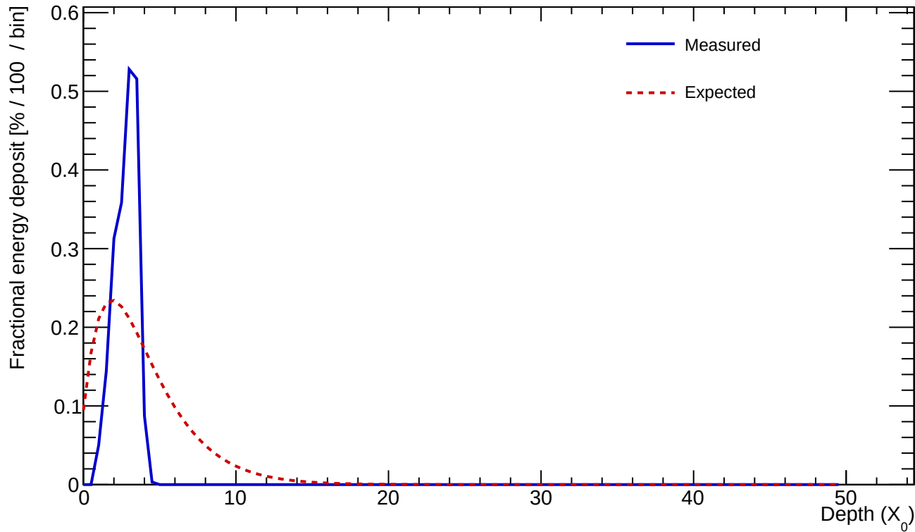
Cluster 395 E=0.518 GeV profileStart=1.00 X_0 \chi=0.5824
