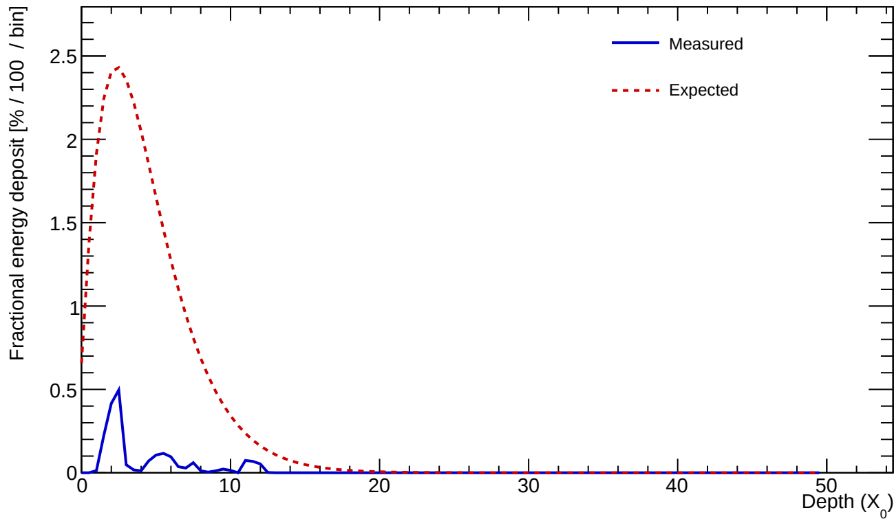
Cluster 2 E=0.843 GeV profileStart=0.50 X_0 \chi=0.8426
