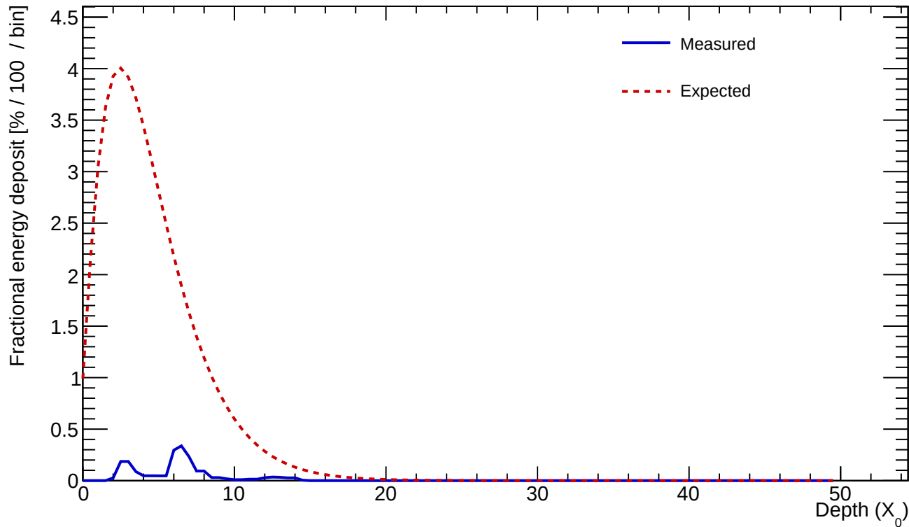
Cluster 324 E=0.931 GeV profileStart=2.00 X_0 \chi=0.7240
