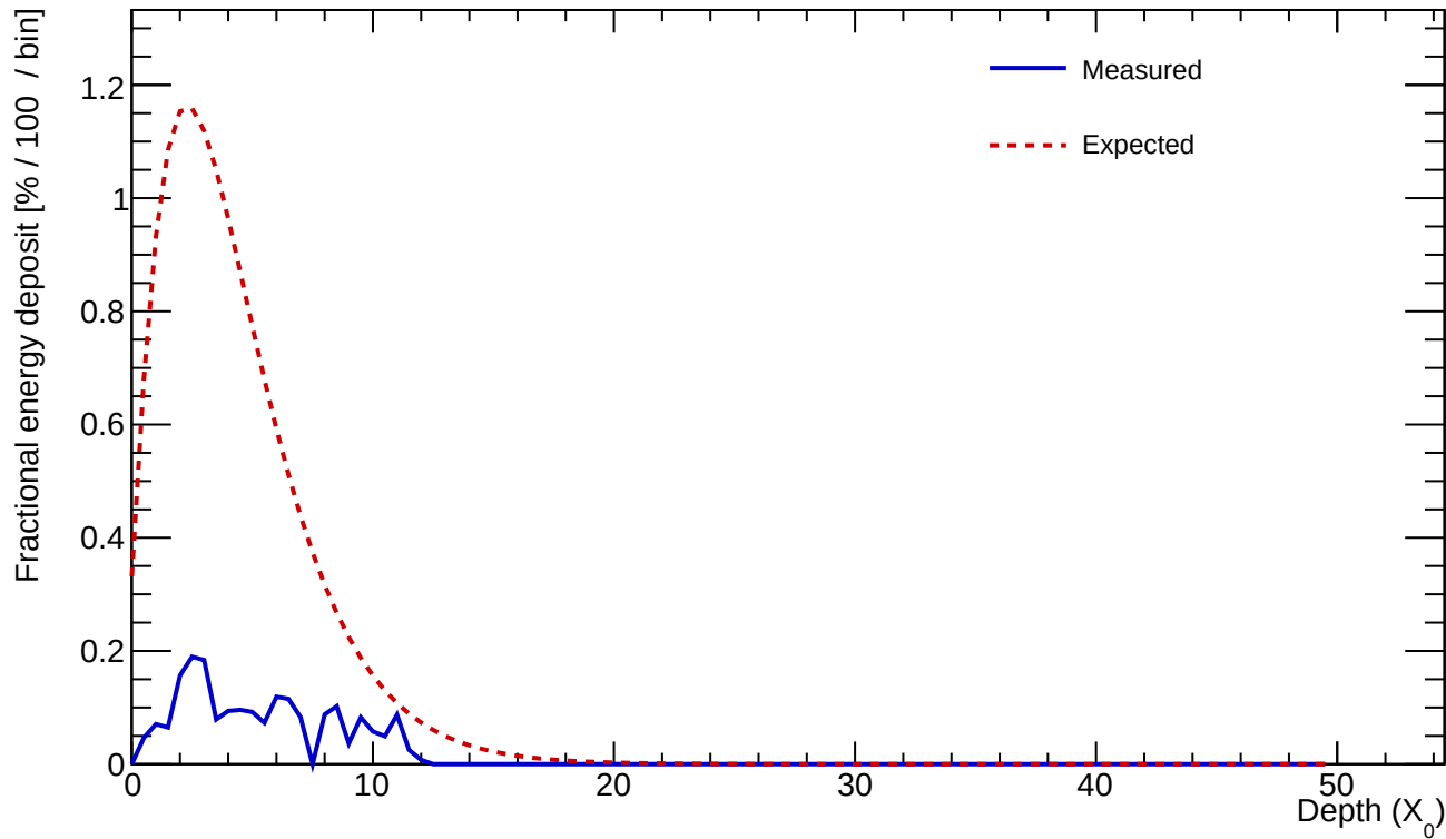
Cluster 158 E=0.791 GeV profileStart=0.50 X_0 \chi=0.3958
