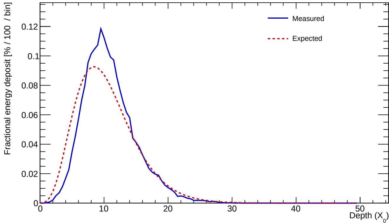
Cluster 48 E=367.406 GeV profileStart=1.00 X_0 \chi=0.1615
