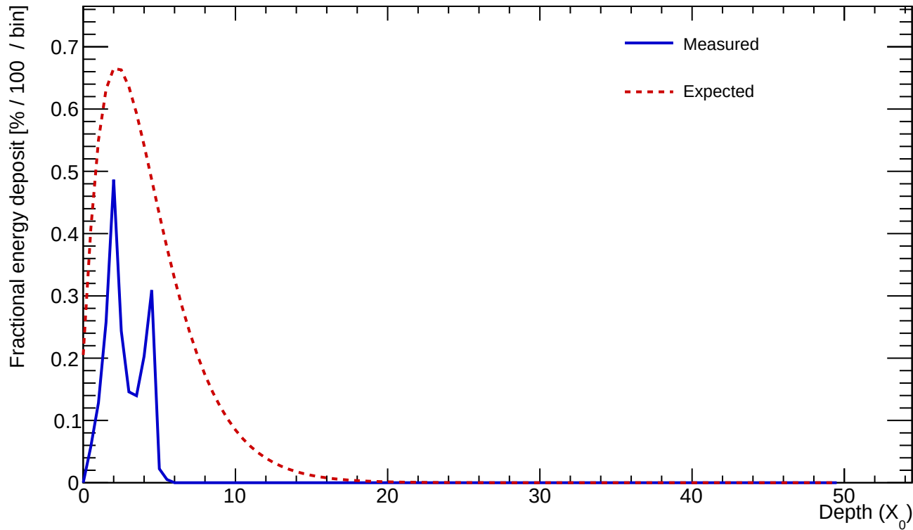
Cluster 353 E=0.725 GeV profileStart=0.50 X_0 \chi=0.4708
