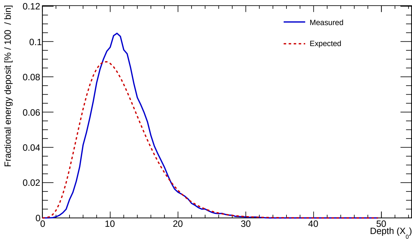
Cluster 18 E=874.176 GeV profileStart=1.00 X_0 \chi=0.1213
