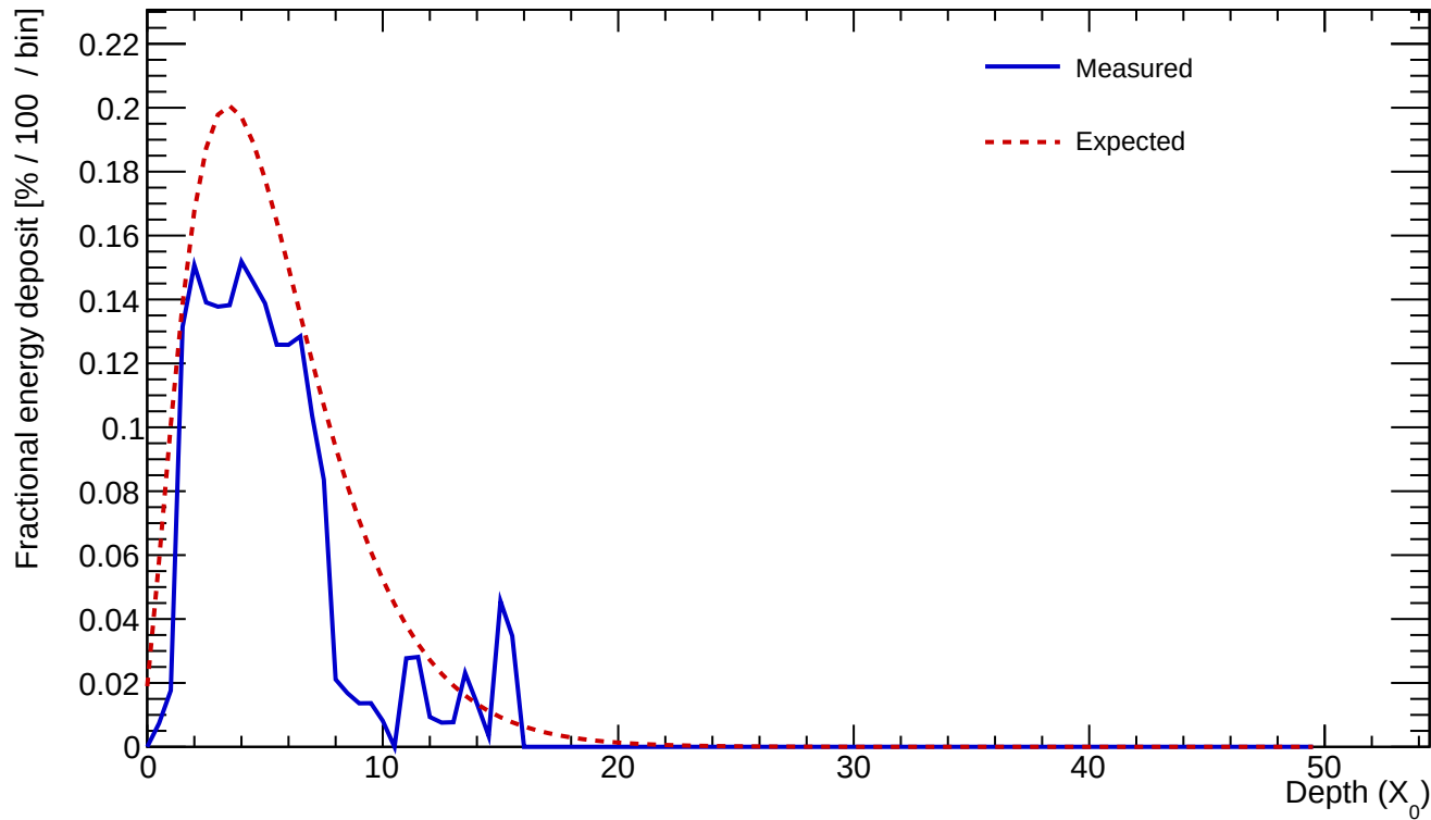
Cluster 6 E=2.525 GeV profileStart=0.50 X_0 \chi=0.3104
