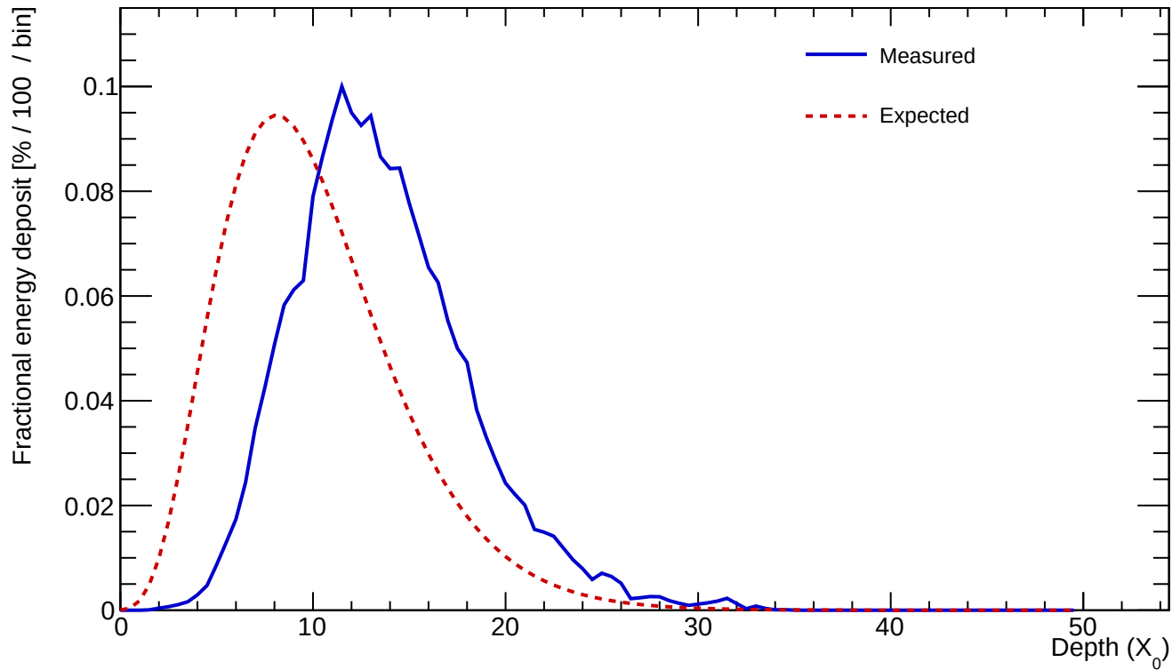
Cluster 217 E=259.220 GeV profileStart=3.50 X_0 \chi=0.0779
