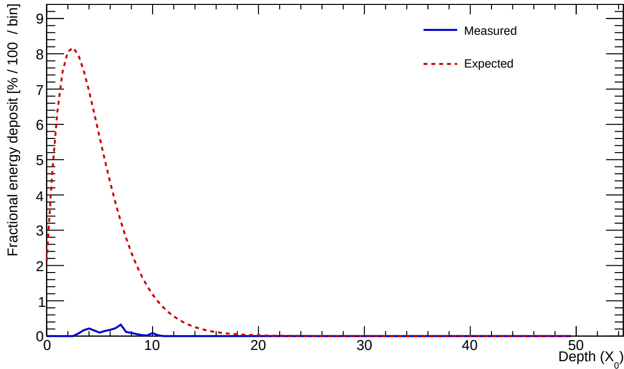
Cluster 322 E=0.880 GeV profileStart=2.50 X_0 \chi=0.3644
