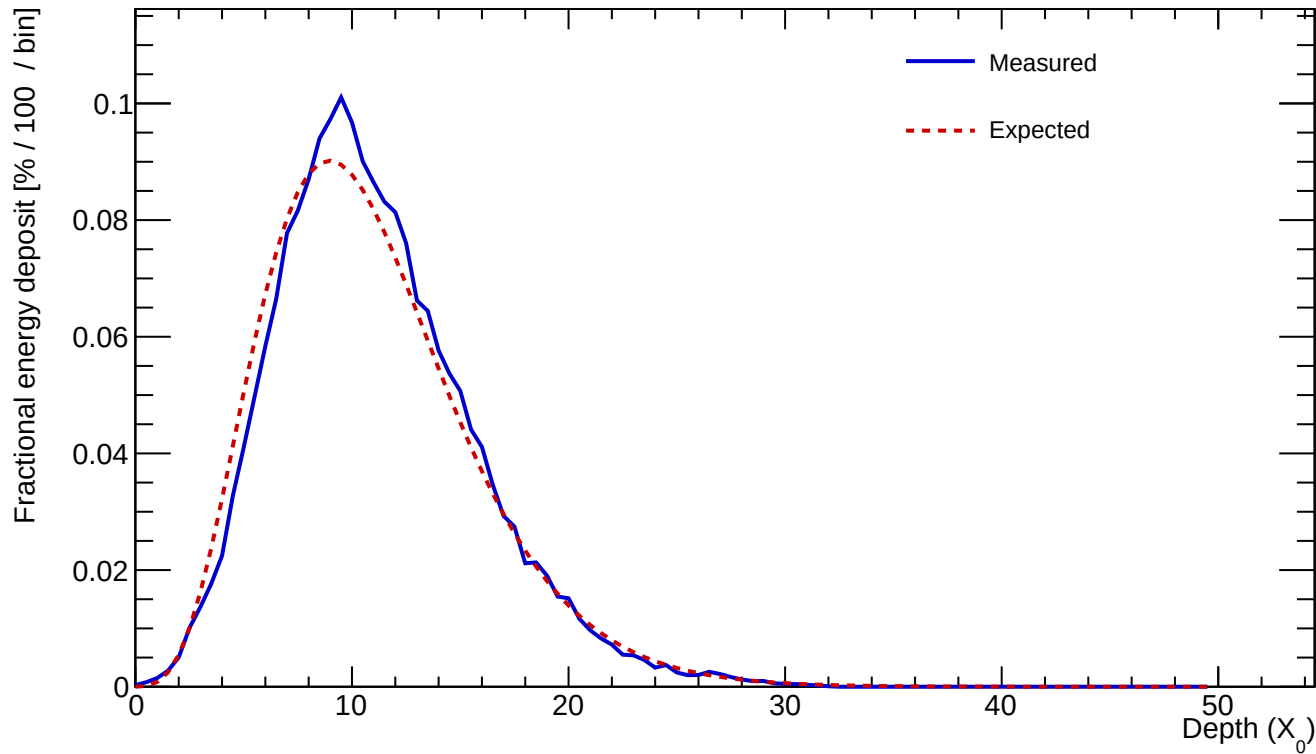
Cluster 115 E=614.362 GeV profileStart=0.50 X_0 \chi=0.0587
