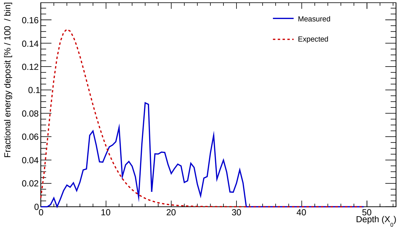
Cluster 269 E=4.565 GeV profileStart=9.00 X_0 \chi=0.9313
