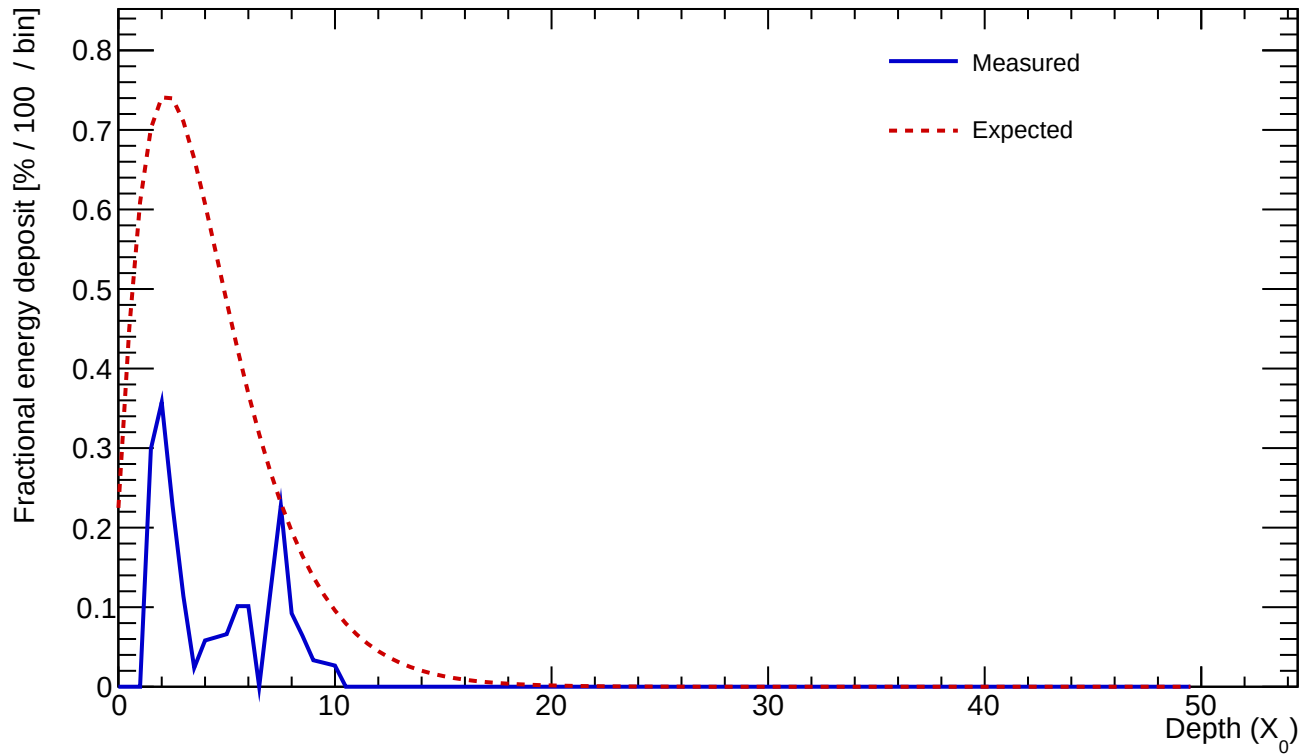
Cluster 354 E=0.740 GeV profileStart=0.50 X_0 \chi=0.6717
