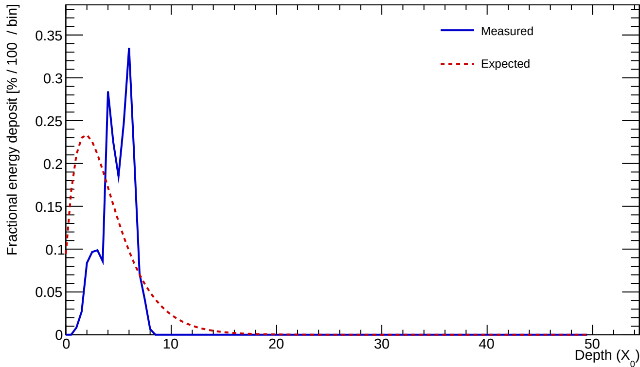
Cluster 67 E=0.517 GeV profileStart=2.50 X_0 \chi=0.4452
