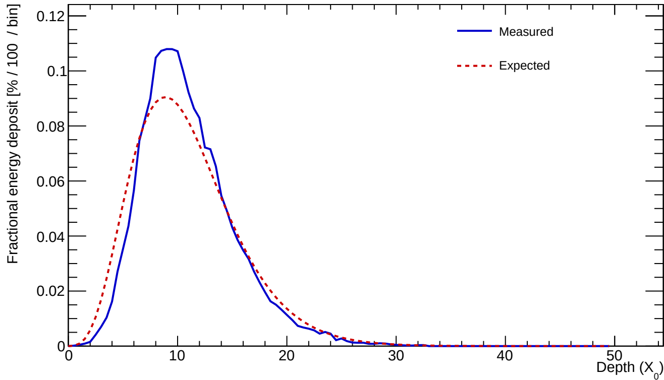
Cluster 24 E=570.082 GeV profileStart=0.50 X_0 \chi=0.1467
