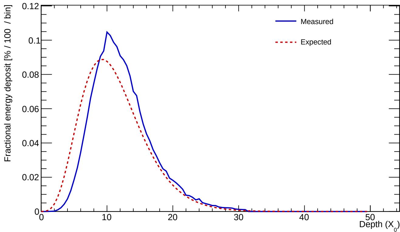
Cluster 80 E=830.333 GeV profileStart=1.50 X_0 \chi=0.1048
