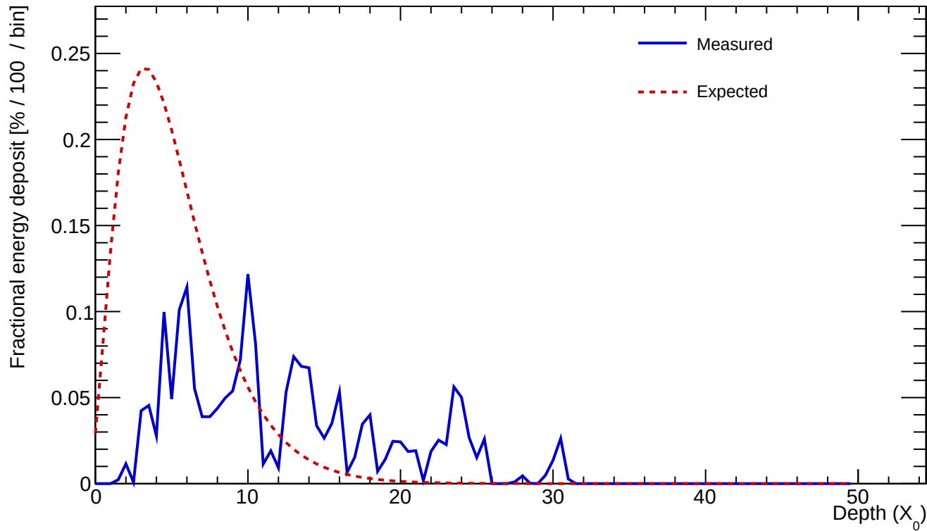
Cluster 64 E=1.991 GeV profileStart=4.00 X_0 \chi=0.7806
