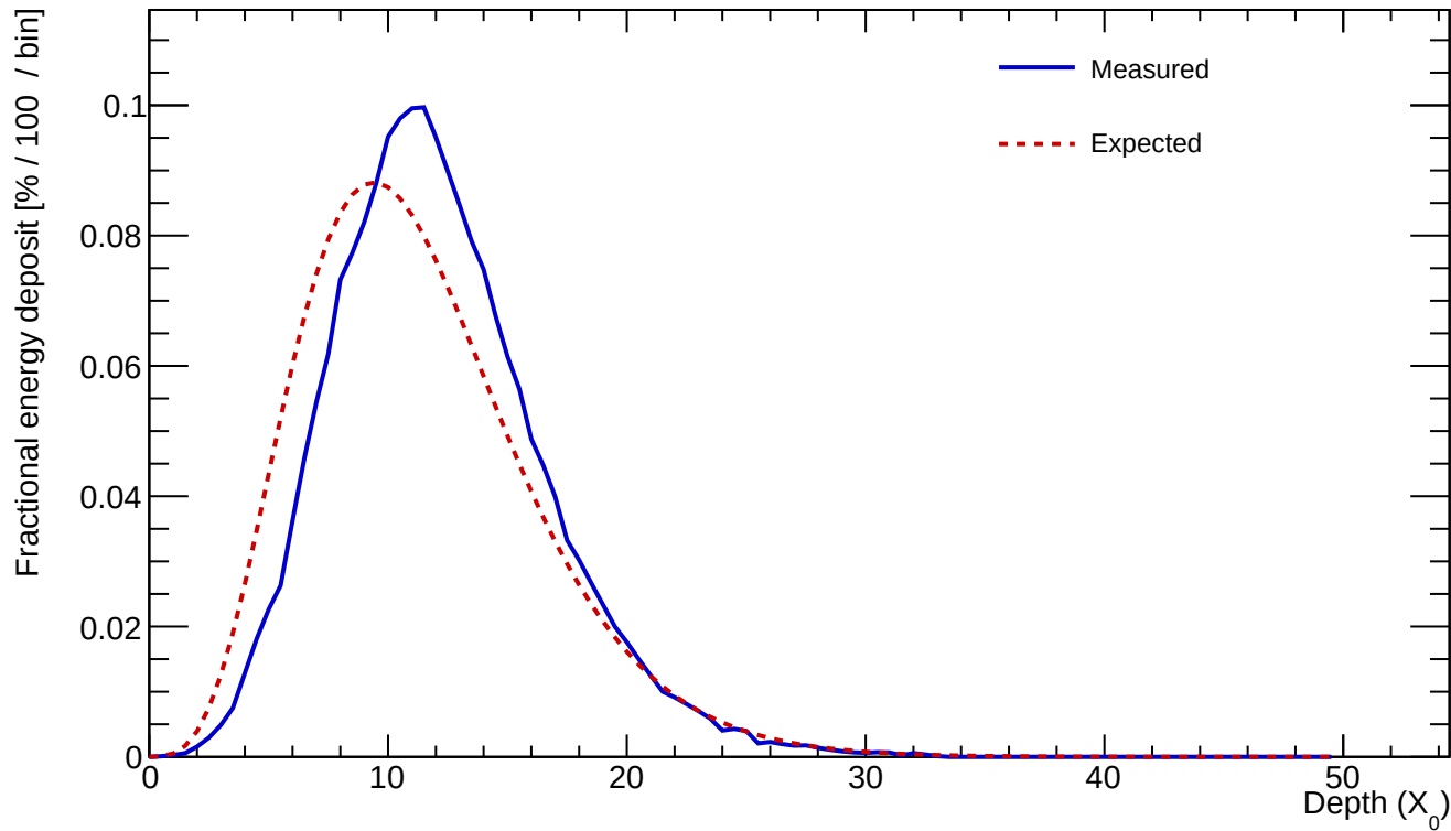
Cluster 9 E=963.523 GeV profileStart=1.00 X_0 \chi=0.1031
