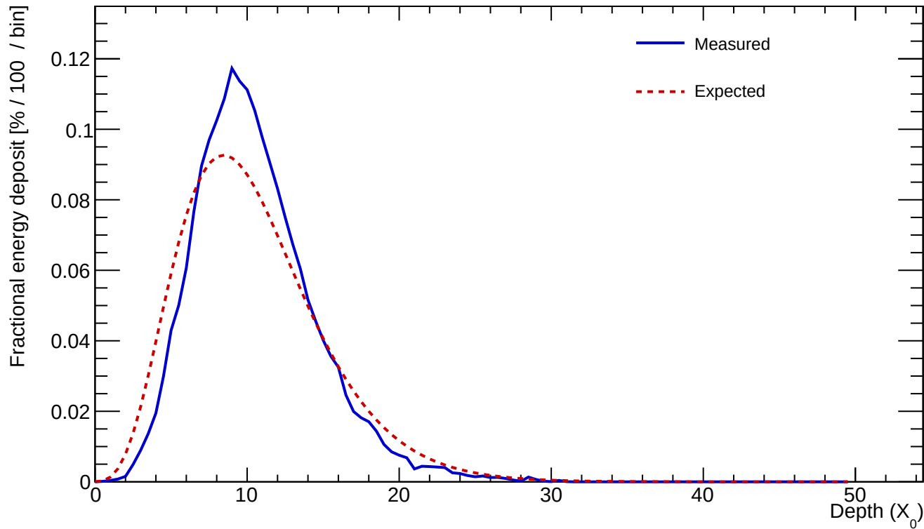
Cluster 23 E=366.990 GeV profileStart=0.50 X_0 \chi=0.1755
