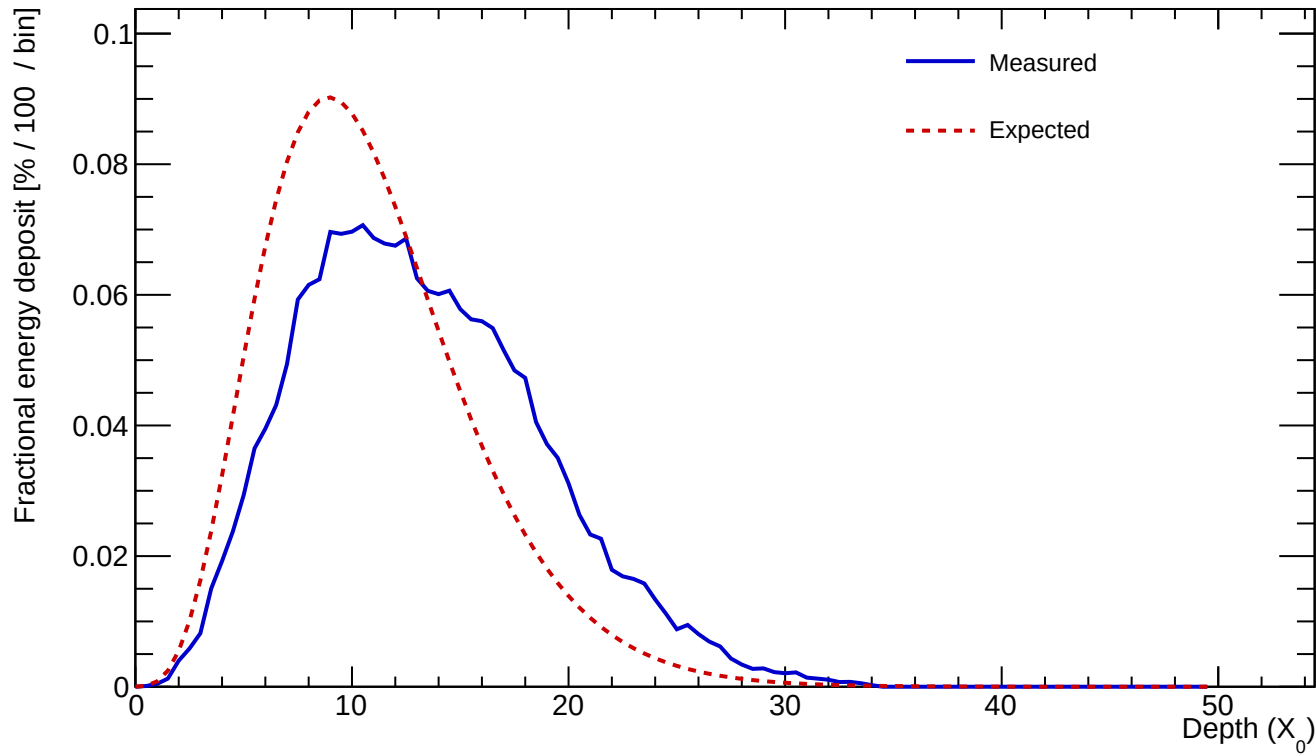
Cluster 11 E=608.651 GeV profileStart=2.00 X_0 \chi=0.2319
