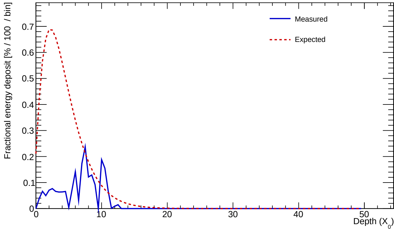
Cluster 229 E=0.730 GeV profileStart=4.50 X_0 \chi=0.6630
