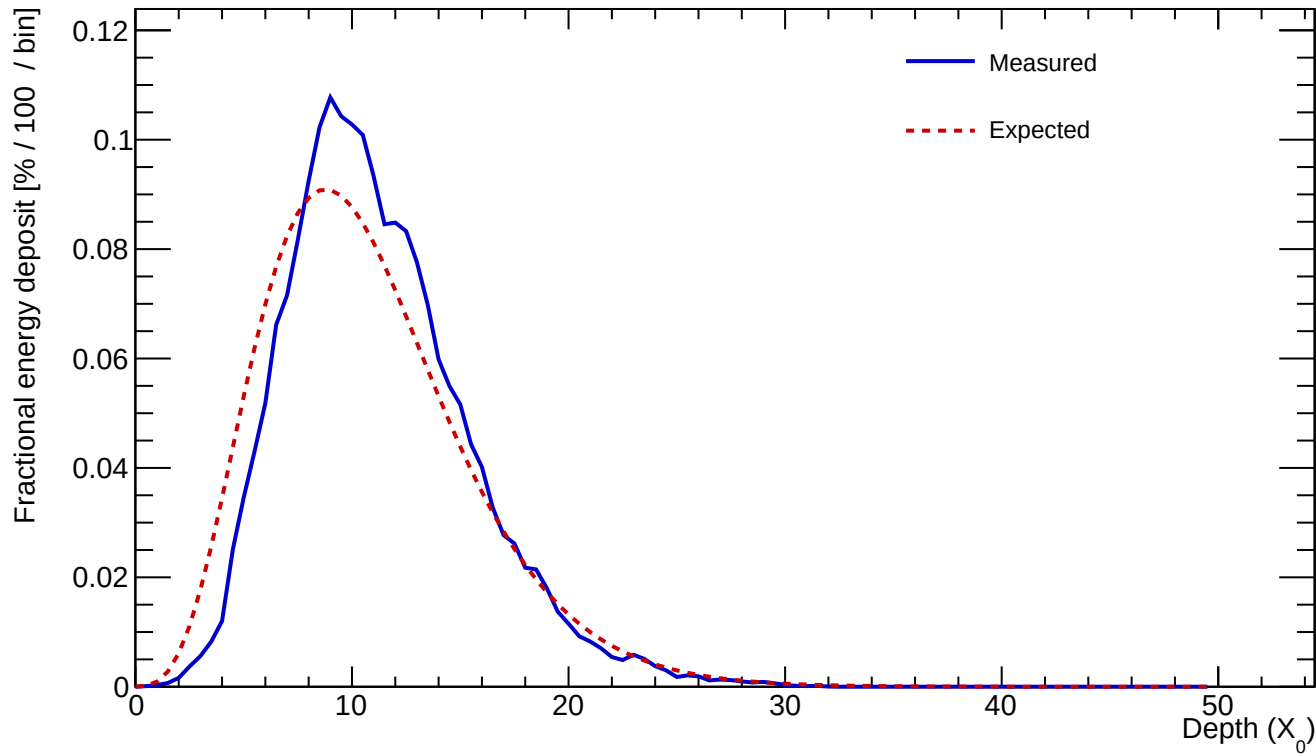
Cluster 17 E=523.137 GeV profileStart=1.00 X_0 \chi=0.1159
