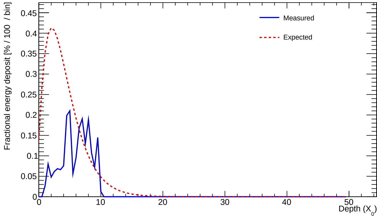
Cluster 343 E=0.644 GeV profileStart=3.50 X_0 \chi=0.4174
