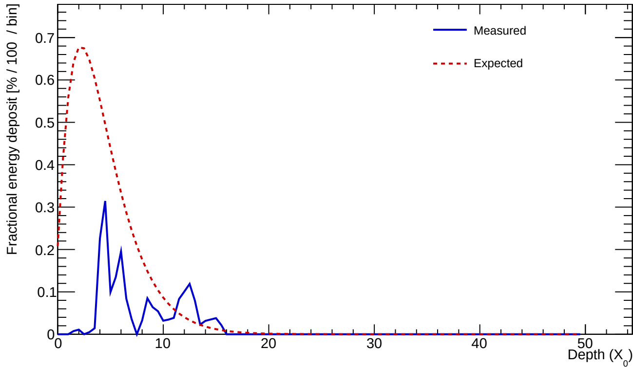
Cluster 95 E=0.727 GeV profileStart=3.00 X_0 \chi=0.6511
