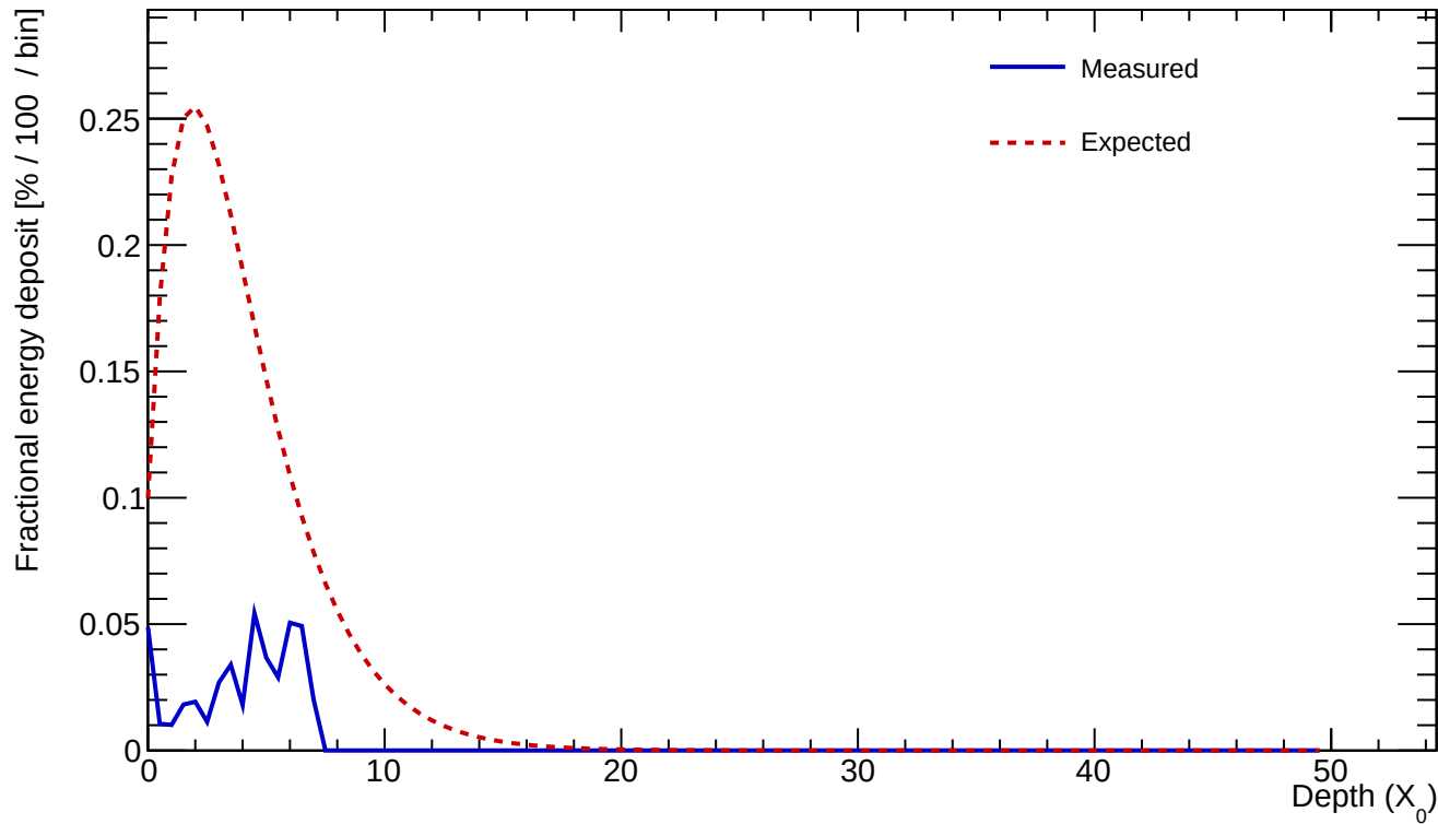
Cluster 388 E=0.538 GeV profileStart=2.50 X_0 \chi=0.4443
