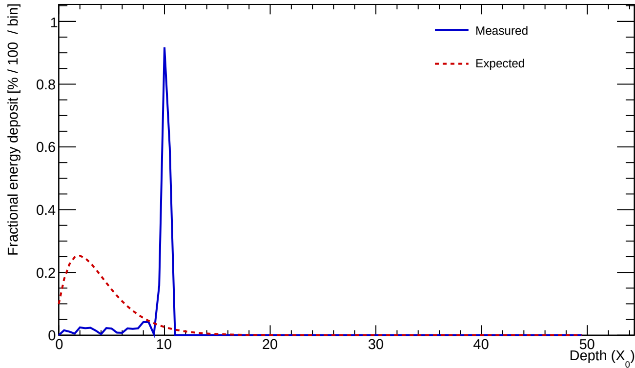
Cluster 176 E=0.537 GeV profileStart=8.50 X_0 \chi=0.5911
