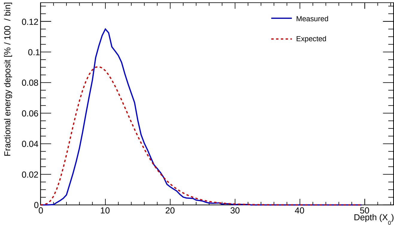
Cluster 118 E=586.199 GeV profileStart=1.50 X_0 \chi=0.1853
