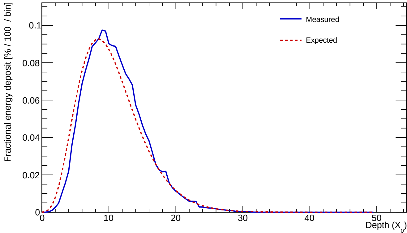
Cluster 43 E=364.055 GeV profileStart=0.50 X_0 \chi=0.0601
