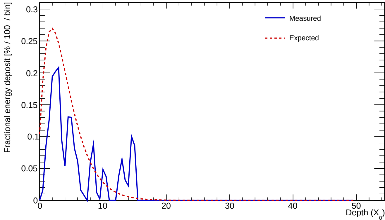
Cluster 228 E=0.552 GeV profileStart=0.50 X_0 \chi=0.5038
