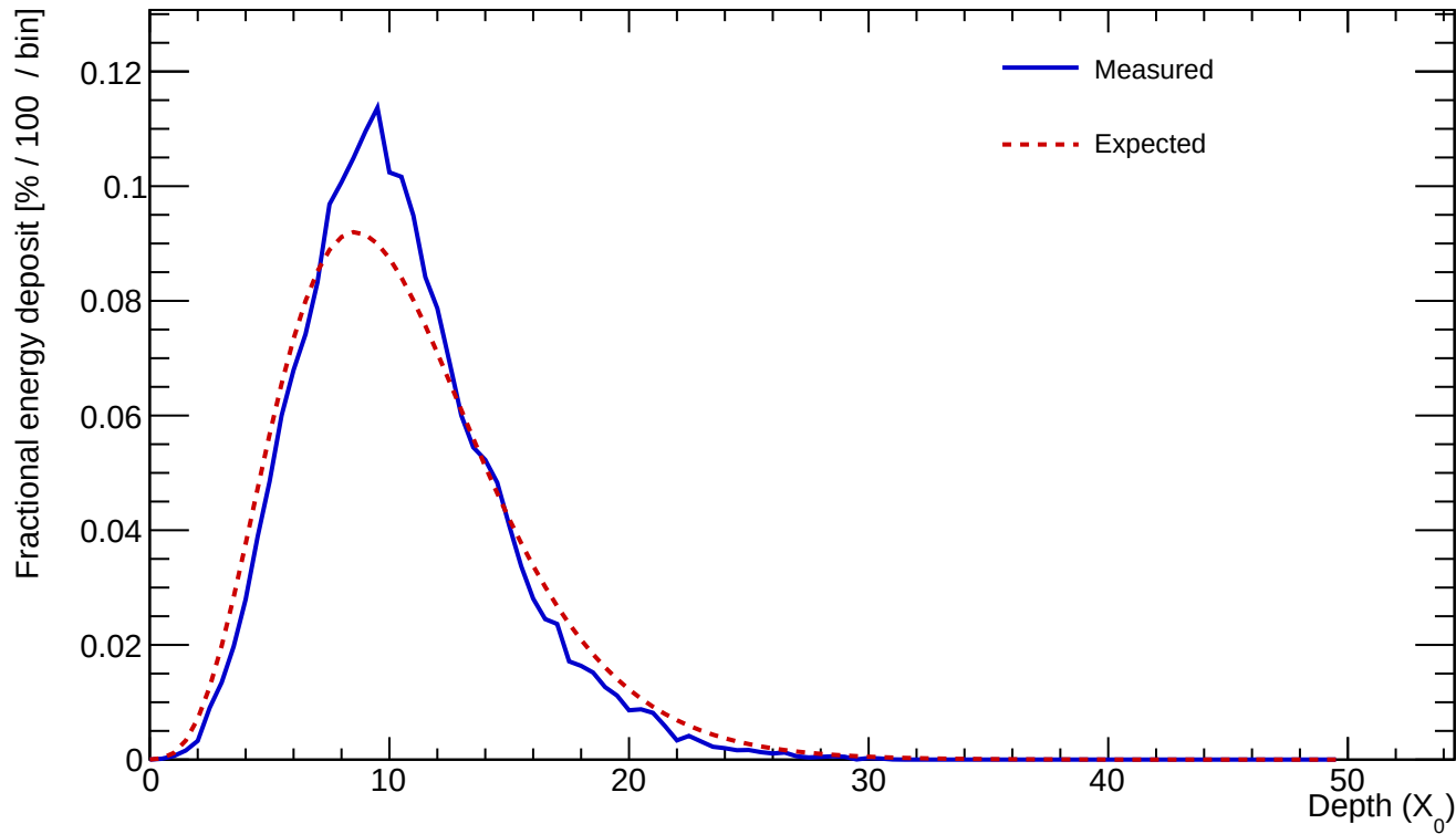
Cluster 57 E=421.725 GeV profileStart=0.50 X_0 \chi=0.1365
