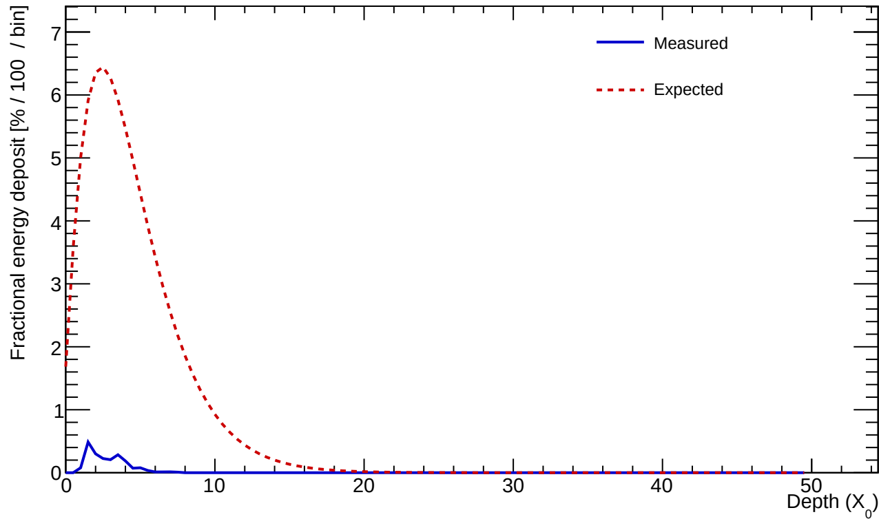
Cluster 387 E=0.875 GeV profileStart=0.50 X_0 \chi=0.6283
