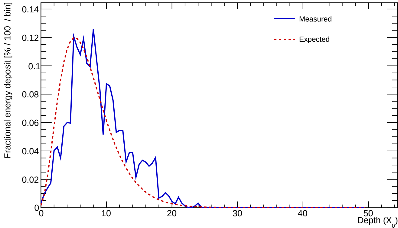
Cluster 7 E=14.030 GeV profileStart=1.50 X_0 \chi=0.2188
