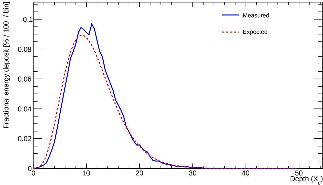
Cluster 16 E=735.772 GeV profileStart=0.50 X_0 \chi=0.0591
