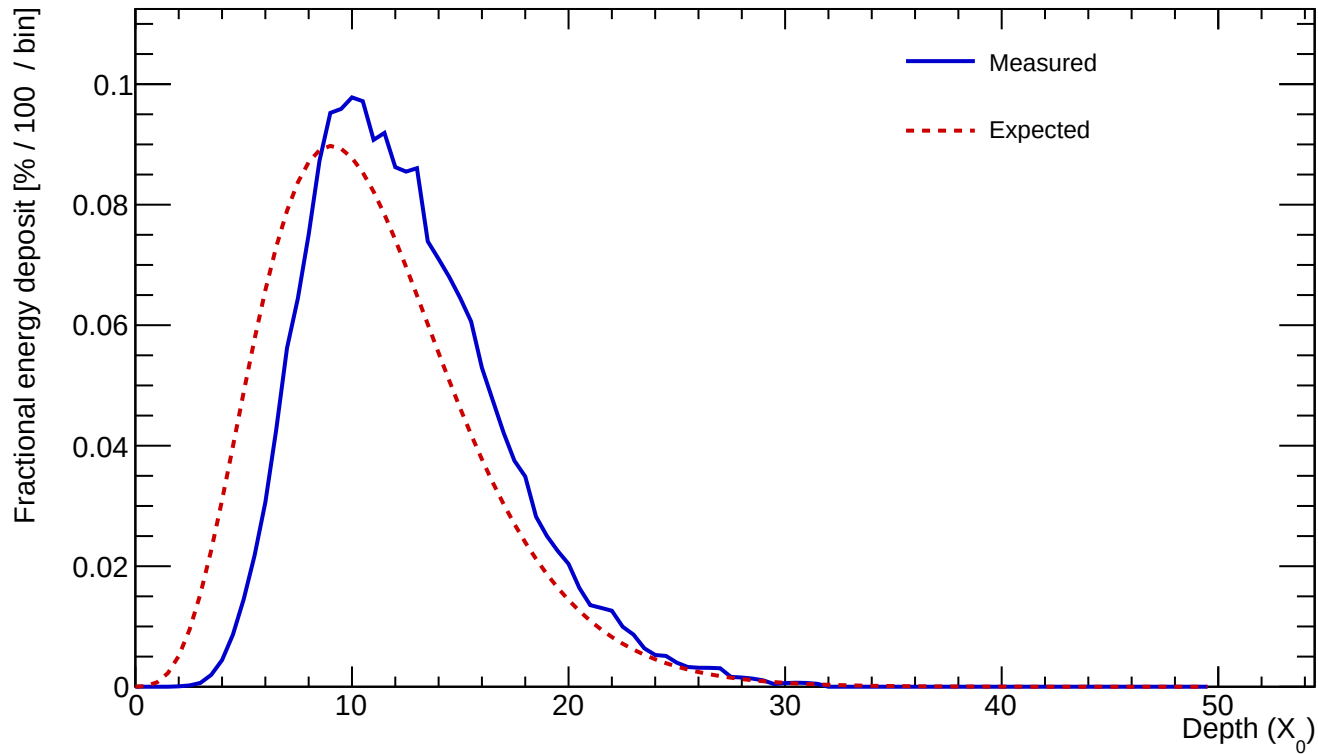
Cluster 49 E=675.652 GeV profileStart=1.50 X_0 \chi=0.0816
