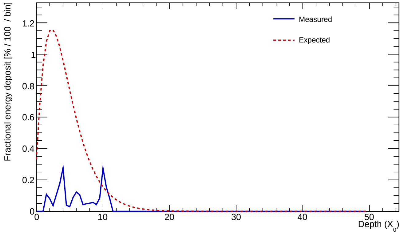
Cluster 310 E=0.790 GeV profileStart=1.50 X_0 \chi=0.5684
