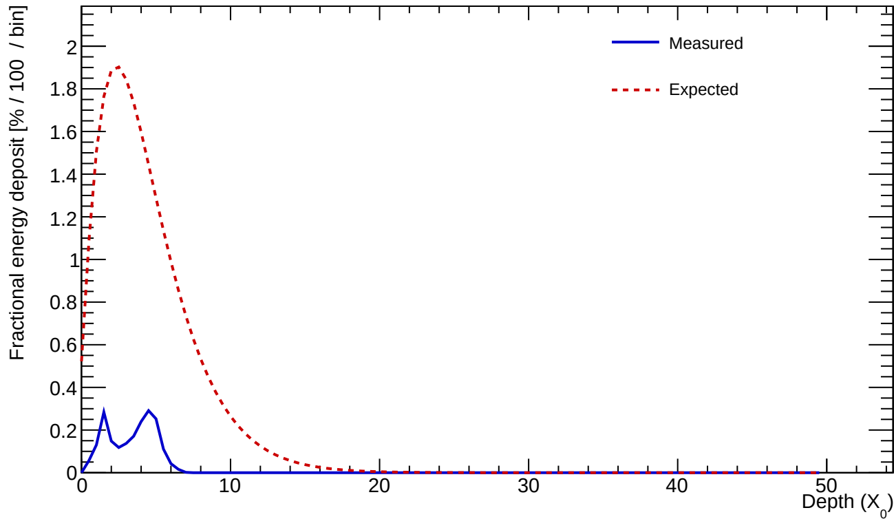
Cluster 340 E=0.829 GeV profileStart=0.50 X_0 \chi=0.4005
