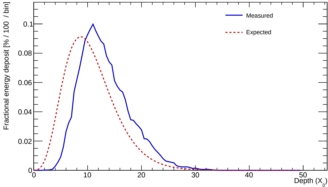
Cluster 113 E=485.065 GeV profileStart=2.50 X_0 \chi=0.0531
