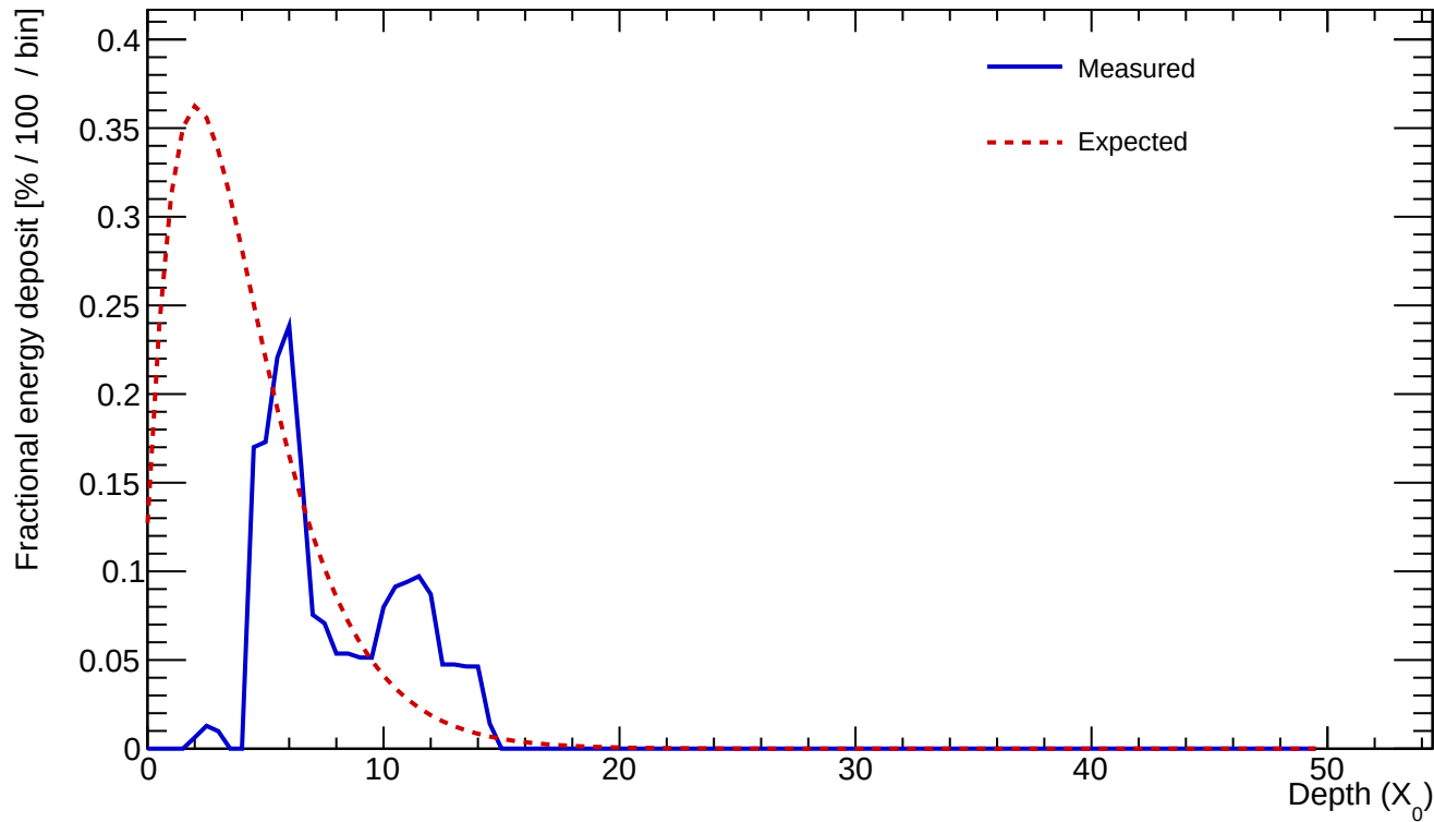
Cluster 173 E=0.617 GeV profileStart=4.00 X_0 \chi=0.4699
