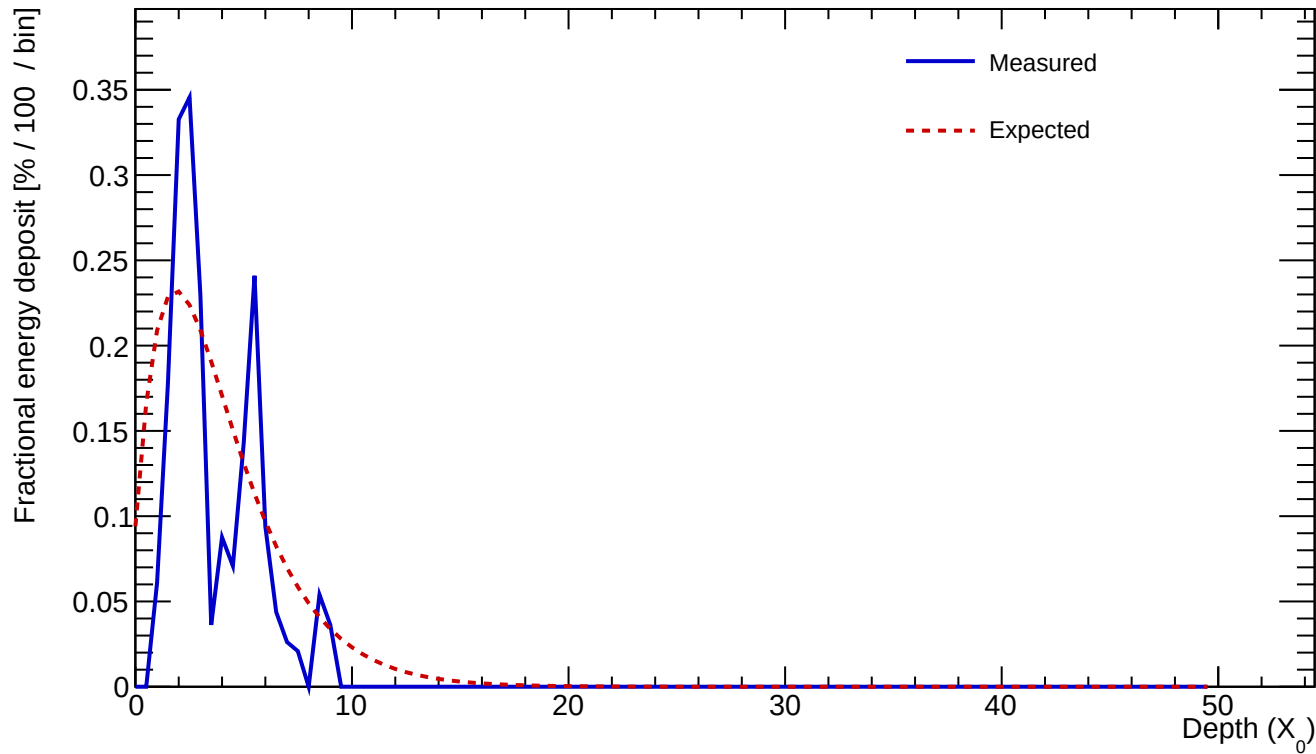
Cluster 298 E=0.515 GeV profileStart=1.00 X_0 \chi=0.5399
