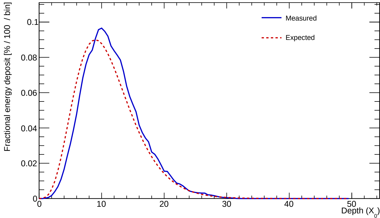
Cluster 167 E=648.987 GeV profileStart=1.00 X_0 \chi=0.0523
