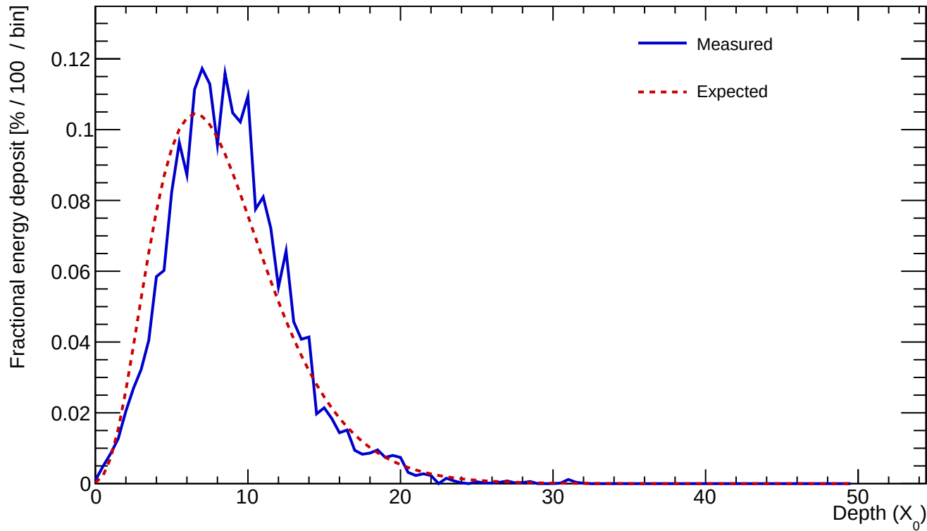
Cluster 81 E=55.465 GeV profileStart=0.50 X_0 \chi=0.1489
