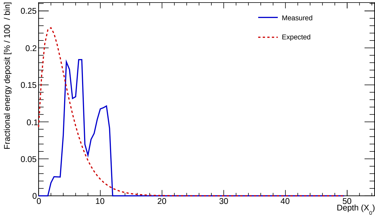
Cluster 218 E=0.511 GeV profileStart=4.00 X_0 \chi=0.3436
