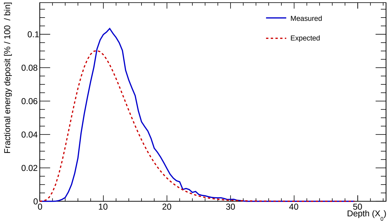
Cluster 19 E=605.459 GeV profileStart=2.00 X_0 \chi=0.1119
