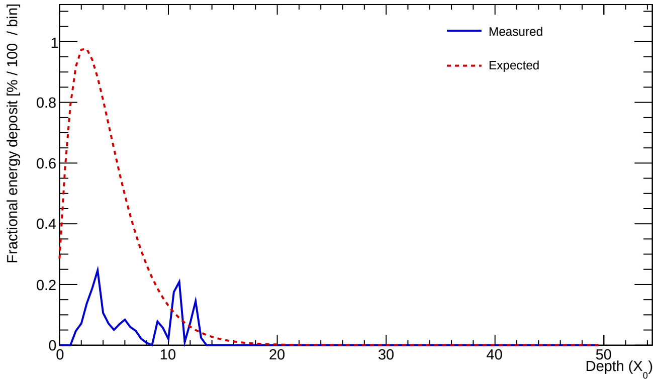
Cluster 390 E=0.773 GeV profileStart=1.50 X_0 \chi=0.6670
