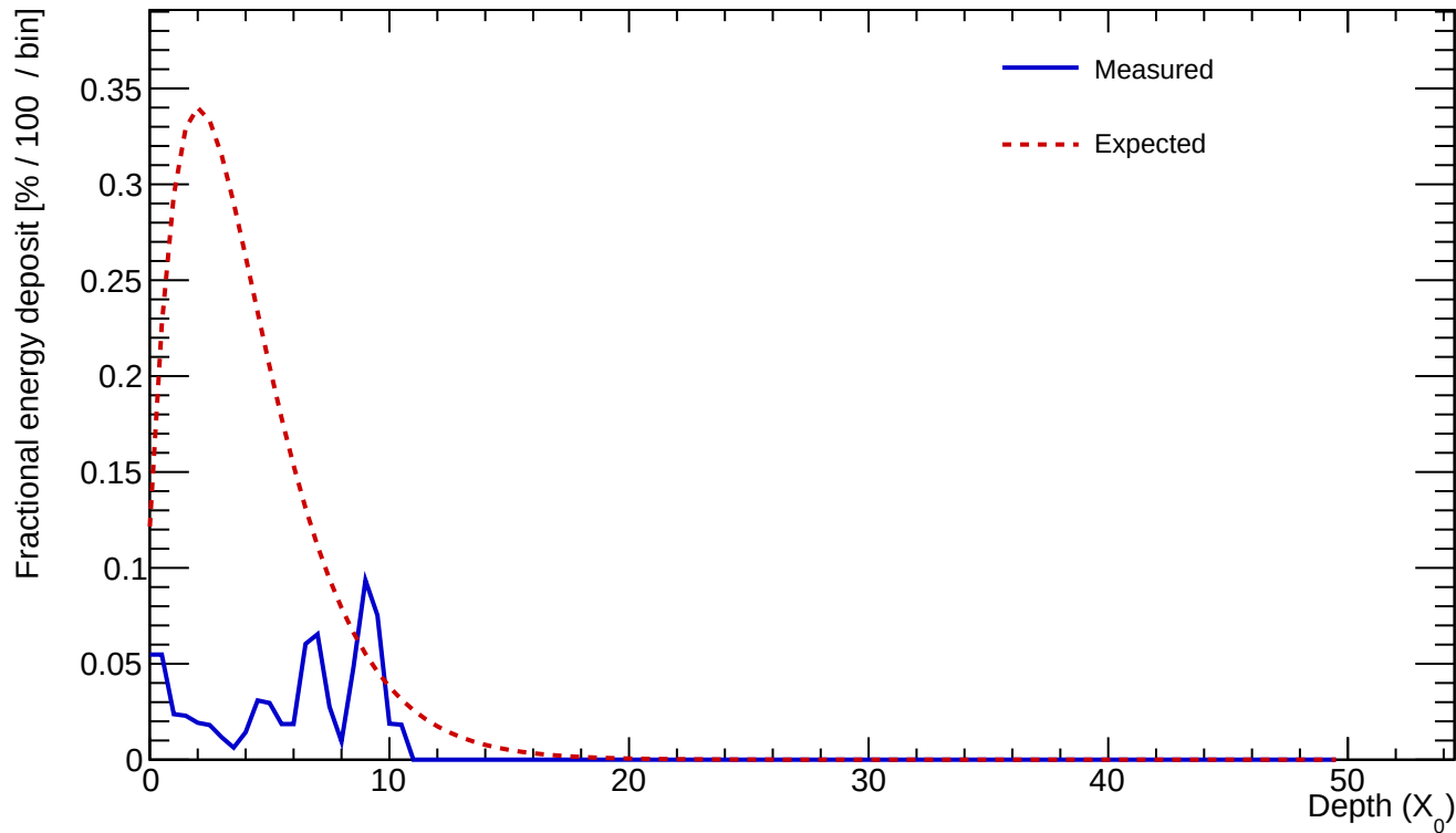
Cluster 260 E=0.604 GeV profileStart=4.50 X_0 \chi=0.6817
