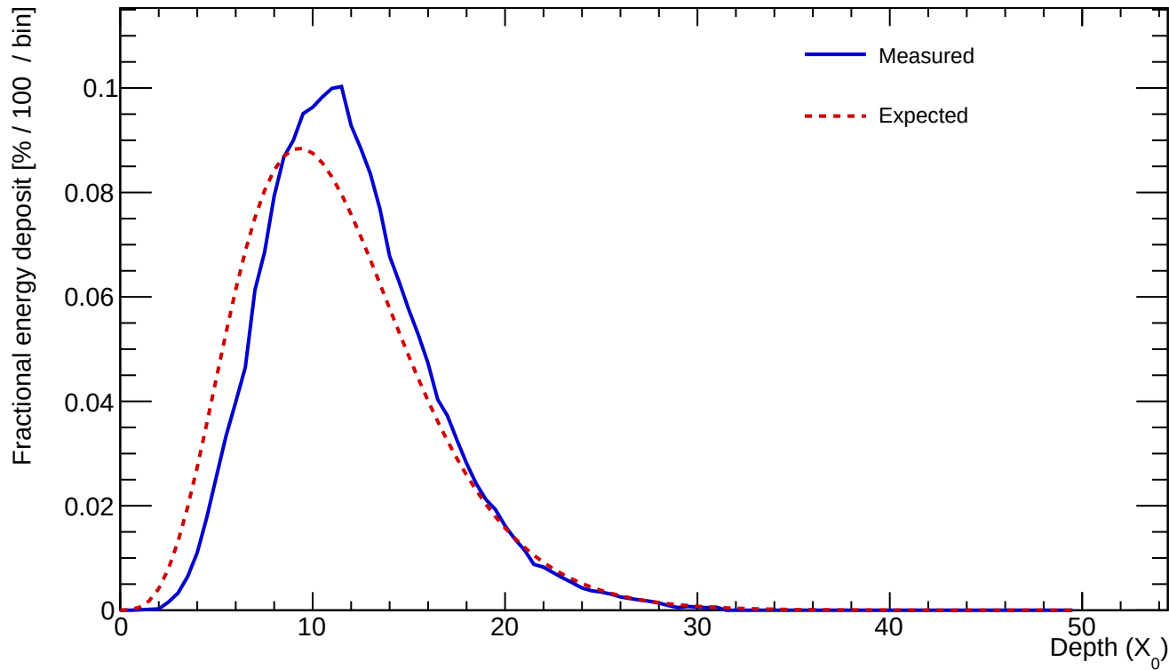
Cluster 78 E=893.692 GeV profileStart=1.00 X_0 \chi=0.1001
