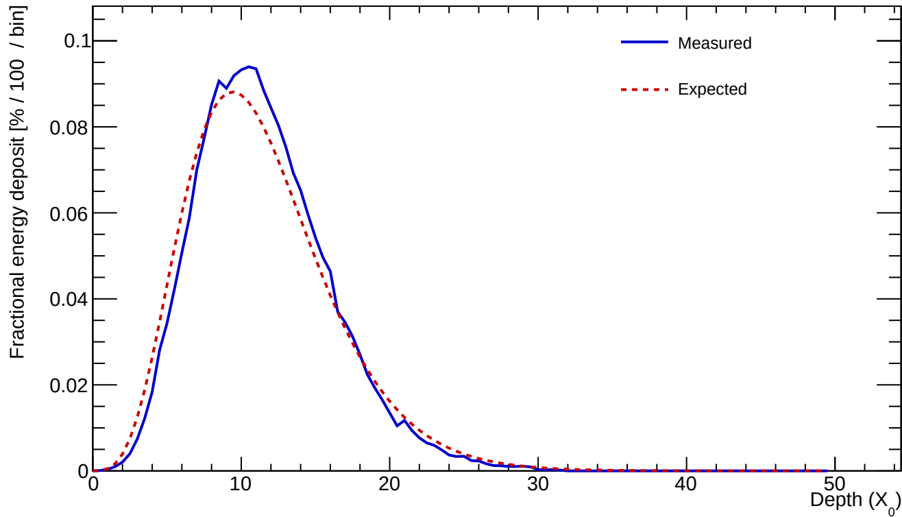
Cluster 75 E=973.936 GeV profileStart=0.50 X_0 \chi=0.0704
