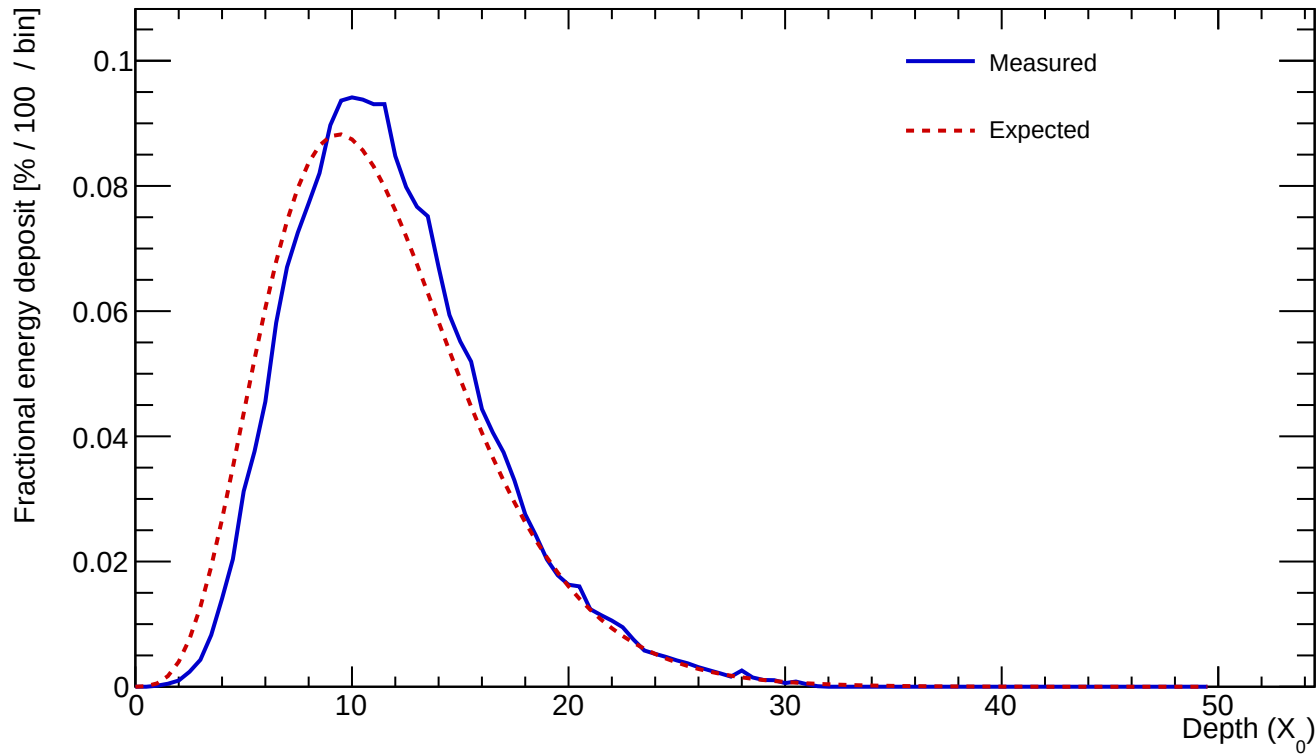
Cluster 422 E=945.115 GeV profileStart=0.50 X_0 \chi=0.0695
