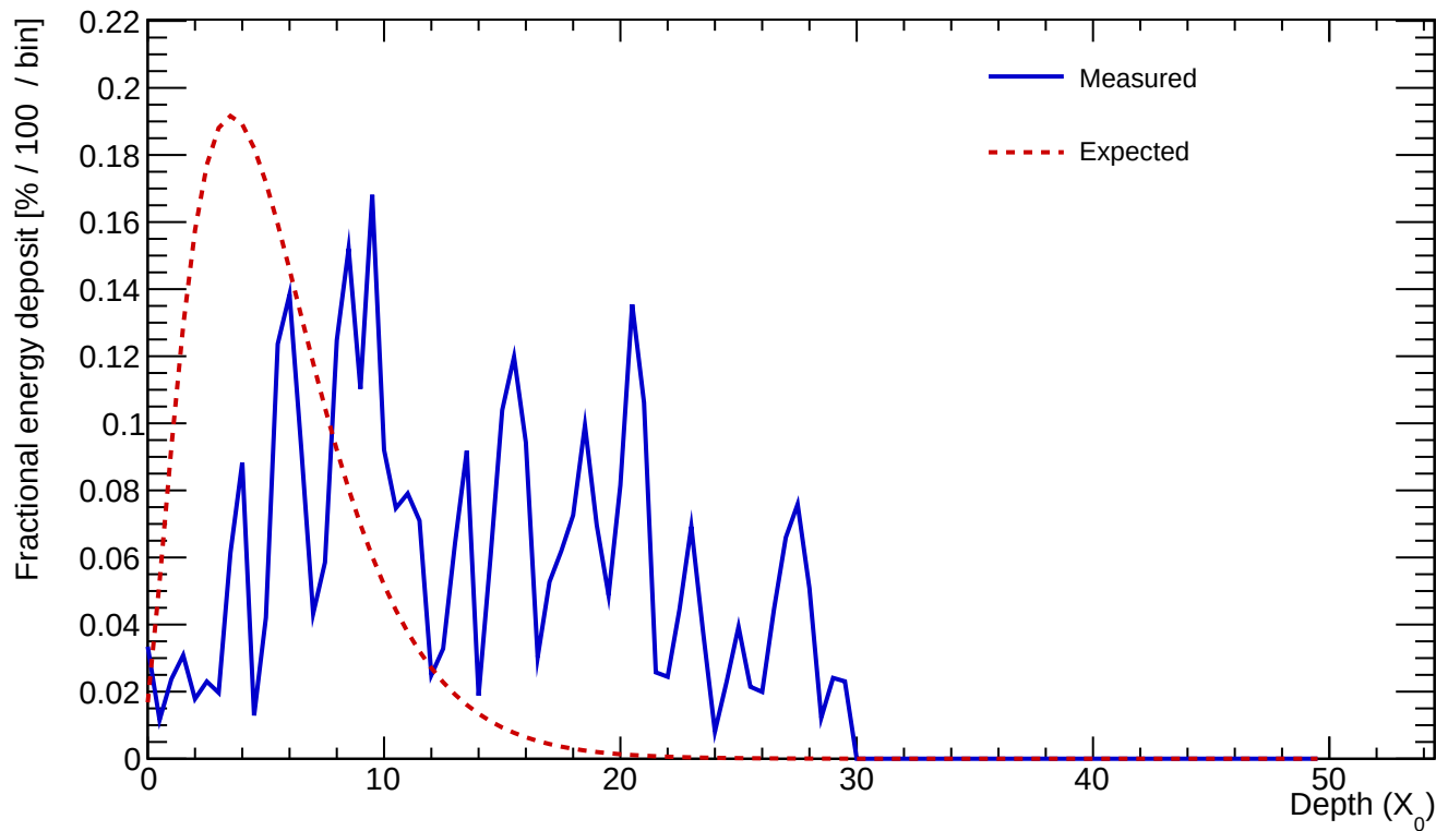
Cluster 125 E=2.715 GeV profileStart=4.50 X_0 \chi=0.8919
