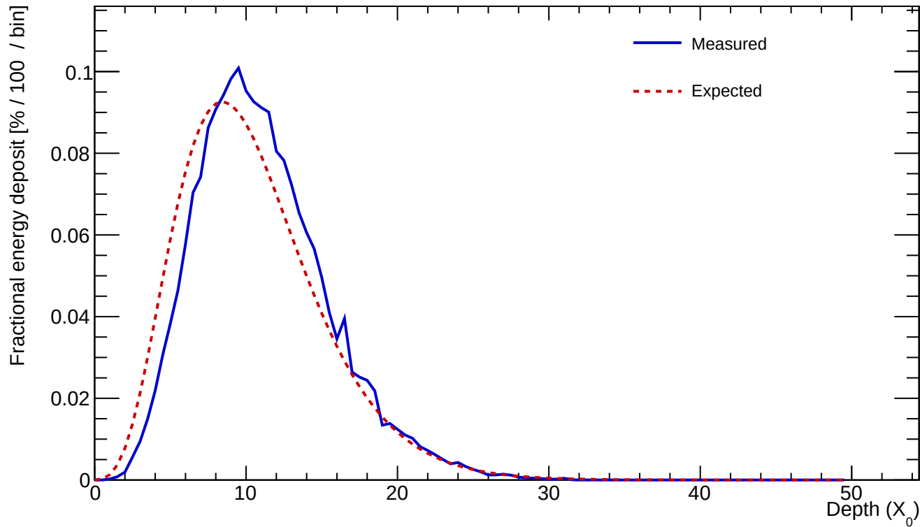
Cluster 37 E=370.430 GeV profileStart=1.00 X_0 \chi=0.0653
