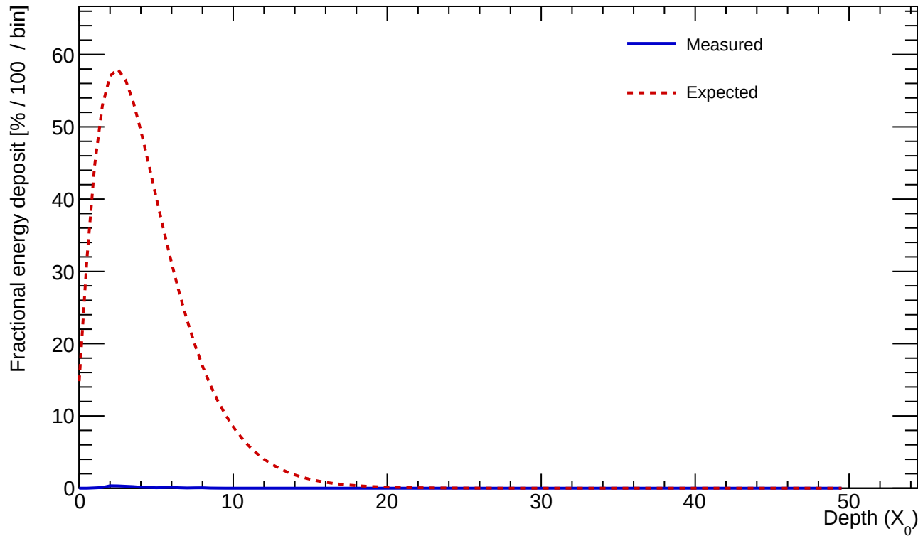
Cluster 389 E=0.898 GeV profileStart=0.50 X_0 \chi=0.4527
