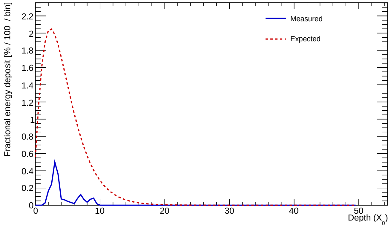
Cluster 97 E=0.834 GeV profileStart=1.00 X_0 \chi=0.6823
