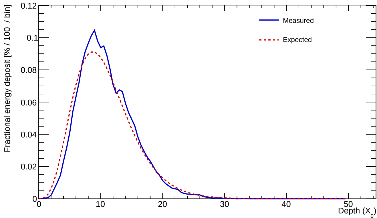
Cluster 178 E=497.944 GeV profileStart=0.50 X_0 \chi=0.0792
