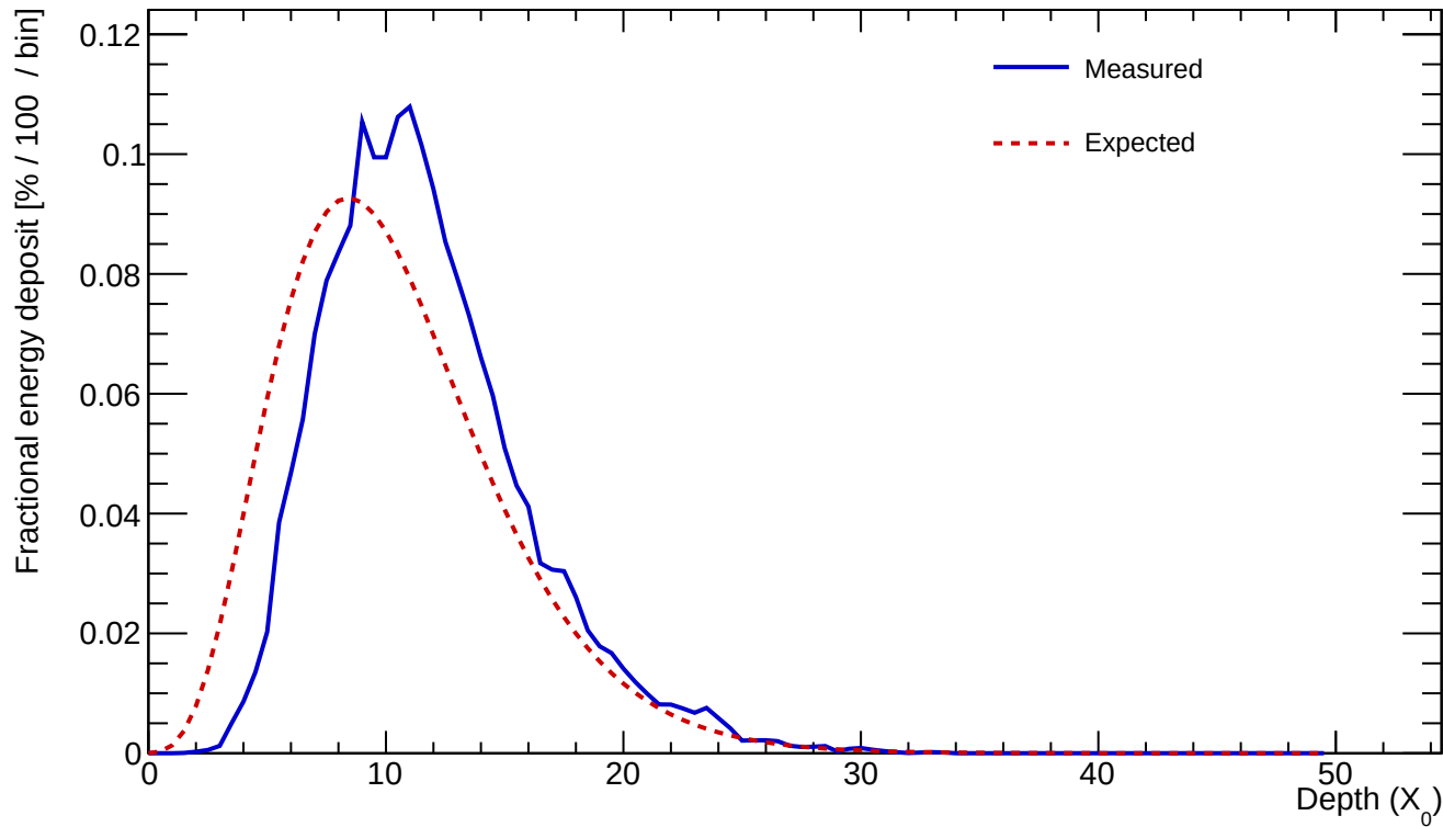
Cluster 38 E=364.665 GeV profileStart=1.50 X_0 \chi=0.1109
