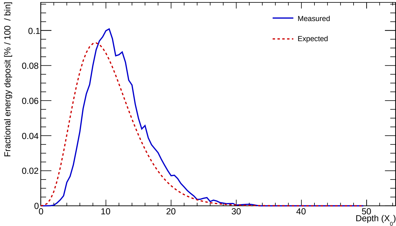
Cluster 415 E=351.498 GeV profileStart=1.50 X_0 \chi=0.0721
