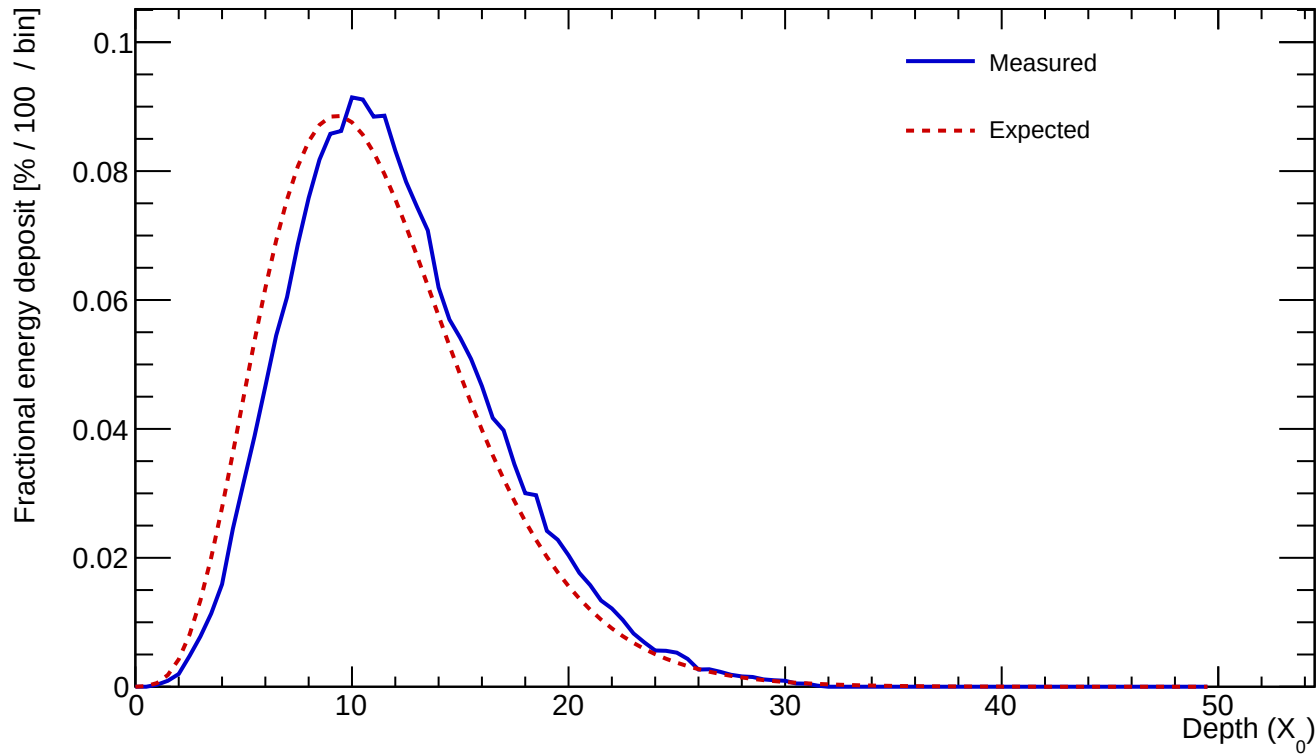
Cluster 42 E=866.781 GeV profileStart=1.00 X_0 \chi=0.0404
