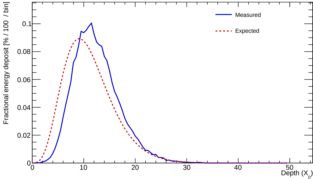
Cluster 35 E=742.416 GeV profileStart=1.50 X_0 \chi=0.0933
