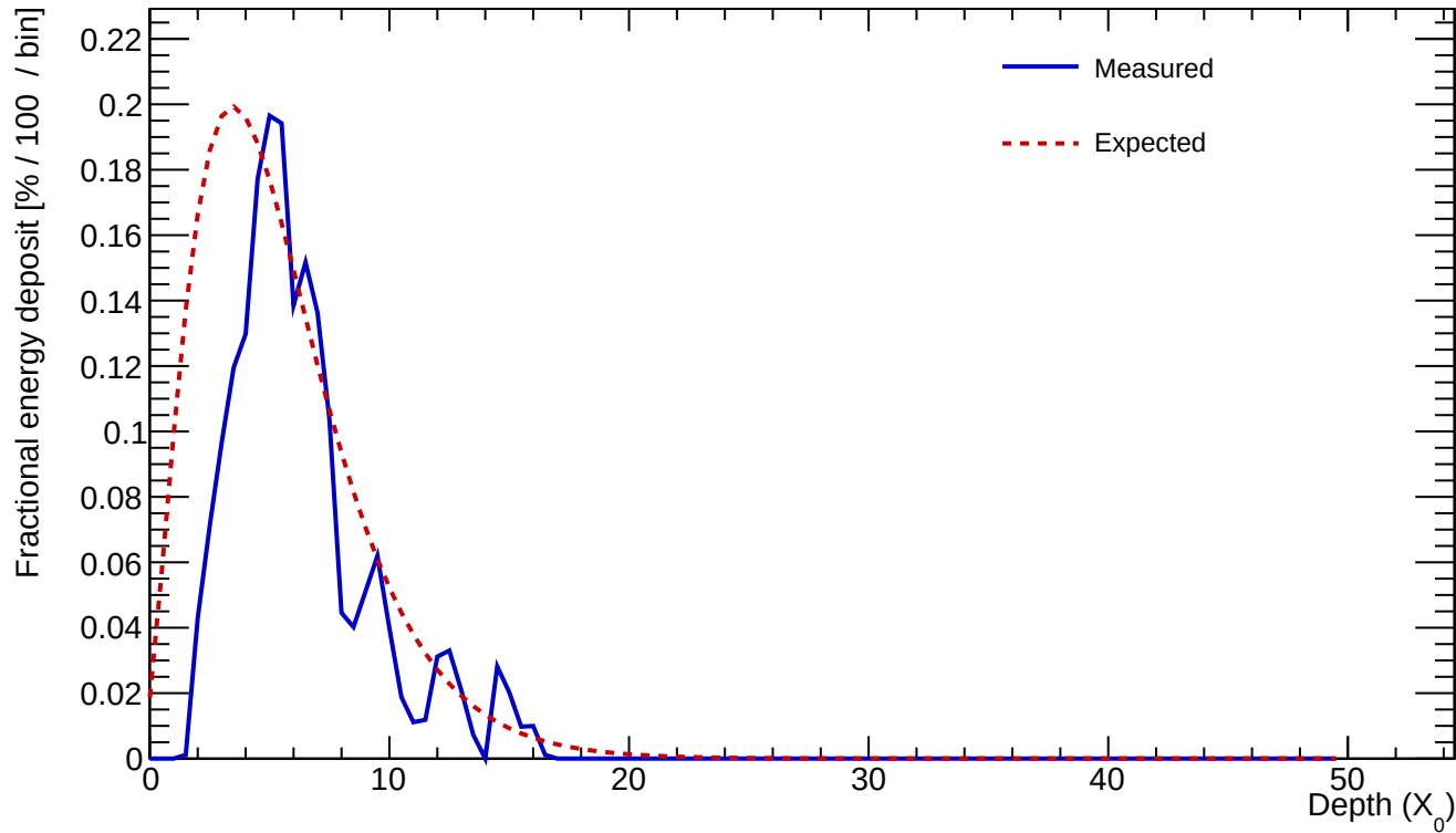
Cluster 307 E=2.550 GeV profileStart=1.50 X_0 \chi=0.2688
