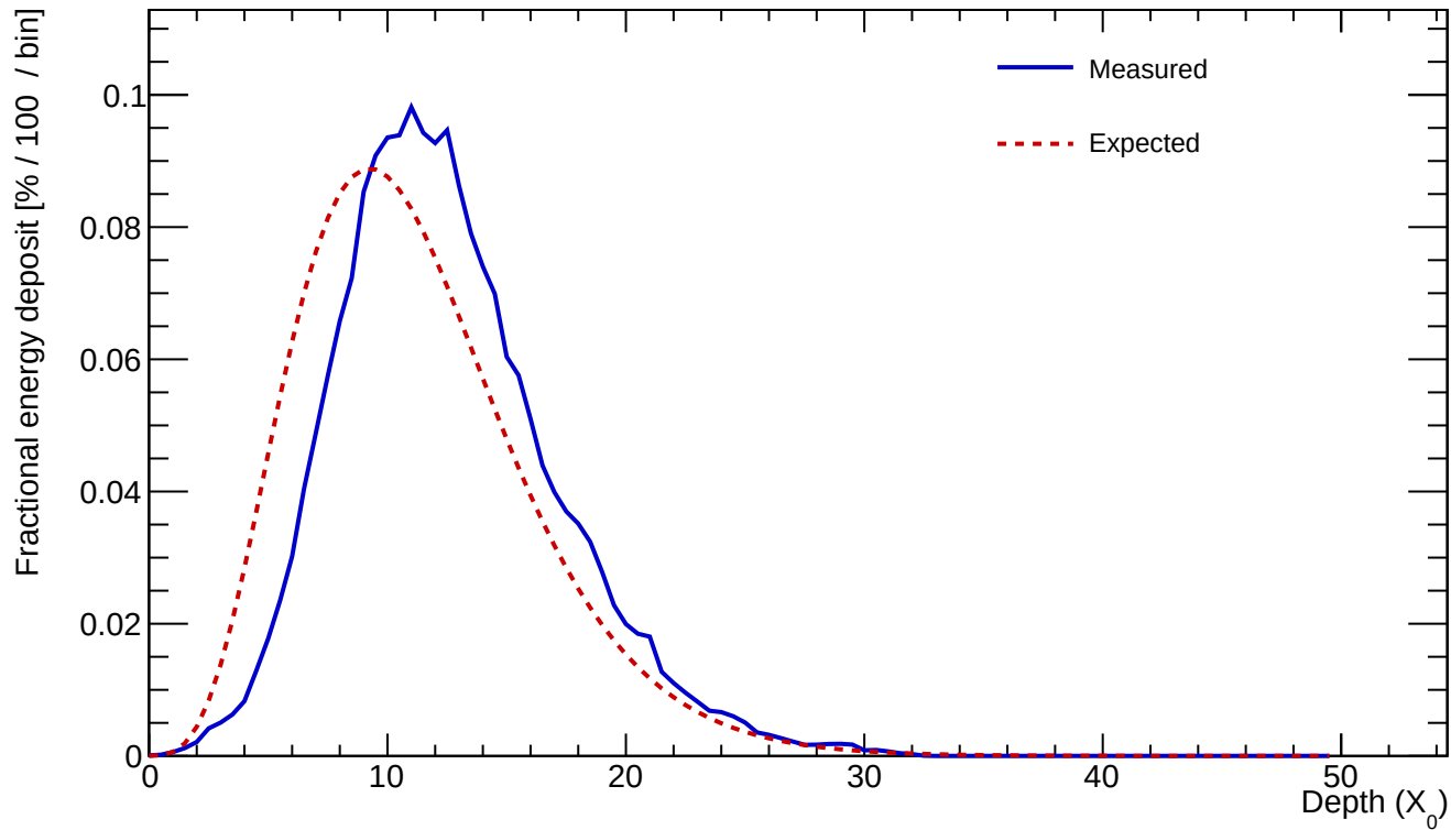
Cluster 138 E=823.202 GeV profileStart=1.50 X_0 \chi=0.0837
