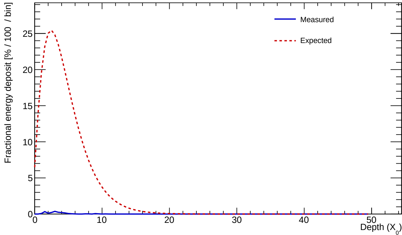
Cluster 356 E=0.901 GeV profileStart=0.50 X_0 \chi=0.6347
