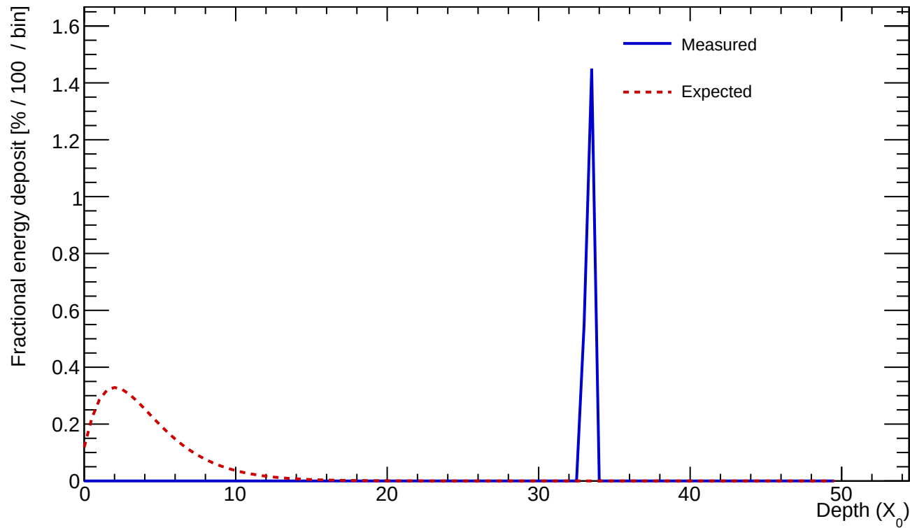
Cluster 41 E=0.597 GeV profileStart=33.00 X_0 \chi=0.0180
