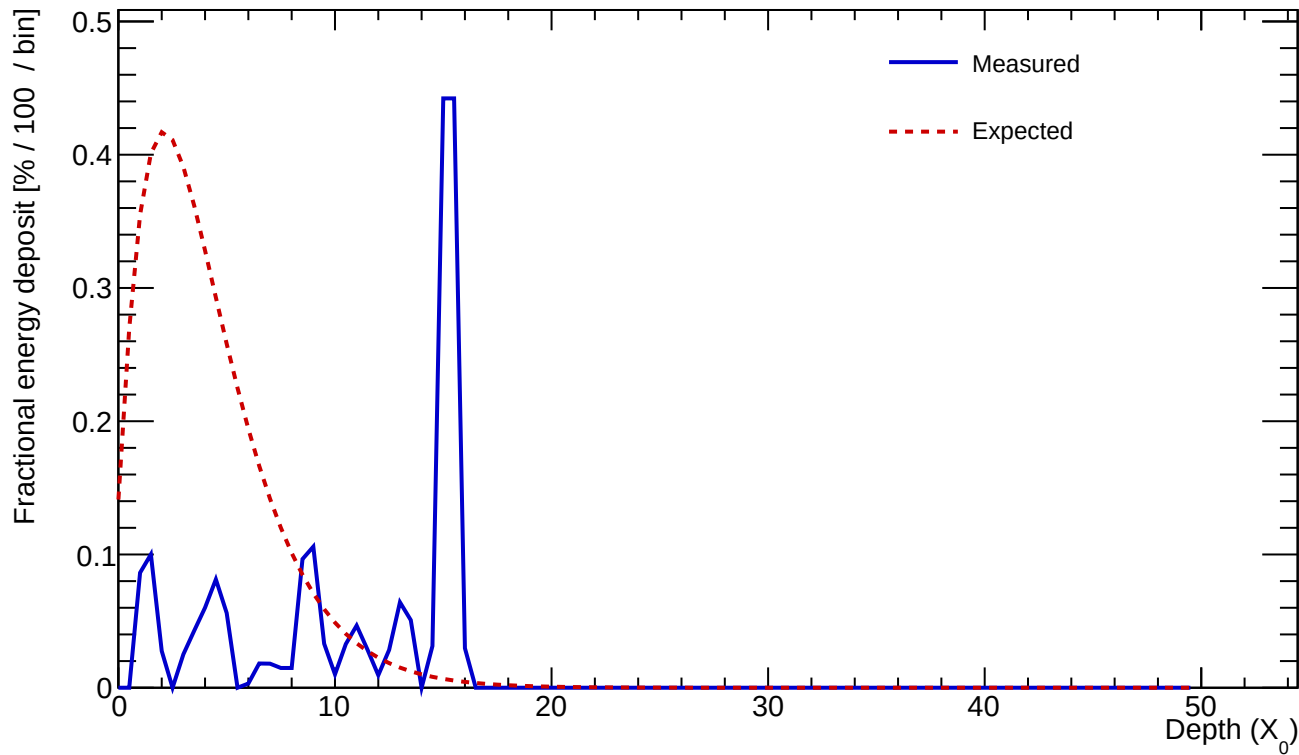
Cluster 58 E=0.645 GeV profileStart=14.50 X_0 \chi=0.8585
