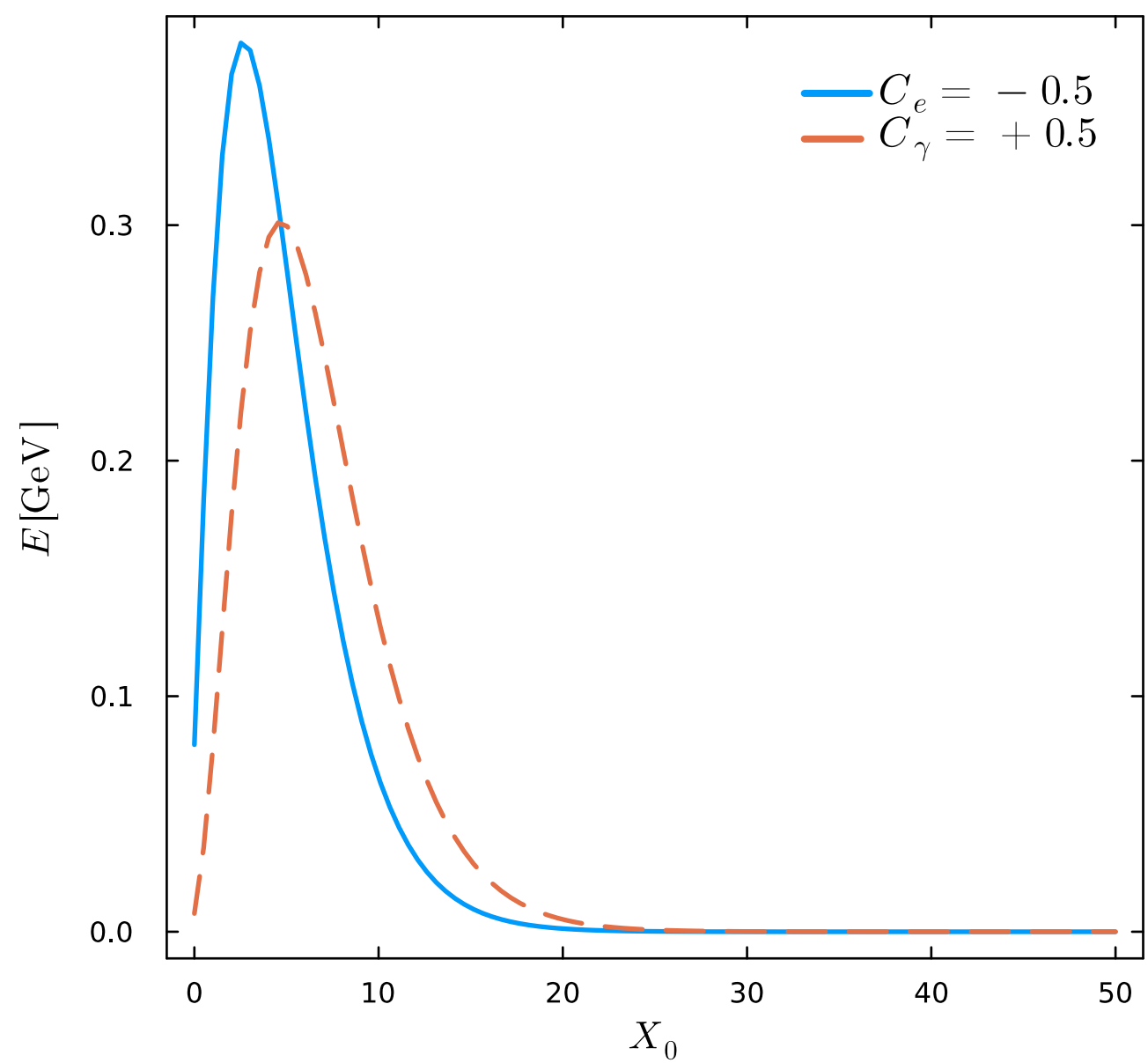
E = 100.0 GeV
