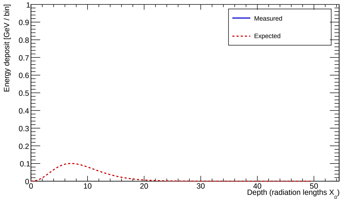
Cluster 1 E=96.120 GeV profileStart=3.00 X_0 \chi=0.2891
