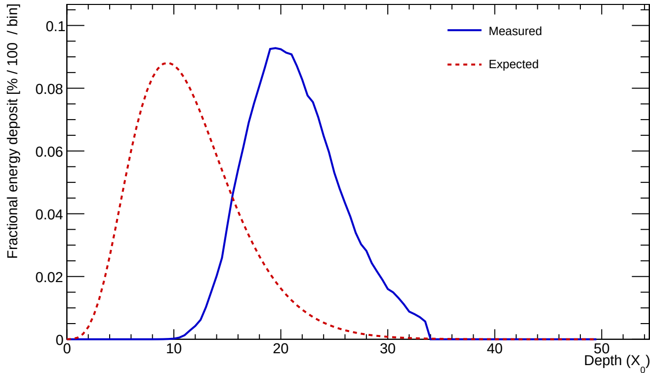
Cluster 63 E=972.940 GeV profileStart=10.50 X_0 \chi=0.0418
