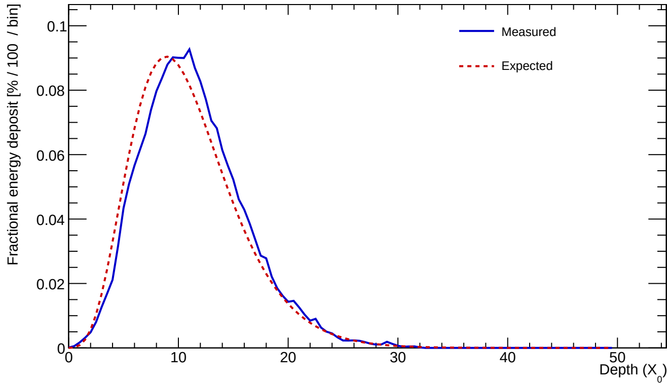
Cluster 232 E=583.510 GeV profileStart=0.50 X_0 \chi=0.0601
