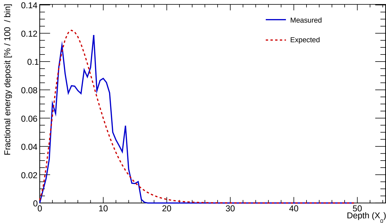
Cluster 22 E=12.246 GeV profileStart=0.50 X_0 \chi=0.2511
