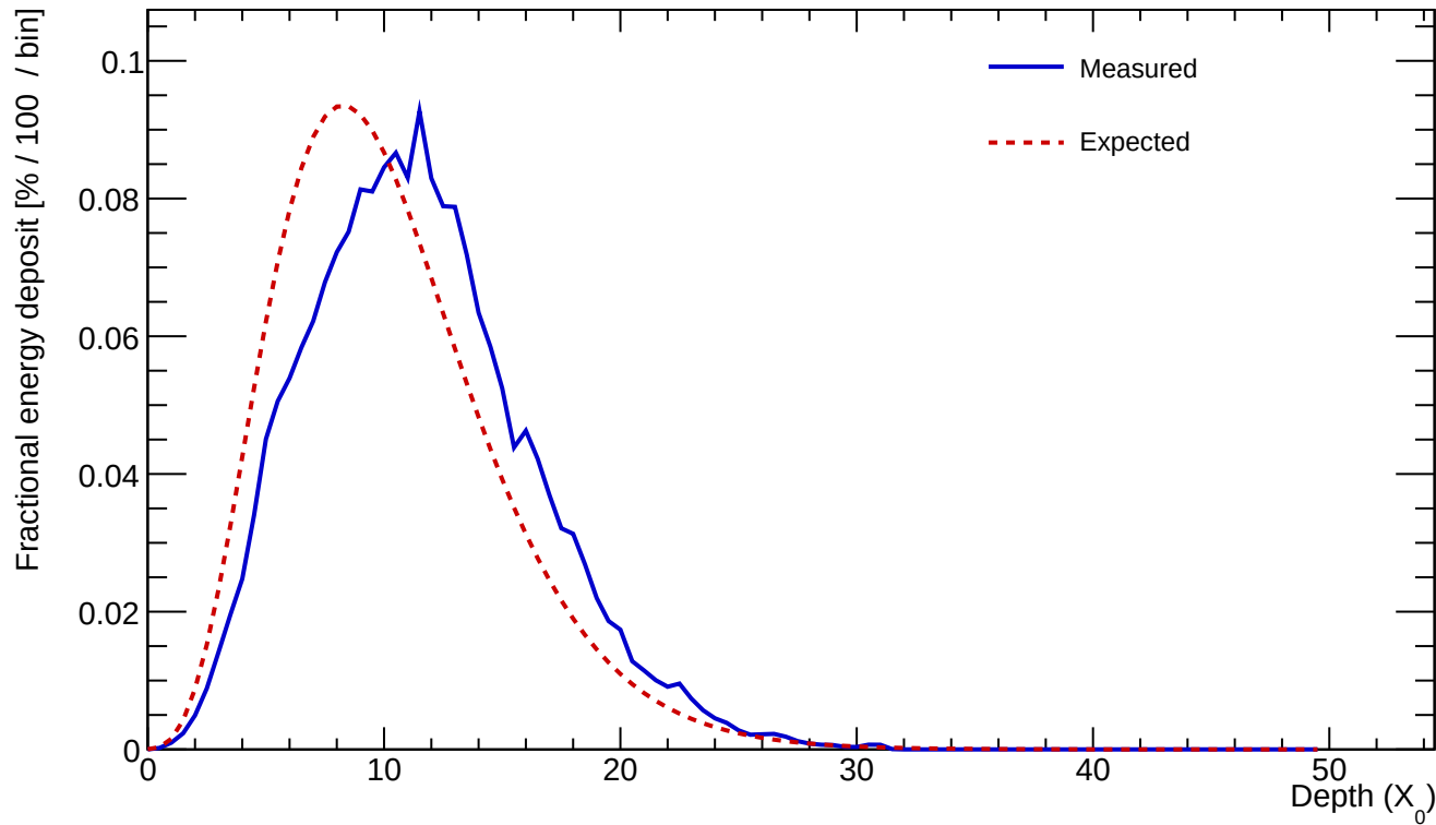
Cluster 85 E=310.512 GeV profileStart=1.50 X_0 \chi=0.1108
