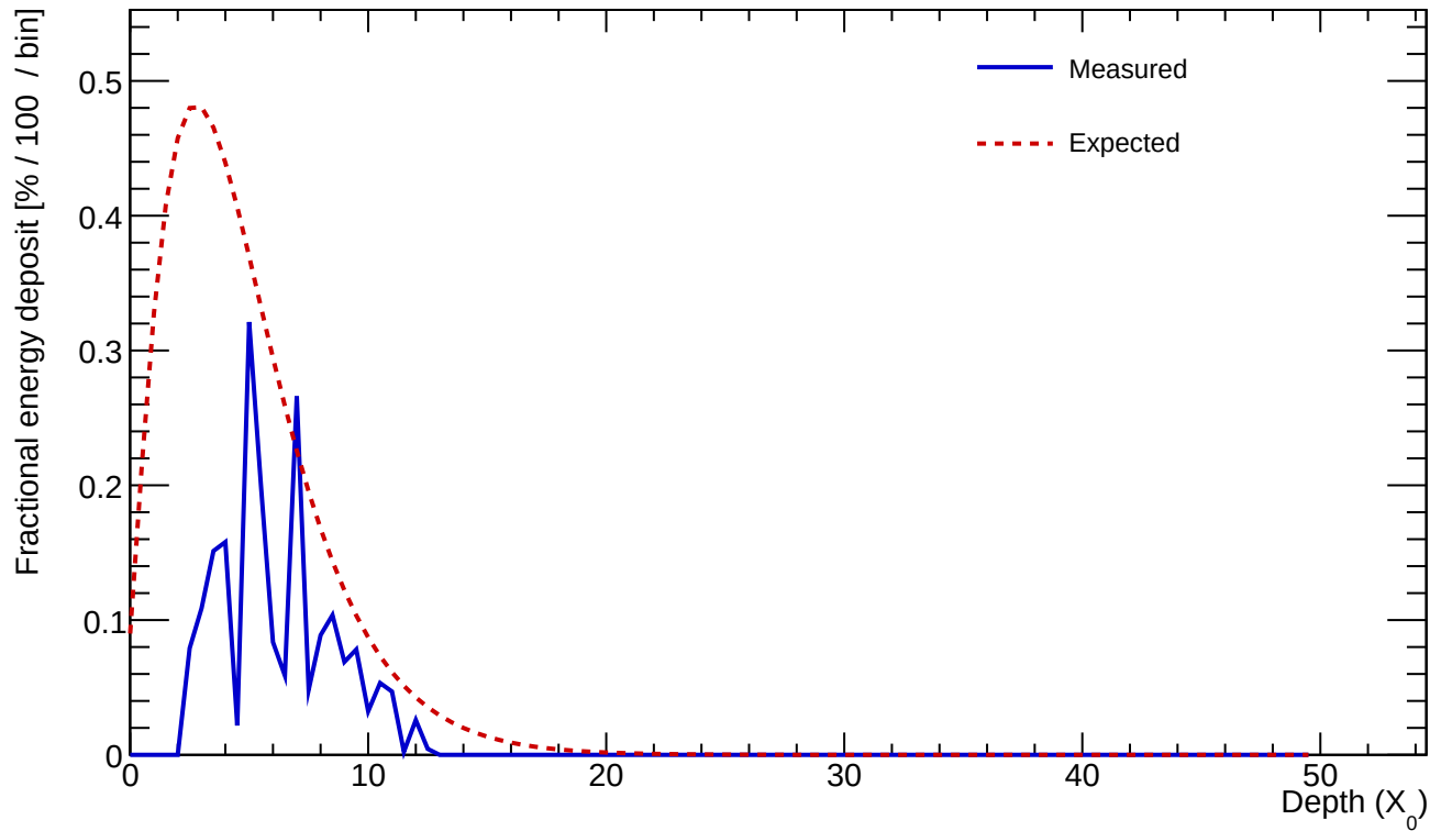
Cluster 124 E=1.269 GeV profileStart=2.00 X_0 \chi=0.4409
