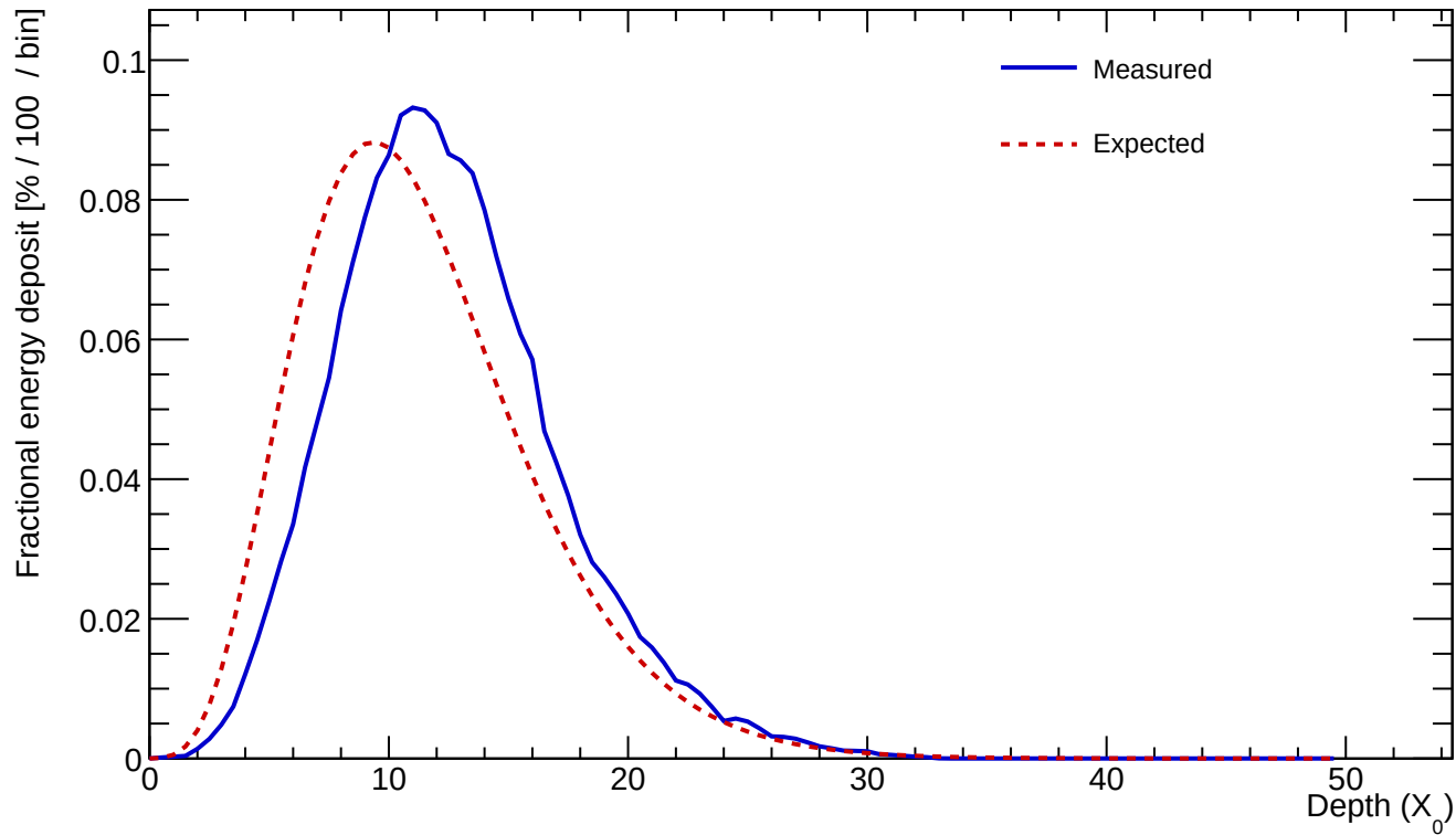
Cluster 144 E=936.203 GeV profileStart=1.50 X_0 \chi=0.0798
