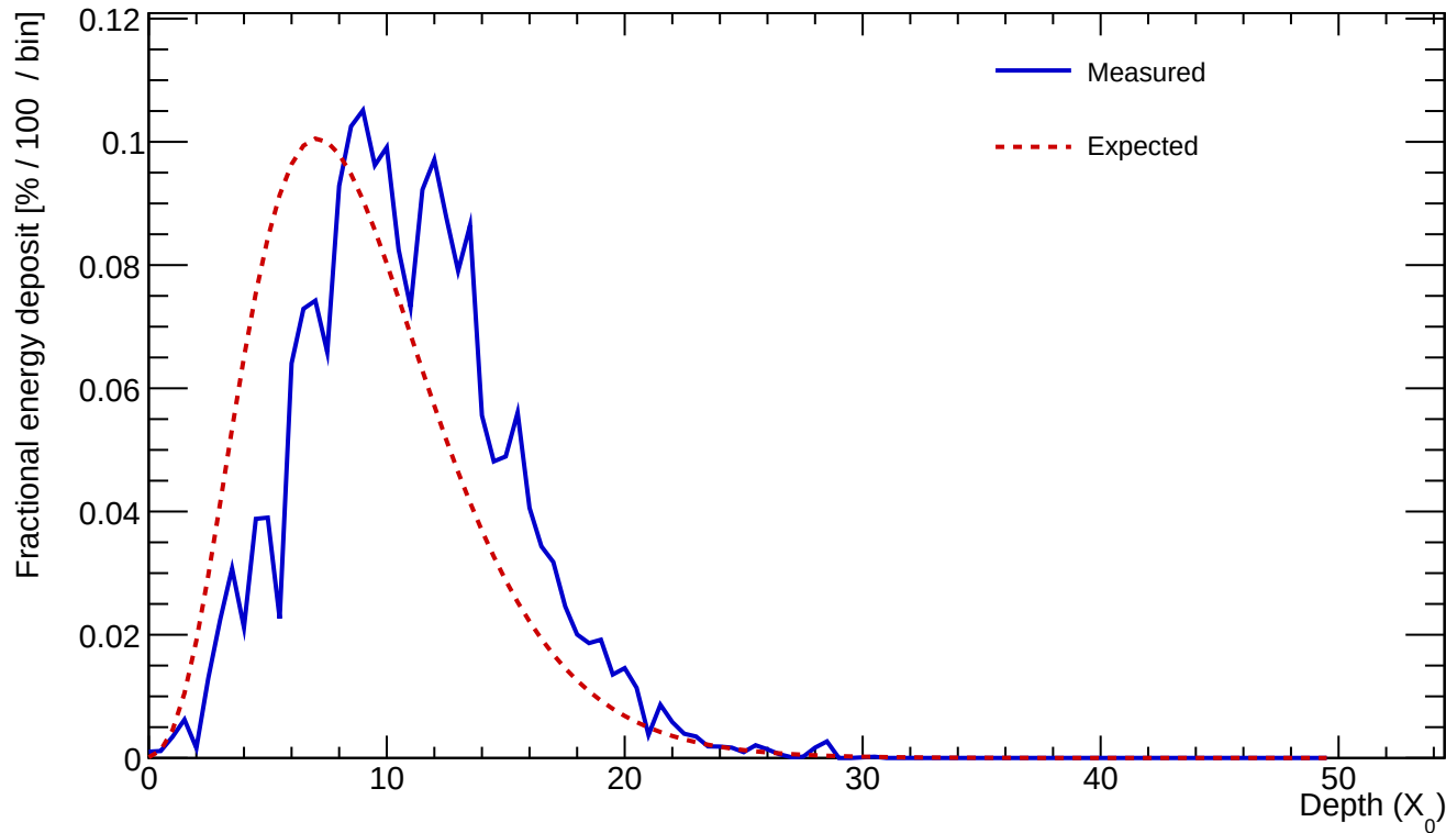
Cluster 171 E=94.835 GeV profileStart=2.00 X_0 \chi=0.1618
