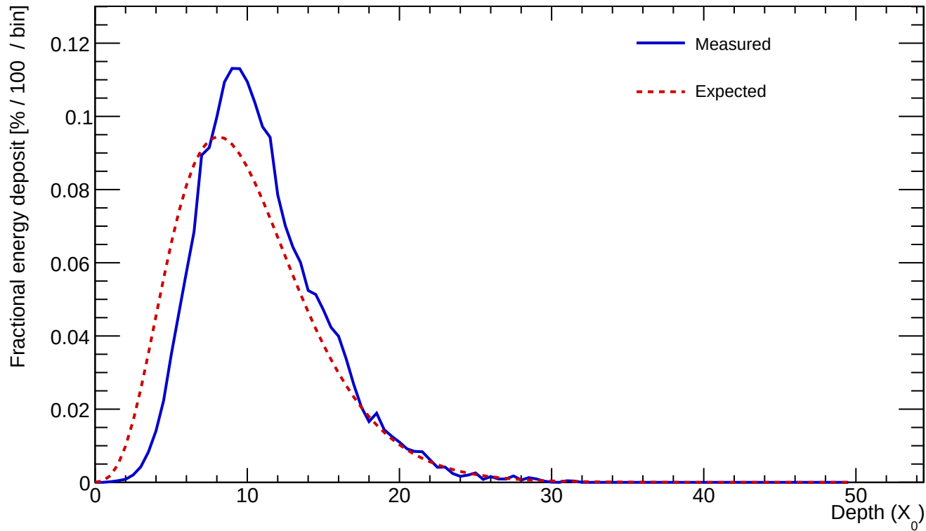
Cluster 64 E=260.500 GeV profileStart=1.00 X_0 \chi=0.1359
