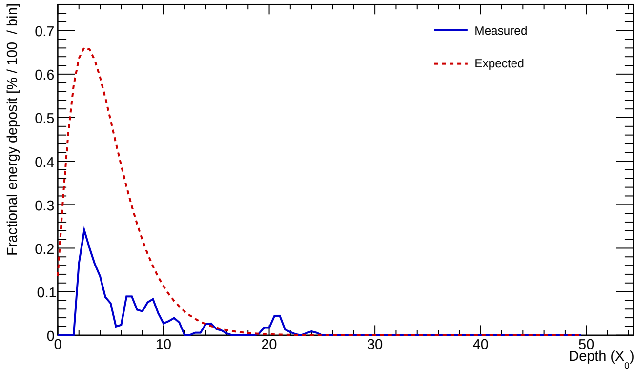
Cluster 218 E=1.145 GeV profileStart=1.00 X_0 \chi=0.5312
