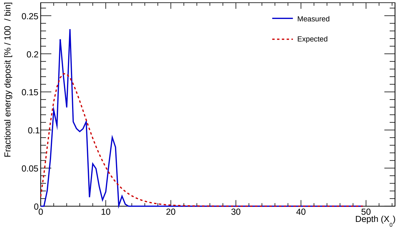
Cluster 231 E=3.238 GeV profileStart=0.50 X_0 \chi=0.3790
