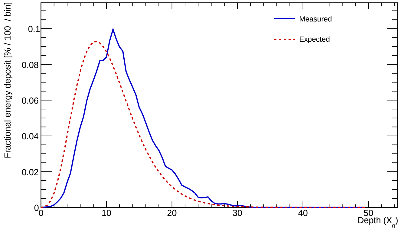
Cluster 57 E=356.453 GeV profileStart=2.00 X_0 \chi=0.0701
