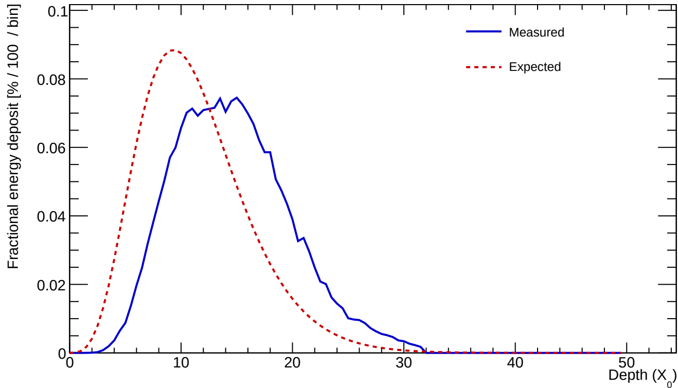
Cluster 174 E=900.870 GeV profileStart=3.50 X_0 \chi=0.1375
