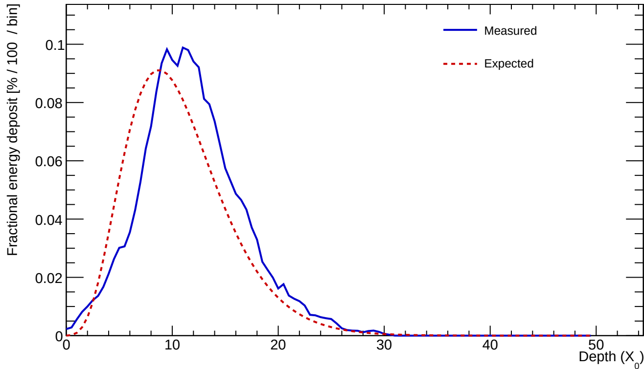
Cluster 165 E=499.187 GeV profileStart=1.50 X_0 \chi=0.1068
