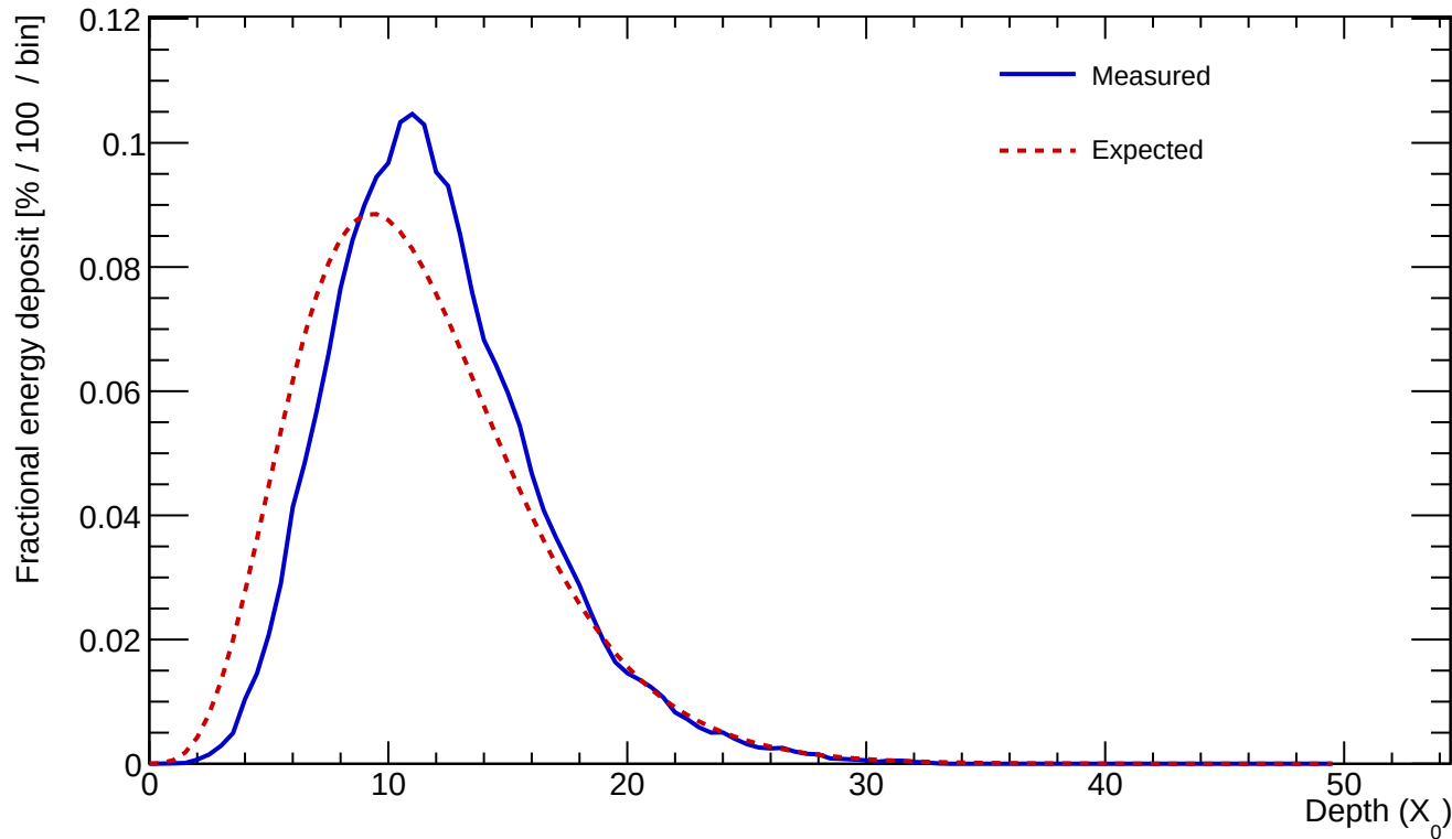
Cluster 13 E=874.176 GeV profileStart=1.00 X_0 \chi=0.1213
