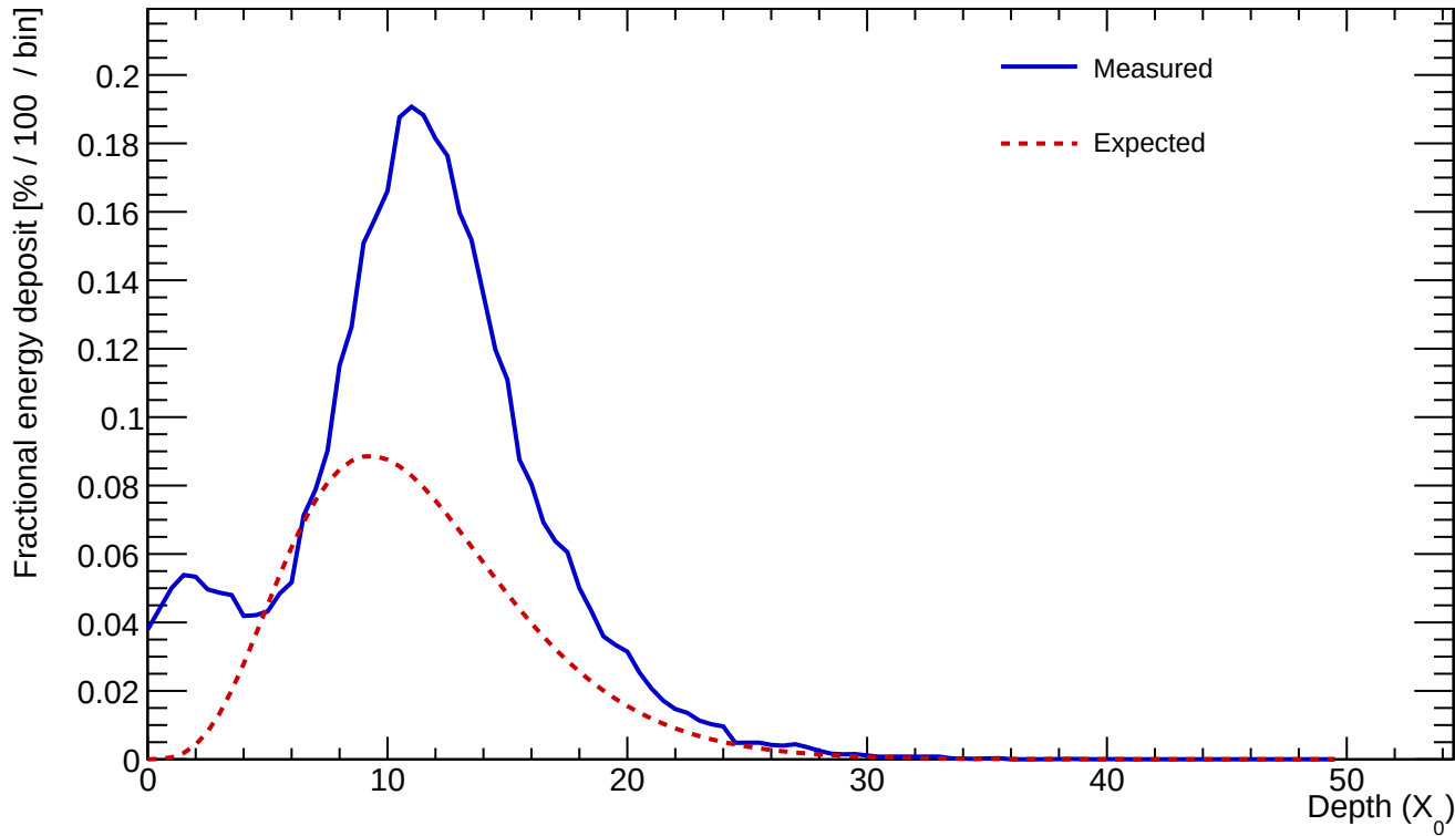
Cluster 6 E=860.846 GeV profileStart=1.00 X_0 \chi=0.2590
