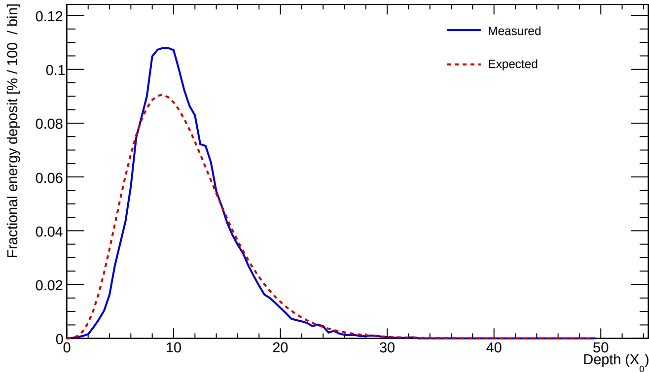
Cluster 18 E=570.082 GeV profileStart=0.50 X_0 \chi=0.1467
