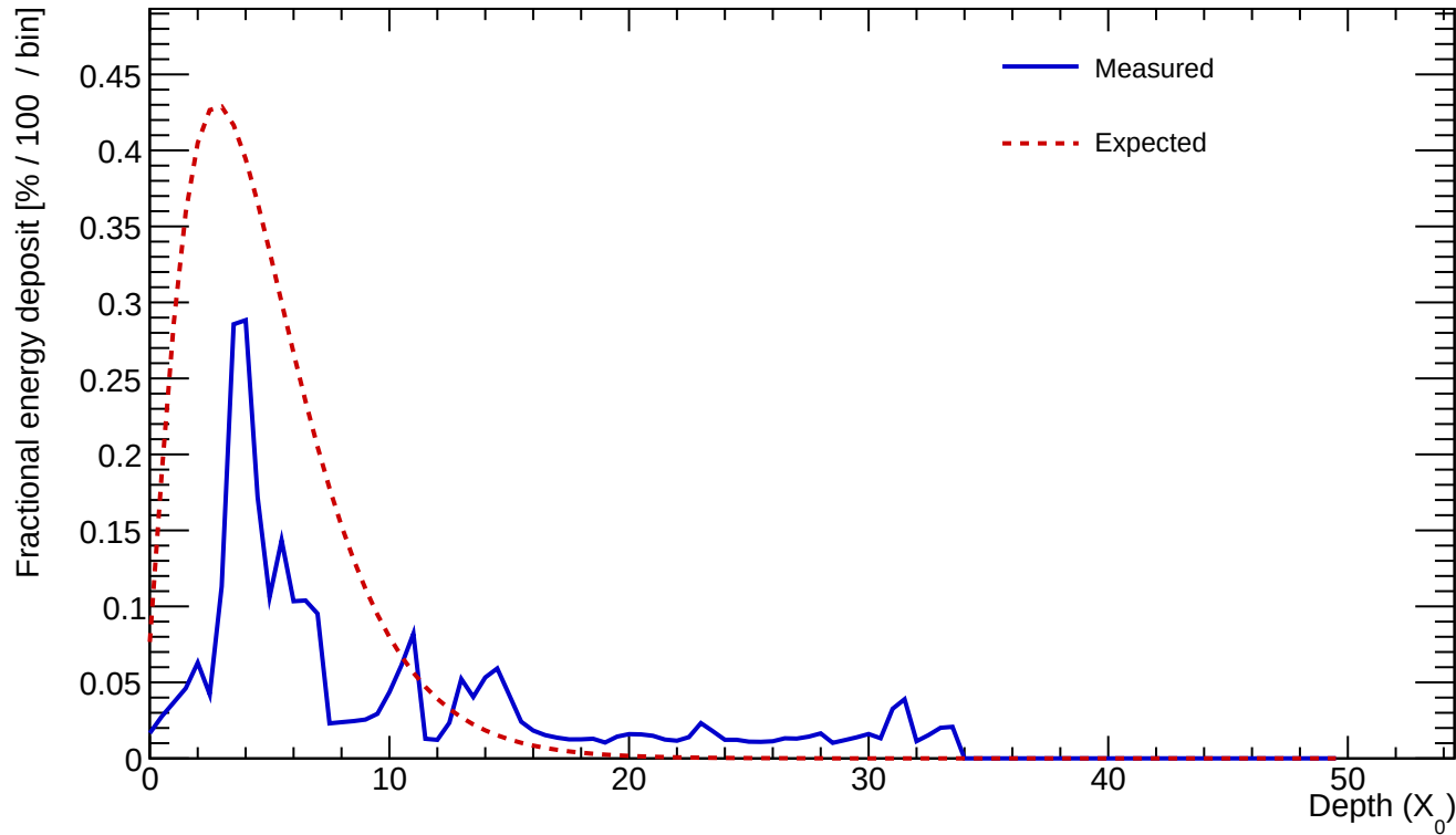
Cluster 233 E=1.332 GeV profileStart=1.00 X_0 \chi=0.7662
