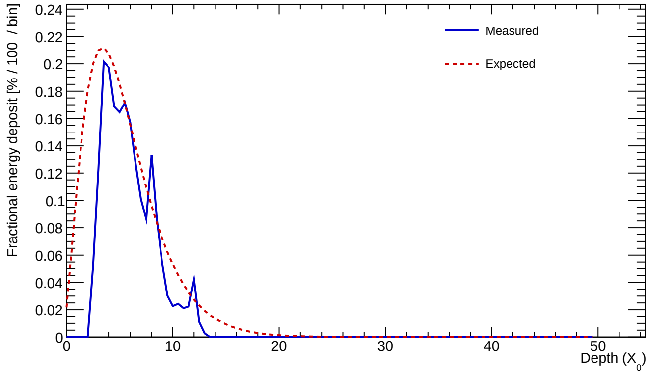
Cluster 121 E=2.333 GeV profileStart=1.50 X_0 \chi=0.3100
