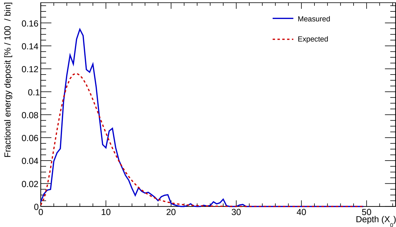
Cluster 226 E=18.089 GeV profileStart=0.50 X_0 \chi=0.1848
