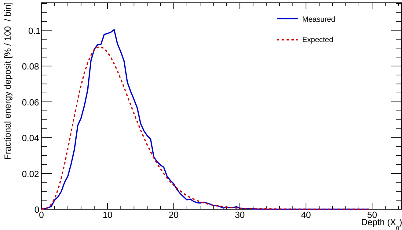
Cluster 92 E=546.355 GeV profileStart=1.00 X_0 \chi=0.1012
