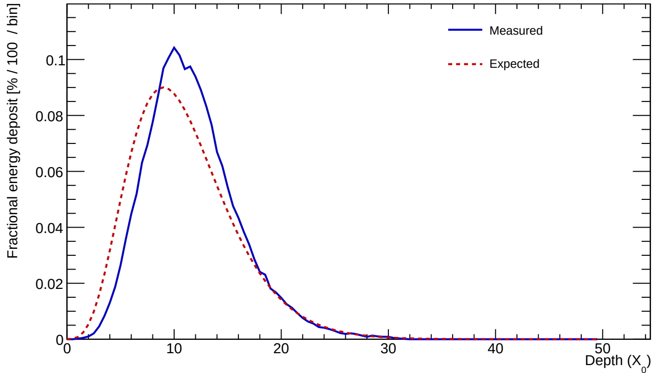
Cluster 28 E=636.145 GeV profileStart=1.00 X_0 \chi=0.1145
