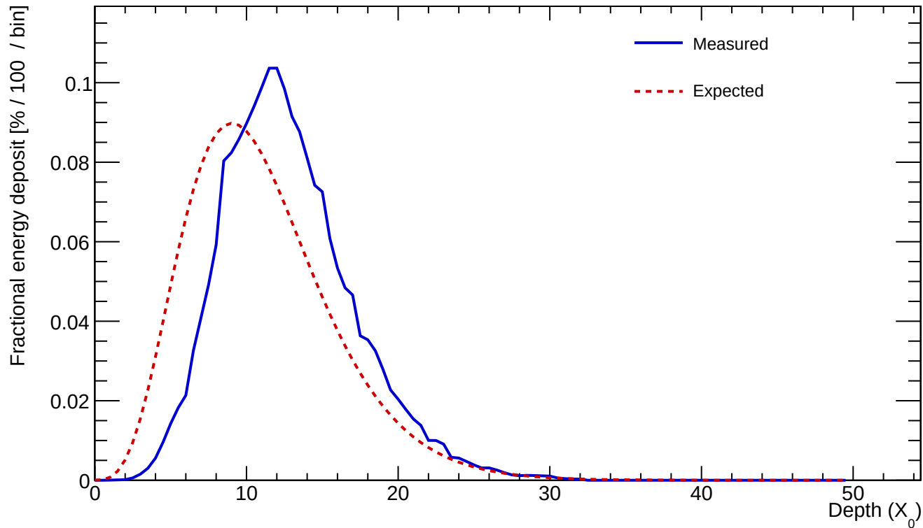
Cluster 67 E=669.163 GeV profileStart=2.00 X_0 \chi=0.1124
