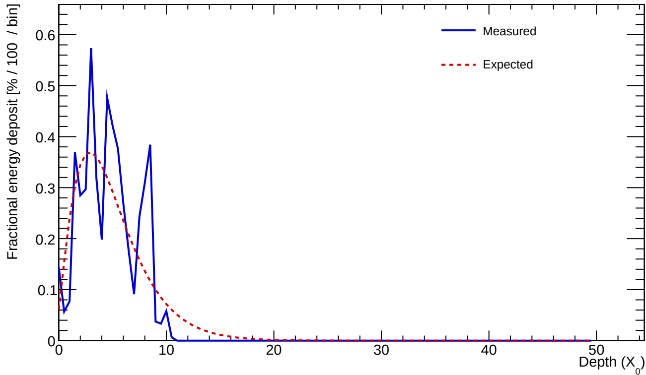
Cluster 39 E=1.436 GeV profileStart=0.50 X_0 \chi=0.3815
