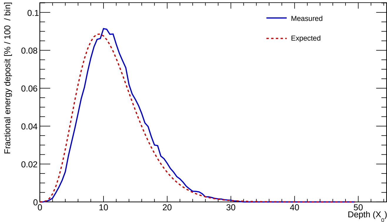
Cluster 32 E=866.781 GeV profileStart=1.00 X_0 \chi=0.0404
