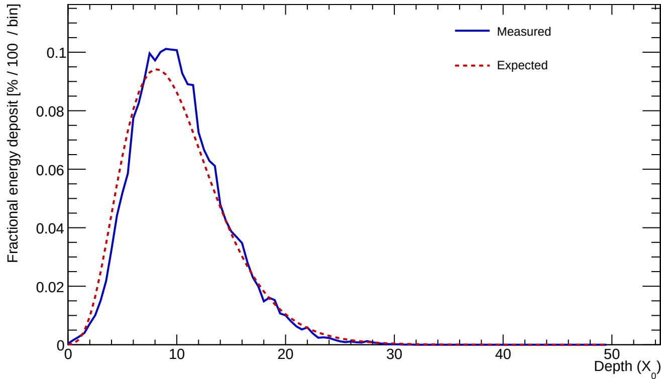
Cluster 83 E=272.099 GeV profileStart=0.50 X_0 \chi=0.0843
