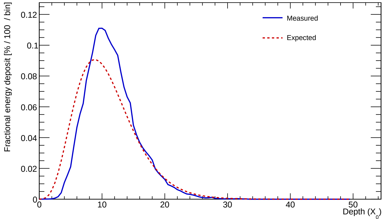
Cluster 54 E=554.164 GeV profileStart=1.00 X_0 \chi=0.1792
