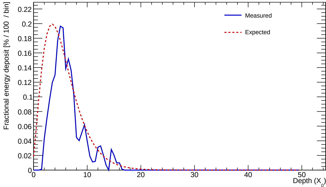
Cluster 223 E=2.550 GeV profileStart=1.50 X_0 \chi=0.2688
