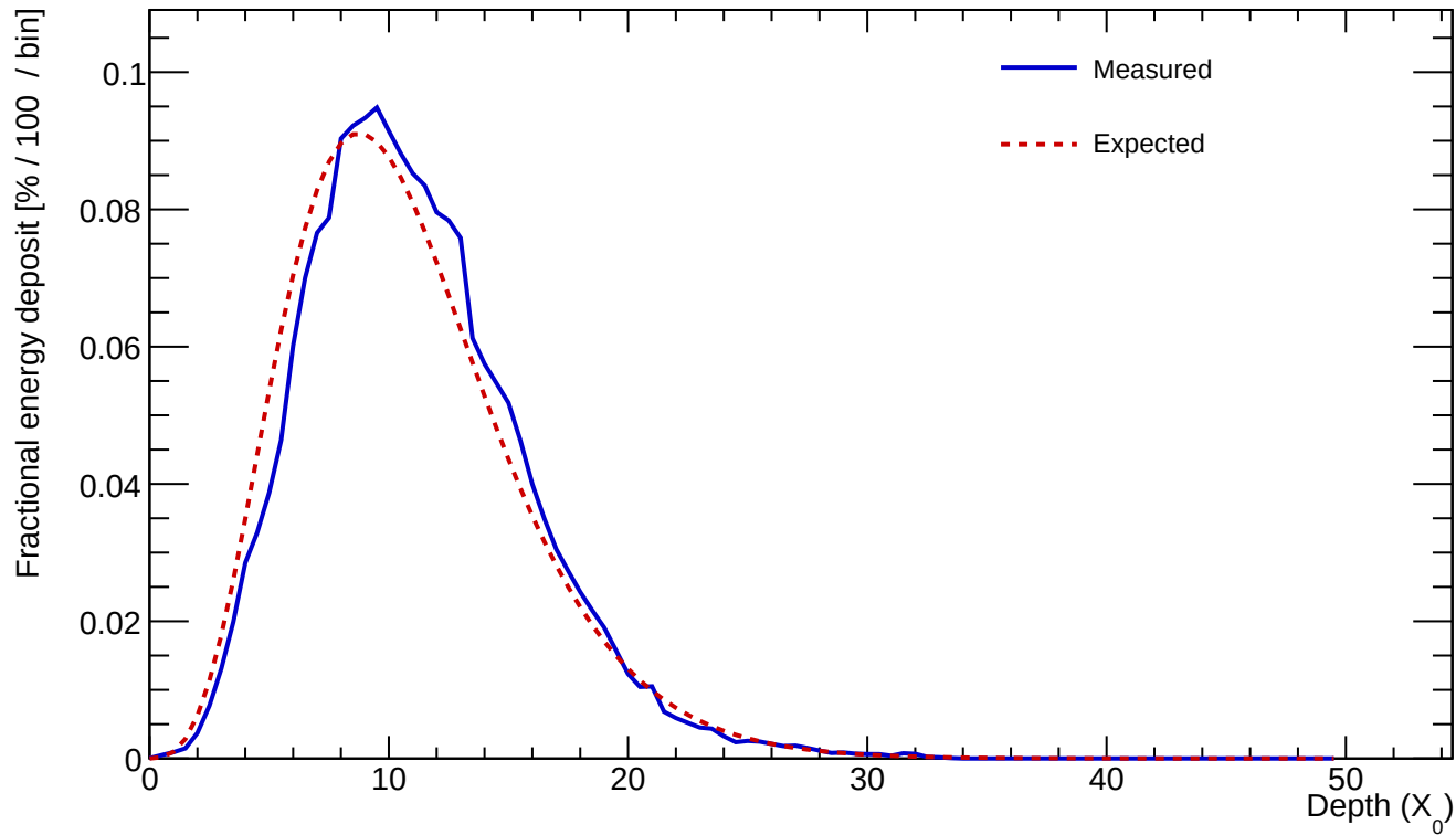
Cluster 156 E=506.673 GeV profileStart=0.50 X_0 \chi=0.0528
