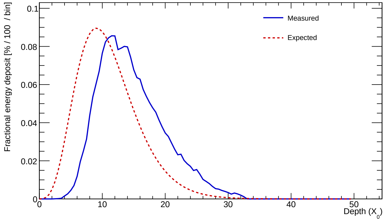
Cluster 51 E=703.234 GeV profileStart=3.50 X_0 \chi=0.1037
