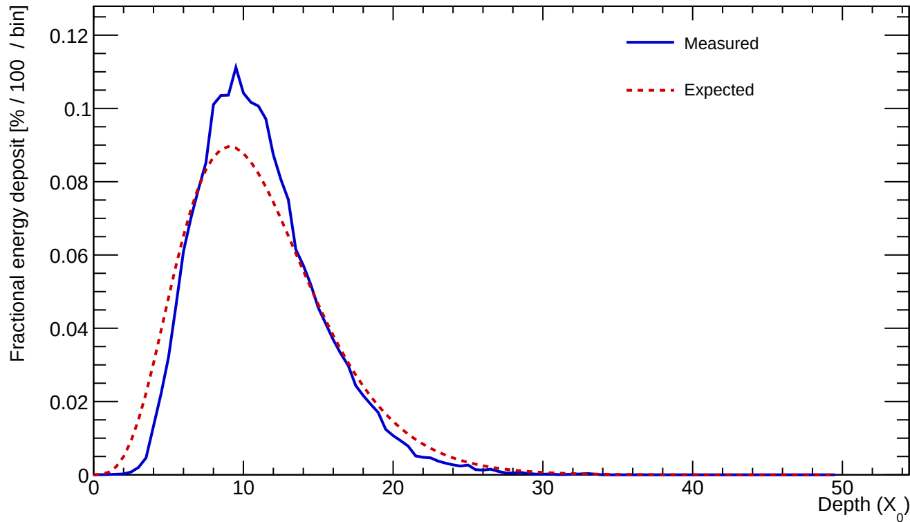
Cluster 55 E=699.841 GeV profileStart=0.50 X_0 \chi=0.1710
