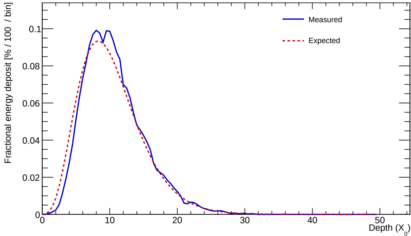
Cluster 74 E=318.743 GeV profileStart=0.50 X_0 \chi=0.0685
