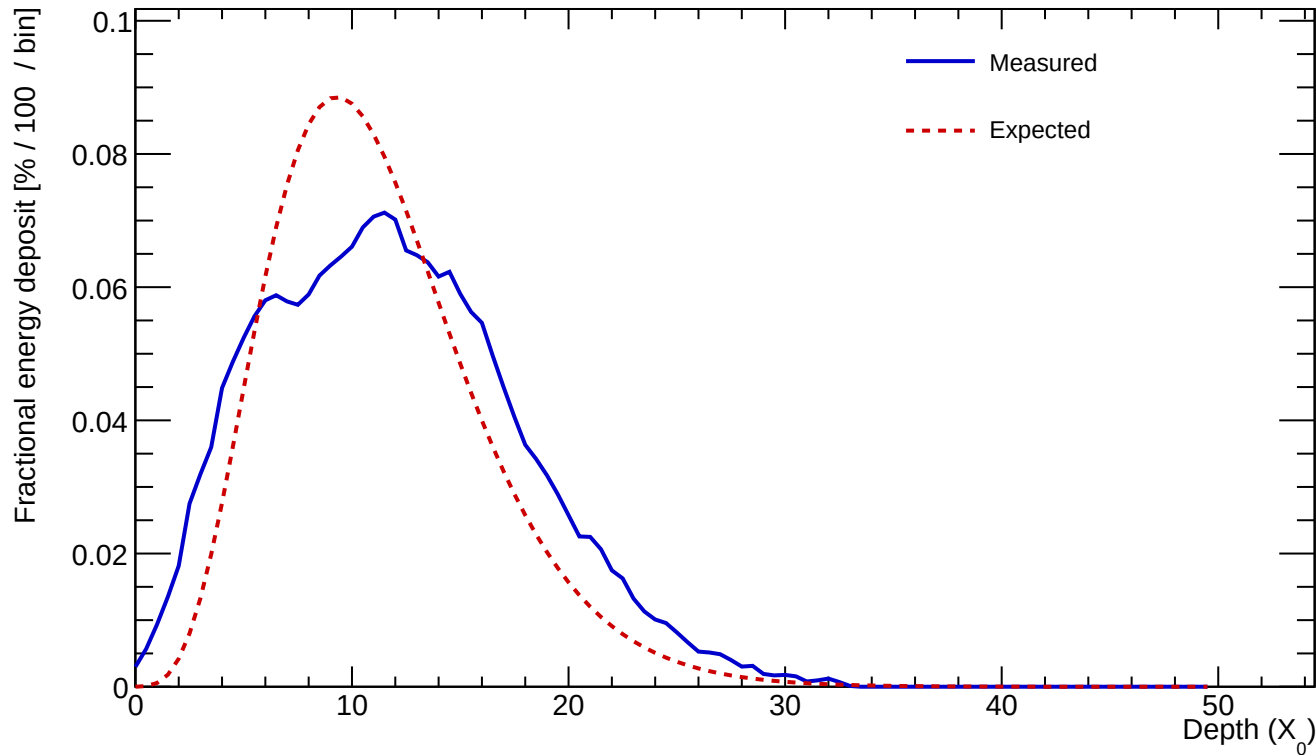
Cluster 52 E=879.891 GeV profileStart=0.50 X_0 \chi=0.2943
