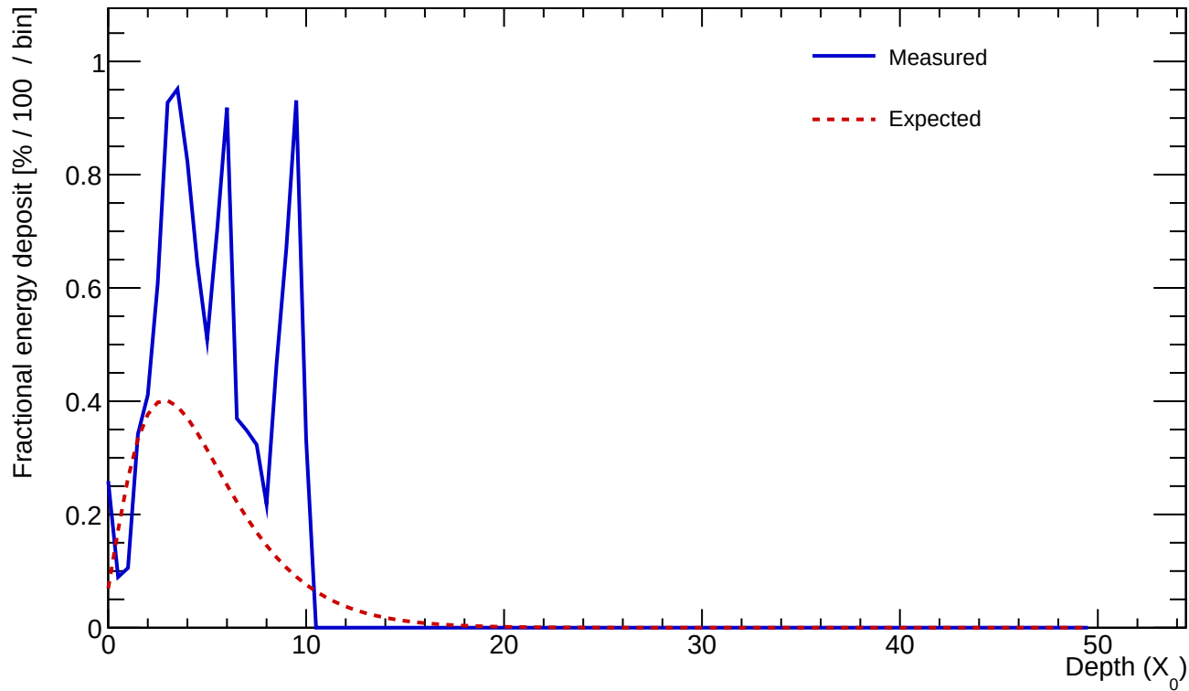
Cluster 267 E=1.375 GeV profileStart=1.00 X_0 \chi=0.3122
