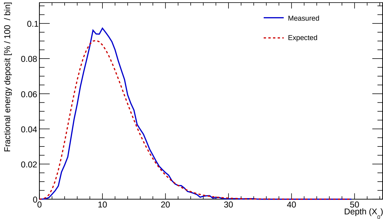
Cluster 60 E=593.123 GeV profileStart=0.50 X_0 \chi=0.0722
