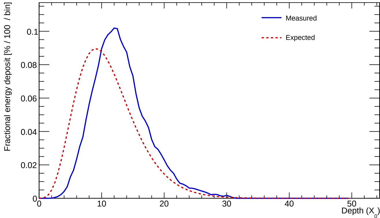
Cluster 31 E=702.385 GeV profileStart=2.50 X_0 \chi=0.1078
