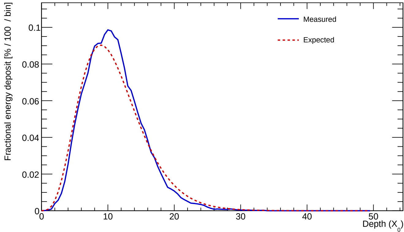
Cluster 277 E=599.181 GeV profileStart=0.50 X_0 \chi=0.0958
