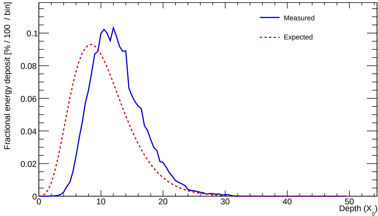
Cluster 88 E=344.077 GeV profileStart=2.50 X_0 \chi=0.0958
