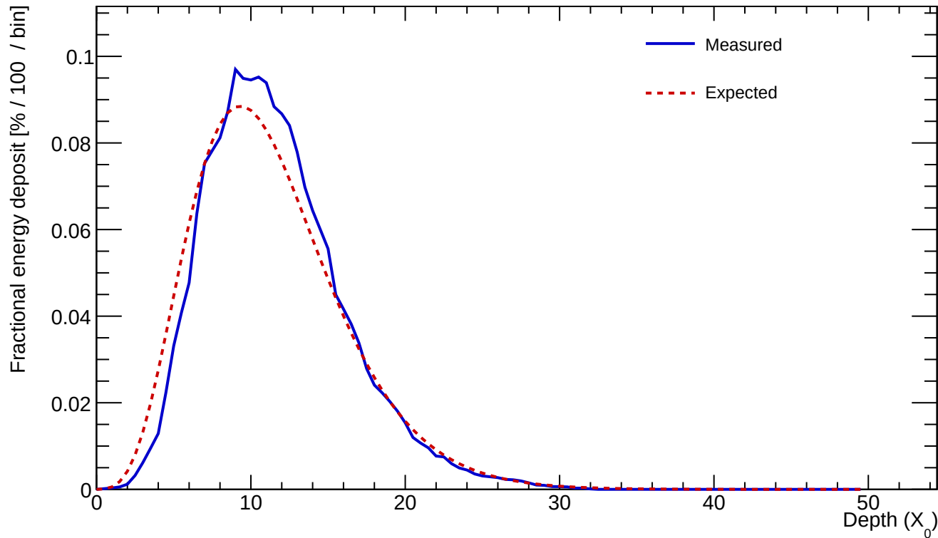
Cluster 36 E=888.224 GeV profileStart=0.50 X_0 \chi=0.0894
