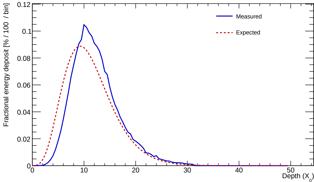
Cluster 58 E=830.333 GeV profileStart=1.50 X_0 \chi=0.1048
