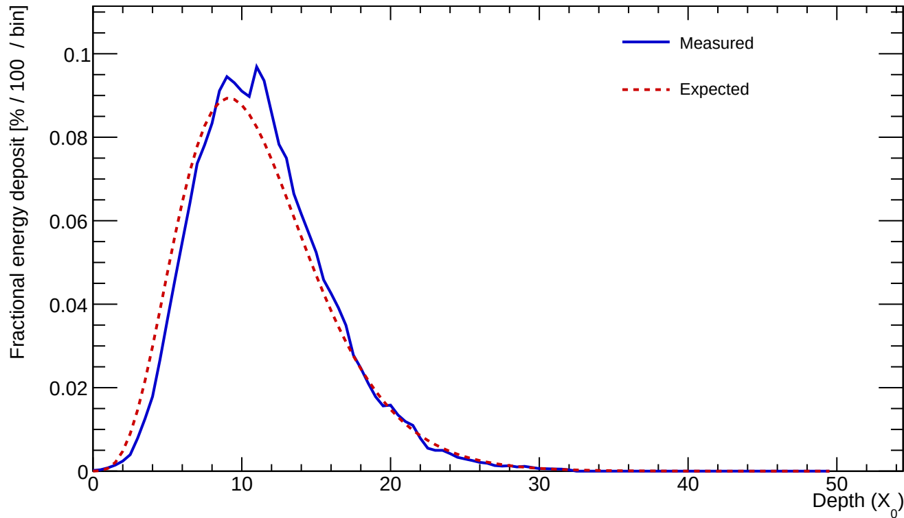
Cluster 11 E=735.772 GeV profileStart=0.50 X_0 \chi=0.0591
