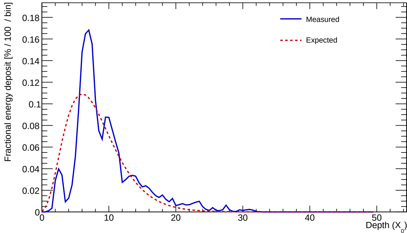
Cluster 117 E=32.861 GeV profileStart=1.00 X_0 \chi=0.3310
