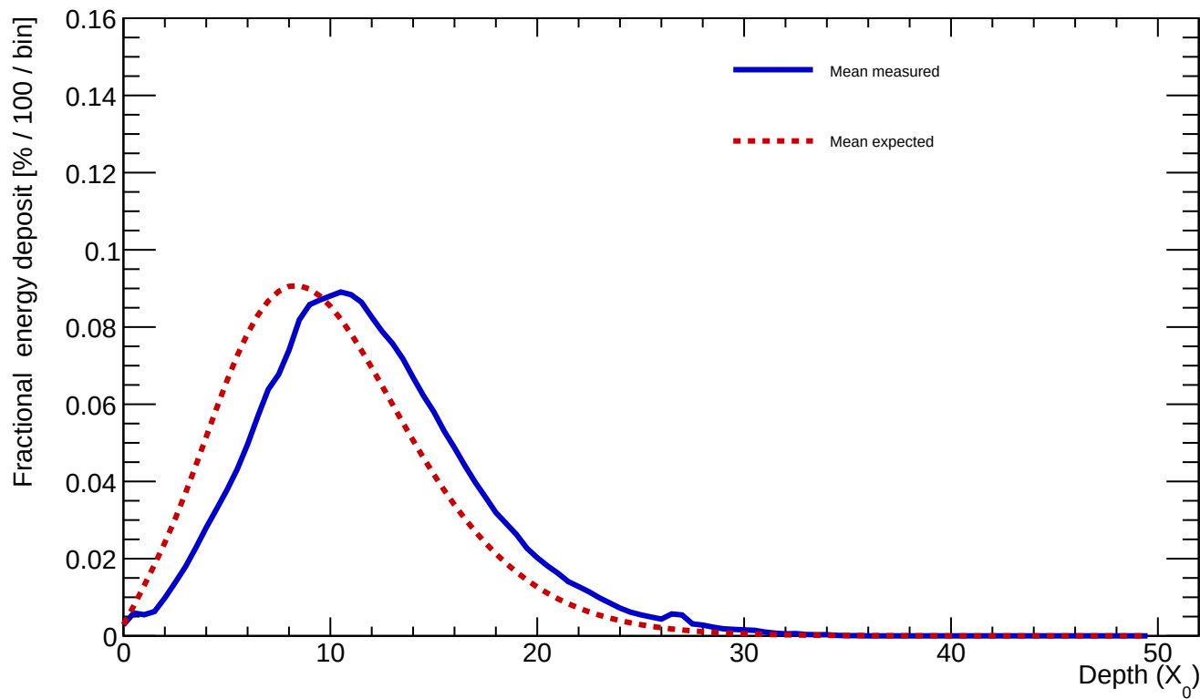
Average longitudinal profile (297 clusters): measured vs expected
