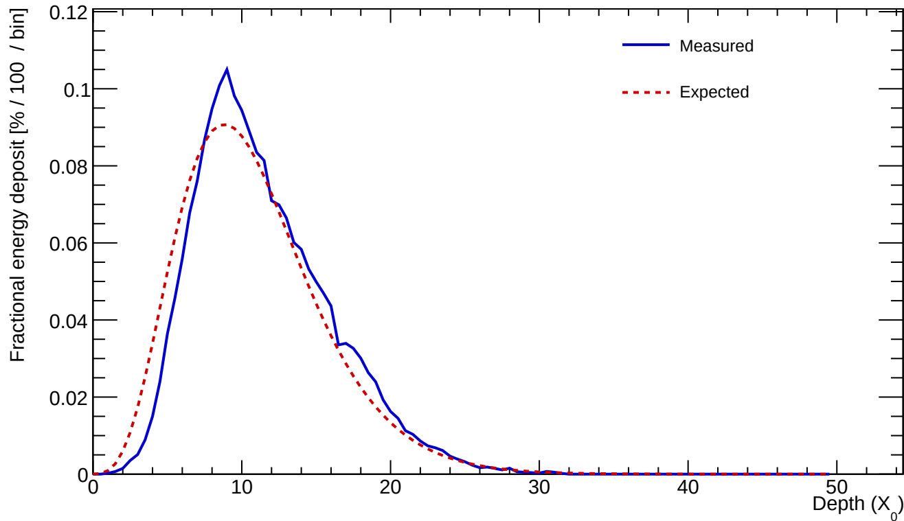
Cluster 146 E=543.545 GeV profileStart=0.50 X_0 \chi=0.0836
