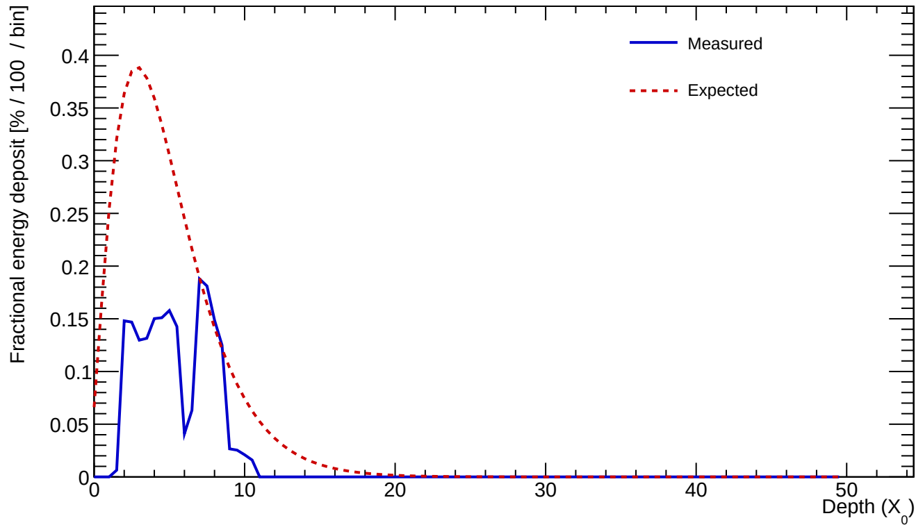
Cluster 217 E=1.398 GeV profileStart=1.50 X_0 \chi=0.3604
