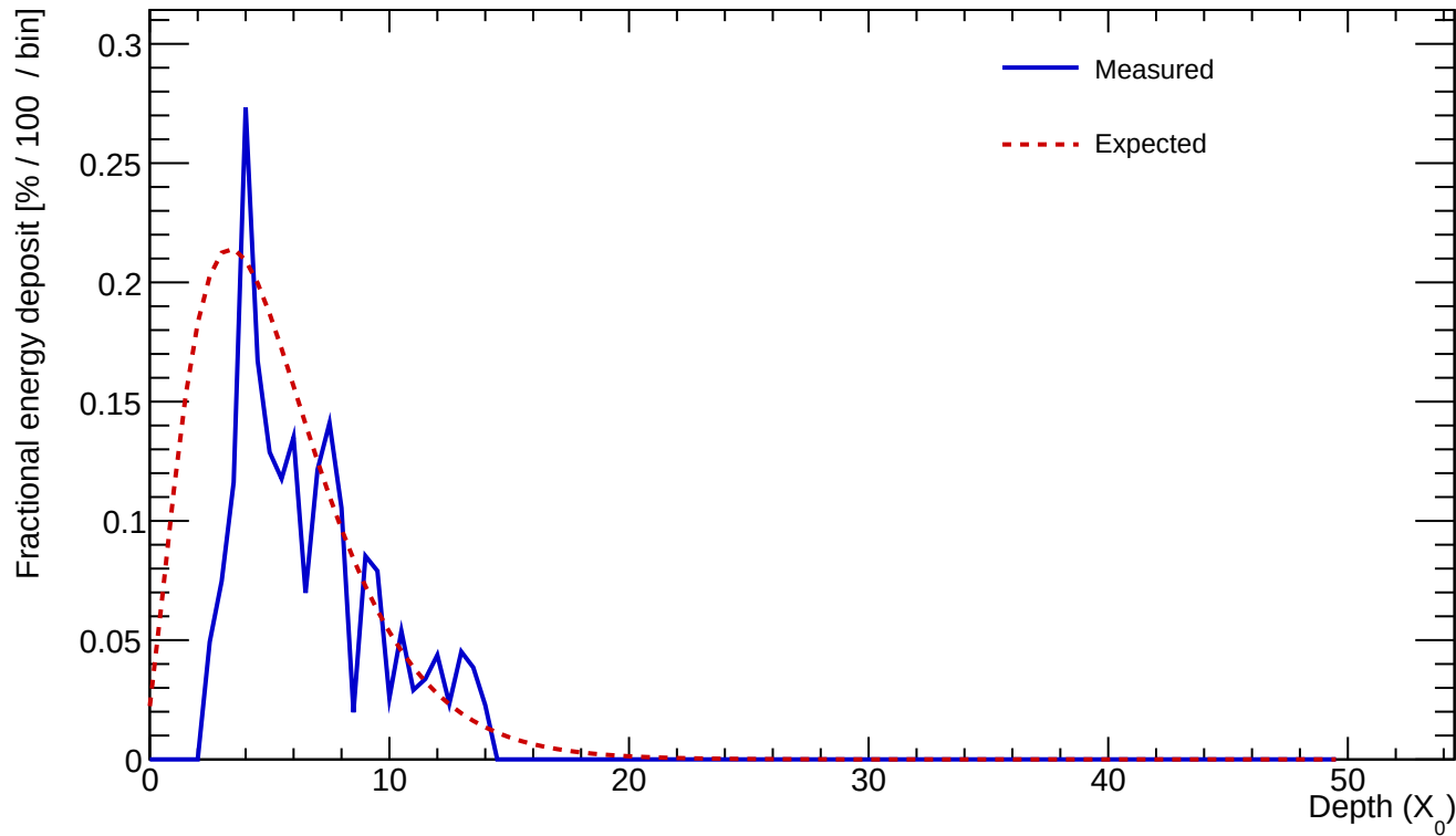
Cluster 122 E=2.299 GeV profileStart=2.00 X_0 \chi=0.2776
