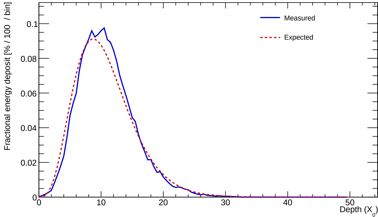
Cluster 143 E=495.391 GeV profileStart=0.50 X_0 \chi=0.0752
