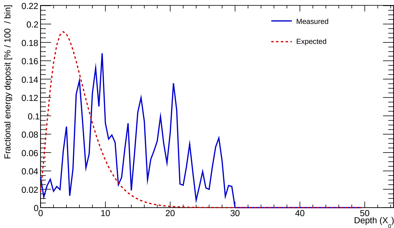
Cluster 94 E=2.715 GeV profileStart=4.50 X_0 \chi=0.8919
