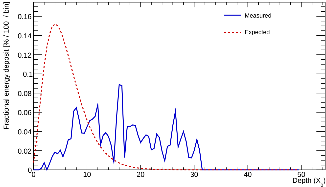
Cluster 198 E=4.565 GeV profileStart=9.00 X_0 \chi=0.9313
