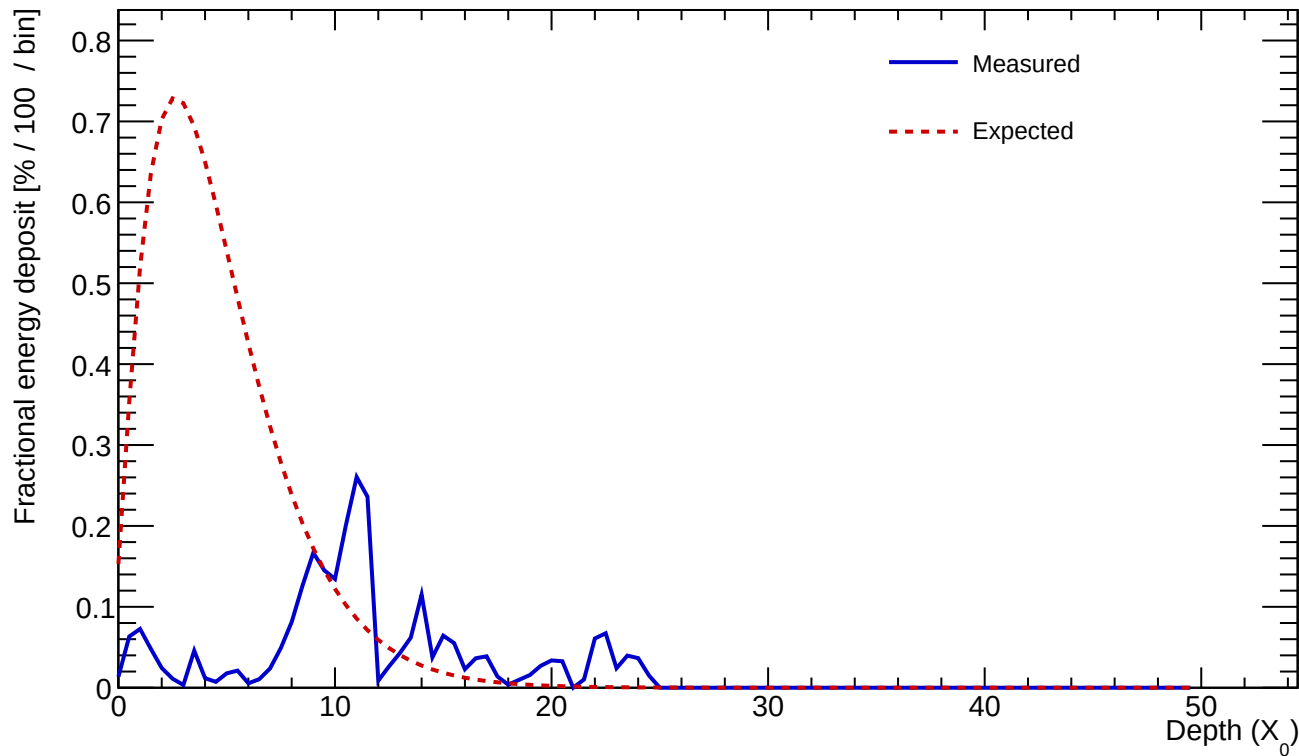
Cluster 8 E=1.118 GeV profileStart=7.50 X_0 \chi=0.5850
