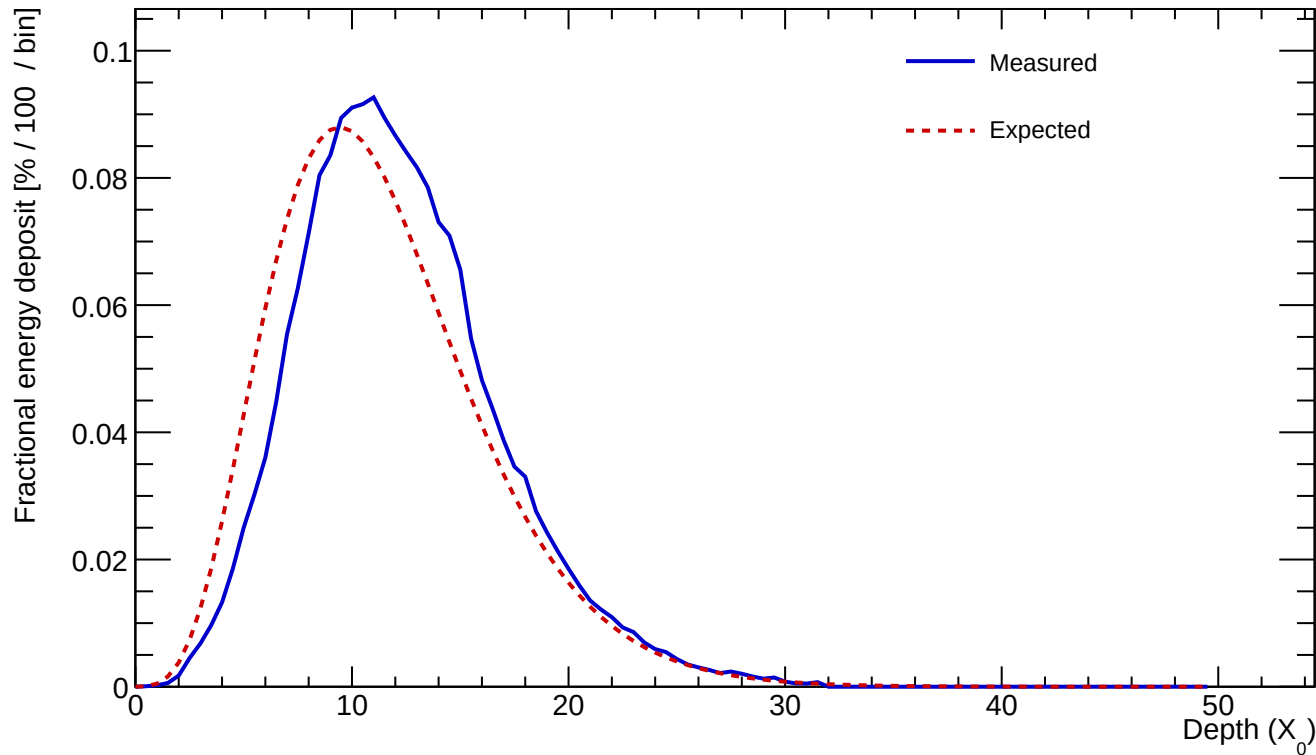
Cluster 73 E=1006.518 GeV profileStart=1.00 X_0 \chi=0.0700
