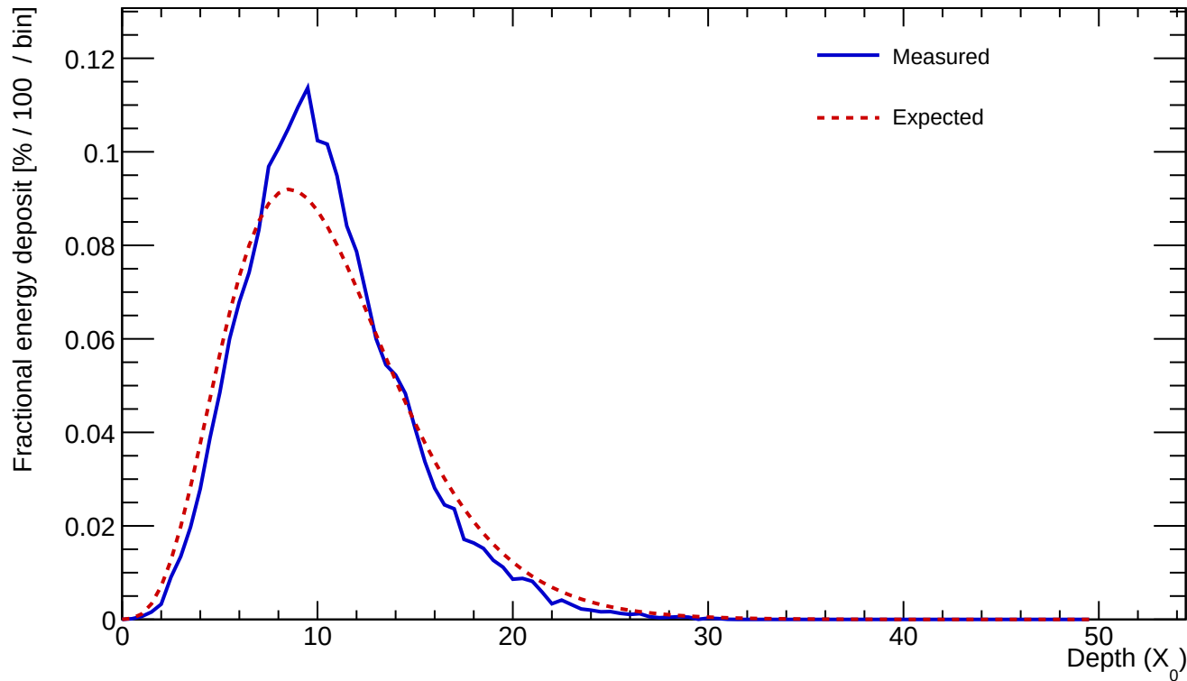
Cluster 41 E=421.725 GeV profileStart=0.50 X_0 \chi=0.1365
