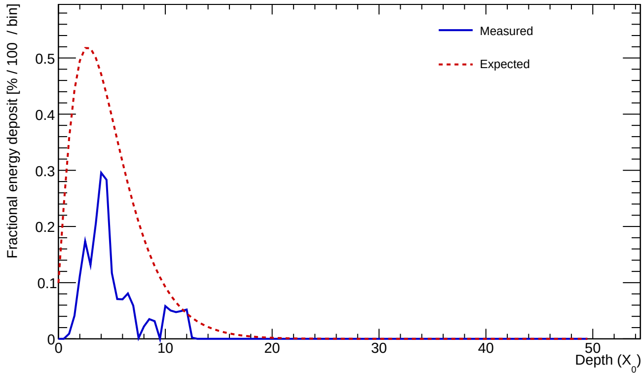
Cluster 123 E=1.234 GeV profileStart=1.00 X_0 \chi=0.4794
