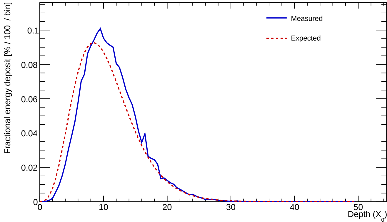
Cluster 29 E=370.430 GeV profileStart=1.00 X_0 \chi=0.0653
