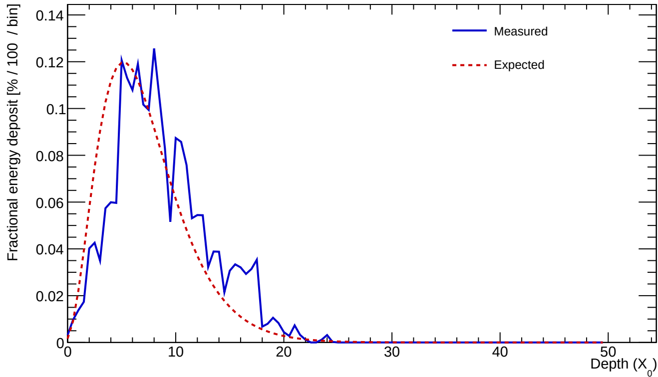
Cluster 3 E=14.030 GeV profileStart=1.50 X_0 \chi=0.2188
