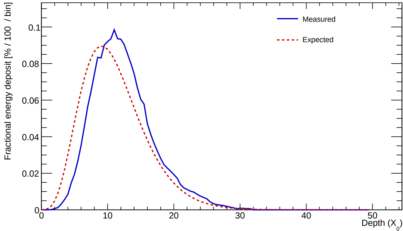
Cluster 249 E=710.334 GeV profileStart=1.50 X_0 \chi=0.0719
