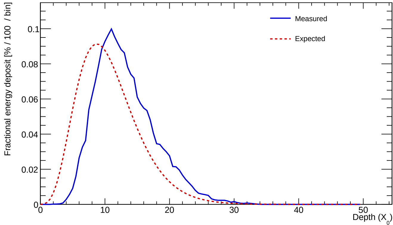
Cluster 84 E=485.065 GeV profileStart=2.50 X_0 \chi=0.0531
