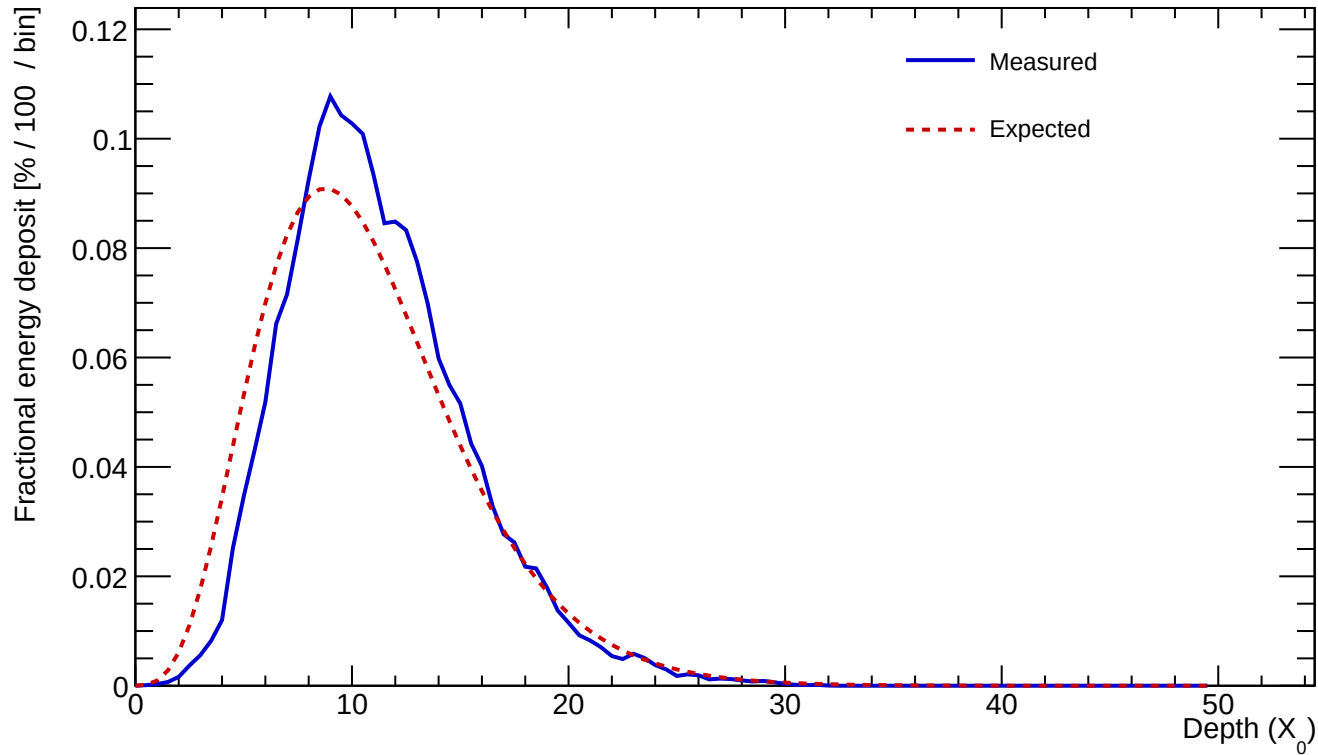
Cluster 12 E=523.137 GeV profileStart=1.00 X_0 \chi=0.1159
