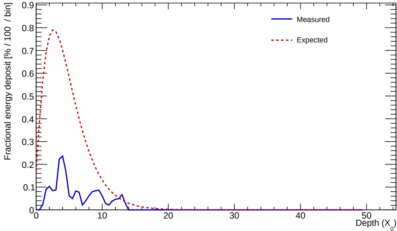
Cluster 224 E=1.098 GeV profileStart=1.00 X_0 \chi=0.4475
