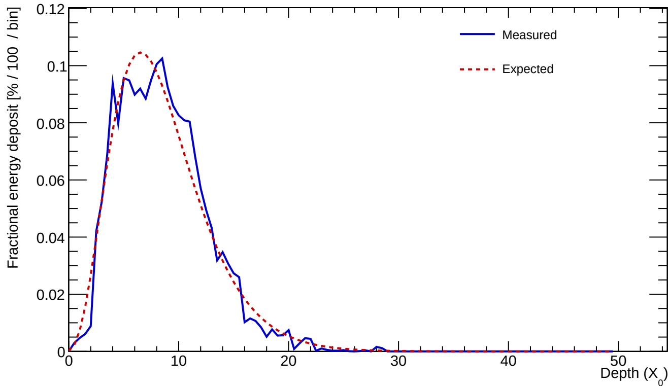
Cluster 120 E=54.391 GeV profileStart=0.50 X_0 \chi=0.1272
