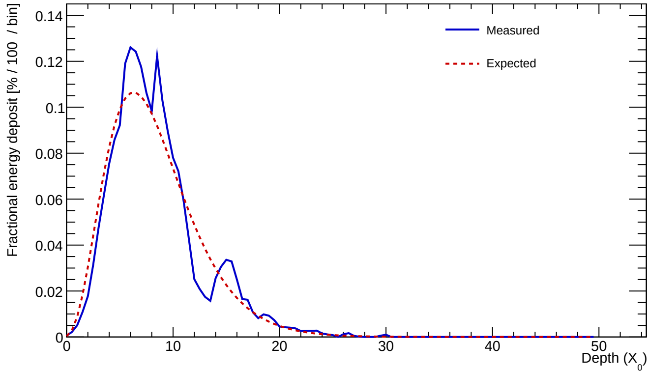
Cluster 90 E=43.509 GeV profileStart=0.50 X_0 \chi=0.1586
