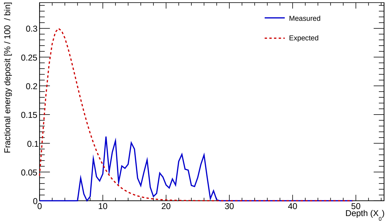
Cluster 263 E=1.644 GeV profileStart=9.00 X_0 \chi=0.7481
