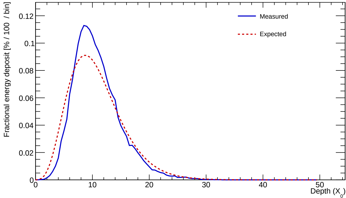
Cluster 19 E=500.274 GeV profileStart=0.50 X_0 \chi=0.1676
