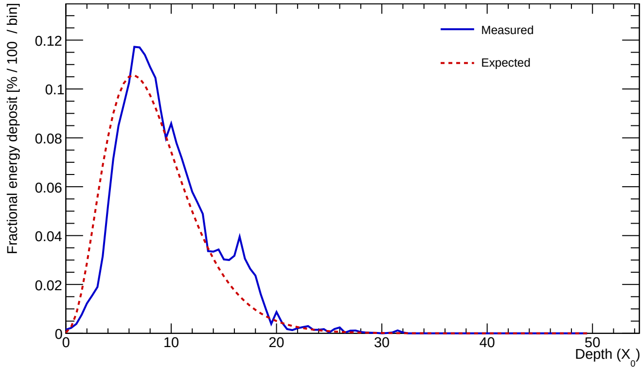
Cluster 91 E=47.977 GeV profileStart=1.00 X_0 \chi=0.1194
