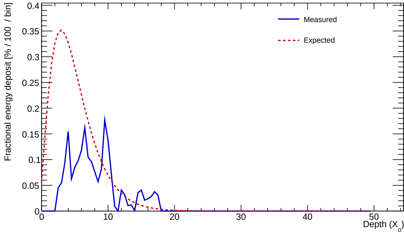
Cluster 125 E=1.478 GeV profileStart=2.50 X_0 \chi=0.4261
