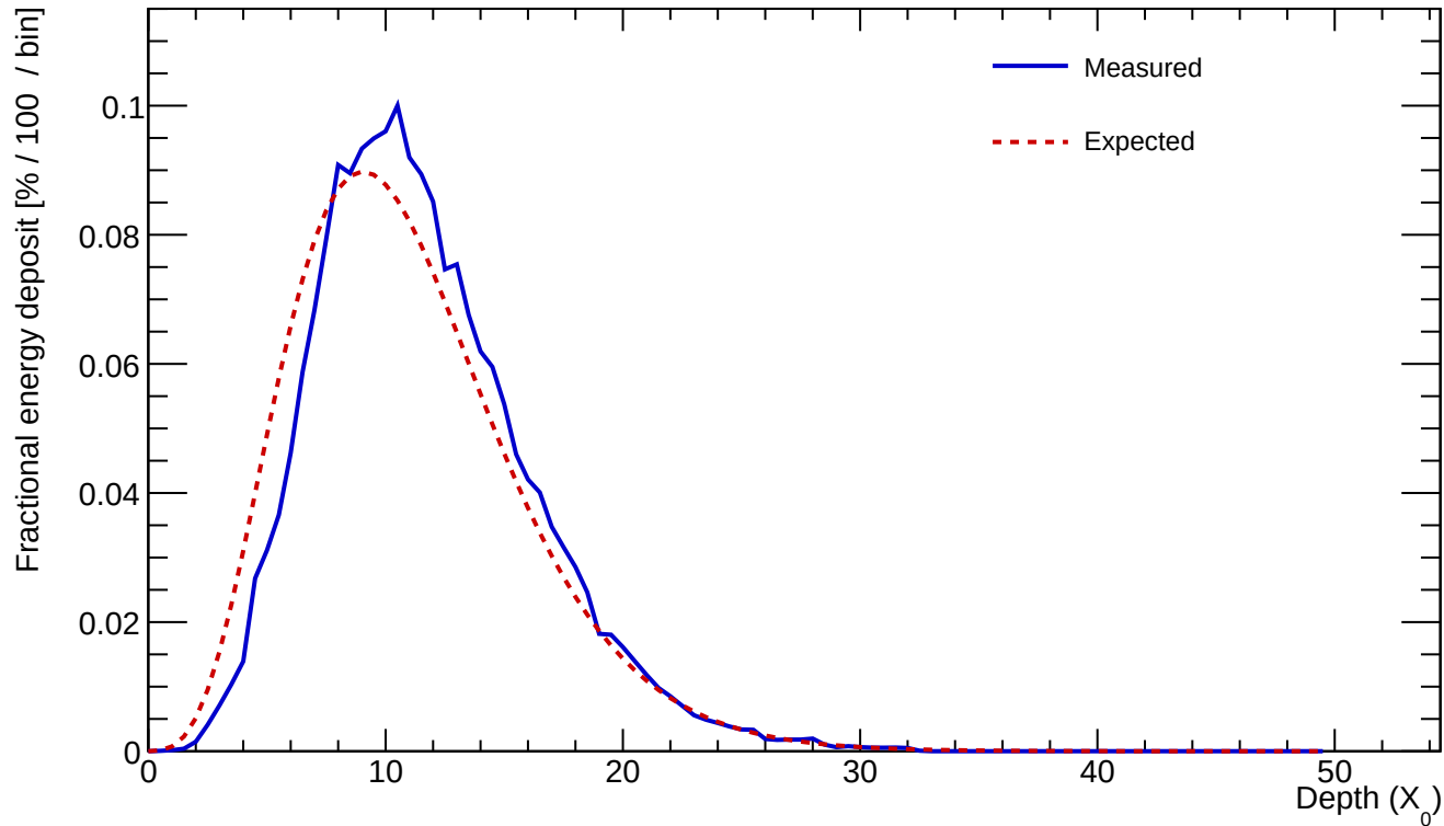
Cluster 241 E=670.533 GeV profileStart=1.00 X_0 \chi=0.0780
