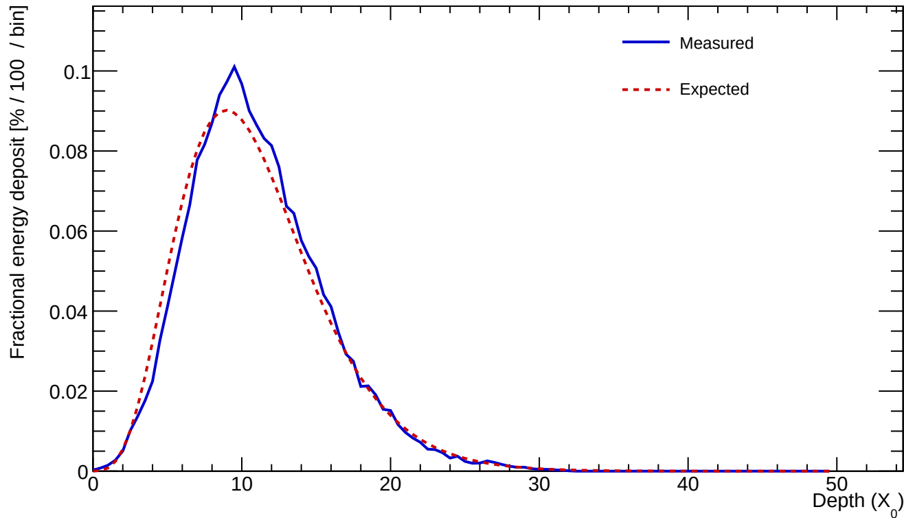
Cluster 86 E=614.362 GeV profileStart=0.50 X_0 \chi=0.0587
