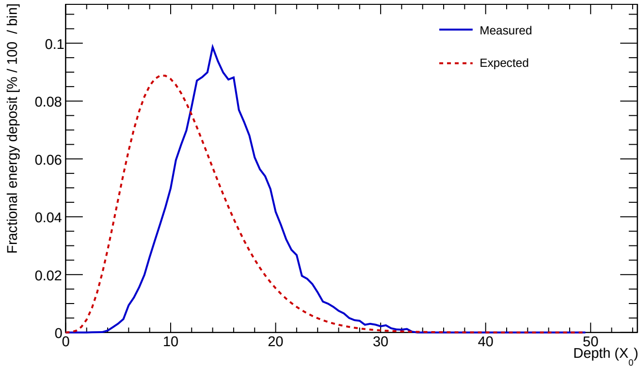
Cluster 93 E=811.974 GeV profileStart=4.50 X_0 \chi=0.0893
