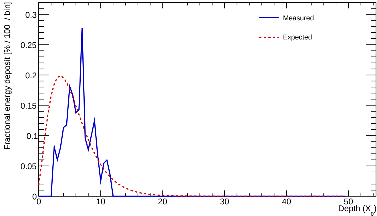
Cluster 69 E=2.561 GeV profileStart=2.00 X_0 \chi=0.2432
