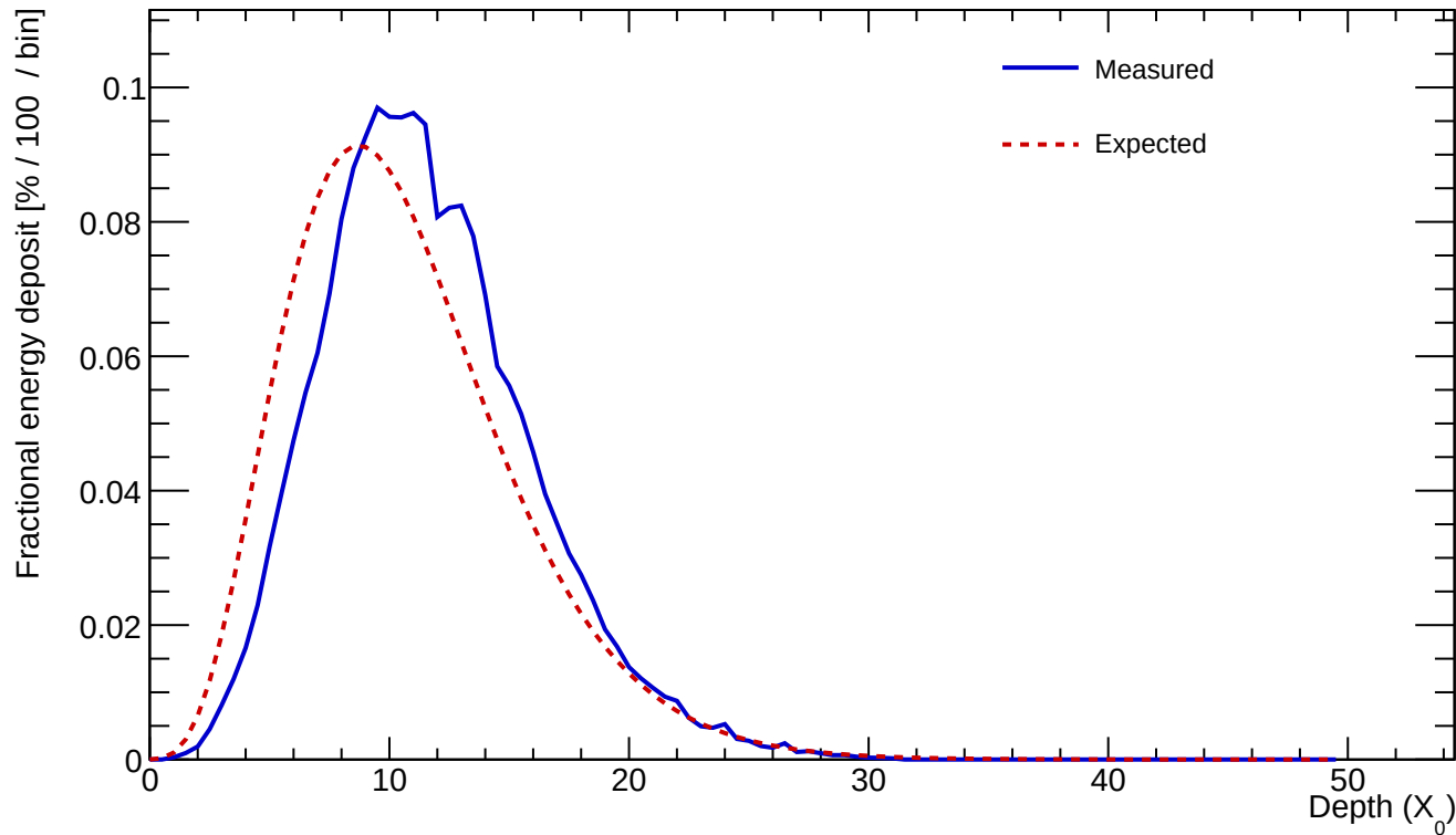
Cluster 44 E=478.515 GeV profileStart=1.00 X_0 \chi=0.0875
