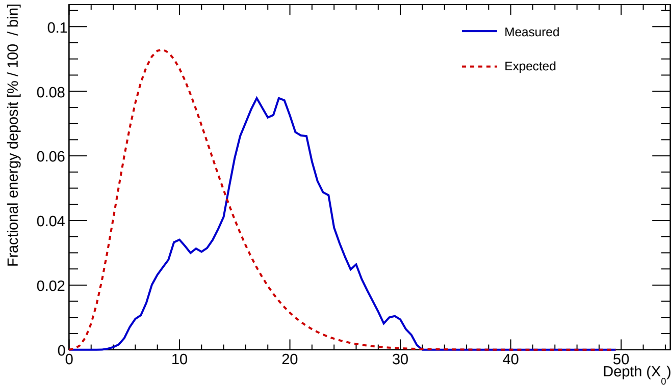
Cluster 66 E=350.286 GeV profileStart=9.00 X_0 \chi=0.2888
