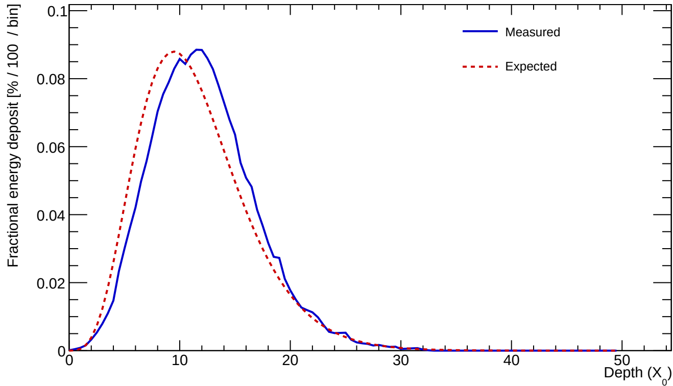
Cluster 235 E=1010.360 GeV profileStart=1.00 X_0 \chi=0.0729
