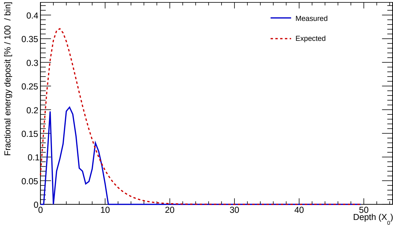
Cluster 230 E=1.433 GeV profileStart=2.00 X_0 \chi=0.4340
