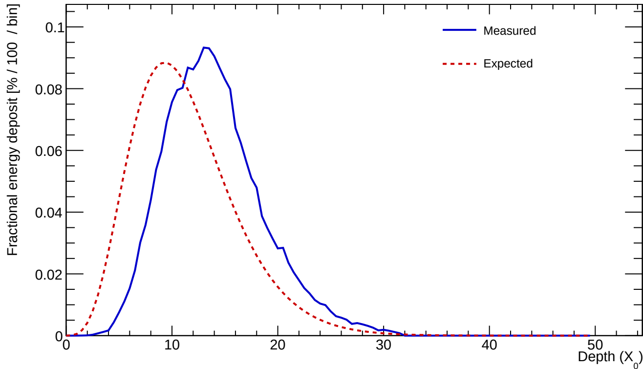
Cluster 42 E=899.600 GeV profileStart=3.00 X_0 \chi=0.0617
