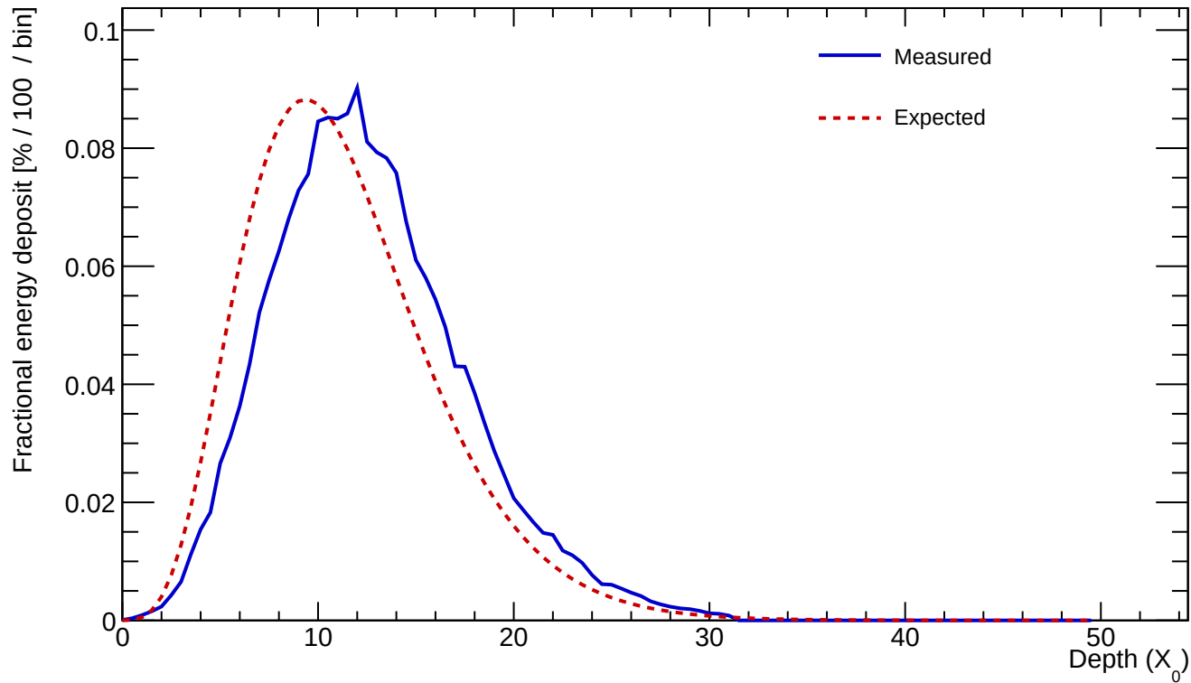
Cluster 173 E=940.180 GeV profileStart=1.50 X_0 \chi=0.0636
