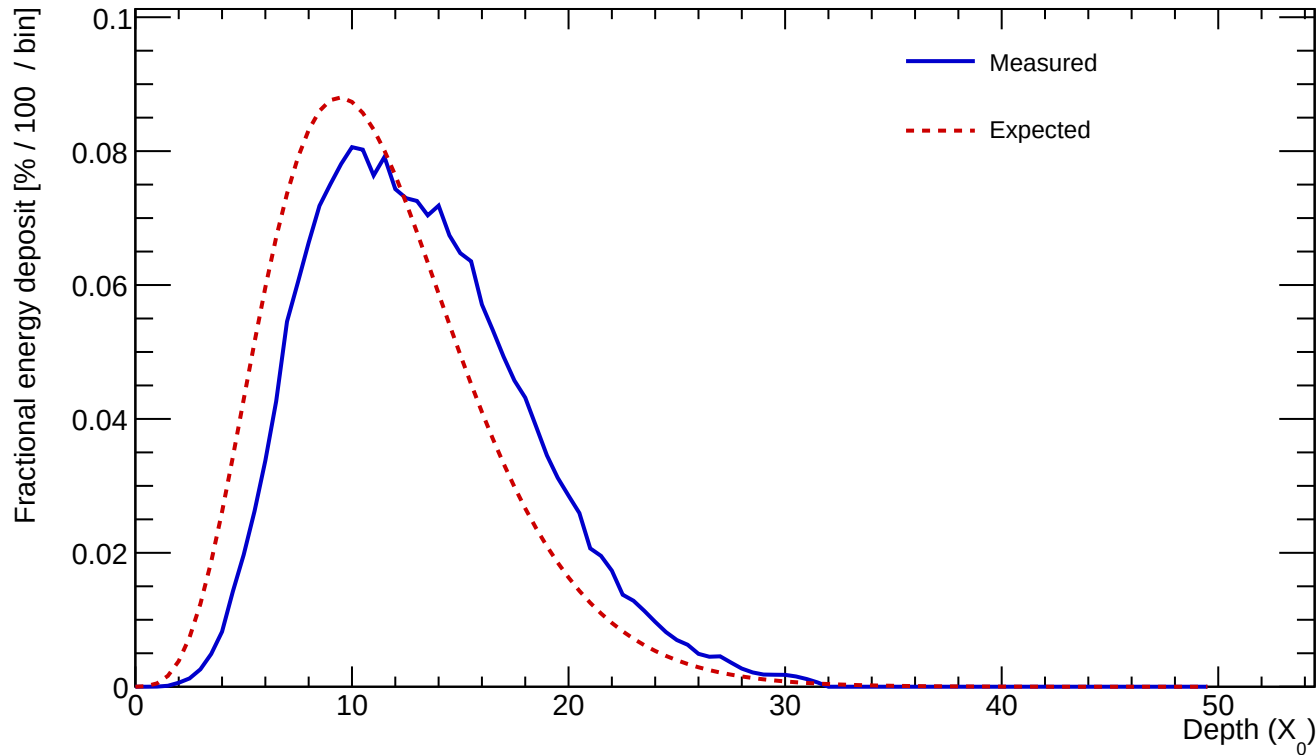
Cluster 25 E=997.707 GeV profileStart=1.50 X_0 \chi=0.0838
