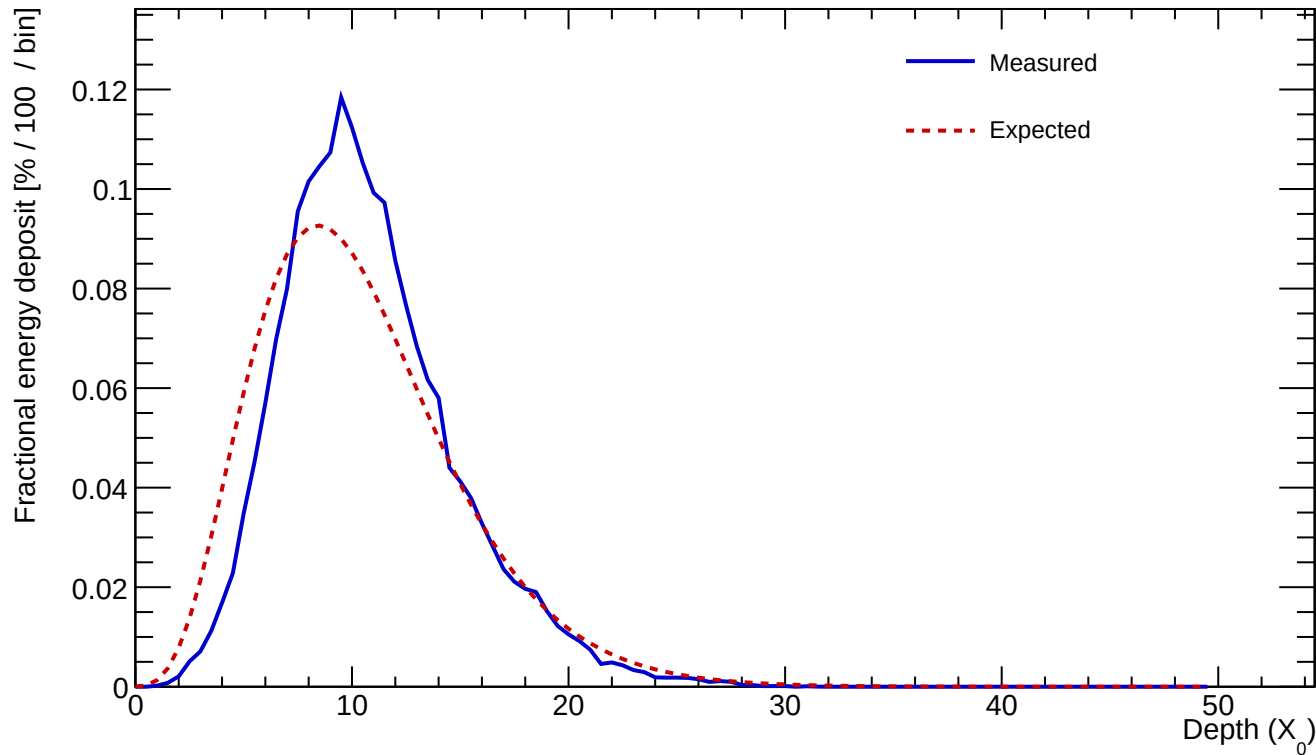
Cluster 37 E=367.406 GeV profileStart=1.00 X_0 \chi=0.1615
