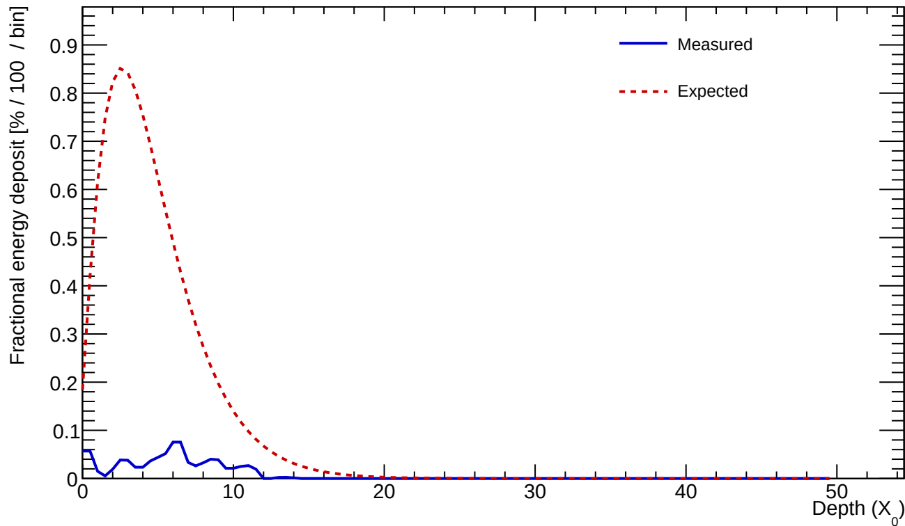
Cluster 49 E=1.081 GeV profileStart=2.00 X_0 \chi=0.5132
