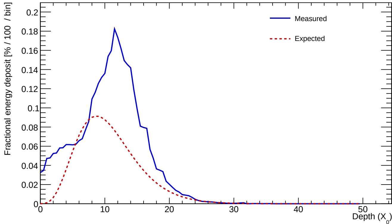
Cluster 76 E=477.923 GeV profileStart=1.50 X_0 \chi=0.3079
