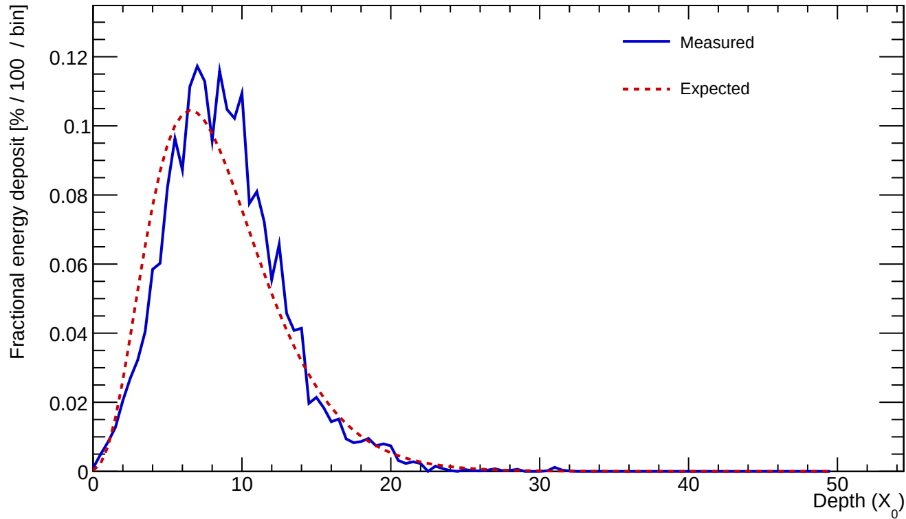
Cluster 59 E=55.465 GeV profileStart=0.50 X_0 \chi=0.1489
