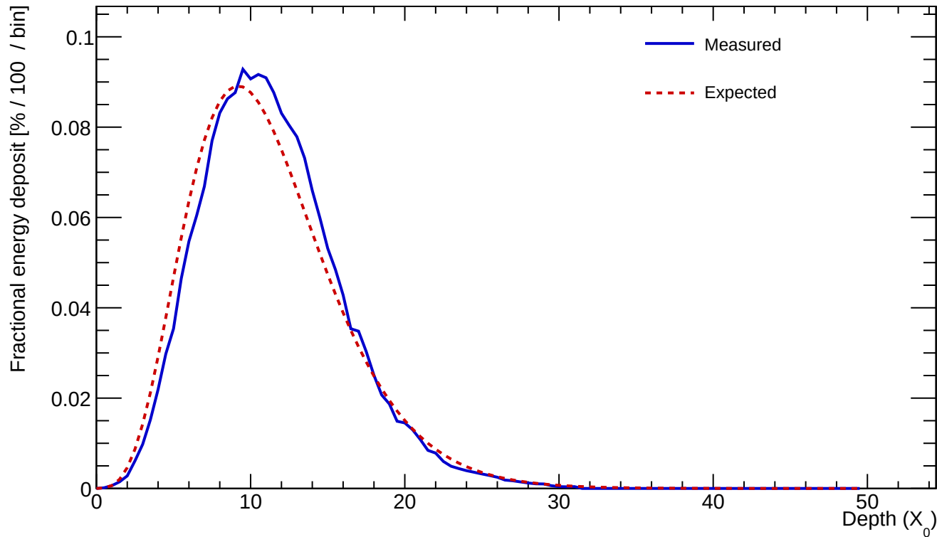
Cluster 215 E=774.770 GeV profileStart=0.50 X_0 \chi=0.0611
