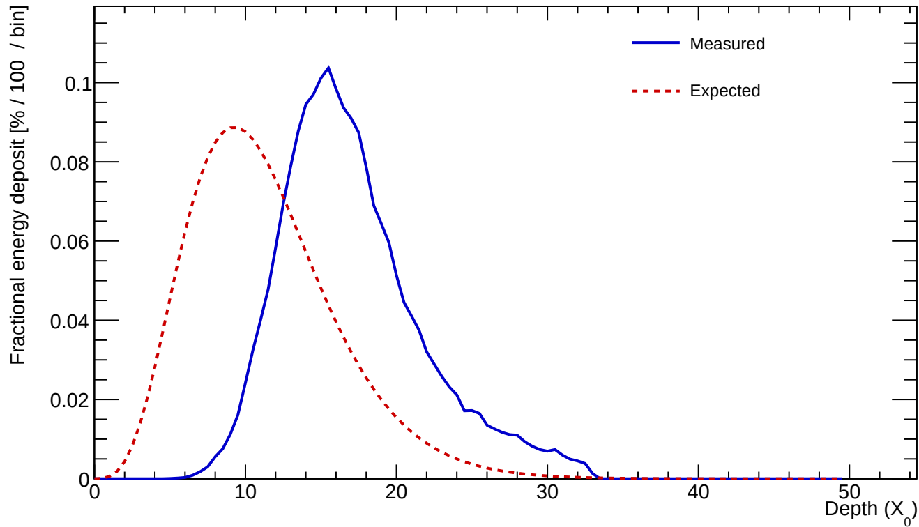
Cluster 4 E=841.880 GeV profileStart=6.00 X_0 \chi=0.1140
