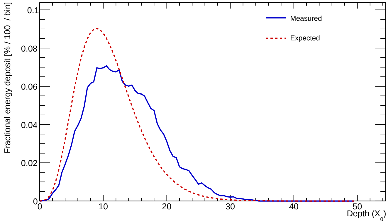
Cluster 7 E=608.651 GeV profileStart=2.00 X_0 \chi=0.2319
