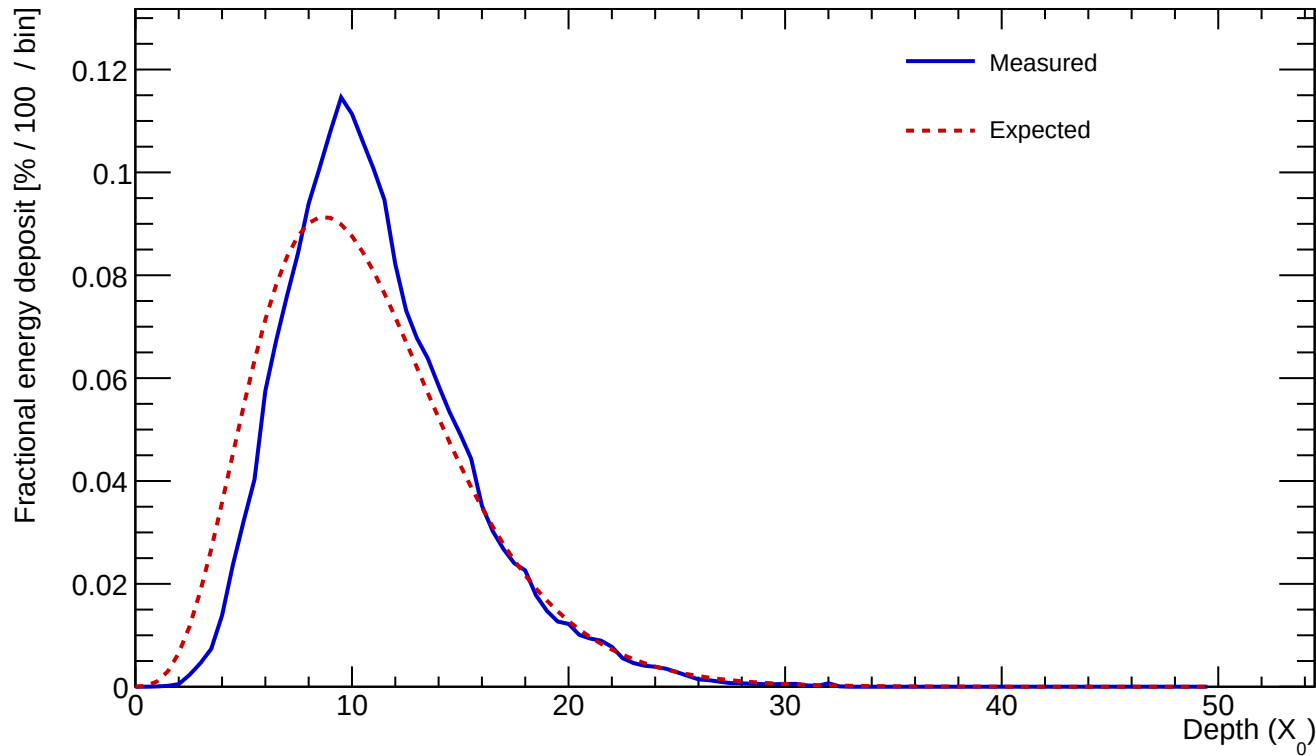
Cluster 46 E=477.433 GeV profileStart=0.50 X_0 \chi=0.1427
