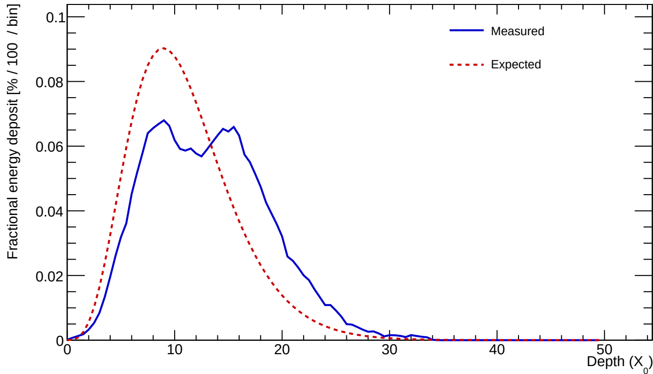
Cluster 43 E=602.461 GeV profileStart=2.00 X_0 \chi=0.2748
