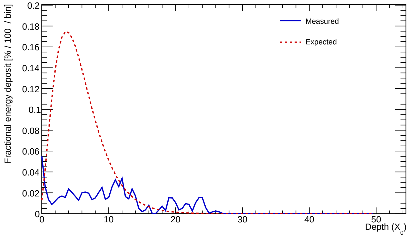
Cluster 264 E=3.219 GeV profileStart=3.00 X_0 \chi=0.8422
