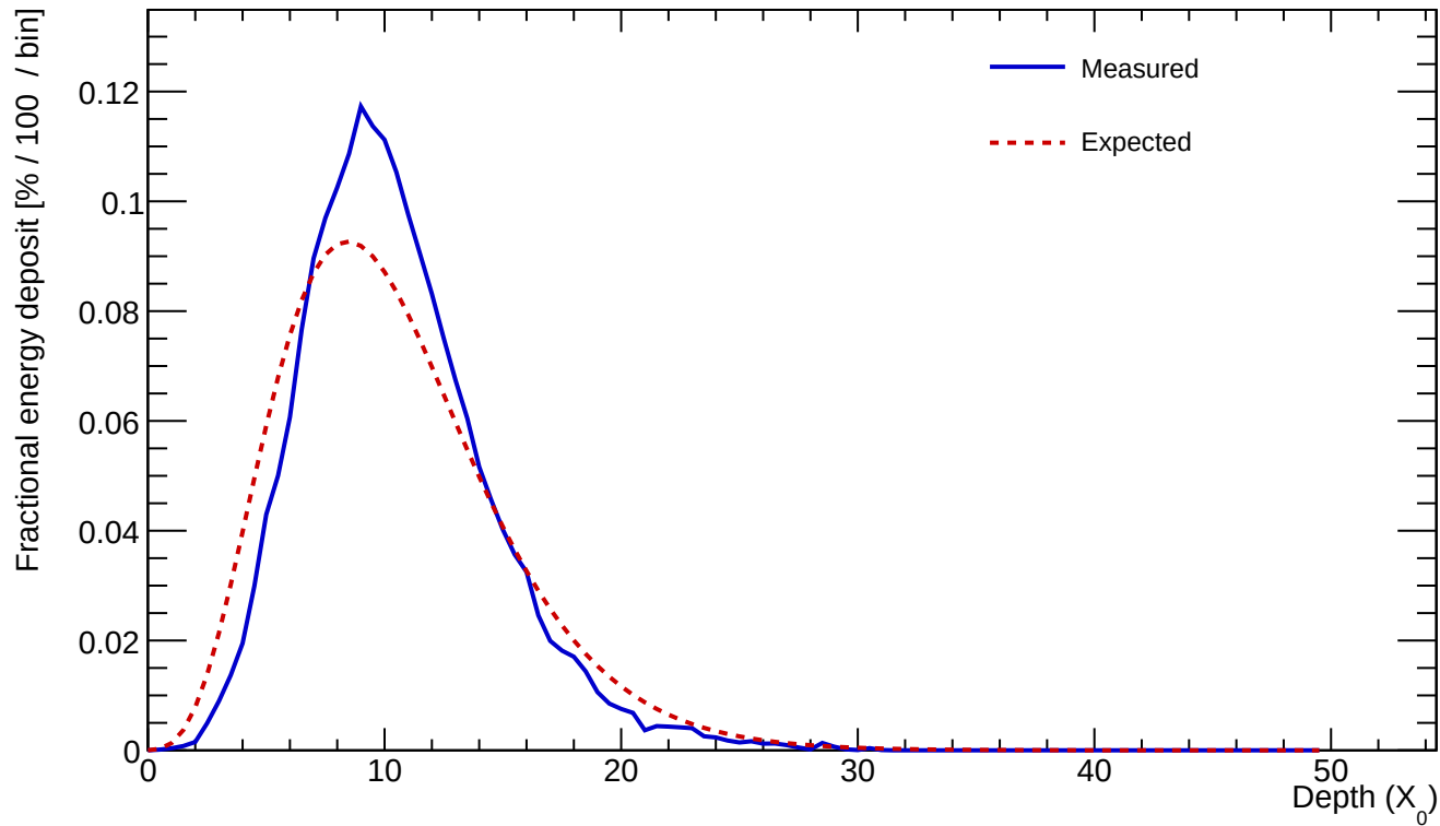
Cluster 17 E=366.990 GeV profileStart=0.50 X_0 \chi=0.1755
