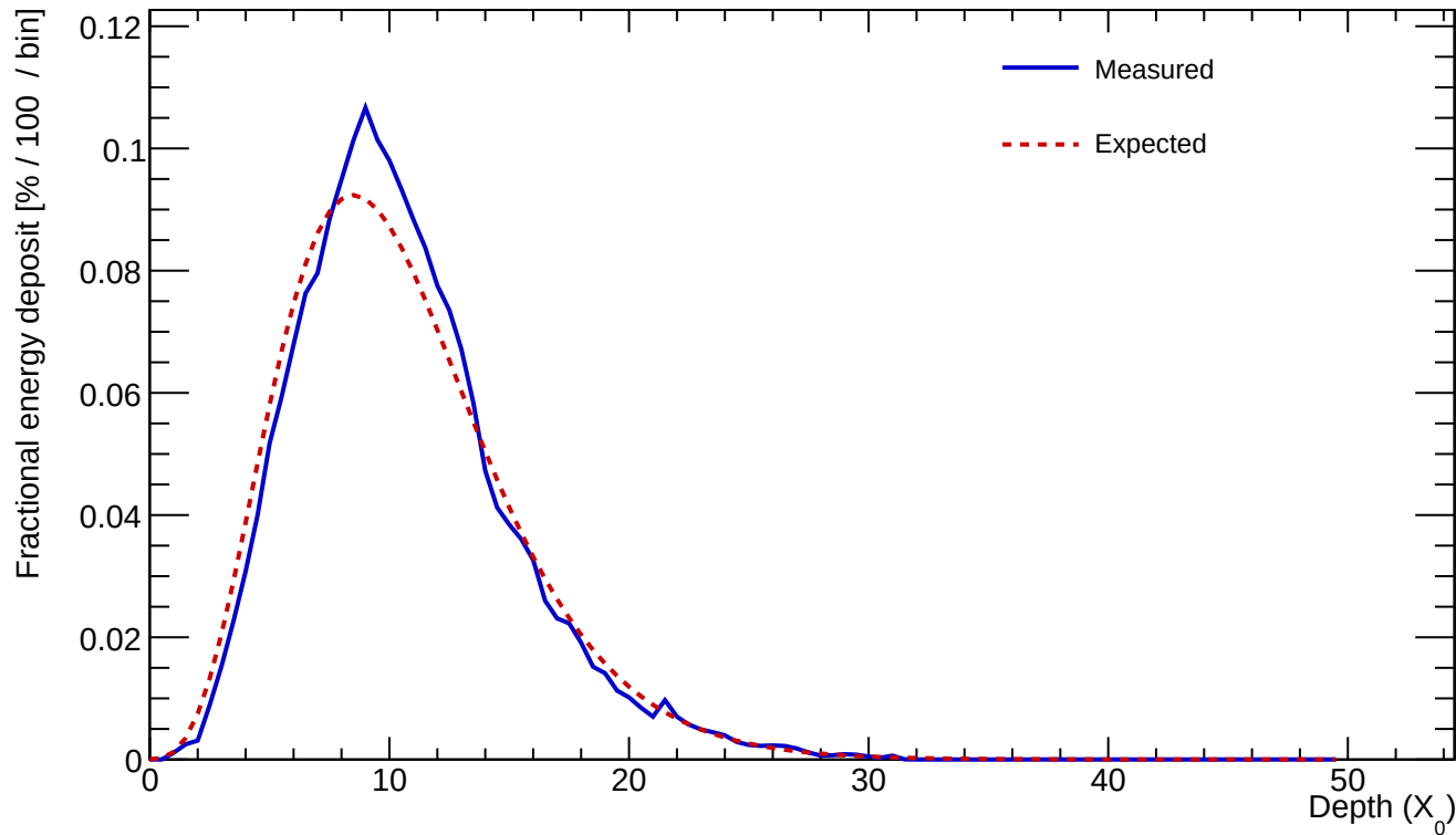
Cluster 79 E=391.078 GeV profileStart=0.50 X_0 \chi=0.0896
