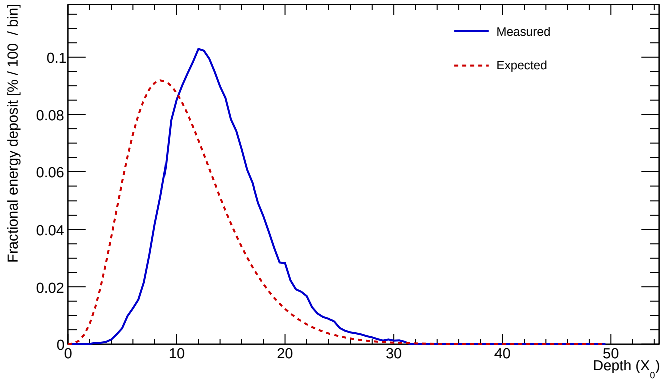
Cluster 71 E=428.287 GeV profileStart=3.50 X_0 \chi=0.0929
