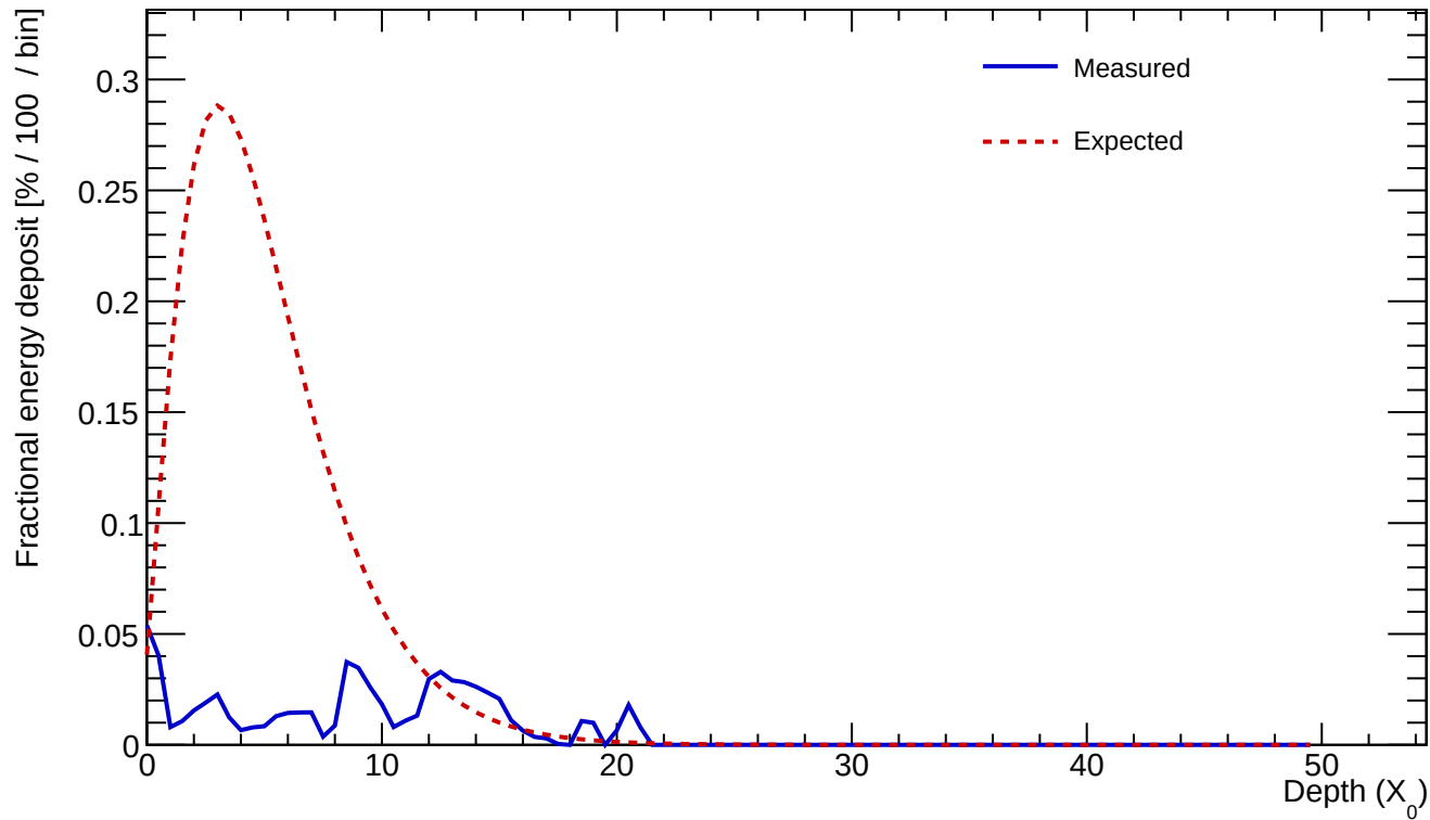
Cluster 280 E=1.695 GeV profileStart=7.00 X_0 \chi=0.8144
