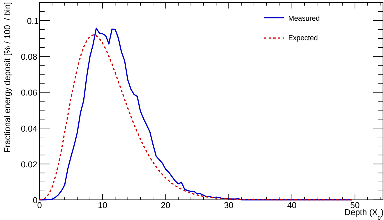
Cluster 26 E=423.436 GeV profileStart=2.00 X_0 \chi=0.0755
