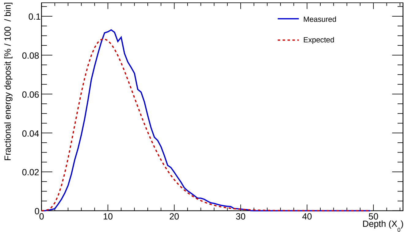
Cluster 40 E=929.979 GeV profileStart=1.00 X_0 \chi=0.0457
