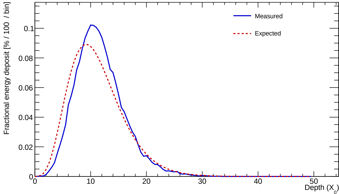
Cluster 50 E=770.350 GeV profileStart=1.00 X_0 \chi=0.1140
