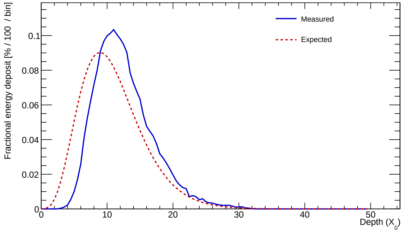
Cluster 14 E=605.459 GeV profileStart=2.00 X_0 \chi=0.1119
