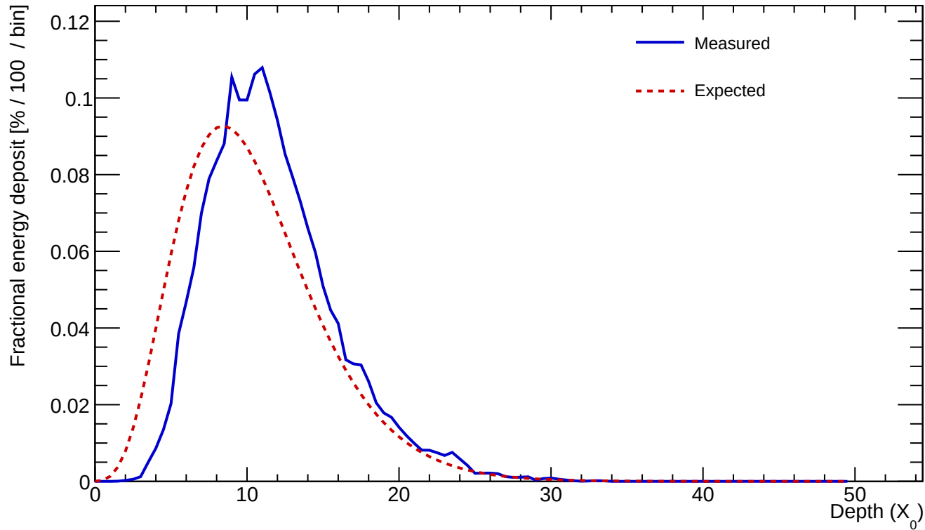
Cluster 30 E=364.665 GeV profileStart=1.50 X_0 \chi=0.1109
