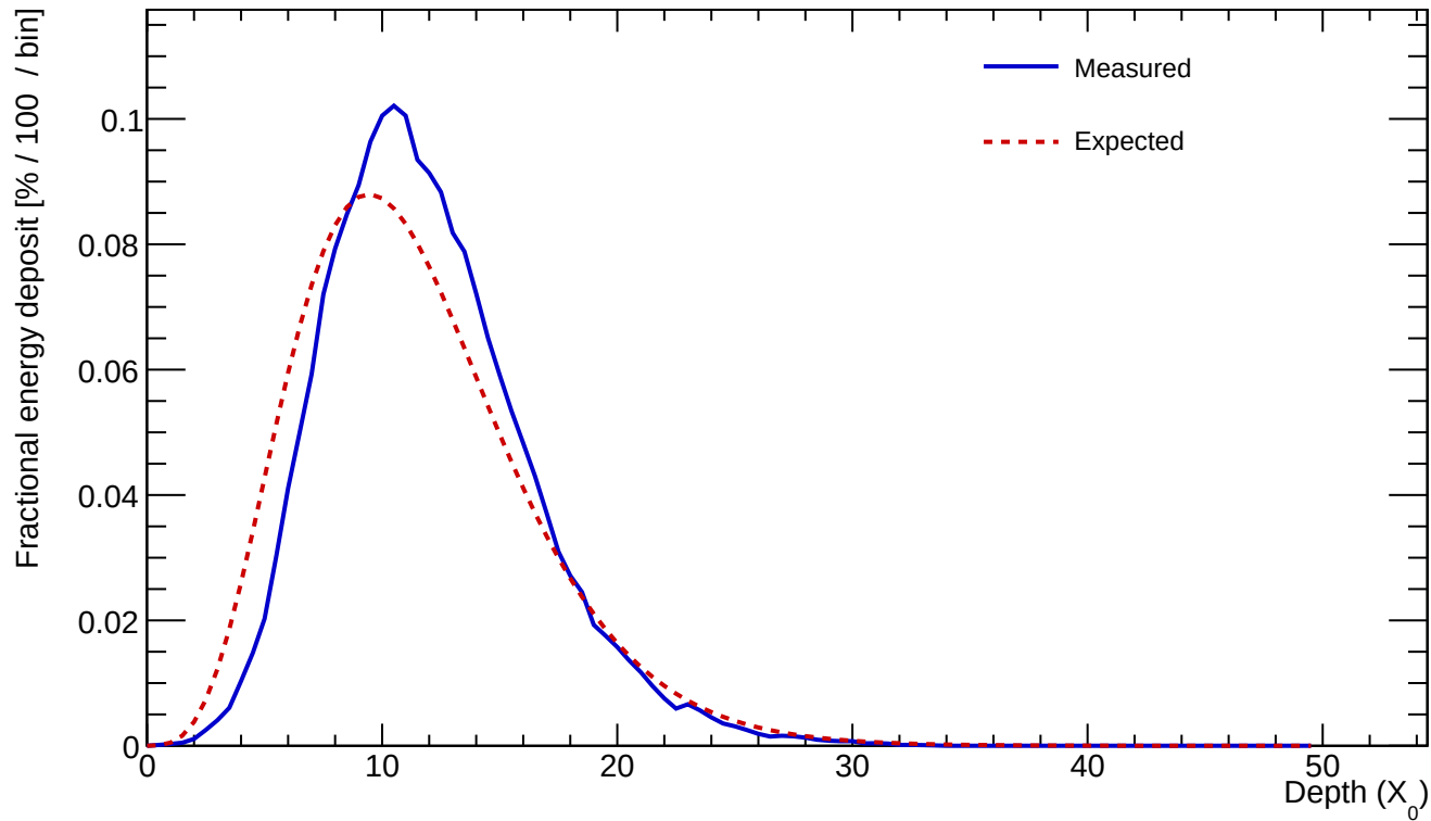
Cluster 131 E=1007.314 GeV profileStart=1.00 X_0 \chi=0.1176
