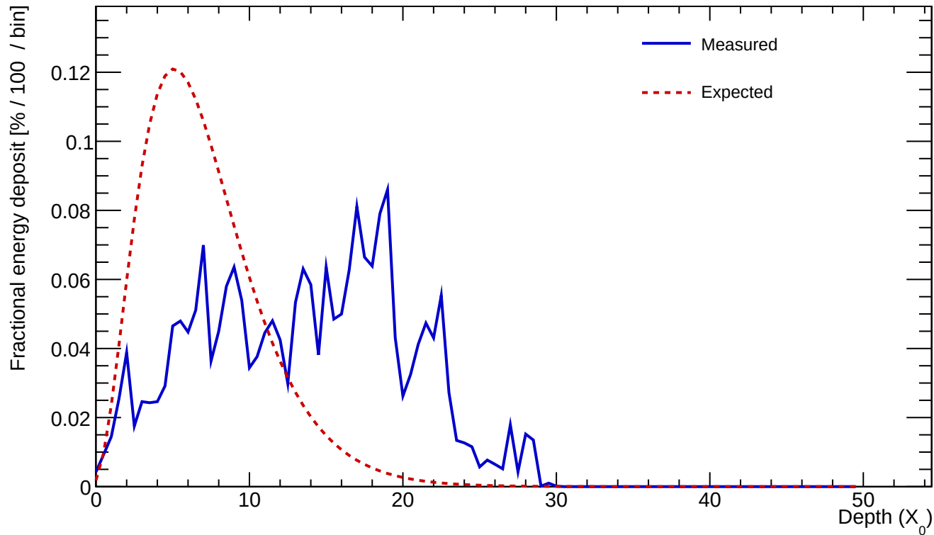
Cluster 237 E=13.050 GeV profileStart=4.50 X_0 \chi=0.8054
