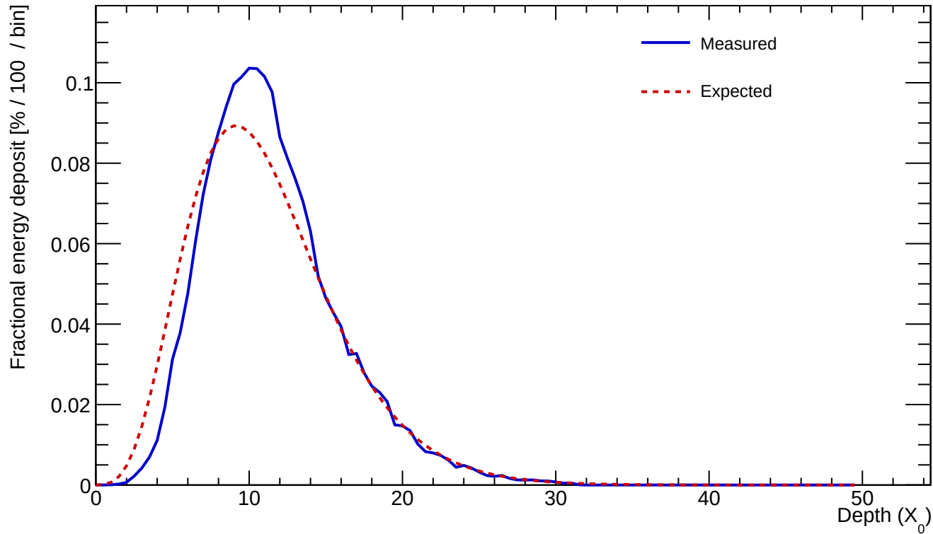
Cluster 278 E=741.777 GeV profileStart=0.50 X_0 \chi=0.1274
