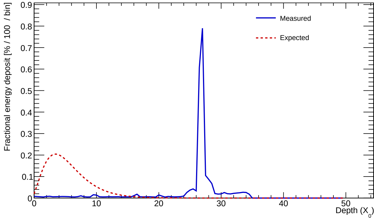
Cluster 35 E=2.449 GeV profileStart=24.00 X_0 \chi=1.0932
