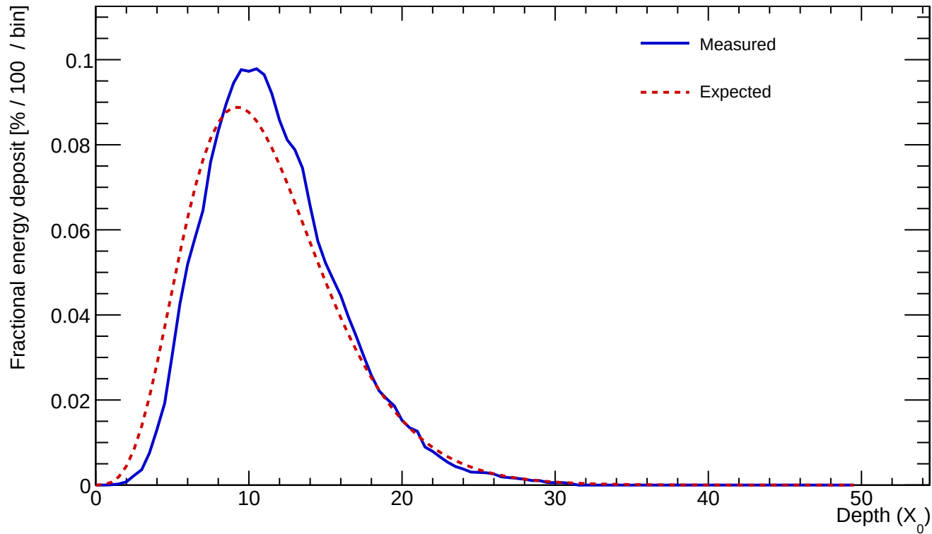
Cluster 254 E=814.927 GeV profileStart=0.50 X_0 \chi=0.0934
