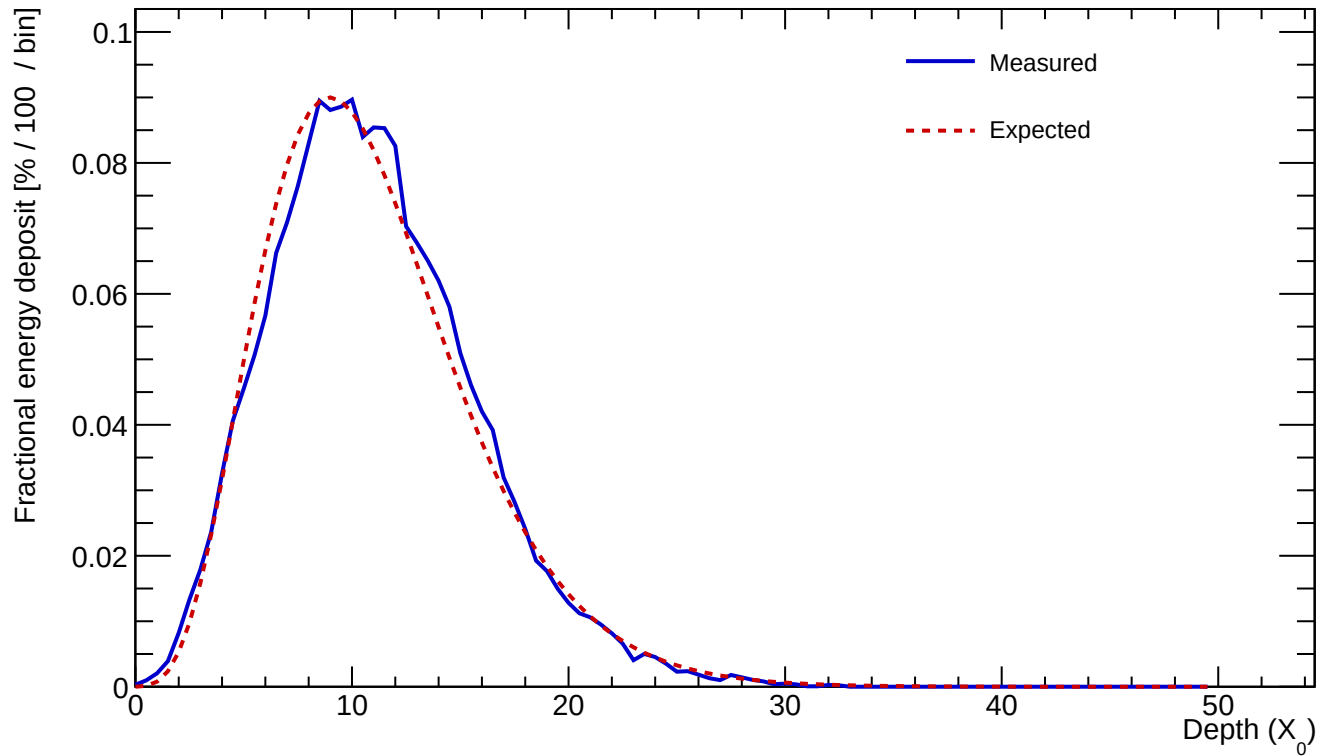
Cluster 75 E=640.344 GeV \text{profileStart}=0.50 X_0 \chi=0.0727
