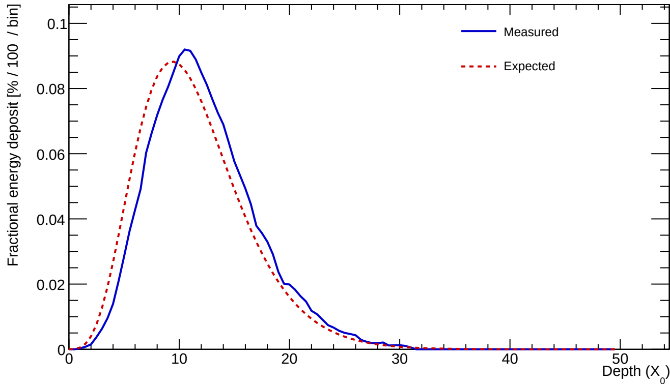
Cluster 96 E=946.820 GeV profileStart=1.00 X_0 \chi=0.0338
