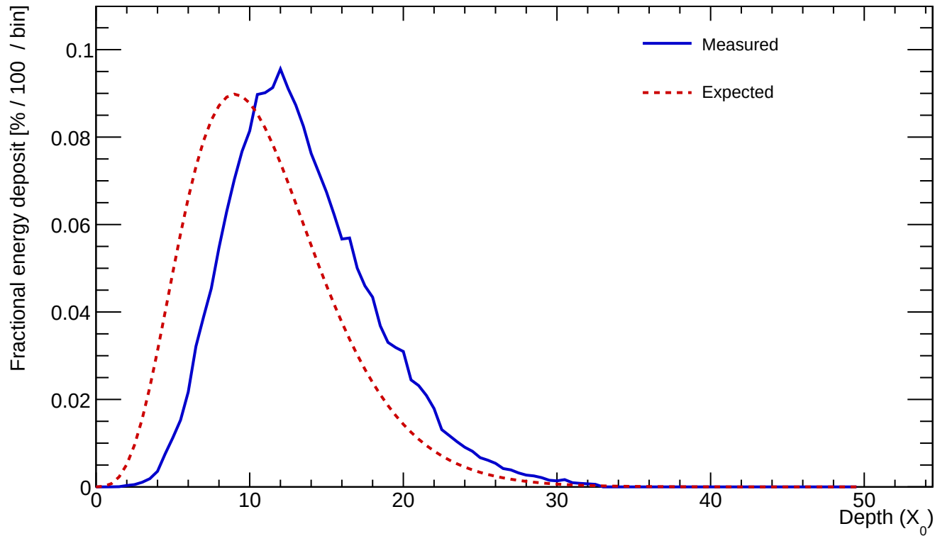
Cluster 78 E=666.176 GeV profileStart=2.50 X_0 \chi=0.0412
