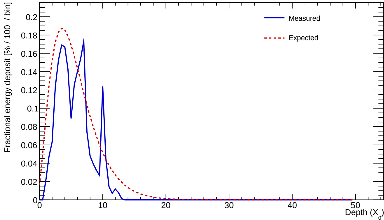
Cluster 126 E=2.823 GeV profileStart=0.50 X_0 \chi=0.3259
