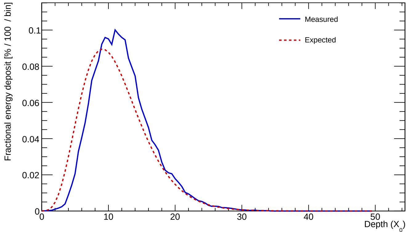
Cluster 166 E=726.428 GeV profileStart=1.00 X_0 \chi=0.1028
