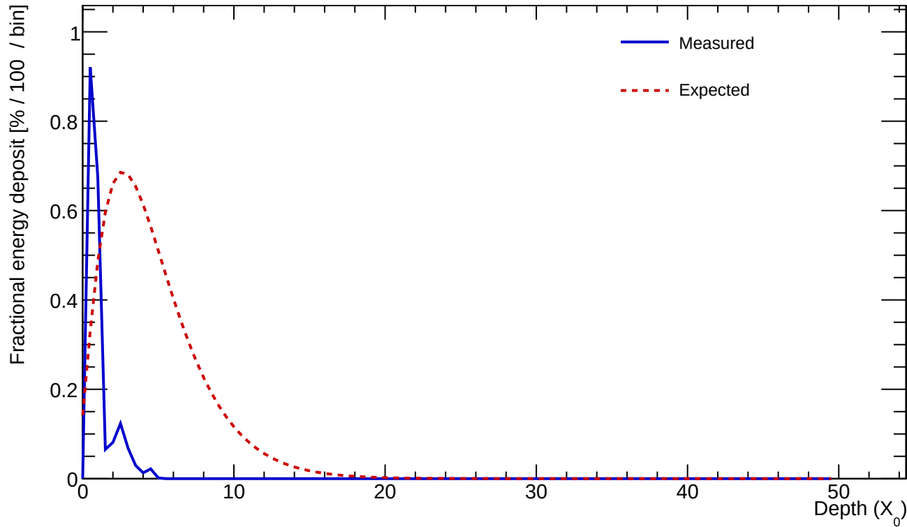
Cluster 265 E=1.134 GeV profileStart=4.50 X_0 \chi=0.9929
