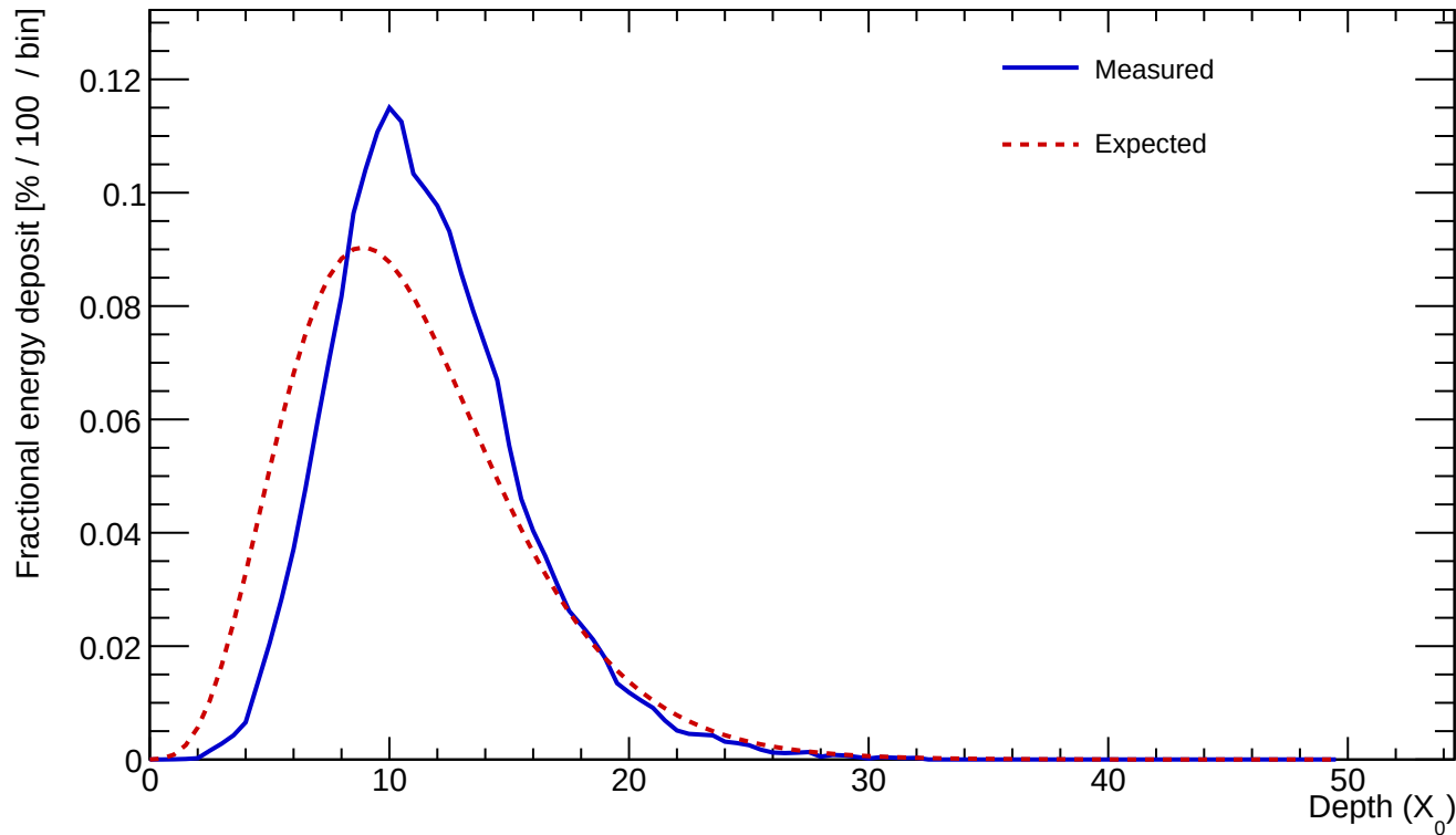
Cluster 89 E=586.199 GeV profileStart=1.50 X_0 \chi=0.1853
