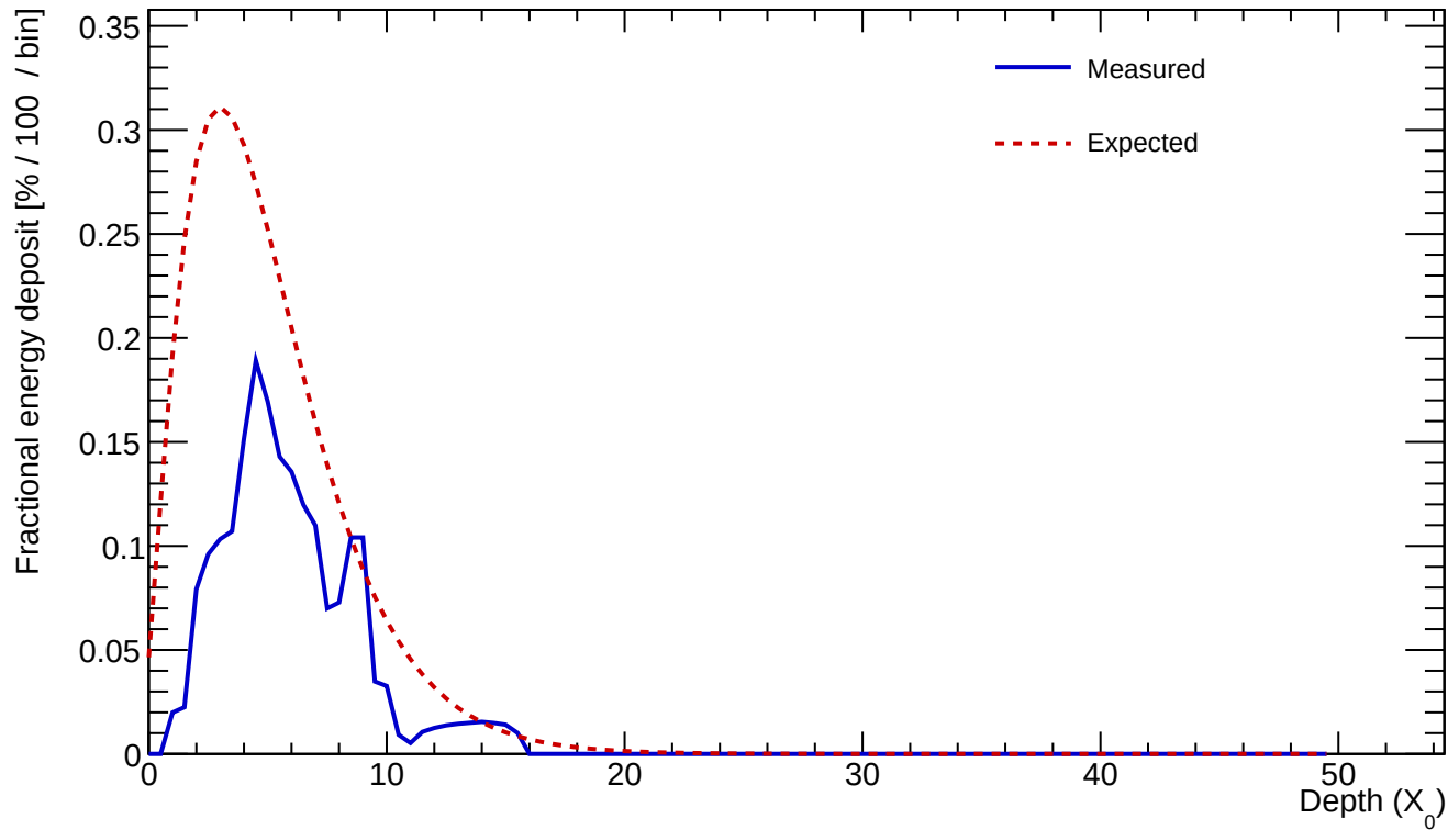
Cluster 161 E=1.601 GeV profileStart=1.50 X_0 \chi=0.2265
