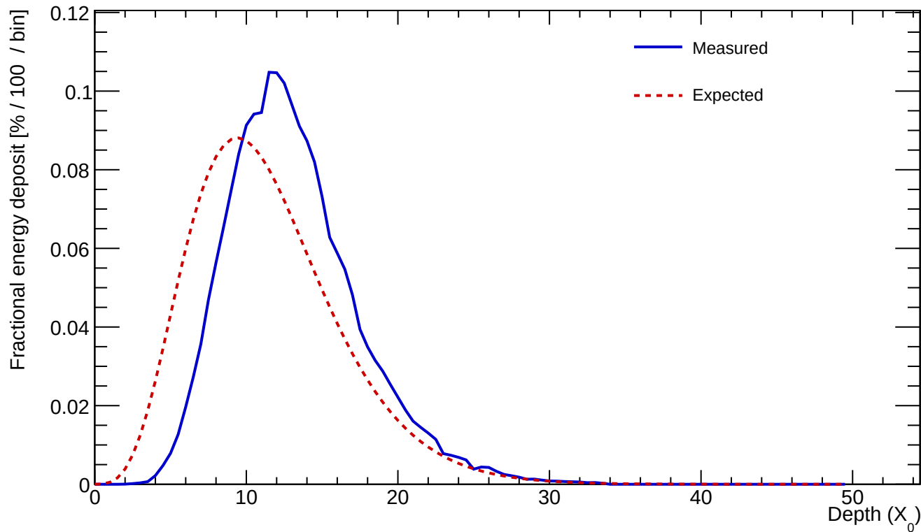
Cluster 95 E=981.870 GeV profileStart=2.00 X_0 \chi=0.1293
