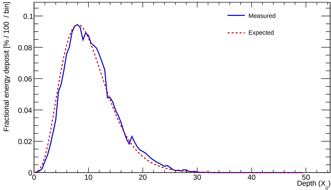
Cluster 145 E=255.260 GeV profileStart=0.50 X_0 \chi=0.0568
