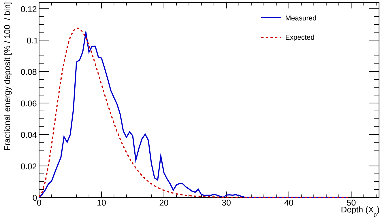
Cluster 118 E=37.568 GeV profileStart=2.00 X_0 \chi=0.1918
