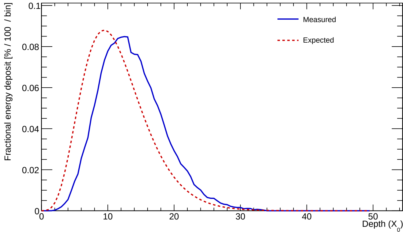
Cluster 262 E=1004.480 GeV profileStart=2.50 X_0 \chi=0.0507
