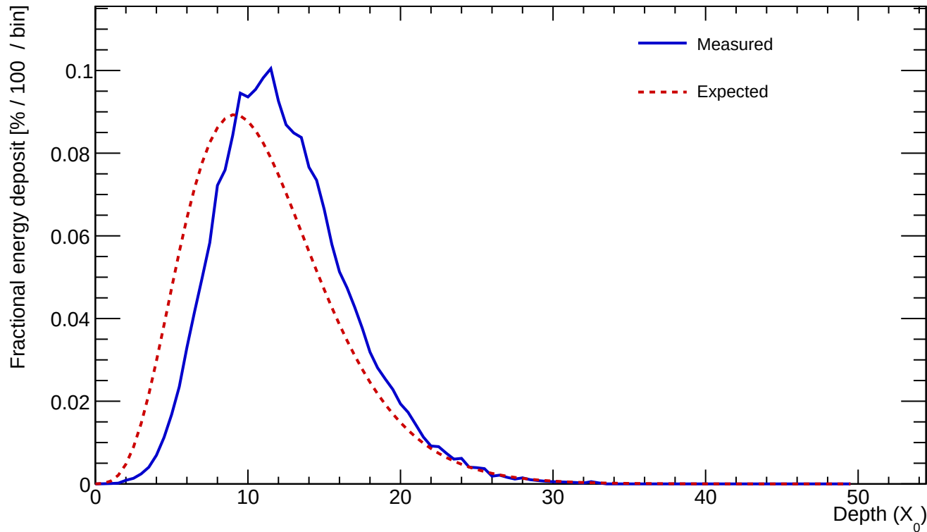
Cluster 27 E=742.416 GeV profileStart=1.50 X_0 \chi=0.0933
