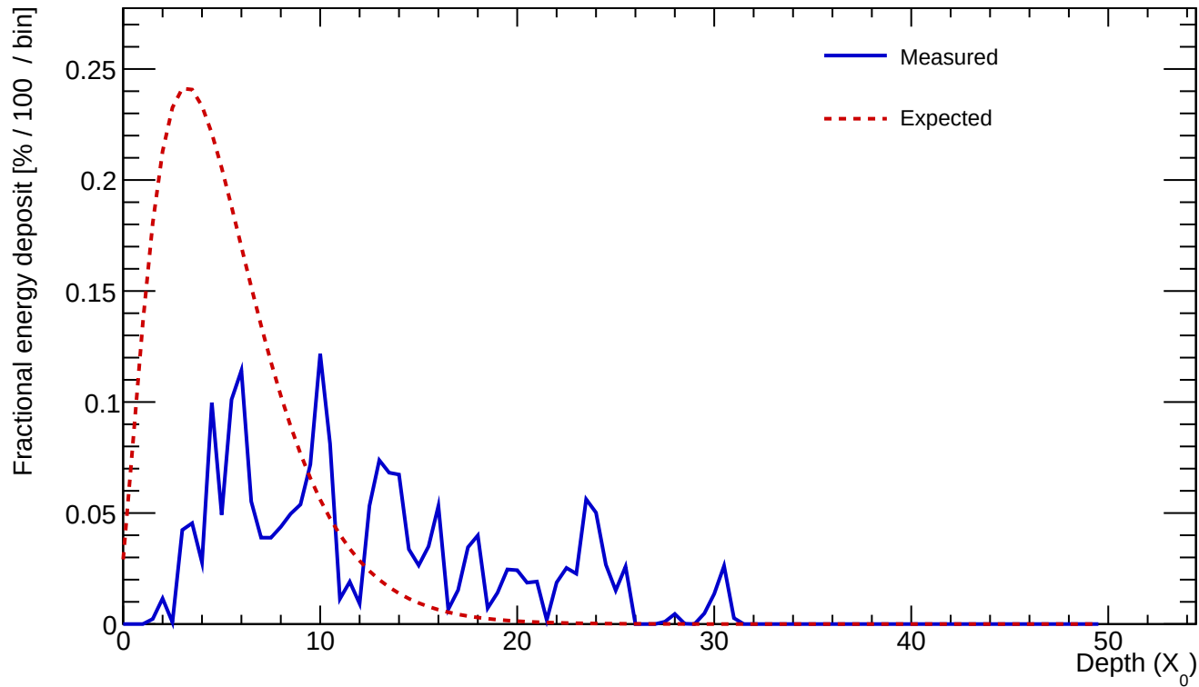
Cluster 47 E=1.991 GeV profileStart=4.00 X_0 \chi=0.7806
