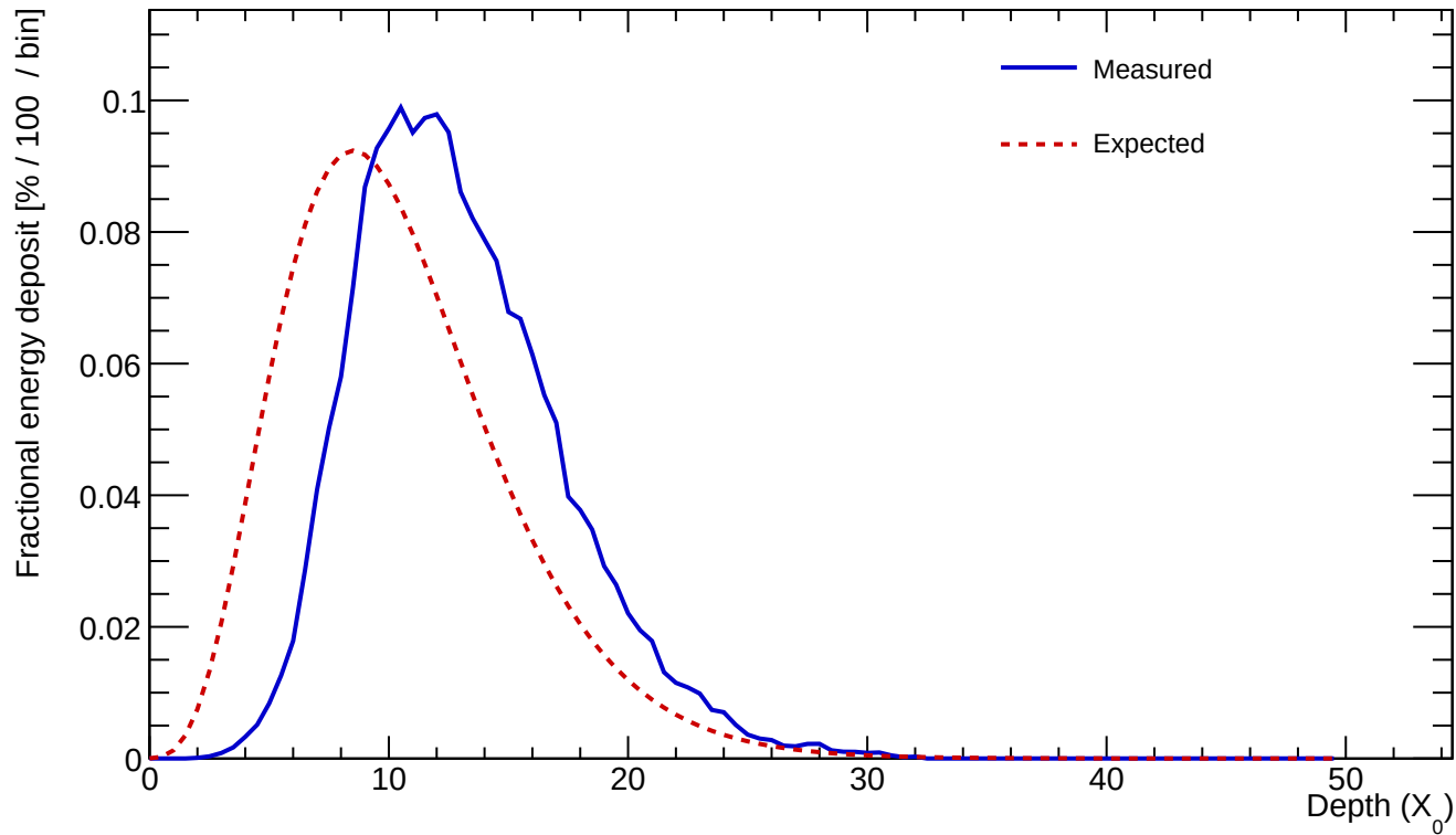
Cluster 72 E=391.032 GeV profileStart=3.00 X_0 \chi=0.0798
