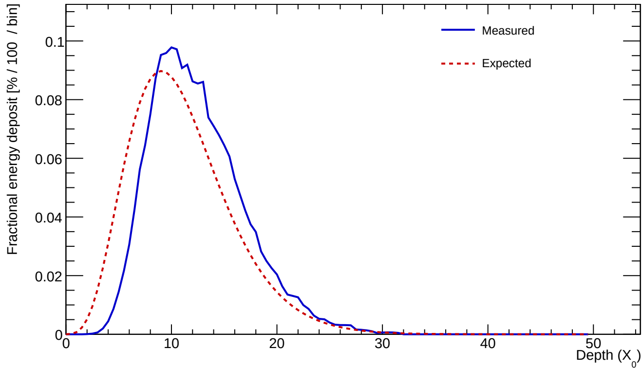
Cluster 38 E=675.652 GeV profileStart=1.50 X_0 \chi=0.0816
