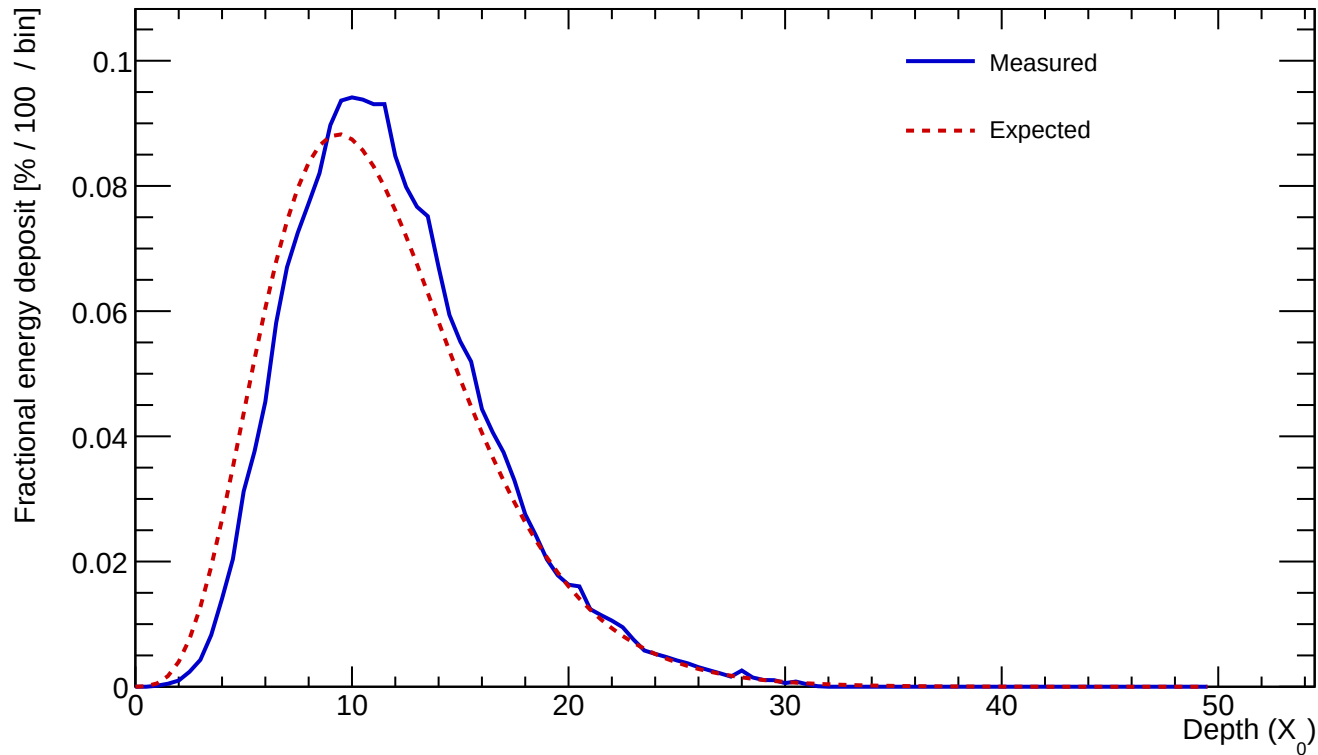
Cluster 291 E=945.115 GeV profileStart=0.50 X_0 \chi=0.0695
