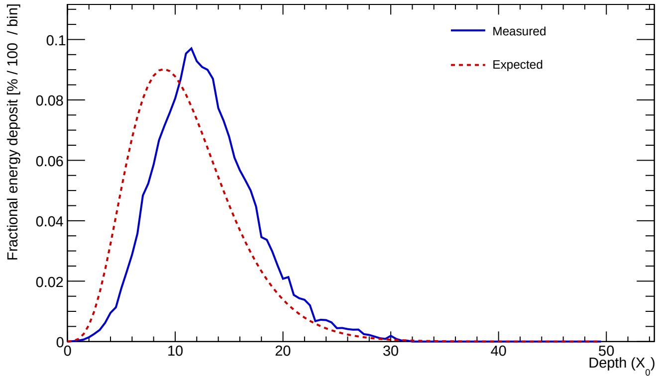
Cluster 82 E=608.824 GeV profileStart=2.50 X_0 \chi=0.0865
