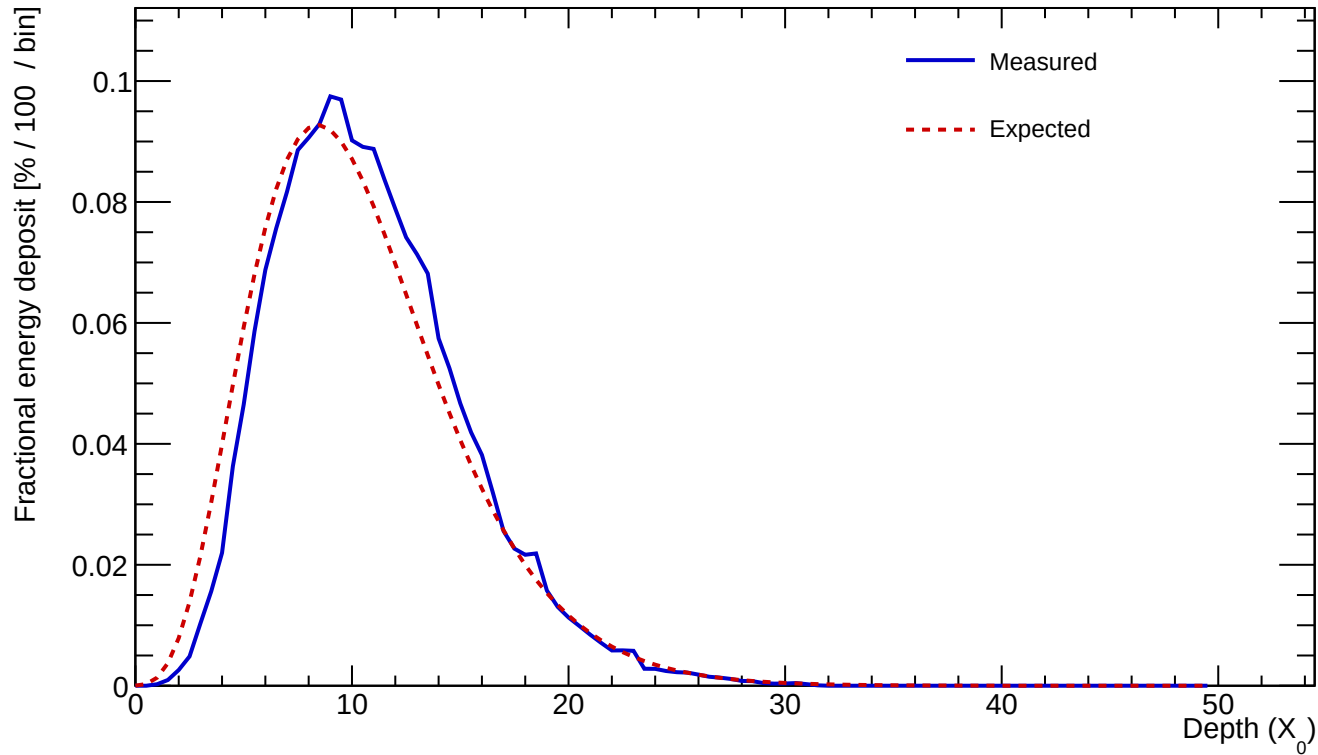
Cluster 33 E=364.055 GeV profileStart=0.50 X_0 \chi=0.0601
