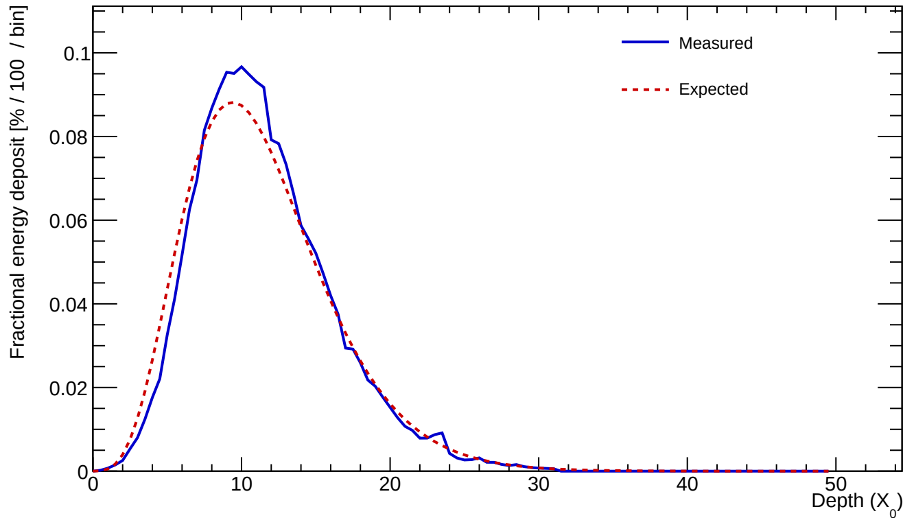
Cluster 238 E=959.026 GeV profileStart=0.50 X_0 \chi=0.0836
