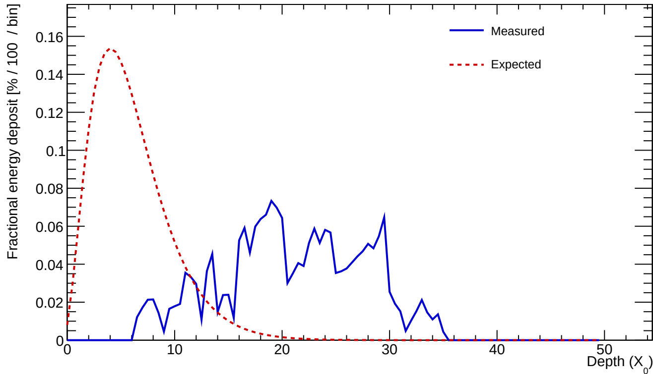
Cluster 179 E=4.407 GeV profileStart=15.00 X_0 \chi=0.7423
