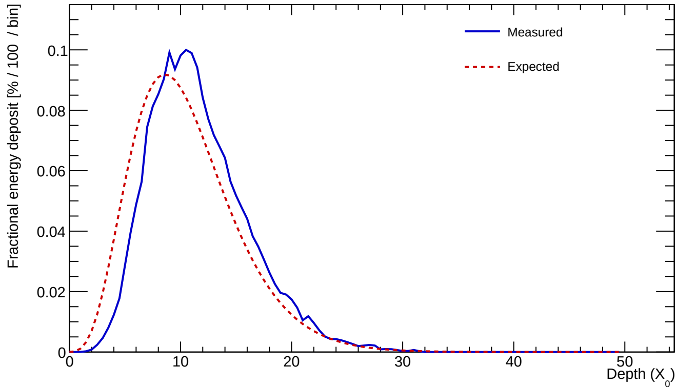
Cluster 133 E=430.550 GeV profileStart=1.00 X_0 \chi=0.0730
