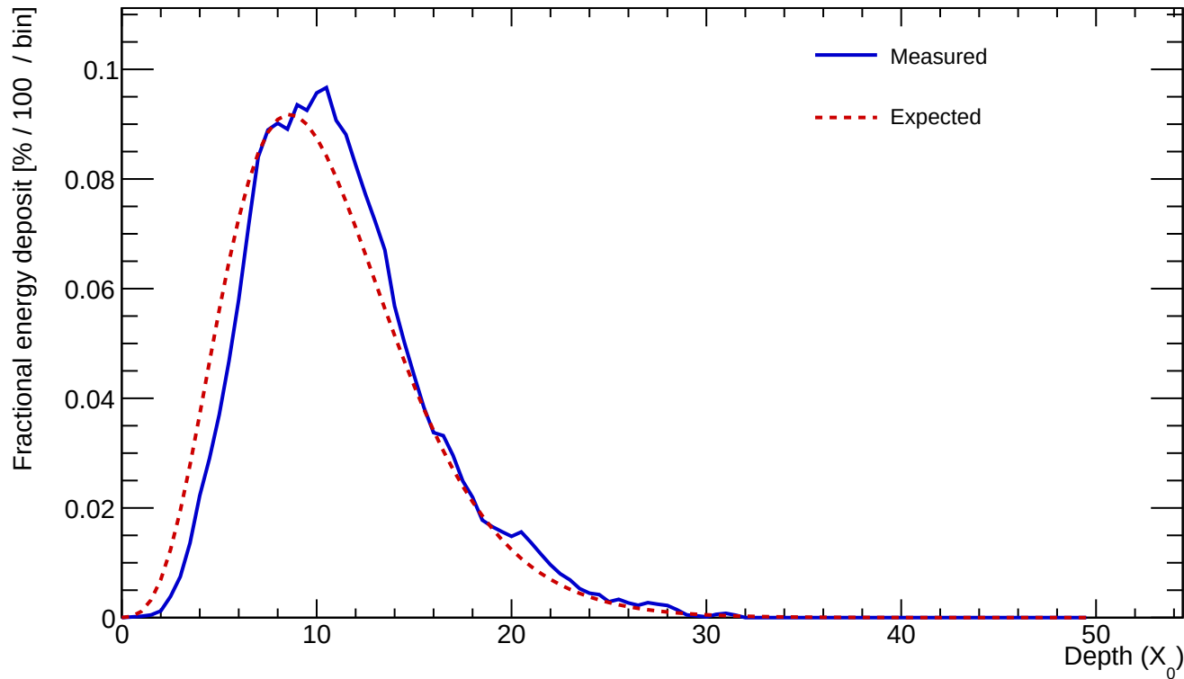
Cluster 21 E=437.123 GeV profileStart=1.00 X_0 \chi=0.0744
