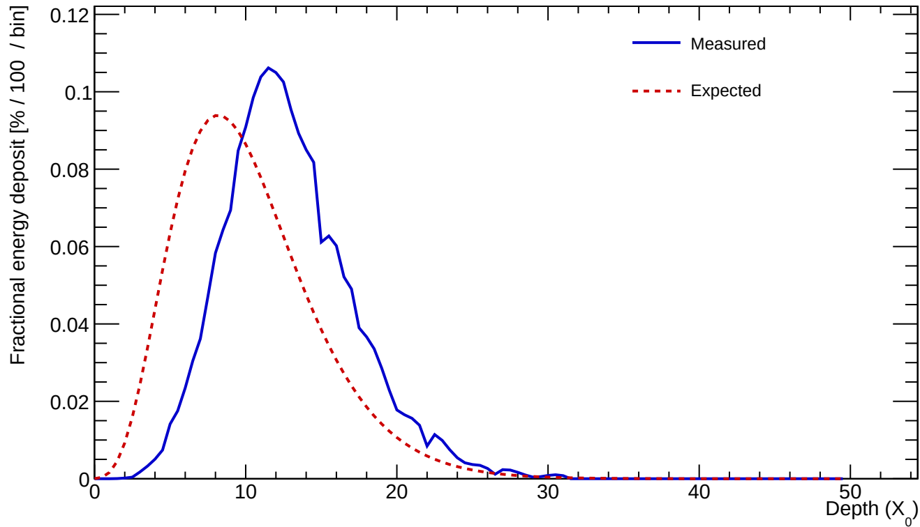
Cluster 62 E=287.505 GeV profileStart=3.00 X_0 \chi=0.1073
