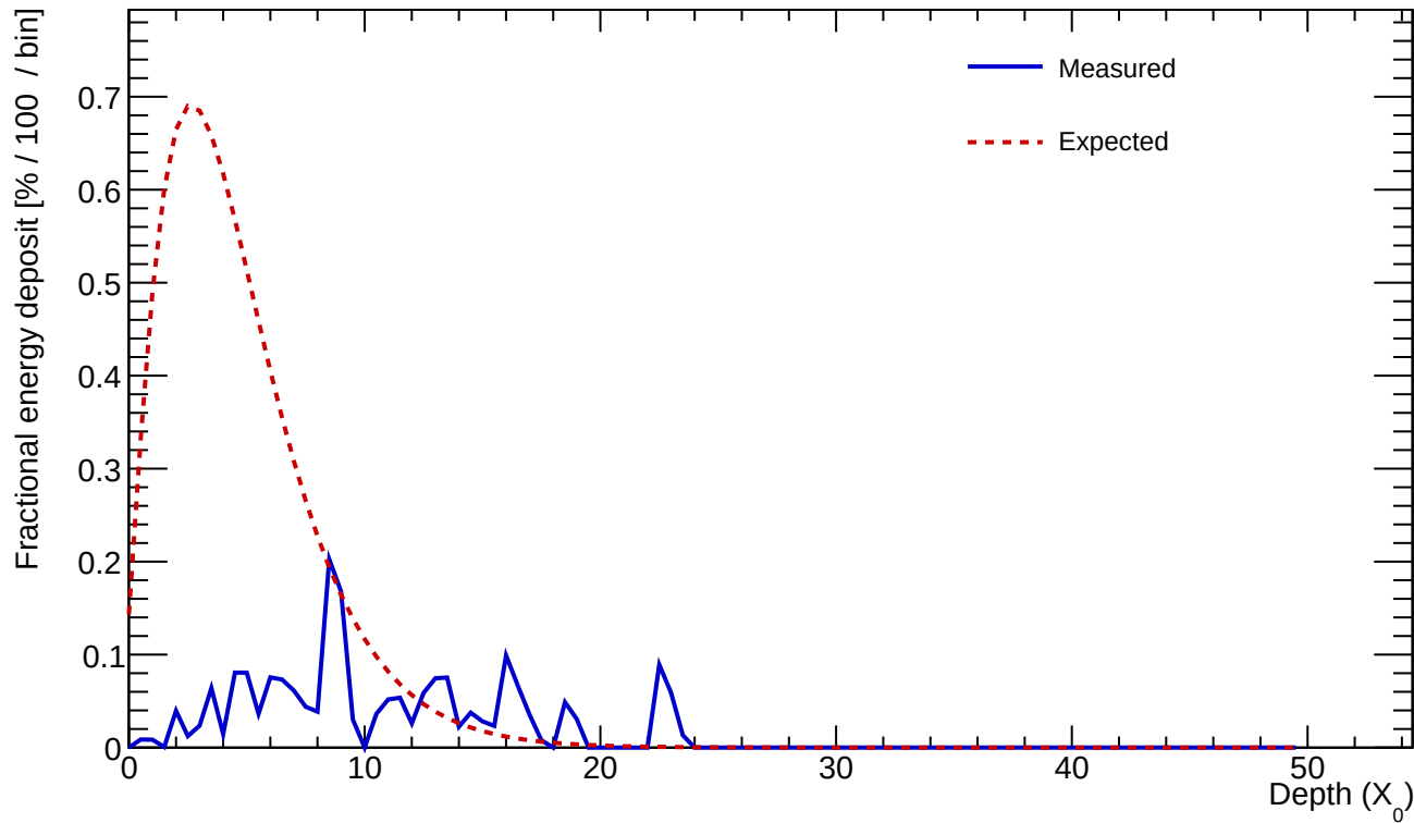
Cluster 167 E=1.133 GeV profileStart=5.50 X_0 \chi=0.8213
