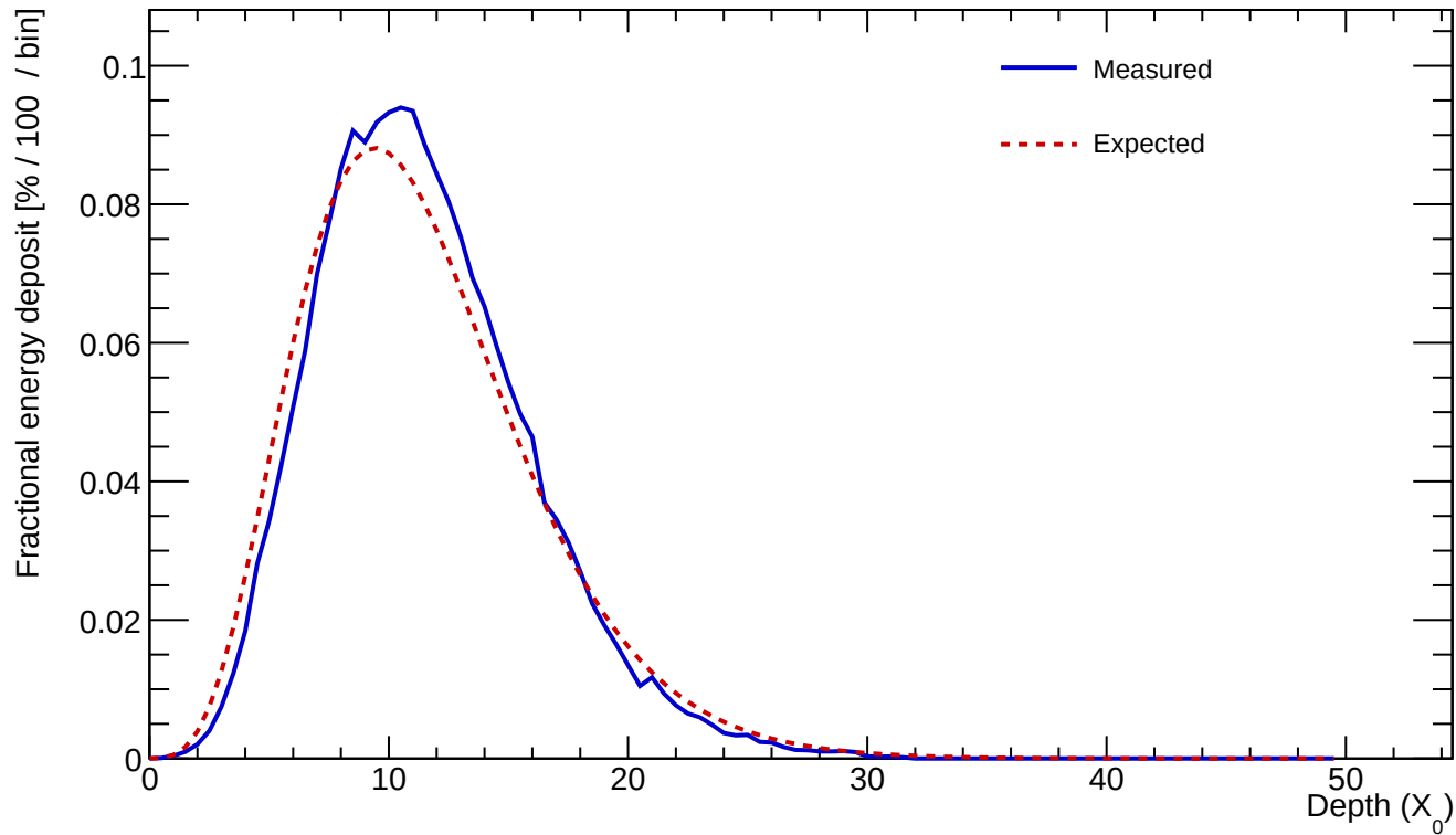
Cluster 53 E=973.936 GeV profileStart=0.50 X_0 \chi=0.0704
