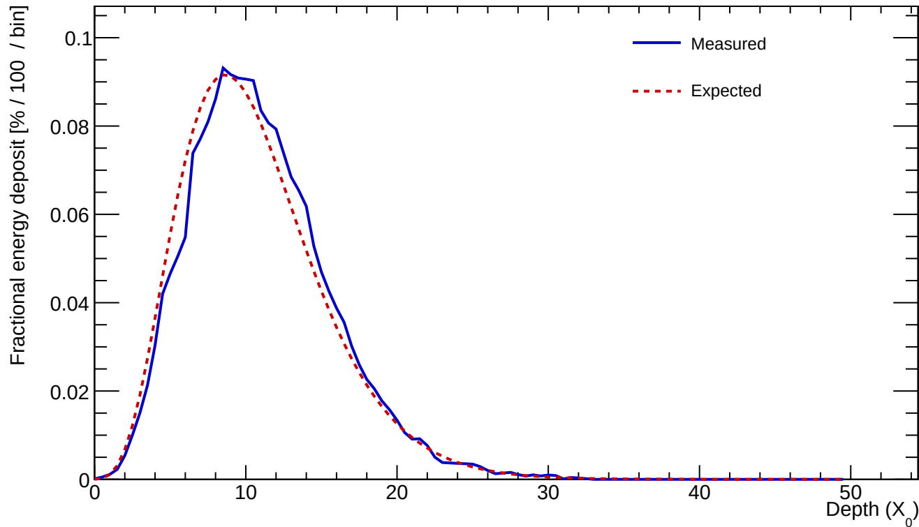
Cluster 48 E=454.072 GeV profileStart=0.50 X_0 \chi=0.0469
