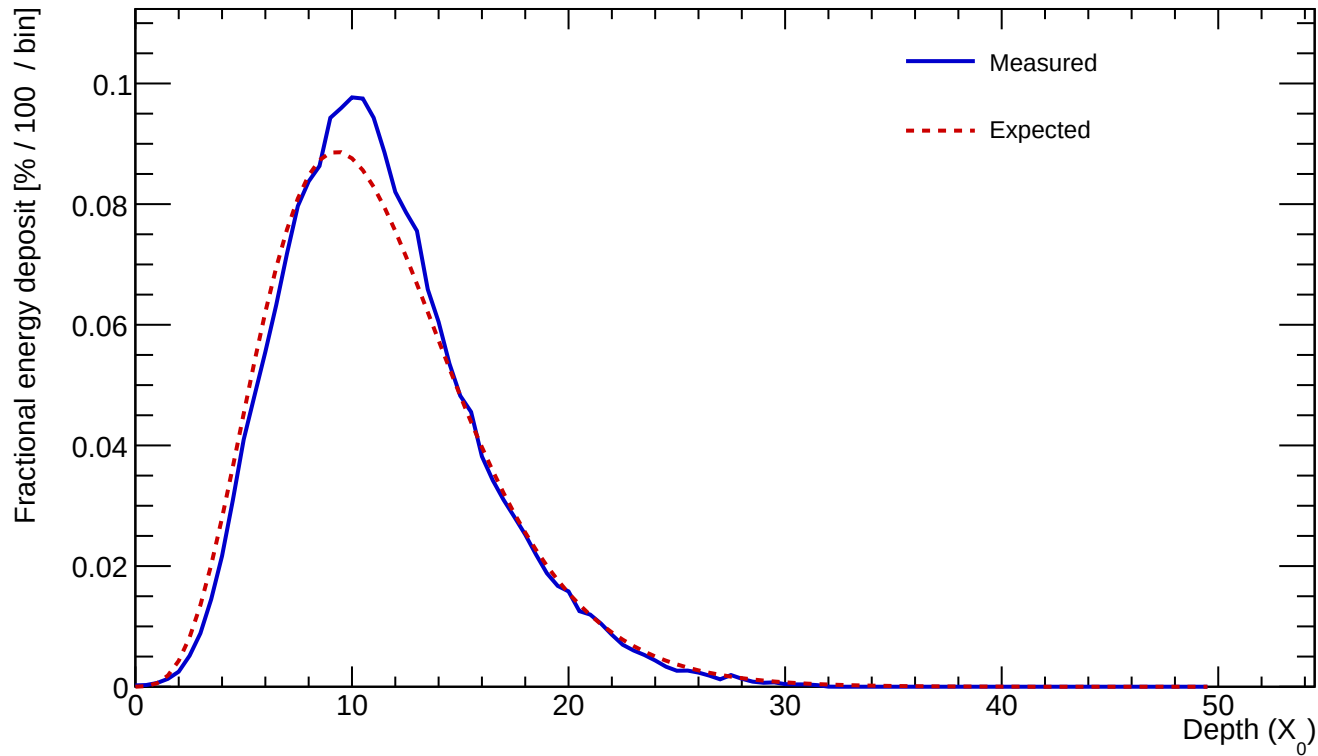
Cluster 15 E=853.050 GeV profileStart=0.50 X_0 \chi=0.0785
