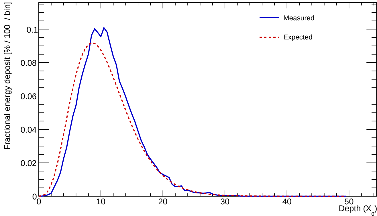
Cluster 65 E=438.574 GeV profileStart=1.00 X_0 \chi=0.0793
