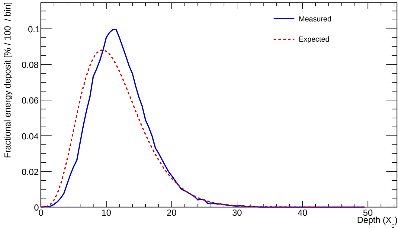
Cluster 5 E=963.523 GeV profileStart=1.00 X_0 \chi=0.1031
