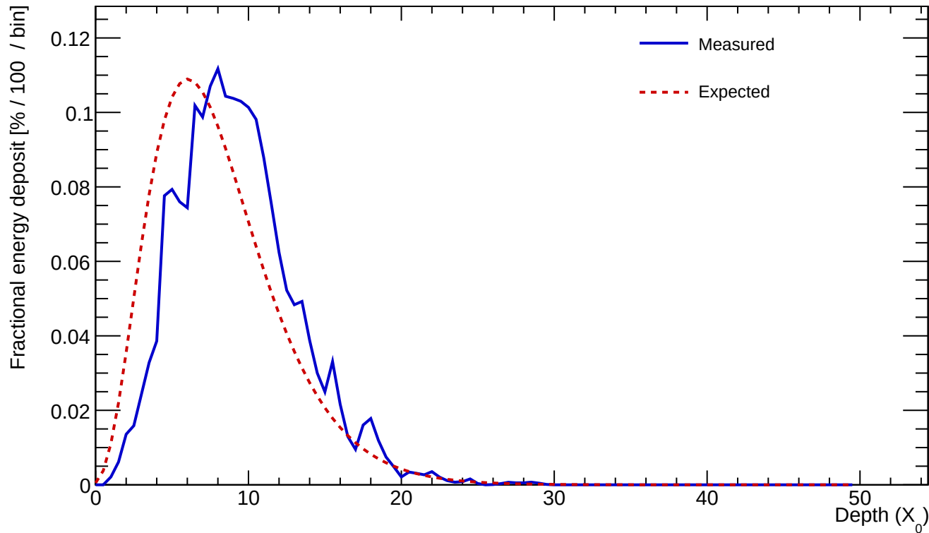
Cluster 163 E=33.305 GeV profileStart=1.50 X_0 \chi=0.1192
