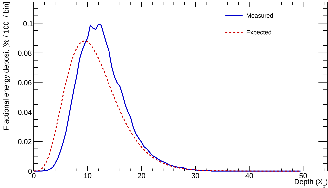
Cluster 229 E=975.725 GeV profileStart=1.50 X_0 \chi=0.1074
