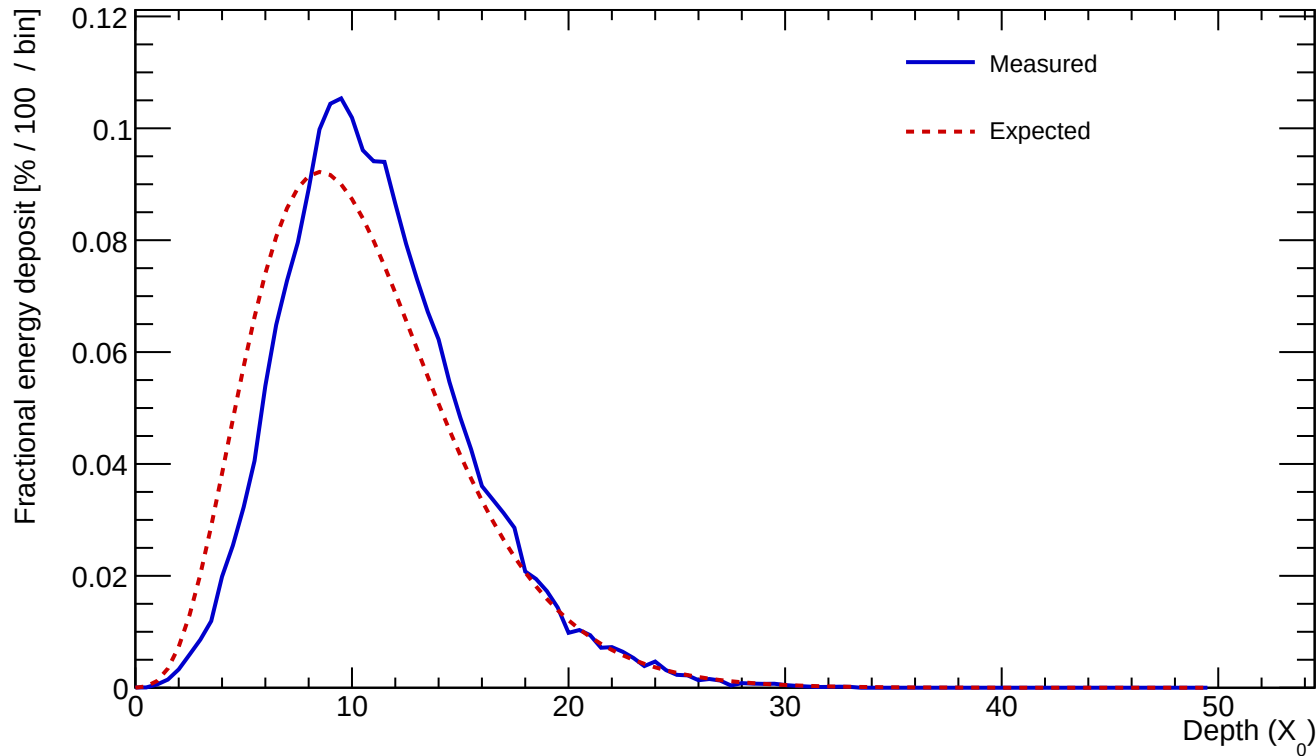
Cluster 34 E=404.431 GeV profileStart=1.00 X_0 \chi=0.0955
