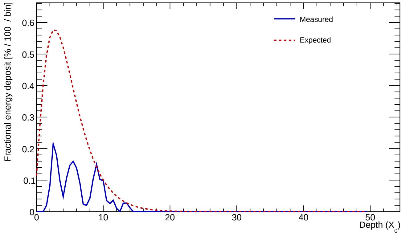
Cluster 68 E=1.191 GeV profileStart=1.50 X_0 \chi=0.4622
