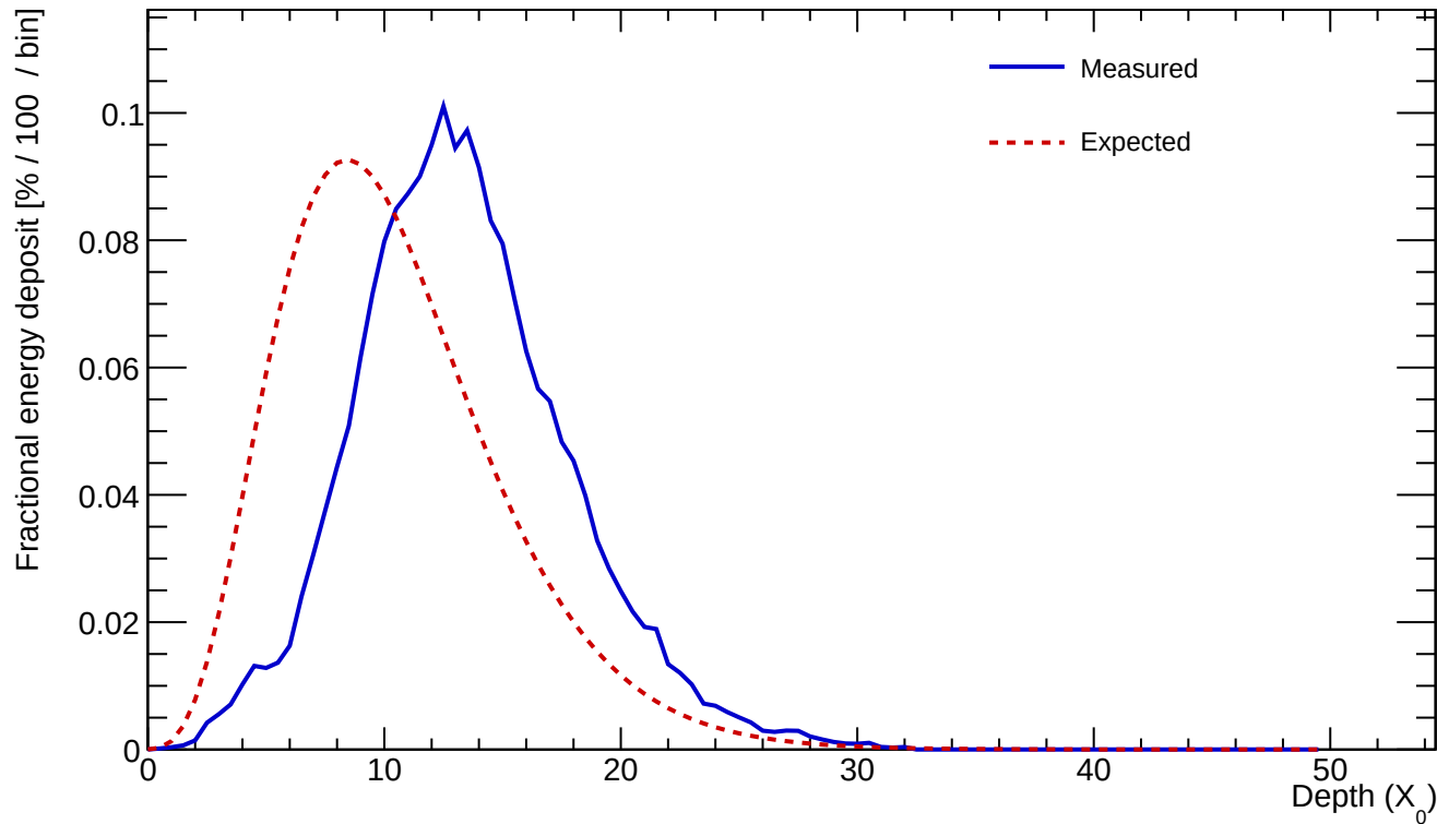
Cluster 87 E=367.868 GeV profileStart=3.50 X_0 \chi=0.1040
