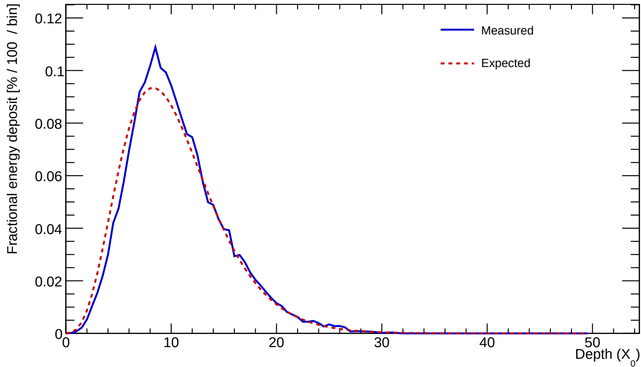
Cluster 245 E=316.114 GeV profileStart=0.50 X_0 \chi=0.0710
