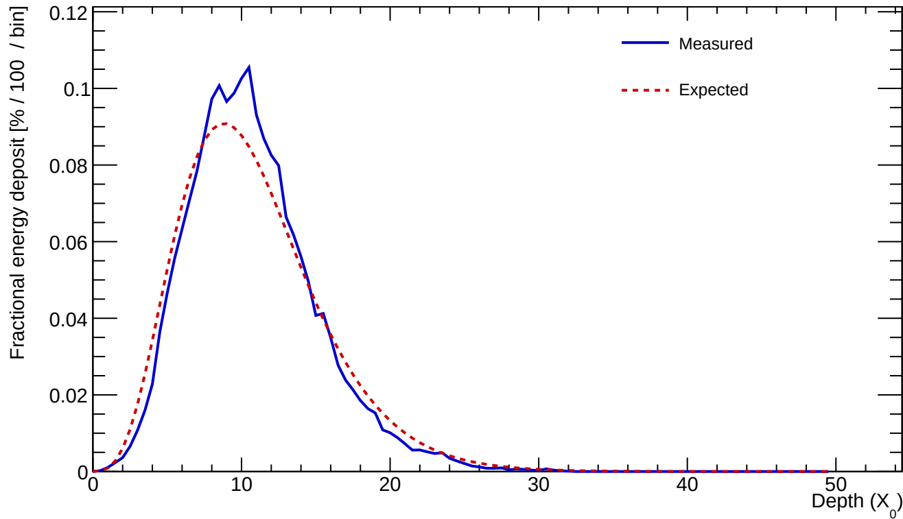
Cluster 23 E=533.003 GeV profileStart=0.50 X_0 \chi=0.1154
