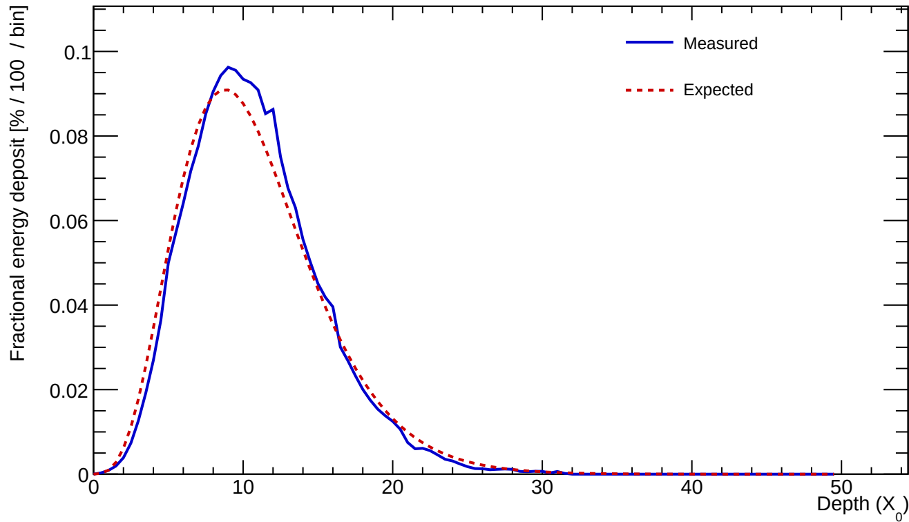
Cluster 138 E=518.001 GeV profileStart=0.50 X_0 \chi=0.0759
