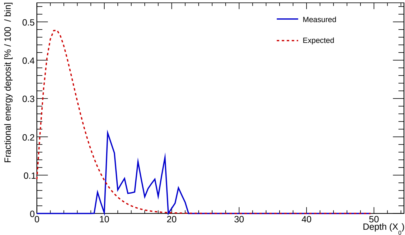
Cluster 45 E=1.271 GeV profileStart=9.00 X_0 \chi=0.5786
