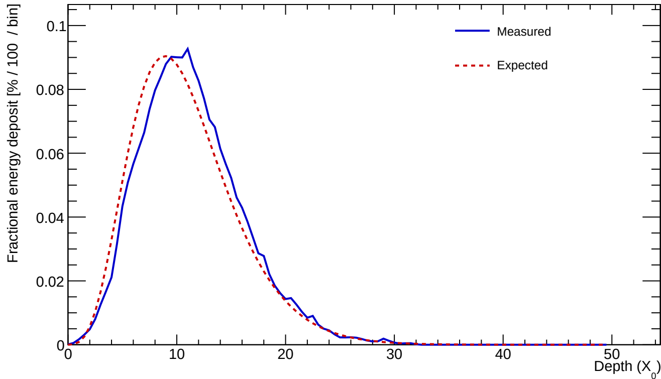
Cluster 201 E=583.510 GeV profileStart=0.50 X_0 \chi=0.0601
