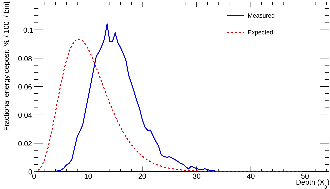
Cluster 67 E=306.698 GeV profileStart=5.50 X_0 \chi=0.0808
