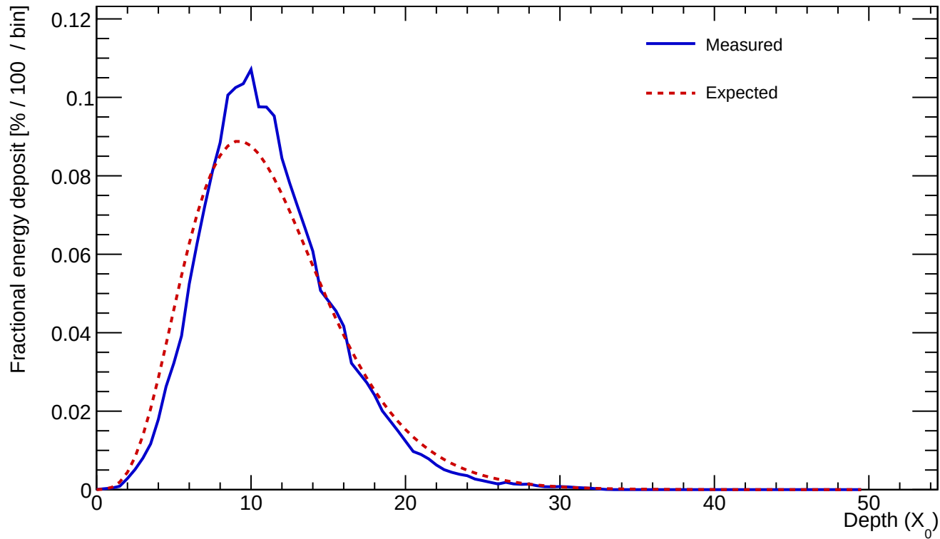
Cluster 164 E=819.030 GeV profileStart=0.50 X_0 \chi=0.1216
