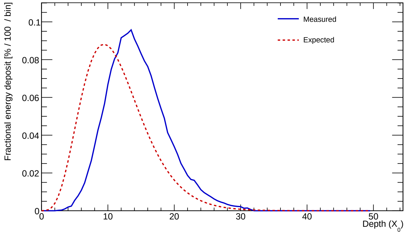
Cluster 133 E=981.253 GeV profileStart=3.50 X_0 \chi=0.0693
