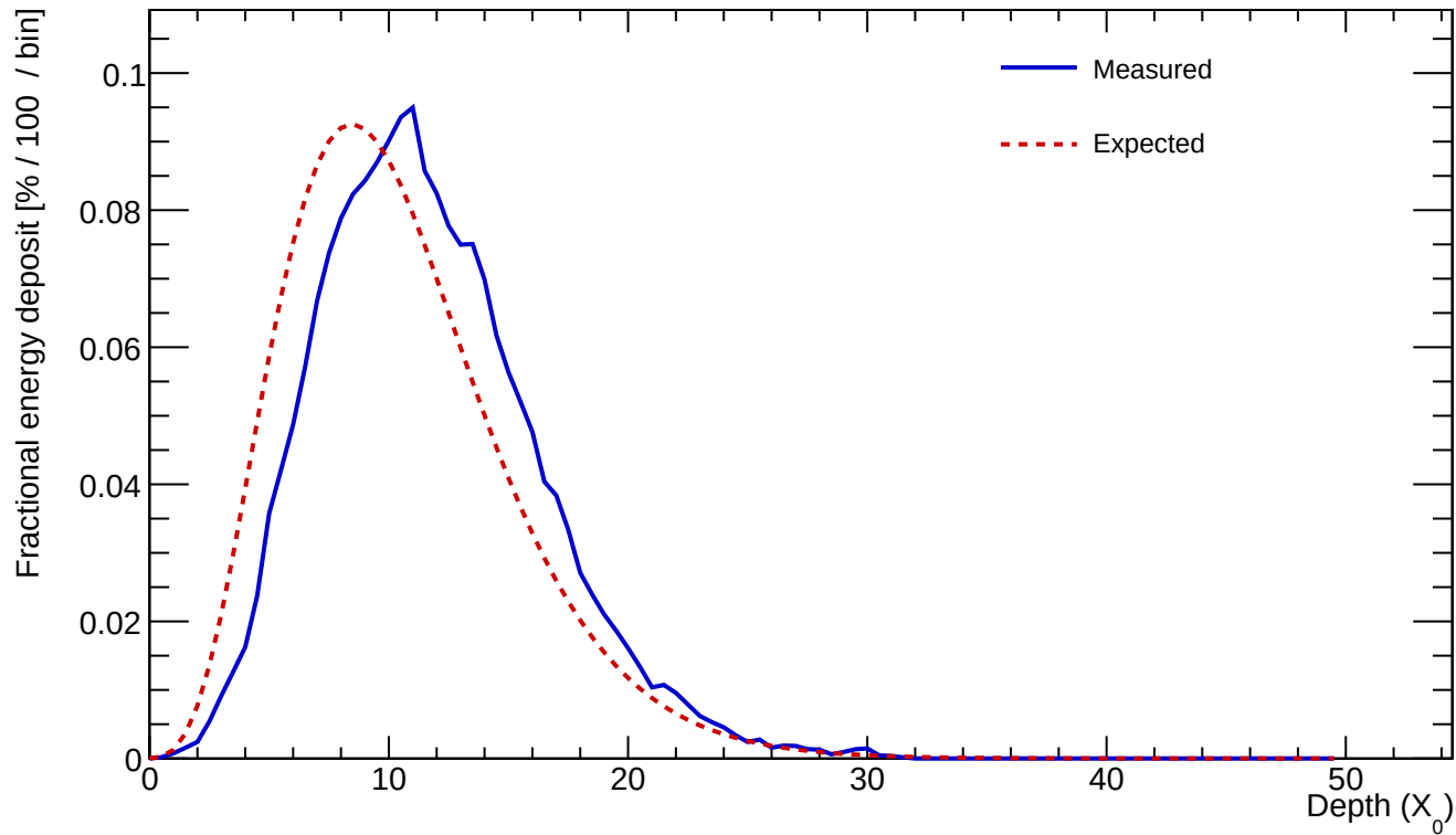
Cluster 149 E=376.058 GeV profileStart=1.50 X_0 \chi=0.0601
