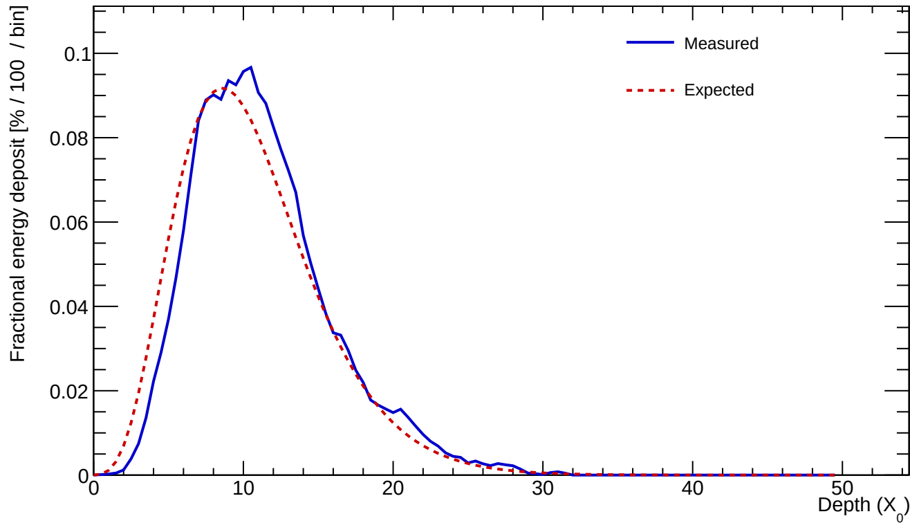
Cluster 16 E=437.123 GeV profileStart=1.00 X_0 \chi=0.0744
