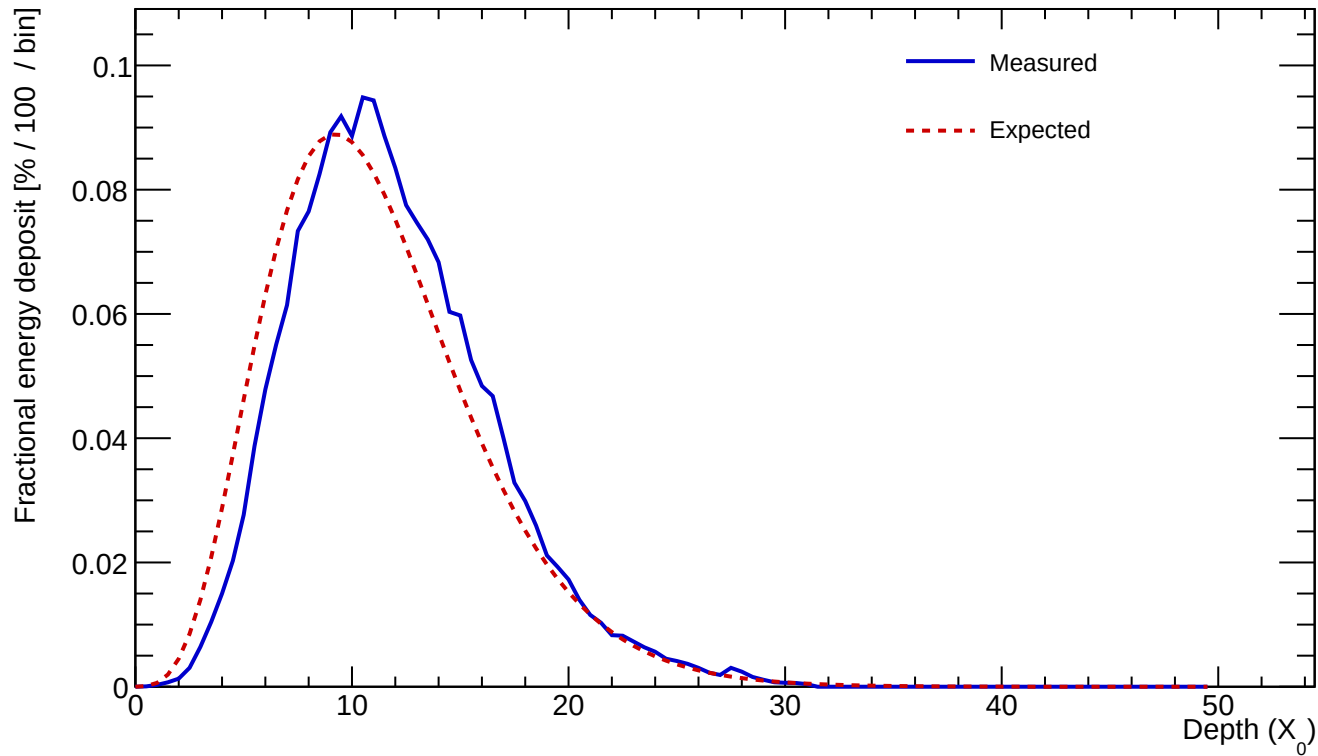
Cluster 115 E=801.341 GeV profileStart=1.00 X_0 \chi=0.0492
