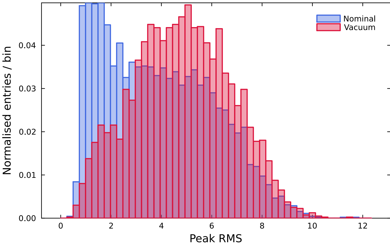
Peak RMS: Nominal vs Vacuum Solenoid
