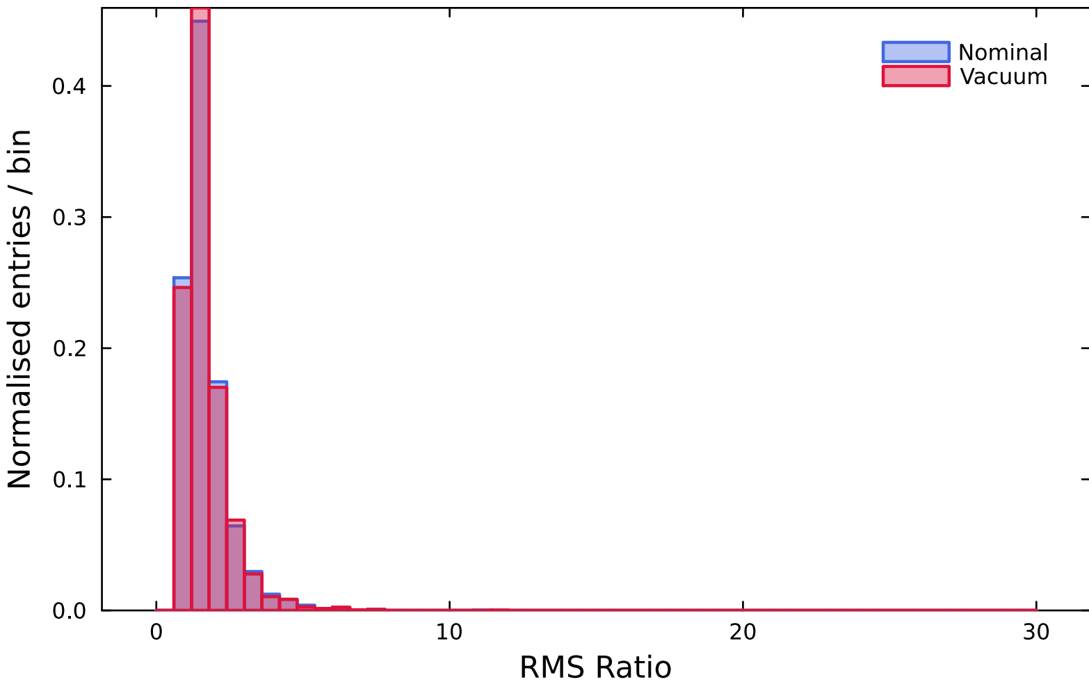
RMS Ratio: Nominal vs Vacuum Solenoid
