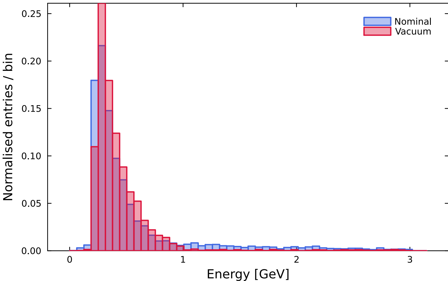
Energy: Nominal vs Vacuum Solenoid
